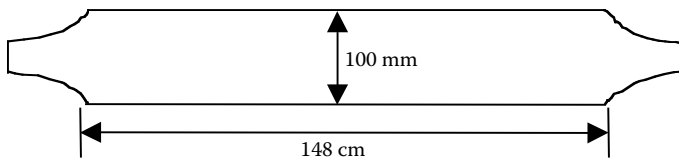
FIGURE 5.3 Fiber composite drive shaft.
