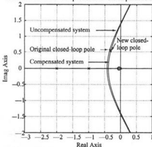
Root-Locus Plots of Compensated and Uncompensated Systems
