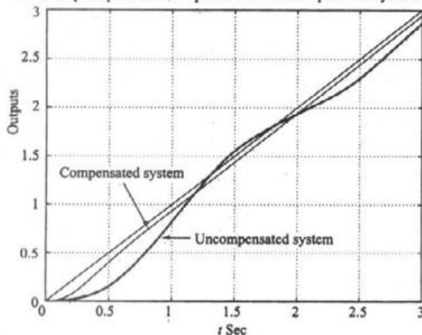
Unit-Ramp Responses of Compensated and Uncompensated Systems
