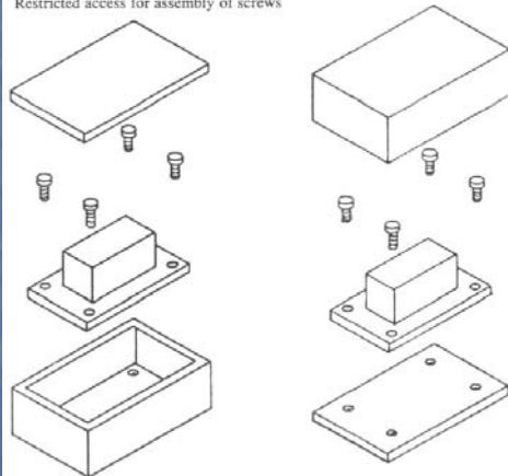
Figure 3.40 Design concept to provide easier access during assembly.
