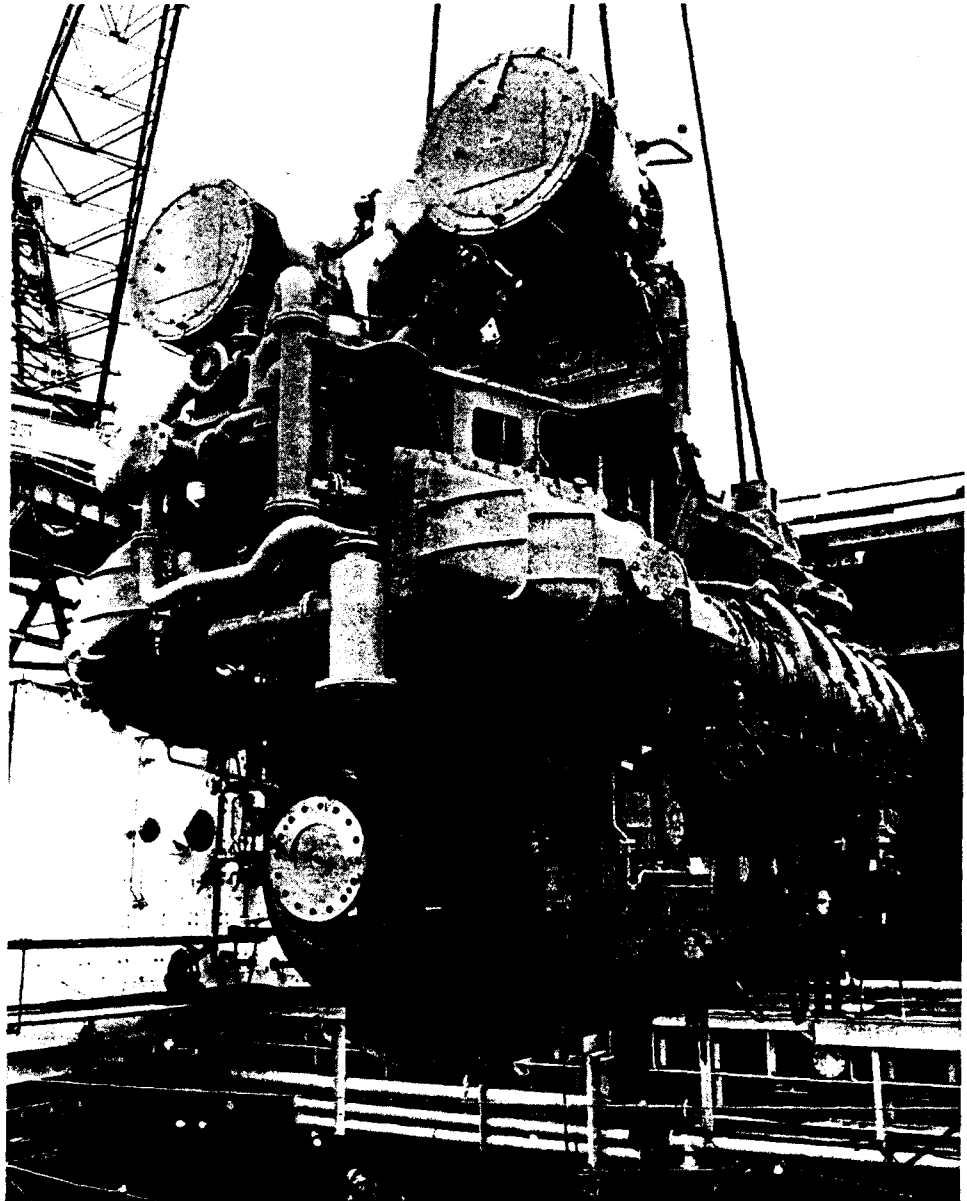
Figure 2-3 Fairbanks Morse ten-cylinder PC4.2 diesel ship engine, capable of producing over 8000 brake horsepower (5970 kW). Printed with permission, Fairbanks Morse Engine Division, Coltec Industries.
