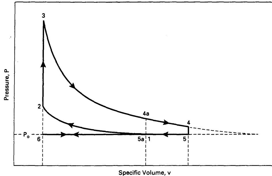
Figure 3-13 Air-standard Atkinson cycle, 6-1-2-3-4-5-6, with larger expansion ratio v_4/v_3 than compression ratio v_1/v_3 . The same engine operating on an Otto cycle would follow cycle 6-1-2-3-4a-5a-6.
