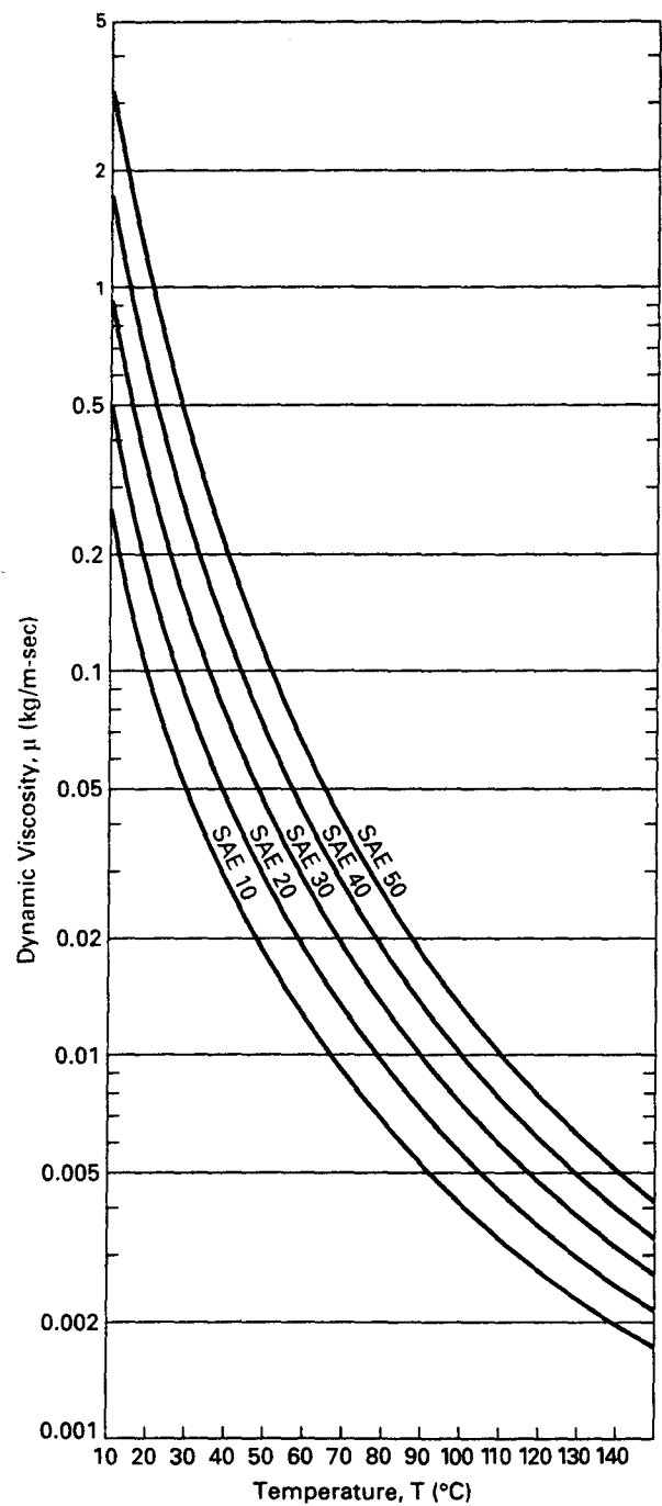
Figure 11-11 Dynamic viscosity as a function of temperature for common engine oils. Adapted from [113].
