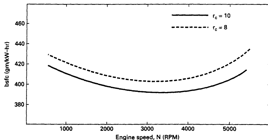
Figure 2-12 Brake specific fuel consumption as a function of engine speed. Fuel consumption decreases as engine speed increases due to the shorter time for heat loss during each cycle. At higher engine speeds fuel consumption again increases because of high friction losses. As compression ratio is increased fuel consumption decreases due to greater thermal efficiency.
