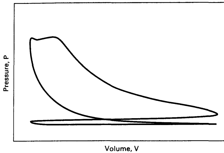
Figure 3-7 Indicator diagram of a historic CI engine operating on an early four-stroke cycle.
