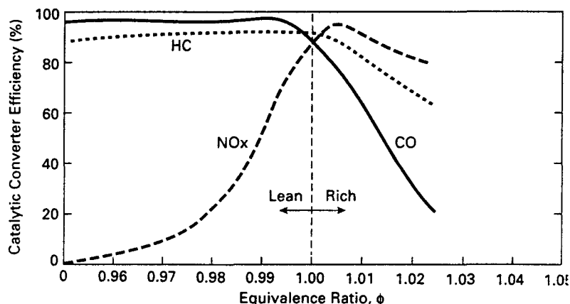
Figure 9-7 Conversion efficiency of catalytic converters as a function of fuel equivalence ratio. Greatest efficiency occurs when engines operate near stoichiometric conditions. Converters are very inefficient for NO x conversion when an engine operates lean. This creates a greater problem for modern CI engines and stratified charge SI engines, which generally operate very lean overall. Adapted from [76].
