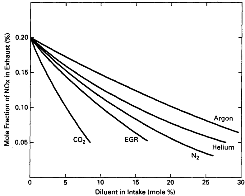
Figure 9-9 Reduction of NOx generation by adding non combustible diluent gas to intake mixture. Adding any non reacting neutral gas to the inlet air–fuel mixture reduces flame temperature and NOx generation. Exhaust gas (EGR) is the one gas that is readily available for engine use. Adapted from [99].
