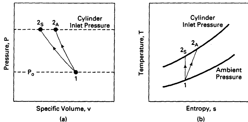
Figure 5-7 Ideal flow process (1-2 s ) and actual flow process (1-2 A ) through a supercharger or a turbocharger compressor in (a) pressure-volume coordinates, and (b) temperature-entropy coordinates.
