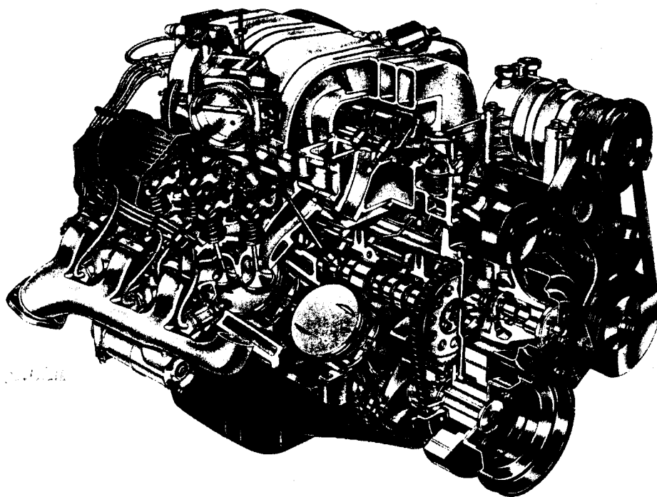
Figure 1-10 General Motors 7.4 liter L29, V8, four-stroke cycle, spark ignition, truck engine. Displacement is 454 in. 3 (7.44 L) with 4.25 in. bore (10.80 cm) and 4.00 in. stroke (10.16 cm). The engine has a maximum speed of 5000 RPM, with a compression ratio of 9.0:1, overhead valves, and multipoint port fuel injection. This engine was used in several models of 1996 Chevrolet and GMC trucks. Copyright General Motors Corp., used with permission.
