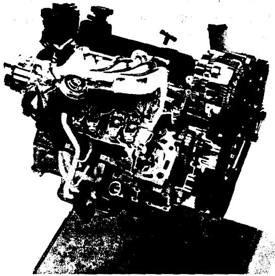
Figure 1-19 Ford 3.0 liter Vulcan V6, spark ignition, four-stroke cycle engine. This was the standard engine of the 1996 Ford Taurus and Mercury Sable automobiles. It is rated at 108 kW at 5250 RPM and develops 230 N-m of torque at 3250 RPM. Courtesy Ford Motor Company.
