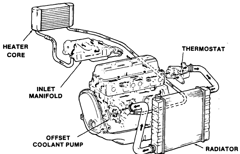
Figure 10-12 Schematic of cooling system of a water-cooled engine. Reprinted with permission from SAE Technical Paper 820111 © 1982, Society of Automotive Engineers, Inc., [135].
