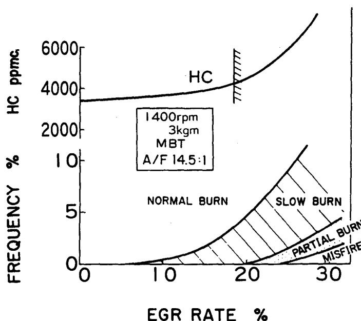
Figure 7-11 Effect of EGR on quality of combustion in an SI engine and hydrocarbon emissions in the exhaust. With no EGR, most cycles will have normal burn time. As the percent of EGR is increased, there will be an increase in cycles with slow burn or partial burn. With too much EGR, combustion in some cycles will die out, resulting in a misfire. Reprinted with permission from SAE Technical Paper 780006 © 1978, Society of Automotive Engineers, Inc., [77].
