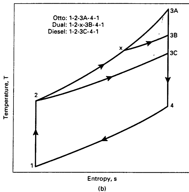
Figure 3-11 Comparison of air-standard Otto cycle, Dual cycle, and Diesel cycle. All engines have the same cylinder input conditions and same compression ratio.
