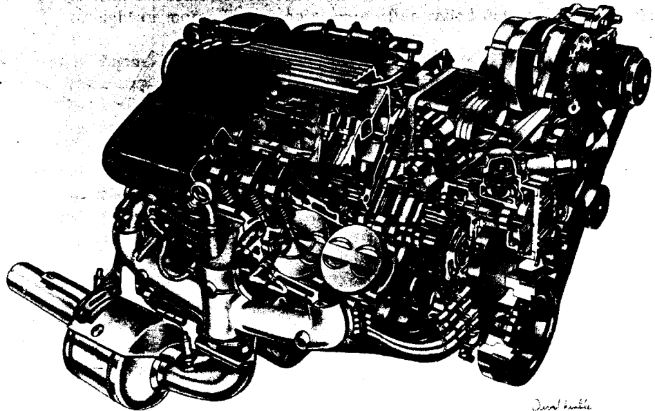
Figure 1-6 Chevrolet LT4 V8, four-stroke cycle, spark ignition engine with 5.7 liter displacement. This fuel-injected, overhead valve engine was an option in the 1986 Corvette. Copyright General Motors Corp., used with permission.
