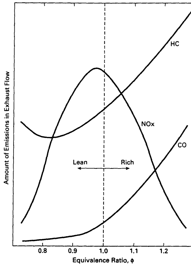
Figure 9-1 Emissions from an SI engine as a function of equivalence ratio. A fuel rich air-fuel ratio does not have enough oxygen to react with all the carbon and hydrogen, and both HC and CO emissions increase. HC emissions also increase at very lean mixtures due to poor combustion and misfires. The generation of nitrogen oxide emissions is a function of the combustion temperature, being greatest near stoichiometric conditions when temperatures are the highest. Peak NOx emissions occur at slightly lean conditions, where the combustion temperature is high and there is an excess of oxygen to react with the nitrogen. Adapted from [58].
