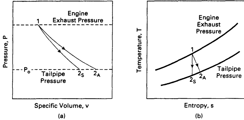
Figure 5-9 Ideal flow process (1-2 s ) and actual exhaust flow process (1-2 A ) through the turbine of a turbocharger in (a) pressure-volume coordinates, and (b) temperature-entropy coordinates. The inlet air flow through the compressor of the turbocharger is the same as shown in Fig. 5-7 for a supercharger.
