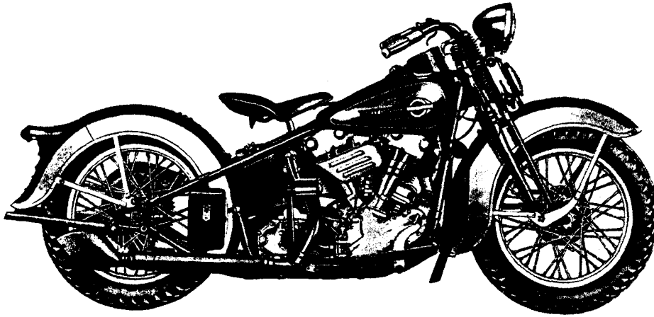
Figure 1-14 Harley-Davidson motorcycle of 1936 powered by "Knucklehead" engine shown in Fig. 1-13. The motorcycle had a rated top speed of 90-95 MPH with a fuel economy of 35-50 MPG. Photograph courtesy of the Harley-Davidson Juneau Avenue Archives. All rights reserved. Copyright Harley-Davidson.
