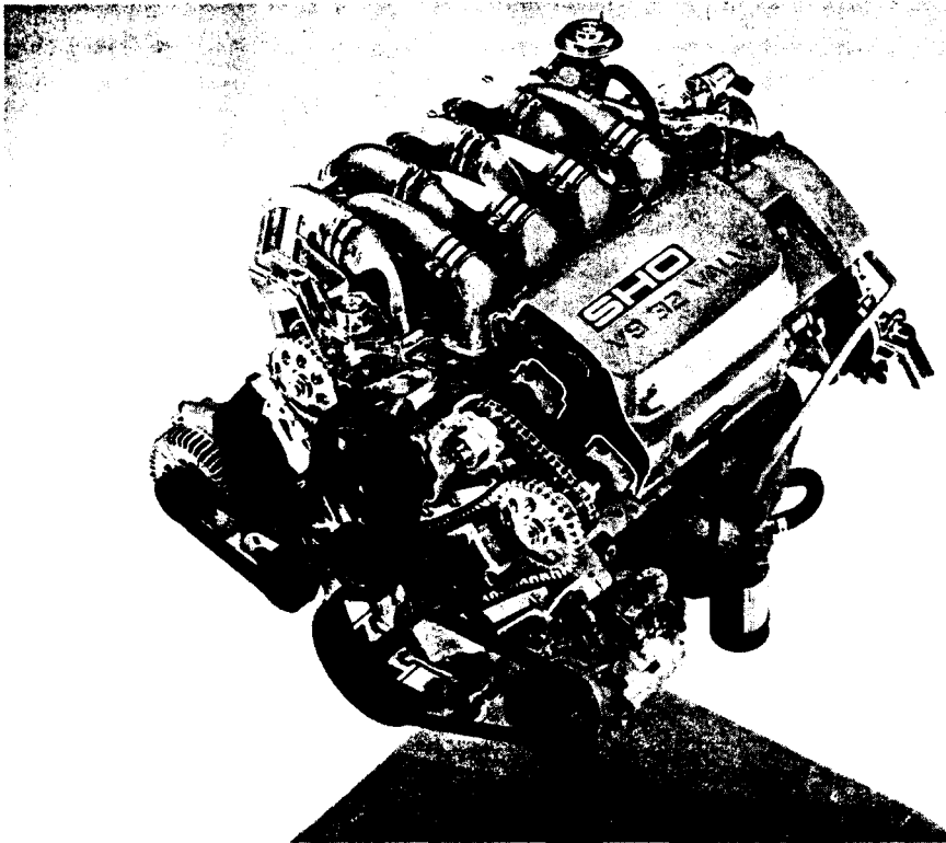
Figure 1-2 Ford Taurus SHO 3.4 liter (208 in. 3 ), spark ignition, four-stroke cycle engine. The engine is rated at 179 kW at 6500 RPM (240 hp) and develops 305 N-m of torque at 4800 RPM (225 lbf-ft). It is a 60° V8 with 8.20 cm bore (3.23 in.), 7.95 cm stroke (3.13 in.), and a compression ratio of 10:1. The engine has four chain driven camshafts mounted in aluminum heads with four valves per cylinder and coil-on-plug ignition. Each spark plug has a separate high-voltage coil and is fired by Ford's Electronic Distributorless Ignition System (EDIS). Courtesy of Ford Motor Company.
