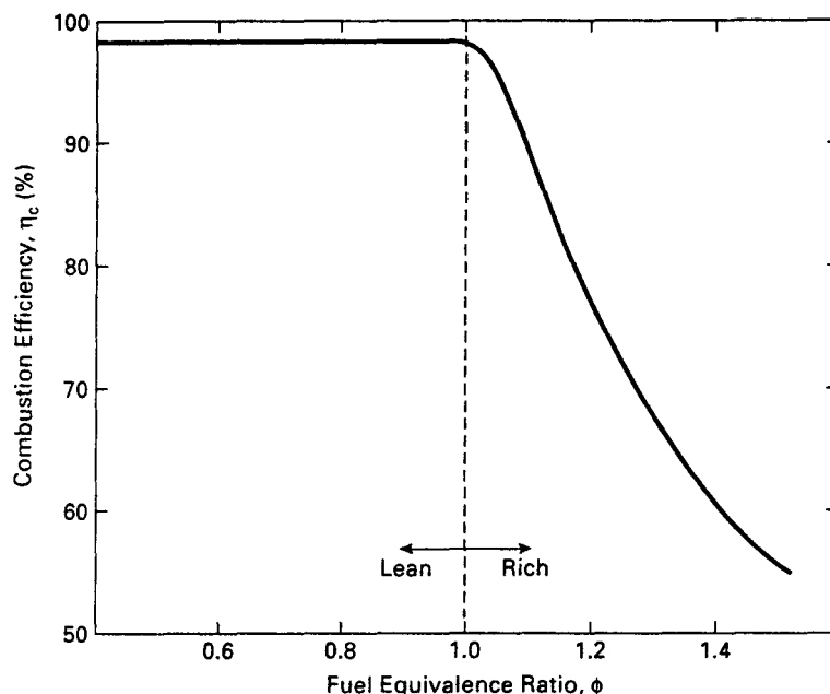
Figure 4-1 Combustion efficiency as a function of fuel equivalence ratio. Efficiency for engines operating lean is generally on the order of 98%. When an engine operates fuel rich, there is not enough oxygen to react with all the fuel, and combustion efficiency decreases. CI engines operate lean and typically have high combustion efficiency. Adapted from [58].
