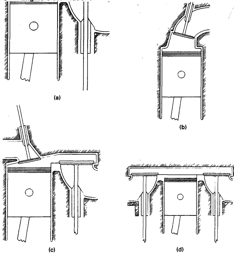
Figure 1-4 Engine Classification by Valve Location. (a) Valve in block, L head. Older automobiles and some small engines. (b) Valve in head, I head. Standard on modern automobiles. (c) One valve in head and one valve in block, F head. Older, less common automobiles. (d) Valves in block on opposite sides of cylinder, T head. Some historic automobile engines.
