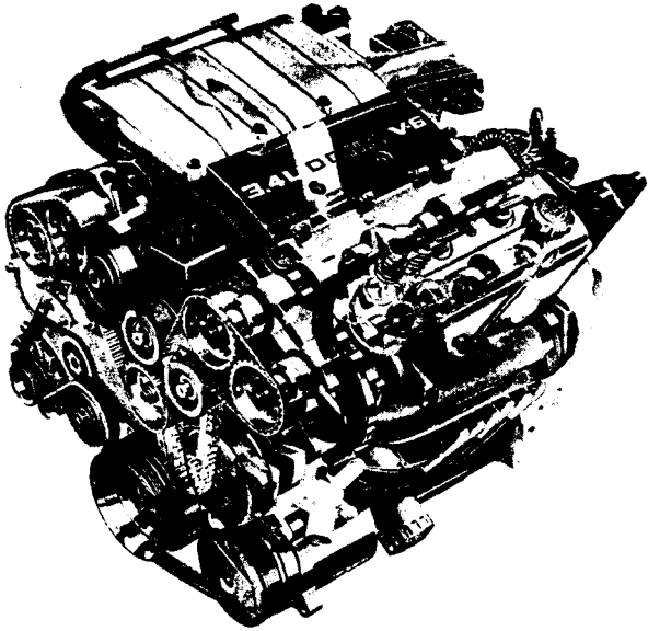
Figure 1-21 General Motors LQ1 3.4 liter V6 engine used in 1996 Chevrolet Lumina, Pontiac Grand Prix, and Oldsmobile Cutless automobiles. This engine has a compression ratio of 9.7:1, bore of 9.203 cm (3.62 in.), stroke of 8.400 cm (3.31 in.), and a maximum speed of 6750 RPM. It has a power rating of 215 hp (160 kW) at 5200 RPM and a torque rating of 220 lbf-ft (298 N-m) at 4000 RPM. Four valves per cylinder are actuated by two overhead camshafts per cylinder bank. The engine heads and intake manifold are made of cast aluminum while the engine block, exhaust manifolds, camshafts, and crankshaft are made of cast iron. Copyright General Motors Corp., used with permission.
