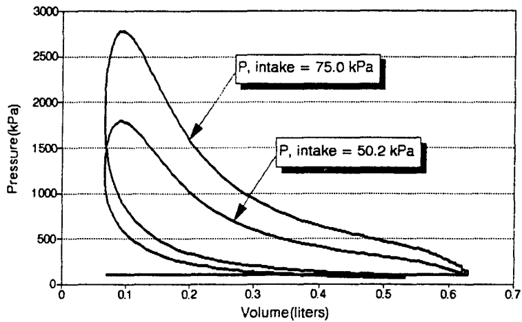
Figure 6-11 Output from General Motors simulation program showing how intake pressure affects pressure-volume indicator diagram of cycle. Reprinted with permission from [41].
