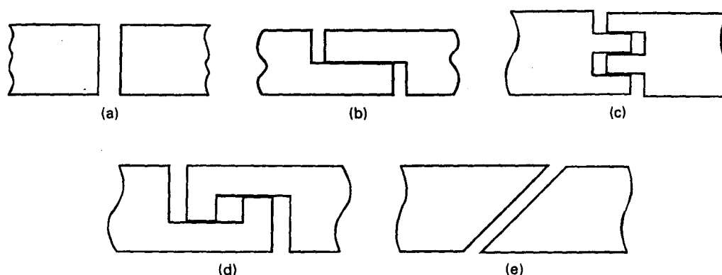
Figure 6-9 Various designs used on the ends of piston rings to reduce blowby flow. Adapted from [34].
