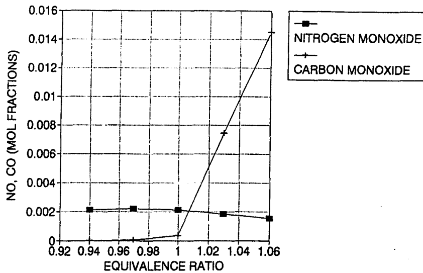
Figure 6-12 Output from General Motors simulation program showing how NO and CO exhaust concentrations are affected by intake equivalence ratio. Reprinted with permission from [41].
