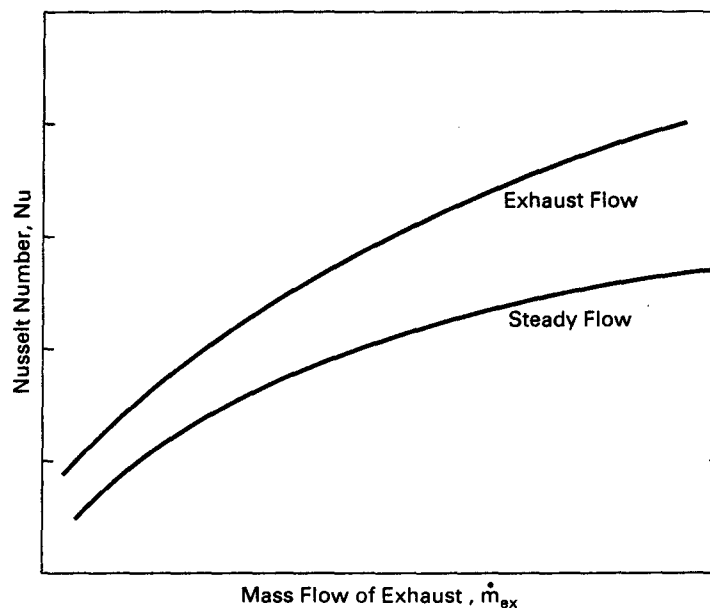
Figure 10-9 Average Nusselt number in the exhaust flow of a reciprocating IC engine. The cyclic pulsing that occurs in the exhaust increases the Nusselt number and convection heat transfer in the exhaust pipe by a factor of about 1.5 over steady flow conditions of equal mass flow rate. Adapted from [82].
