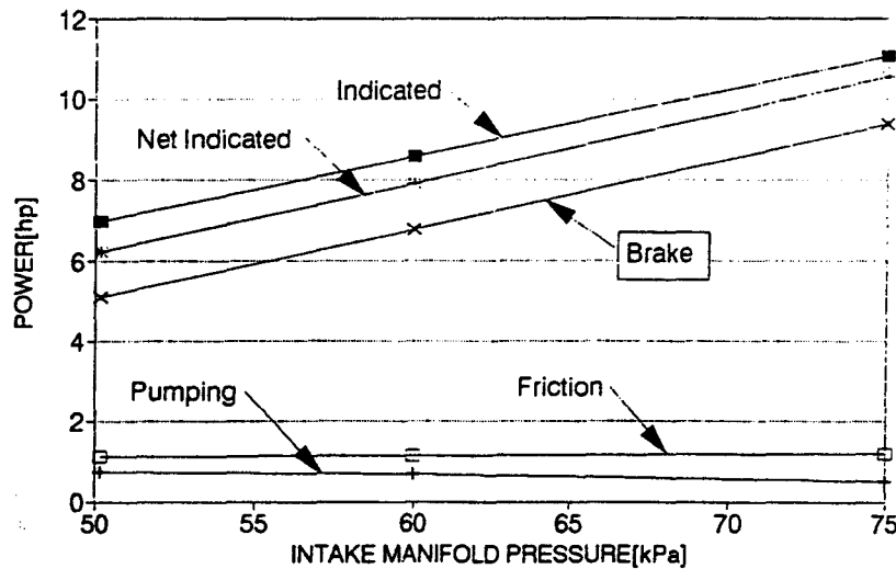
Figure 6-14 Output from General Motors simulation program showing output power as a function of intake pressure. Reprinted with permission from [41].
