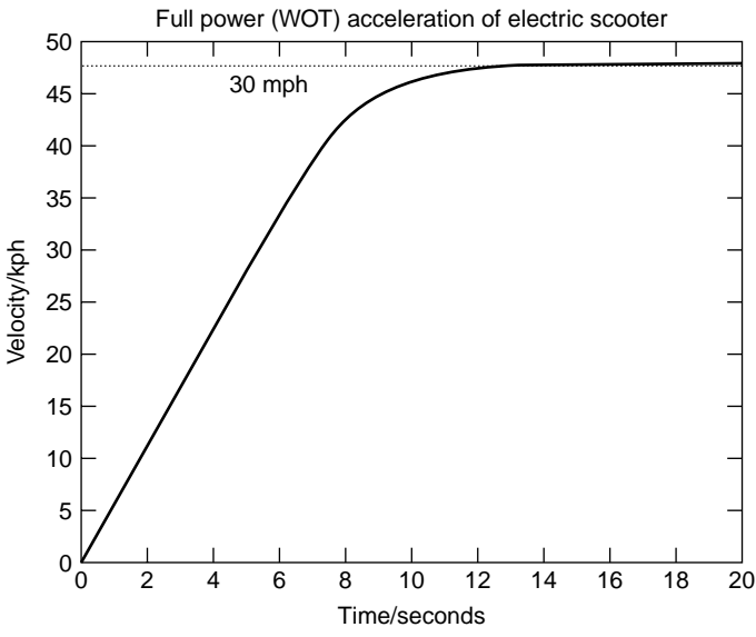
Figure 7.4 A graph showing the acceleration of a design of electric scooter, being the solution of equations (7.15) and (7.16), as approximated by equations (7.17) and (7.18), with a 0.1 s time step
