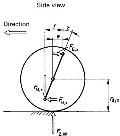
Fig. 3.146 If the spring is supported on the lower suspension control arm and if the front axle has caster, the supporting ball joint will be in front of the wheel centre. Forces F_{Z,W} and F_{G,z} form a moment, which generates the reaction forces -F_{E,x} and +F_{G,x} in the direction of the suspension control arm axes of rotation. In the example these are assumed to be parallel to the ground.
