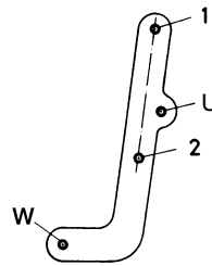
Fig. 3.8 Template for easy calculation of alteration in track, can be used on double wishbone suspensions (Fig. 3.7) and longitudinal link axles (Fig. 3.9).
