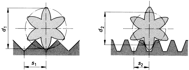
Fig. 3.97 If the steering rack is designed in such a way that the pinion gear is given a larger pitch circle ( d_1 , left) in the middle than on the outside ( d_2 , right), the rack travel reduces from s_1 to s_2 as the wheels are turned more: the ratio becomes larger, the rack moment smaller (illustration: ZF).
