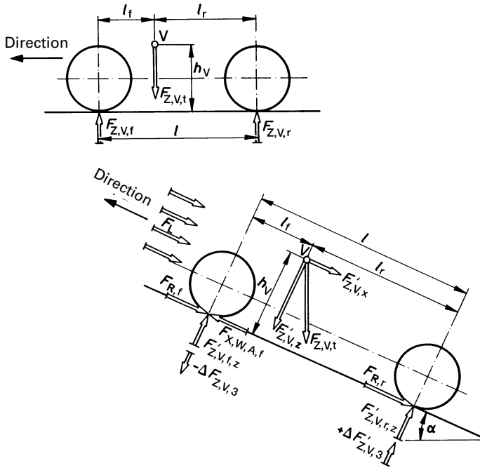
Fig. 6.21 Paths and forces necessary for calculating the skid point, shown on a front-wheel drive vehicle that is travelling up an incline at a constant speed.
