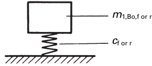
Fig. 5.7 On the simple vibration system, the level of the body frequency n_{f \text{ or } r} (front or rear) depends only on the weight or mass proportion m_{1,Bo,f \text{ or } r} of the body over a front or rear axle side and the spring rate c_{f \text{ or } r} , which on linear springing is a quotient of force and travel: c_{f \text{ or } r} = F/s . On progressive springing, the change in force \Delta F over a minimum travel range \Delta s plays a part c_{f \text{ or } r} = \Delta F/\Delta s (see Fig. 5.12).
