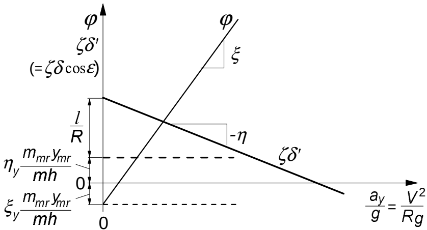
Fig. 10.16. The ground steer angle \delta' and the roll angle \phi due to path curvature 1/R and c.g.lateral offset y_{mr} and the variation with lateral acceleration a_y .
