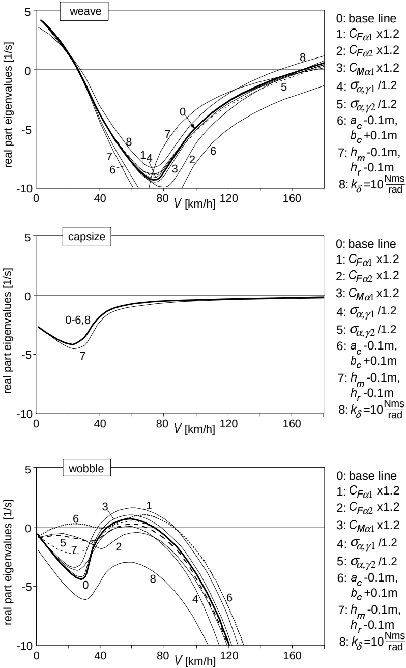
Fig. 10.9. Effect of realistic changes in parameter values on stability characteristics.
