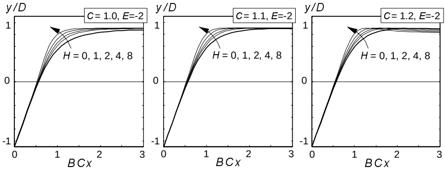
Fig. 4.11. Sharpness of curves near the peak may be increased by introducing additional term with additional sharpness factor H (according to Eq.(4.55)).
