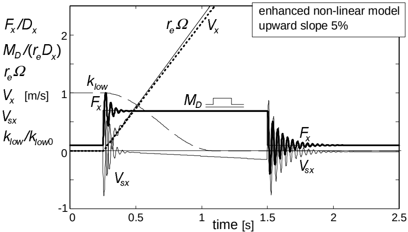
Fig. 8.32. Same simulation as in Fig. 8.31 but now using the enhanced non-linear transient tyre model with carcass compliance ( V_{low} = 2.5\text{m/s} ). Only at low speed a frequency difference can be observed to occur. Very similar results are obtained with the fully non-linear transient models with changing relaxation length.
