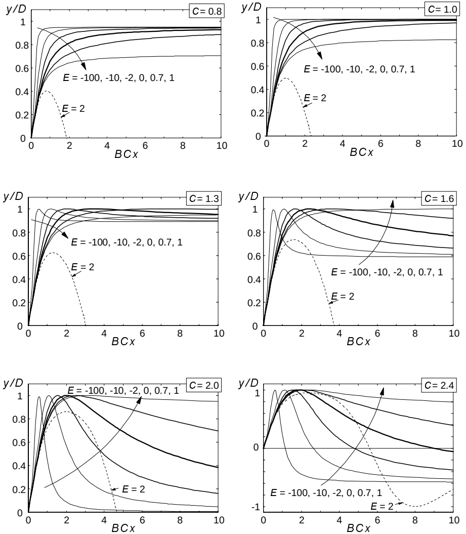
Fig. 4.10. The influence of the shape factors C and E on the appearance of the curve according to Eq.(4.49). Note that a value of E > 1 does not produce realistic curves with peak values < D .
