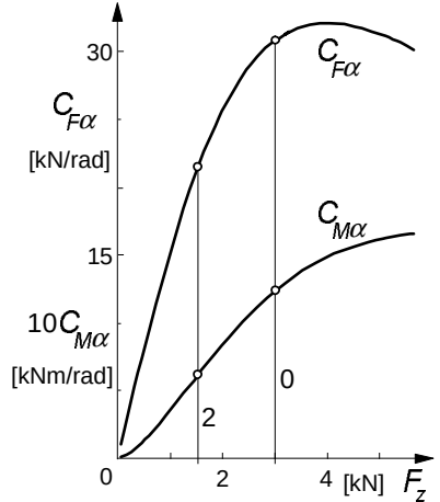
Fig.4.4. Cornering and aligning stiffness versus wheel load.
