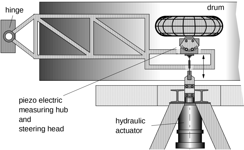
Fig. 9.38. The trailing arm ‘pendulum’ test rig exciting the tyre almost purely laterally. Frequencies up to ca. 25 Hz adequate for assessing the tyre relaxation length and gyroscopic coupling parameter.
