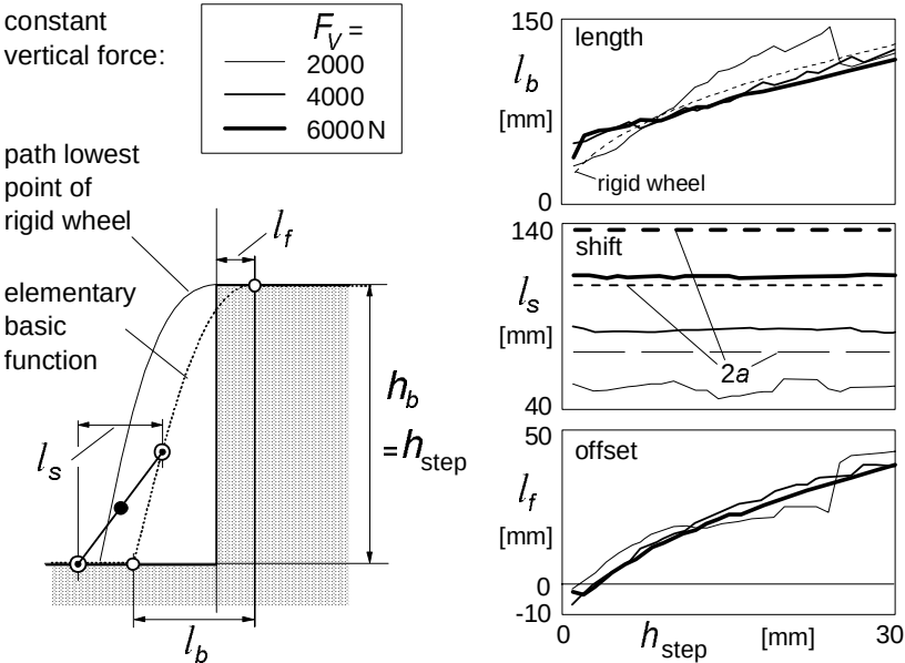
Fig. 9.54. Parameter values for the elementary basic curve established at constant vertical loads by computations using a flexible ring model with tread elements, Zegelaar (1998).
