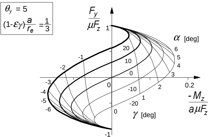
Fig. 3.29. The corresponding Gough plot
