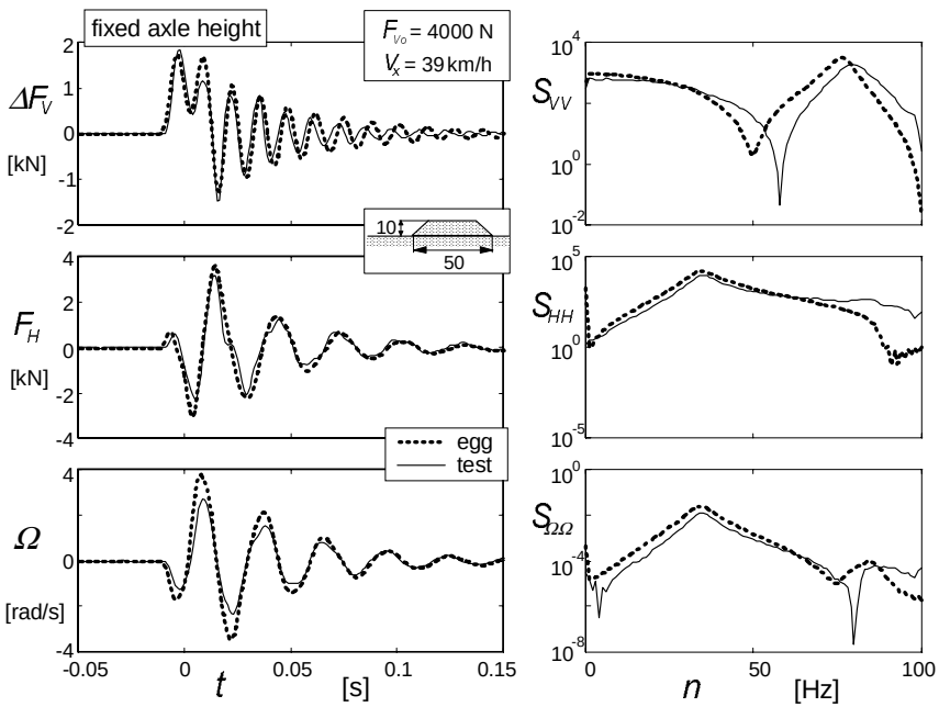
Fig. 9.66. Same as Fig.9.65 but at different speed.
