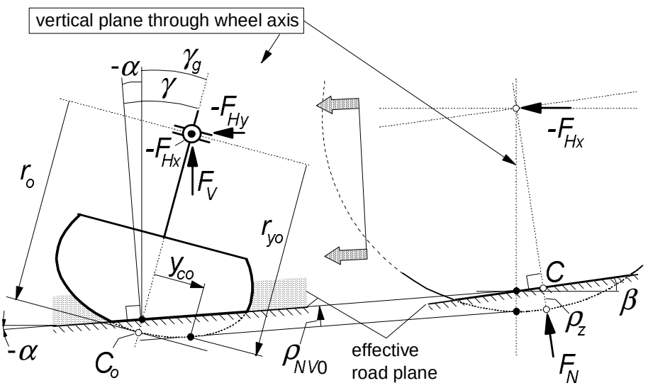
Fig. 9.71 . Situation with wheel camber \gamma and road camber \alpha at a forward slope \beta .
