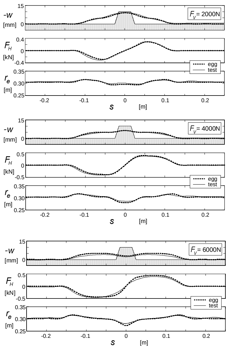
Fig. 9.63. Rolling over a trapezium cleat (length: 50mm, height: 10mm). Measured and calculated variation of vertical axle displacement, horizontal longitudinal force and effective rolling radius at three different constant vertical loads. Measurements carried out on the Delft flat plank machine (very low speed) and calculations conducted with the use of the tandem egg technique (Fig. 9.56) and Eq. (9.258). Tandem egg parameters according to Table 9.6.
