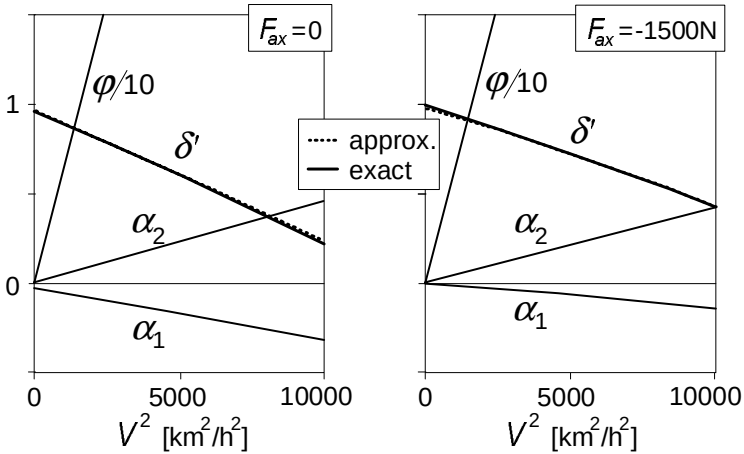
Fig. 10.17. Steer, roll and slip angles per unit non-dimensional path curvature l/R versus speed squared V^2 = a_y R (left: non-accelerating, right: braking) according to the exact and approximate theories.
