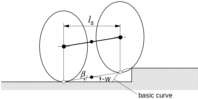
Fig. 9.56. The two-egg tandem configuration of Schmeitz, generating the effective road height and slope.
