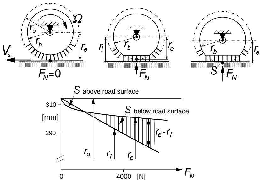
Fig. 9.59. The effective rolling radius varying with a change in normal load.
