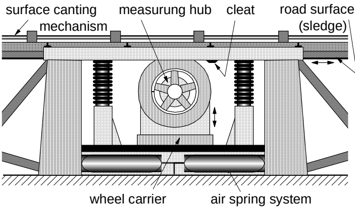
Fig. 9.62. The Delft flat plank machine with stroke of 7m and road canting system, cf. Fig. 7.11.
