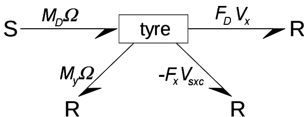
Fig. 9.33. Power flow diagram (bond graph) of driven tyre wheel combination in steady state.
