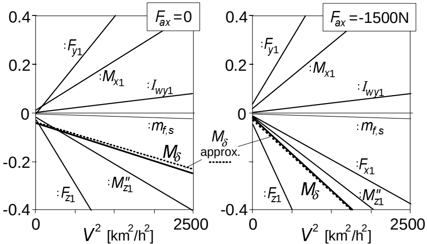
Fig. 10.20. The non-dimensional steer torque ( M_\delta/(F_{z10}l) ) and its components (cf. Eq.(10.147)) per unit non-dimensional path curvature 1/R . In M''_{z1} the F_{x1} contribution is omitted.
