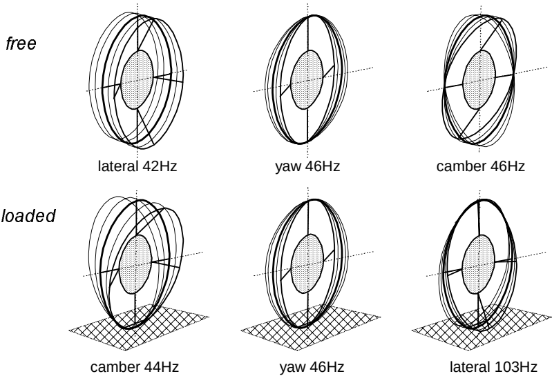
Fig. 9.40. Calculated out-of-plane vibrational modes of tyre/wheel system with axle fixed and tyre free or loaded on the drum surface with vertical load F_N = 4000\text{N} and zero speed.
