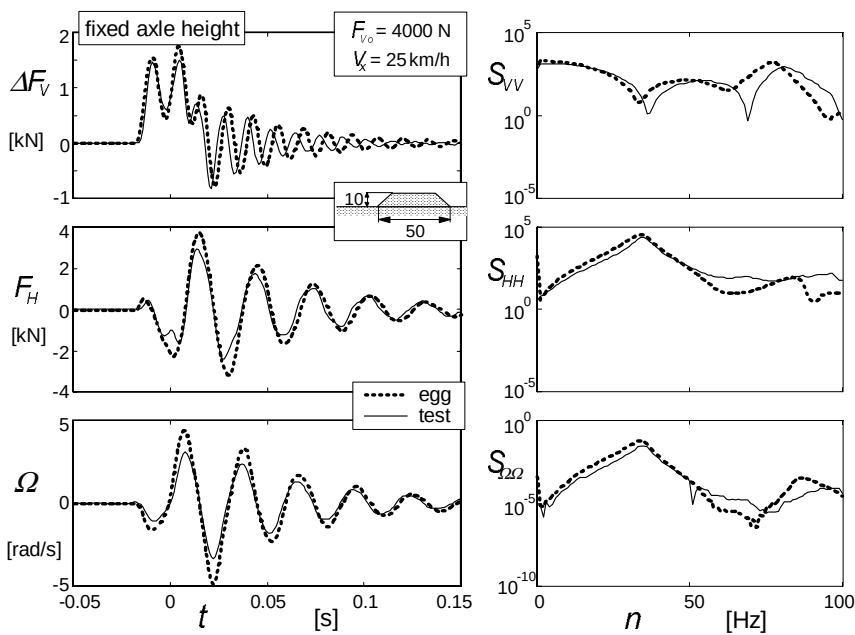
Fig. 9.65. Same as Fig.9.64 but at different speed and initial vertical load .
