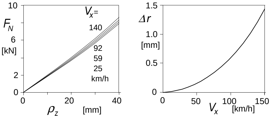
Fig. 9.31. Vertical load vs radial deflection characteristics at various forward velocities and tyre radius growth with speed.
