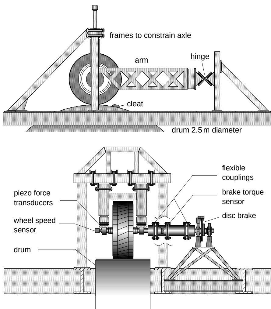
Fig. 9.37. Dynamic brake and cleat test facility in side and front view.
