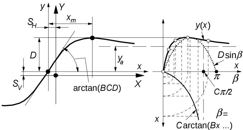
Fig. 4.9. Curve produced by the original sine version of the Magic Formula, Eqs.(4.49). The meaning of curve parameters have been indicated.
