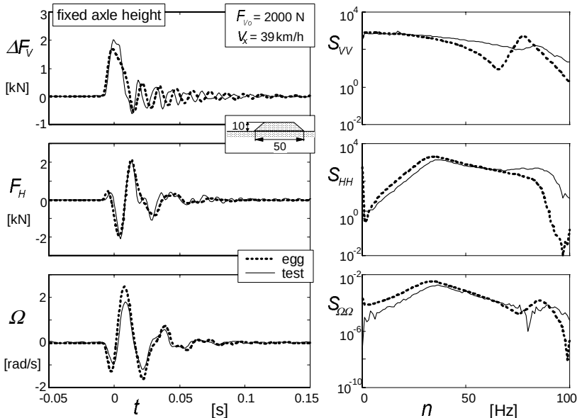
Fig. 9.64. Time traces and power spectra of vertical force, horizontal longitudinal force and angular velocity for wheel running at given speed of 39 km/h and initial vertical load of 2000N over trapezium cleat at constant axle height using SWIFT tyre parameters and obstacle parameters of Table 9.6. (Schmeitz).
