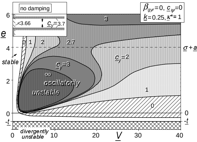
Fig. 6.6. Influence of lateral suspension compliance with non-dimensional stiffness c_y on stability. Gyroscopic couple and steer stiffness not regarded. Non-dimensional parameters: f=0 , \underline{m}=0.5 , \underline{t}=0.5 , \underline{\sigma}=3 .
