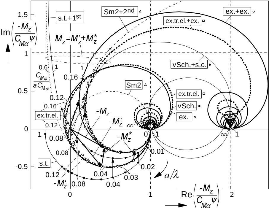
Fig.5.27. Nyquist plot of the non-dimensional frequency response function of the aligning moment M_z with respect to the wheel yaw angle \psi . Contributing components M'_z due to lateral deformations and M''_z due to tread width and associated longitudinal deformations. Parameters: \sigma = 3a and C_{M\phi} = aC_{M\alpha} Exact and approximate models: ex.: exact 'bare' string model; vSch.: Von Schlippe; Sm2: Smiley second order; s.t.: straight tangent; a0: point contact (hidden by Sm2); ex.tr.el.: exact w. tr.elmts. ex.: exact (brush); s.c.: straight connection (linear interpolation); 2nd: second-order approximation; 1st: first-order approx. (also C_{M\phi} = 0.6 aC_{M\alpha} ).
