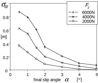
Fig. 7.8. Relaxation length measured at various wheel loads, decaying with increasing slip angle.
