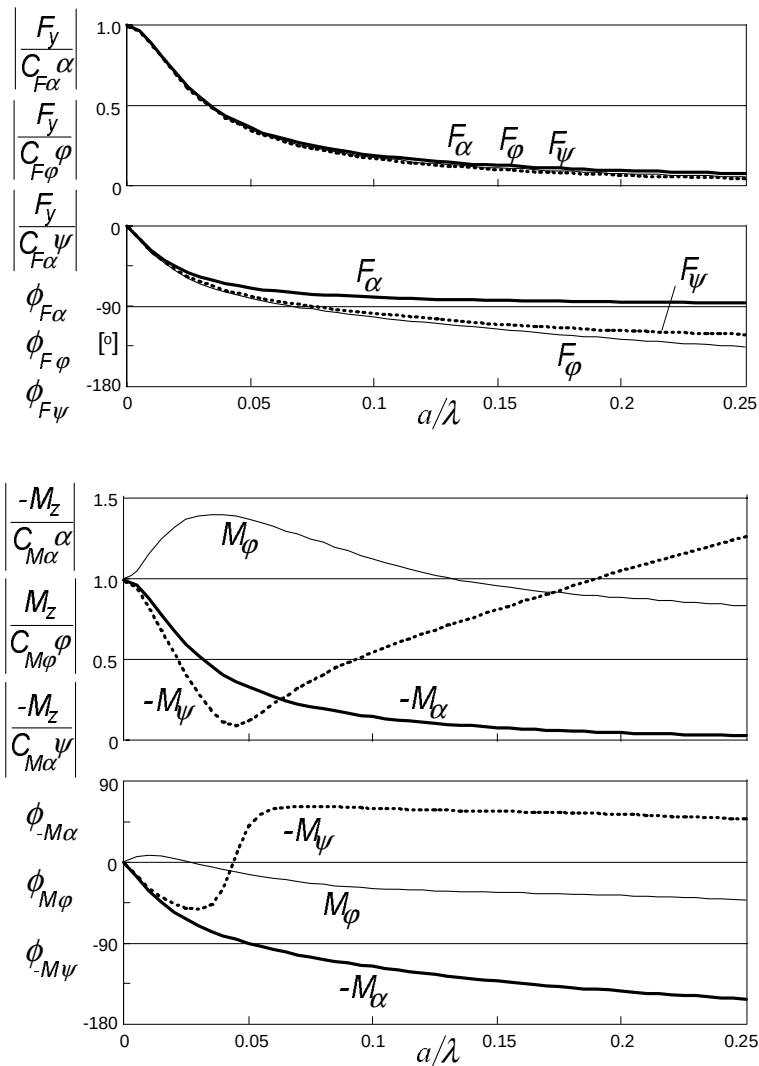
Fig. 9.16. Frequency response function of system with tread width. Curves for the force and moment responses to side slip \alpha , turn slip (path curvature) \phi and steer angle \psi have been indicated.
