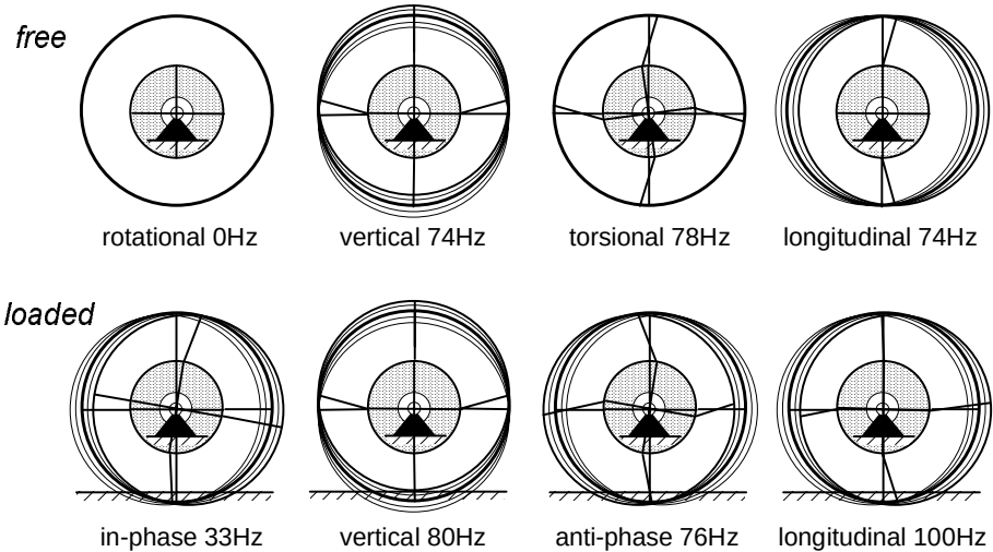
Fig. 9.39. Calculated in-plane vibrational modes of tyre/wheel system with axle fixed and tyre free or loaded on the drum surface with vertical load F_N = 4000\text{N} and at zero speed.
