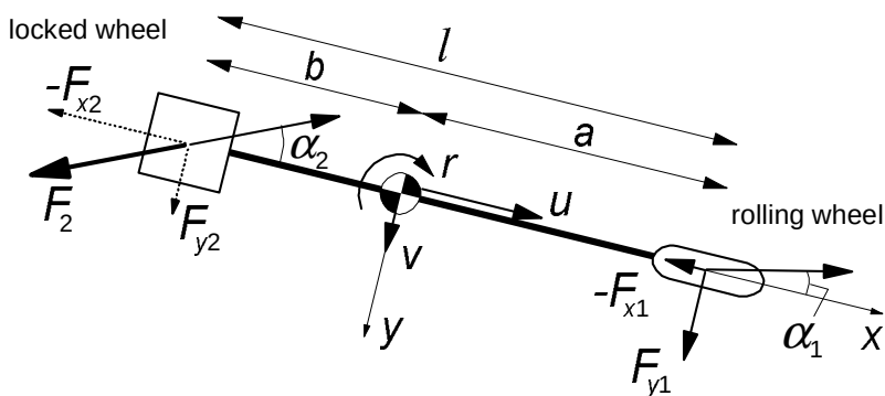
Fig.3.40. 'Bicycle' model with one wheel locked.
