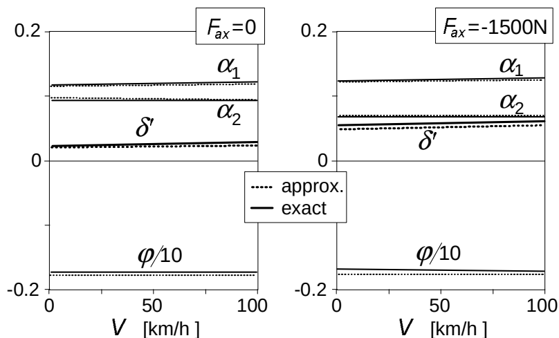
Fig. 10.18. Steer, roll and slip angles and the steer torque per m lateral c.g. offset y_{mr} that occur at straight line motion (according to the exact and approximate theories).
