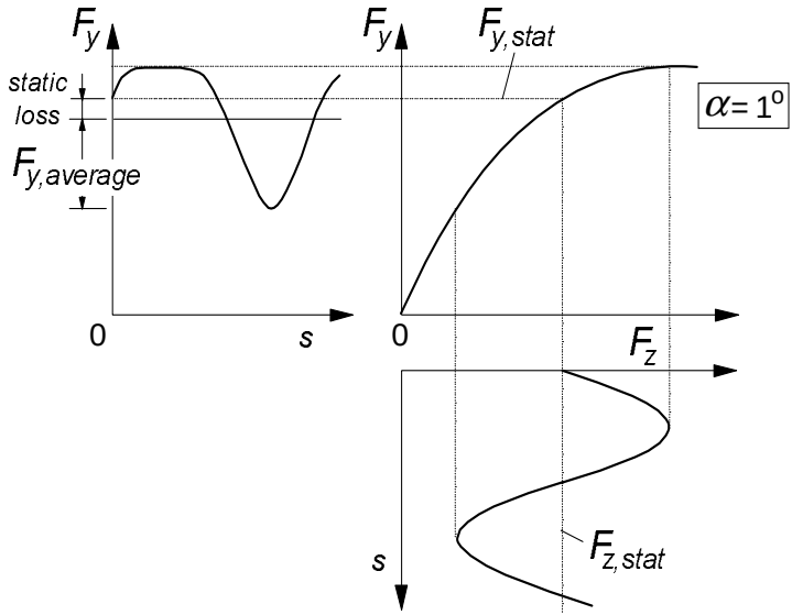
Fig. 8.4. The static loss in average side force due to the curved force vs load relationship.
