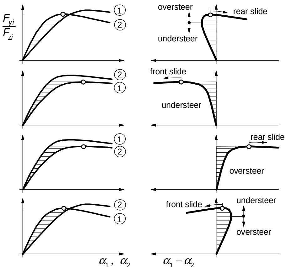
Fig. 1.18. A number of handling curves arising from the pairs of normalized tyre characteristics shown left. Only the main branch of handling curve is drawn (1: front, 2: rear).
