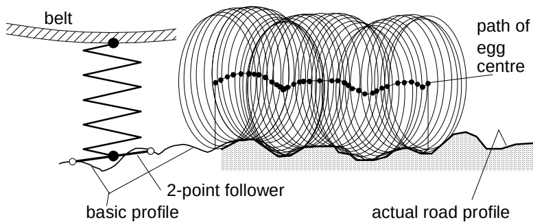
Fig. 9.57. The egg generating the basic road profile and three-point follower moving over it.
