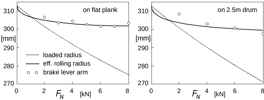
Fig. 9.34. Tyre radii as function of the normal load measured at zero or very low speed.
