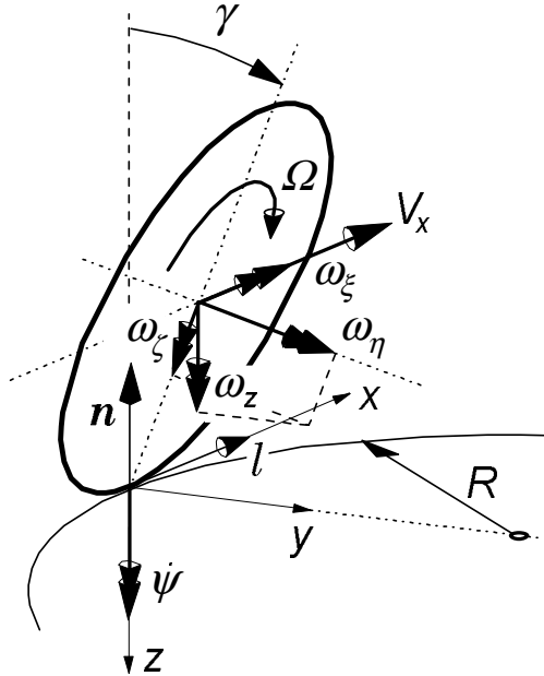
Fig. 2.6. Rotational slip resulting from path curvature and wheel camber (slip angle = 0).
