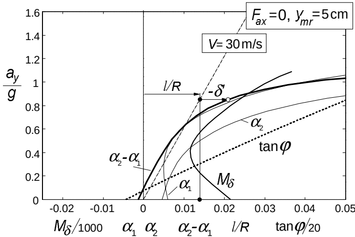
Fig. 10.28. The handling diagram at zero forward acceleration with 5cm lateral shift of the centre of gravity of combined rider and mainframe mass ( V = 108\text{ km/h} ).
