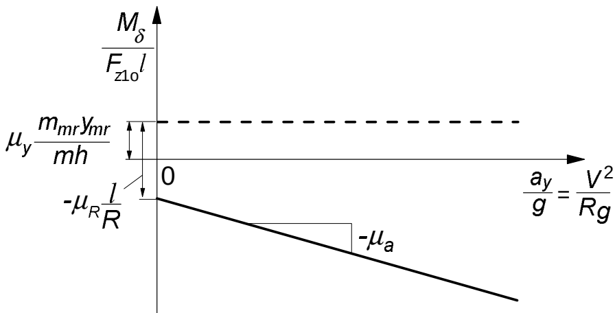
Fig. 10.19. The non-dimensional steer torque due to path curvature 1/R and c.g.lateral offset y_{mr} and the variation with lateral acceleration a_y or speed V .
