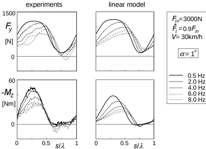
Fig. 8.6. Side force and aligning torque response to wheel load variation at a small slip angle.
