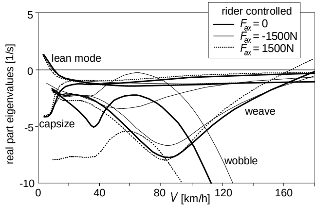
Fig. 10.13. The stability diagram with feed-back steer torque control of Fig.10.12 activated.
