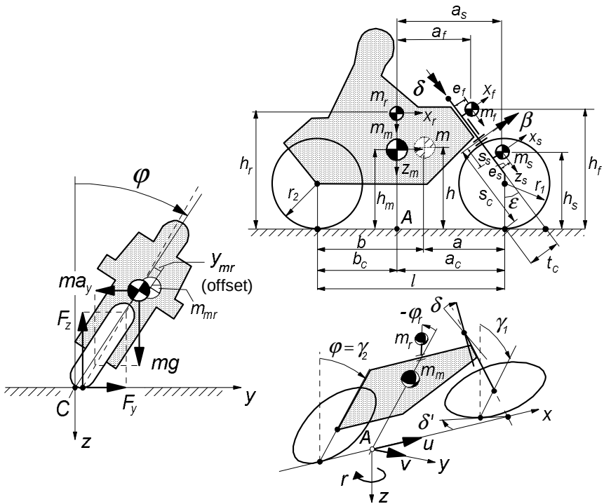
Fig. 10.1. Motorcycle model configuration.
