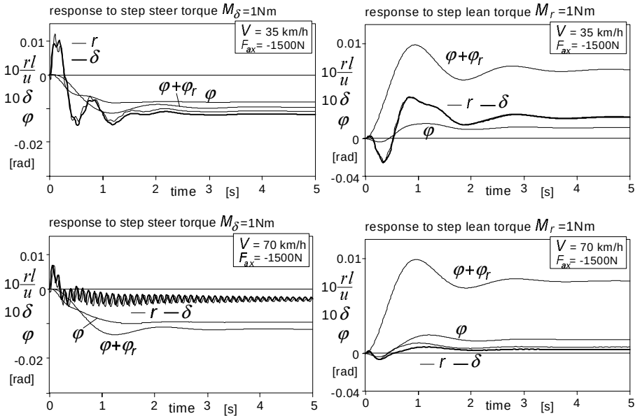
Fig. 10.15. The step responses of motion variables to unit steer and rider lean torque while braking, F_{ax} = -1500 \text{ N} (with rider stabilising control).
