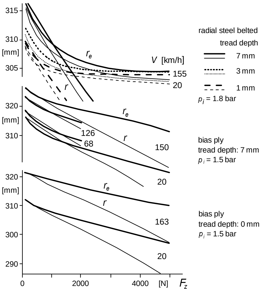
Fig. 8.12. Tyre effective rolling radius and loaded radius as a function of wheel load, measured on 2.5 m drum at different speeds and for different tread depths and tyre design. Note the different scales for the radial and bias-ply tyre radii.
