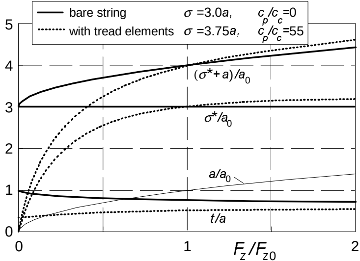
Fig.5.31. The variation of the relaxation length and half the contact length as a ratio to the static value of the latter and the ratio of the pneumatic trail to half the contact length with normalised vertical load both for the bare string model and for the model with tread elements.
