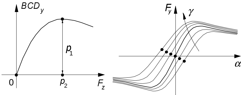
Fig. 4.12. Cornering stiffness versus vertical load and the influence of wheel camber, Eq. (4.56).
