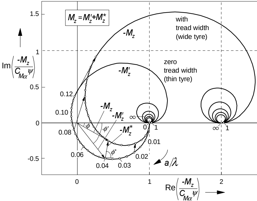
Fig 5.18. Nyquist plot of the non-dimensional frequency response function of the aligning moment M_z with respect to the wheel yaw angle \psi . The contributing components M_z' due to lateral deformations and M_z^* due to tread width and associated longitudinal deformations. Parameters: \sigma = 3a and C_{M\psi} = aC_{M\alpha}
