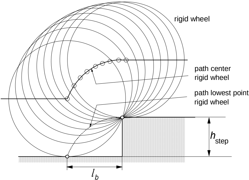
Fig. 9.53. The rigid wheel rolling over an upward step change in road level.
