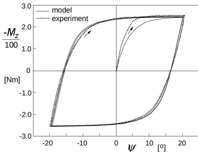
Fig. 9.22. Calculated and experimentally assessed variation of the moment versus steer angle for a non-rolling tyre pressed against a flat plate at a load F_z = 4800\text{N} .
