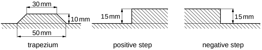
Fig. 9.46. Three typical obstacles used in Zegelaar's research.
