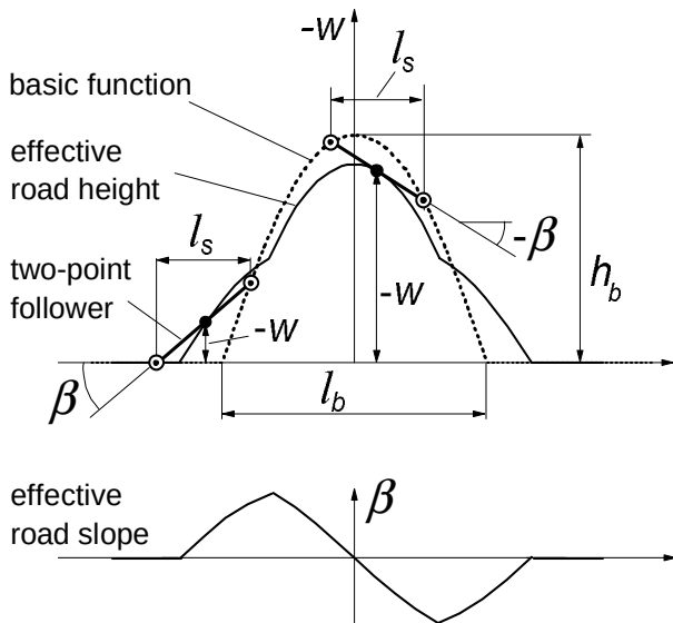
Fig. 9.51. Alternative method to determine the effective road height and slope using the basic curve with height h_b and the two-point follower with length equal to the shift l_s .
