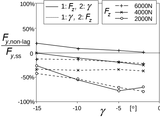
Fig. 7.13. Non-lagging part of side force response for the cases (1) applying camber after having loaded the tyre and (2) loading the tyre normal to the road after having cambered the wheel 'in the air'.
