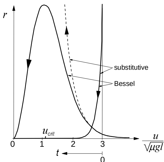
Fig. 3.43. Solutions of the exact and the approximated linear systems representing the variation of the yaw rate r with forward velocity u or with time t .
