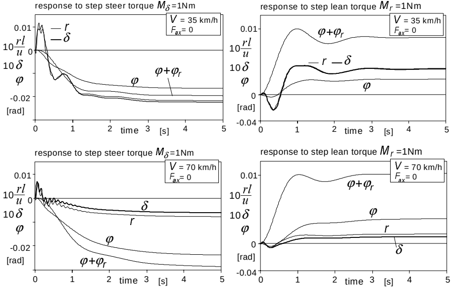
Fig. 10.14. The step responses of motion variables to unit steer and rider lean torque at zero forward acceleration, F_{ax} = 0 (with rider stabilising control).
