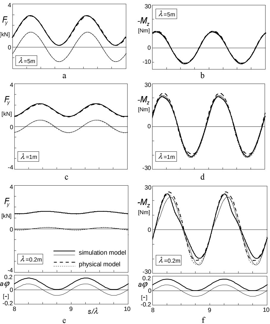
Fig.9.11. Side force and aligning torque responses of the non-linear brush simulation model with flexible carcass to sinusoidal path curvature variations (turn slip at \alpha = 0 ) of the wheel plane with an amplitude of a\varphi of 0.08 and average levels of 0 (thin curves) and 0.08 (fat curves), compared with results of the physical model (broken curves).
