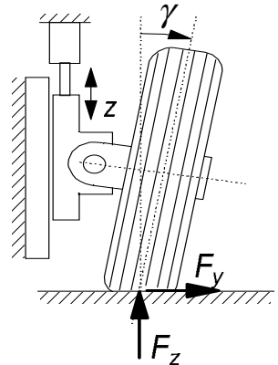
Fig. 7.14. Cambered wheel moved up and down (Exercise 7.1).
