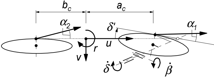
Fig. 10.4. Top view of the single track vehicle showing the front and rear slip angles.
