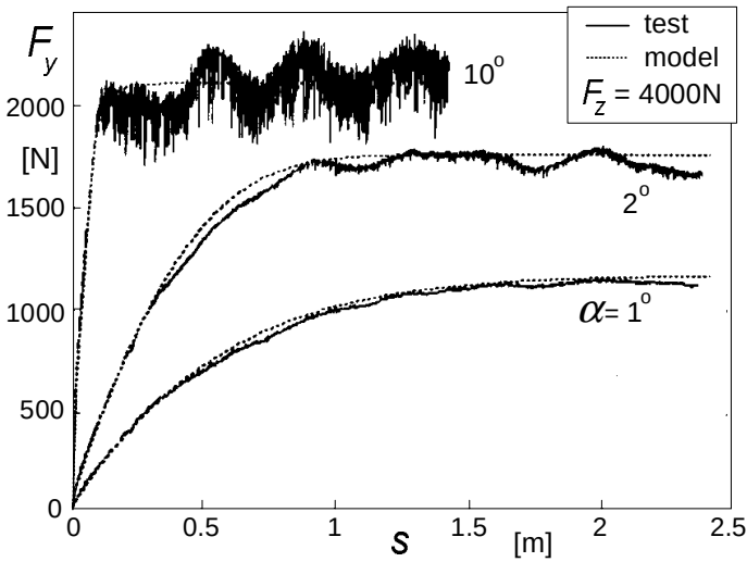
Fig. 7.5. Side force response to small and large step change in slip angle as assessed by flat plank experiments and computed with the model defined by Eqs.(7.32) or (7.29).
