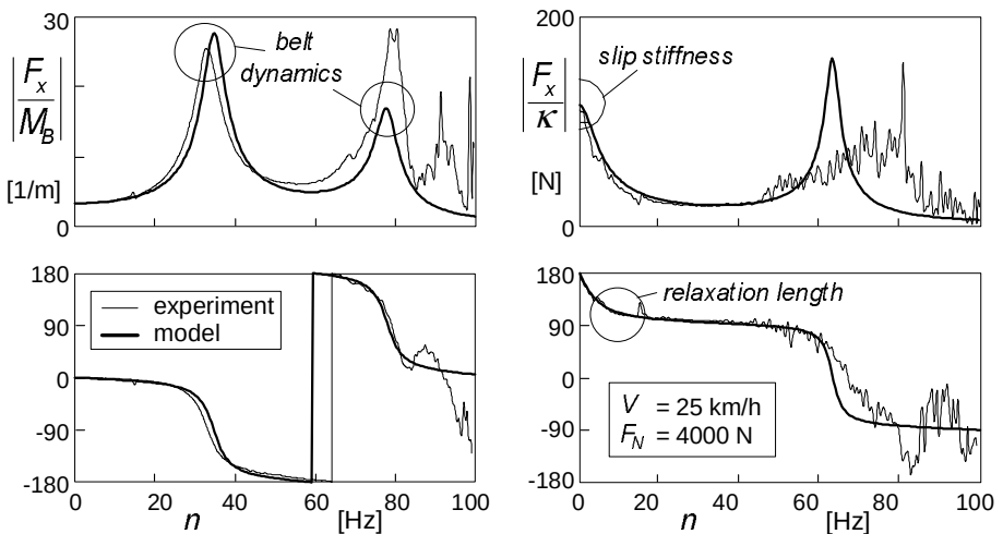
Fig. 9.41. Measured and calculated in-plane frequency response functions at an average braking force of 450 N and assessed at a braking force standard deviation of 75 N.
