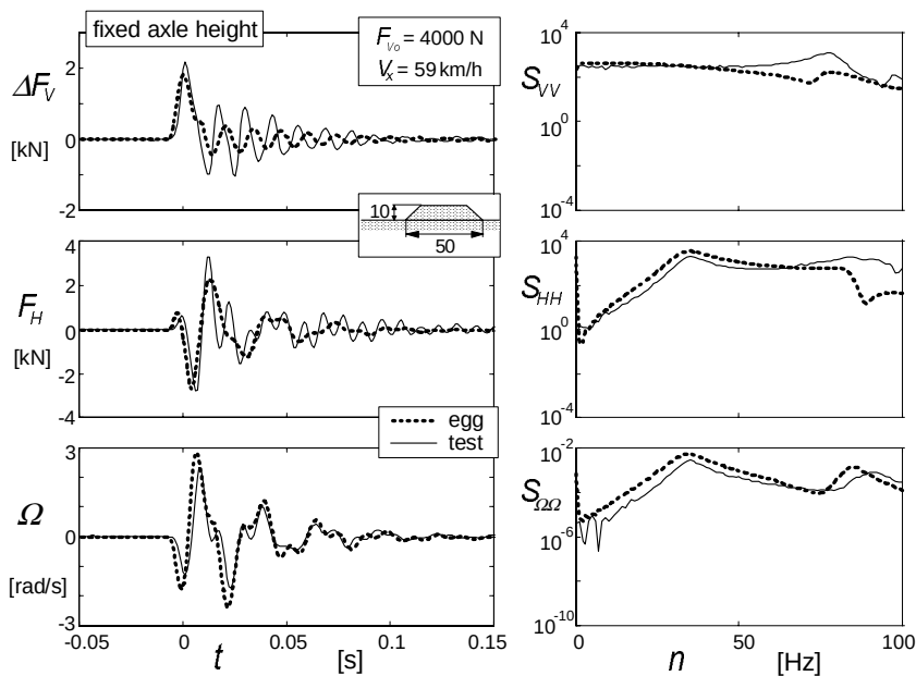
Fig. 9.67. Same as Fig.9.66 but at different speed.
