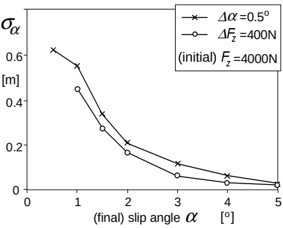
Fig. 7.10. Relaxation lengths resulting from small step changes in slip angle or wheel load, as function of slip angle level, Higuchi (1997).
