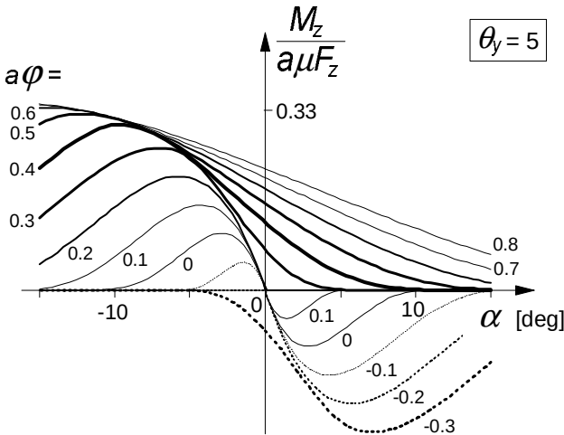
Fig. 3.32. Aligning torque characteristics of the single row brush model up to large levels of spin. (Compare with Fig.3.28 where spin is small and a\phi = 0.33 \sin\gamma ).
