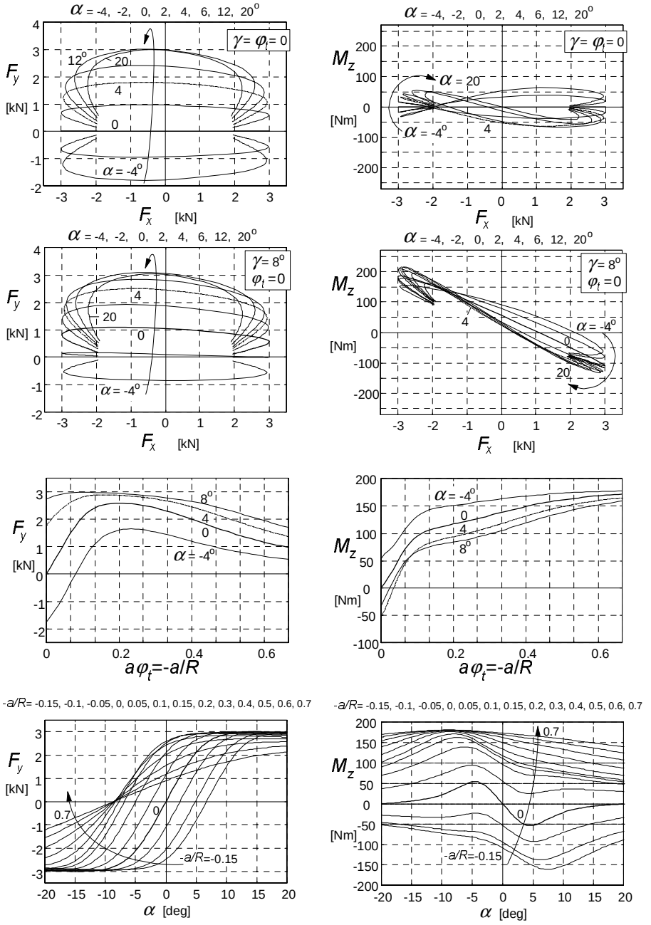
Fig. 4.19. Magic Formula results for steady-state response of forces F_{x,y} and moment M_z to slip angle \alpha , slip ratio \kappa , camber angle \gamma and path curvature \phi_l = -1/R .
