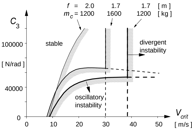
Fig. 1.30. Stability boundaries for the car caravan combination in the caravan cornering stiffness versus critical speed diagram. Vehicle parameters according to Table 1.1, in addition: h = 2\text{m} , g = 2\text{m} , k_c = 1.5\text{m} ( I_c = m_c k_c^2 ), cf. Fig. 1.29.
