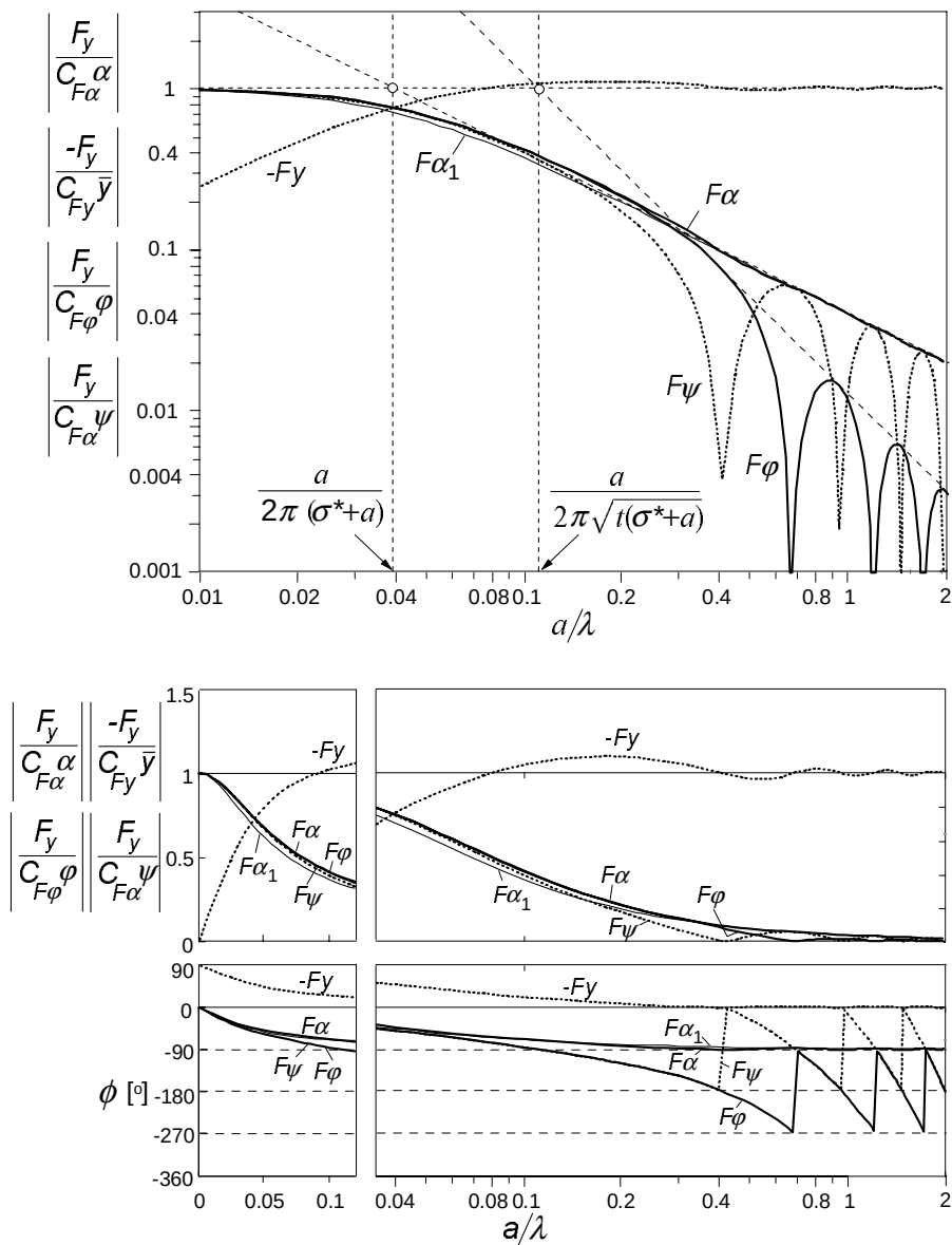
Fig. 5.33. Frequency response functions of the string model with tread elements for the side force with respect to various motion input variables. For the response to \alpha a first-order approximation with the same cut-off frequency, \omega_s=1/(\sigma^*+a) , has been added ( F\alpha_1 ). Three ways of presentation have been used: log-log, lin-log and lin-lin. The model parameters are: \sigma = 3.75a , c_p/c_c=55 which leads to \sigma^*=3a , t=0.49a .
