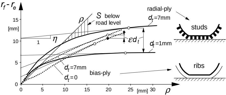
Fig. 8.13. Reduction of effective rolling radius r_e with respect to tyre free radius r_f due to tyre radial deflection \rho and tread depth change d_t . Situation at nominal load, F_{zo} = 3000\text{N} , has been indicated by circles.
