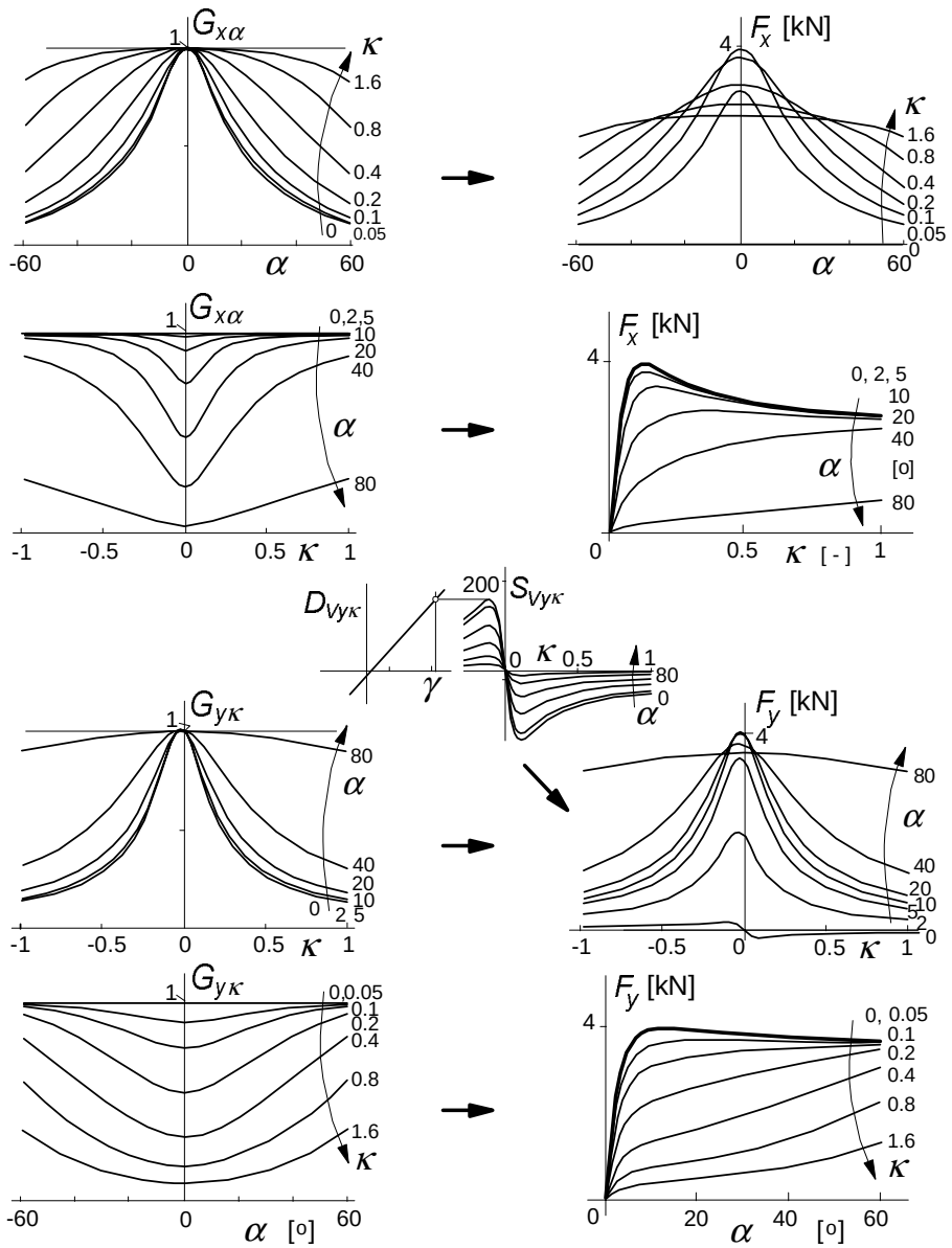
Fig. 4.15. Nature of weighing functions and the resulting combined slip longitudinal and lateral forces, the latter also affected by the \kappa induced ply-steer 'vertical shift' S_{vy\kappa} .
