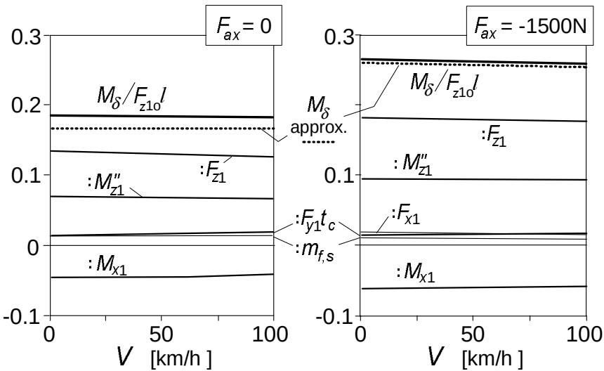
Fig. 10.21. The non-dimensional steer torque ( M_\delta/(F_{z10}l) ) and its components (cf. Eq.(10.147)) per m.c.g. lateral offset y_{mv} . In M''_{z1} the F_{x1} contribution is removed.
