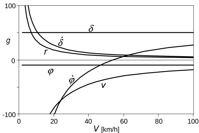
Fig. 10.12. Hypothetical rider steer torque feed-back stabilising control gains versus speed.
