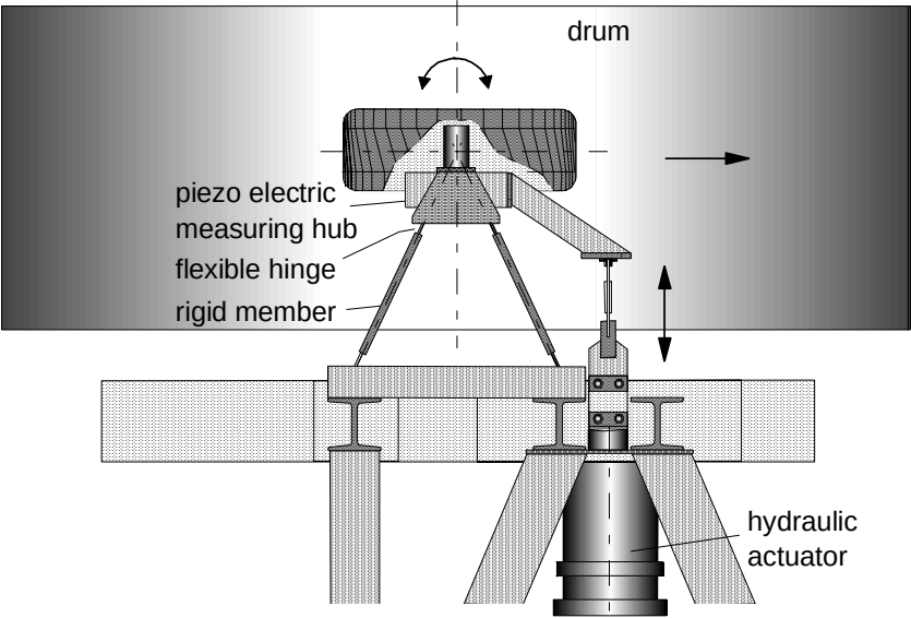
Fig. 9.39. The yaw oscillation test rig featuring centre point steering. Frequencies up to ca. 65 Hz enabling the assessment of tyre out-of-plane inertia and stiffness parameters including residual stiffnesses and rigid modes.
