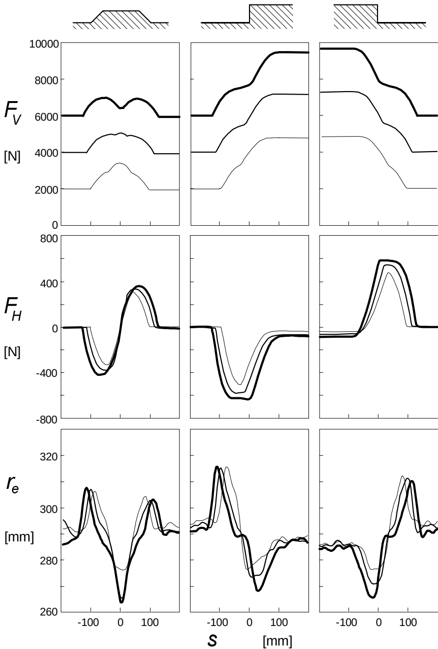
Fig. 9.47. Rolling over a trapezium cleat, an upward and a downward step (Fig.9.46) at very low speed and for three axle heights. Diagrams show measured variations of the vertical force F_V (upward +), the longitudinal horizontal force F_H (forward +) and the effective rolling radius r_e , Eq.(9.238). Tyre dimensions: 205/60R15).
