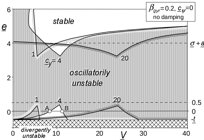
Fig. 6.8. Influence of lateral (camber) suspension compliance with gyroscopic coupling. Steer stiffness is equal to zero. Steer and tread damping equal to zero. Eigenvalues and eigenvectors of points A and B are analysed in Figs.6.22,23.
