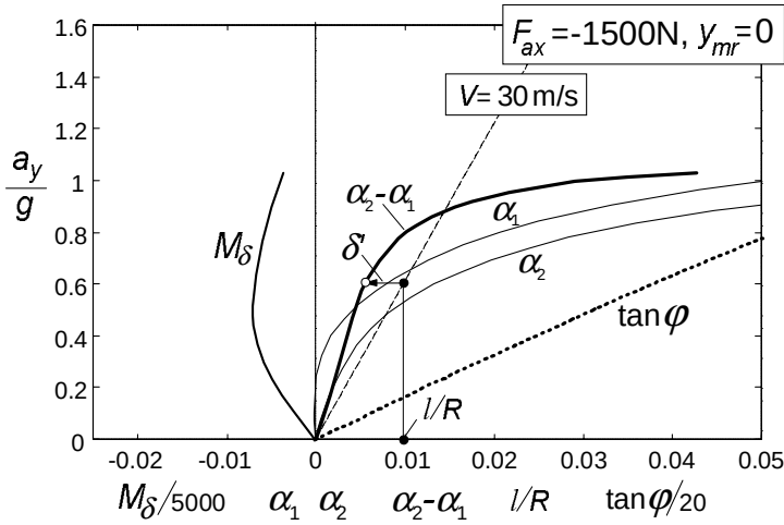
Fig. 10.26. The handling diagram at braking ( V = 108 \text{ km/h} ).
