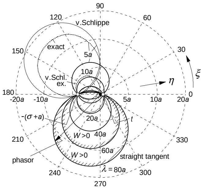
Fig. 6.20. Mode shape plot (amplitude ratio \eta , phase \zeta ) with Besselink's zero energy circles for different wavelengths and tyre model approximations, indicating mode shapes for which shimmy begins to show up (instability occurs if at a particular value of the motion wavelength \lambda the phasor end point gets inside the corresponding circle). At smaller wavelengths the circle belonging to the straight tangent approximation begins to appreciably deviate from the exact or Von Schlippe representation.
