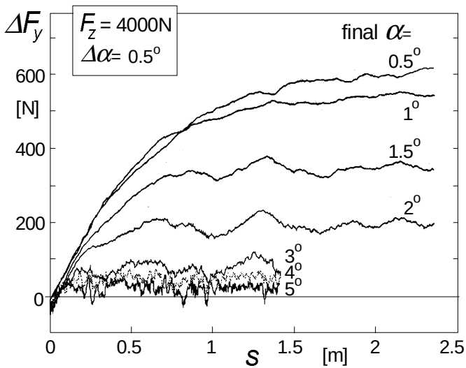
Fig. 7.6. Side force response to small increment of slip angle \Delta\alpha at different levels of slip angle indicating the decrease of relaxation length at increasing slide slip level which is in agreement with expression (7.36).
