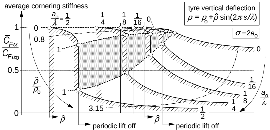
Fig. 5.50. Computed variation of average cornering stiffness with amplitude of the vertical tyre deflection, \rho , and path frequency, 1/\lambda , for the bare string model.
