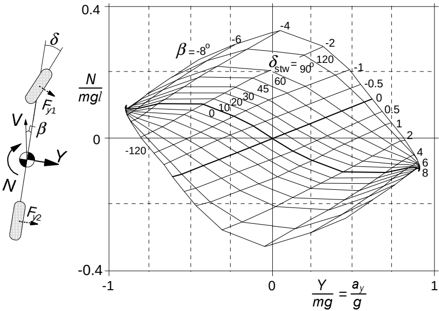
Fig. 1.27. The MM diagram portraying the car's potential manoeuvring capacity.
