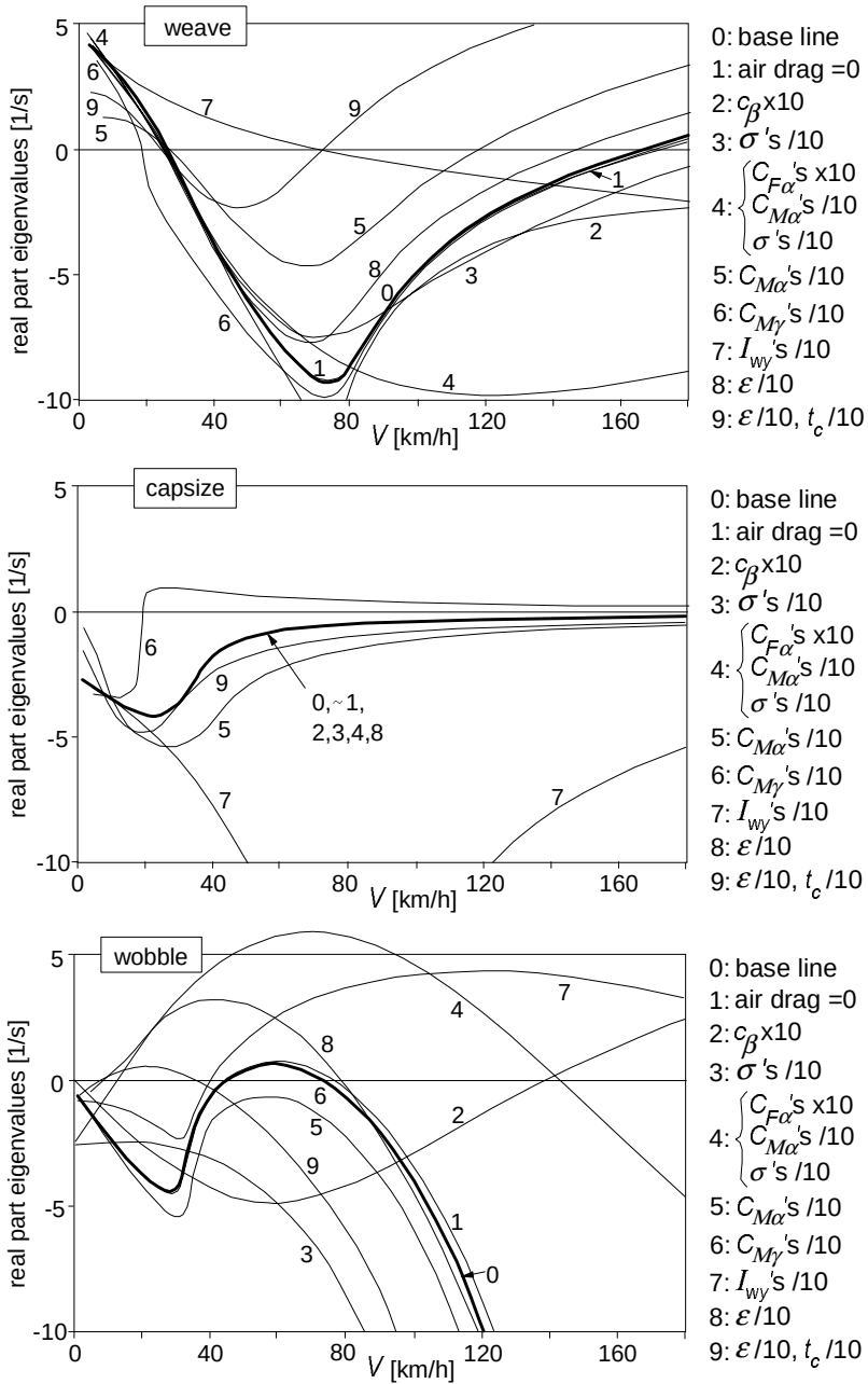
Fig. 10.8. Effect of drastic changes in model parameter values on stability characteristics.
