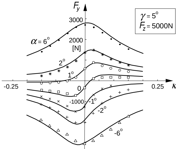
Fig. 4.16. The combined slip side force characteristics in the presence of a camber angle, Bayle et al. (1993).
