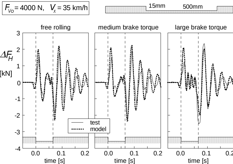
Fig. 9.70. The horizontal force variation when traversing a pot hole while the wheel is being braked at three different levels of brake torque ( M_B = \text{ca. } 4, 375, 850\text{Nm} respectively, Zegelaar, 1998). Experiments on 2.5m drum, calculations using obstacle parameters according to Fig.9.54.
