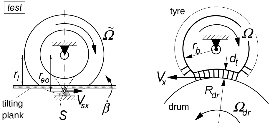
Fig. 9.61. Two components of rolling over a curved obstacle.
