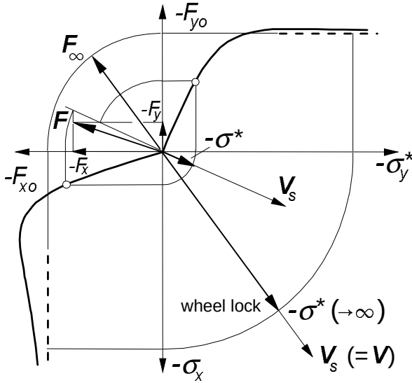
Fig.. 4.6. Construction of the resulting combined slip force from the pure slip characteristics according to Eqs.(4.31).
