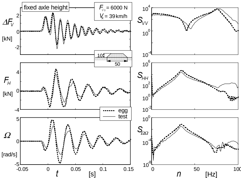
Fig. 9.68. Same as Fig.9.66 but at different initial vertical load .
