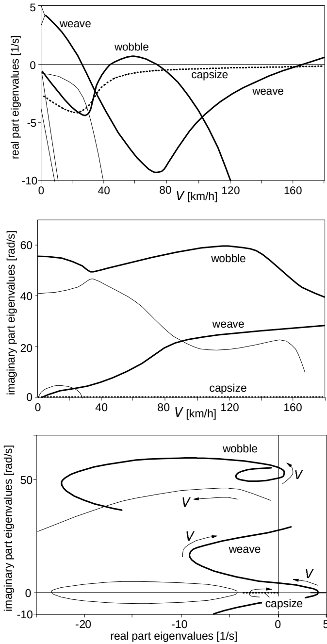
Fig. 10.7. Baseline configuration (rigid rider, with air drag, zero forward acceleration, no control). Real and imaginary parts of eigenvalues versus speed of travel V .
