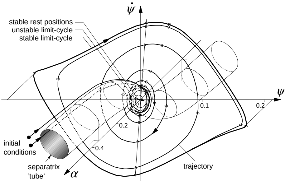
Fig. 6.27. Solutions in the three-dimensional state space. System with non-linear tyre and dry friction ( V = 6.66 , \sigma = 3 , \varrho = 0 , k'' = k = \delta = 0 , K = 0.0035 ). Line piece for possible rest positions, unstable and stable limit-cycle. Tube shaped separatrix separating space of trajectories leading to a rest position from the space of solution curves leading to the stable limit-cycle.
