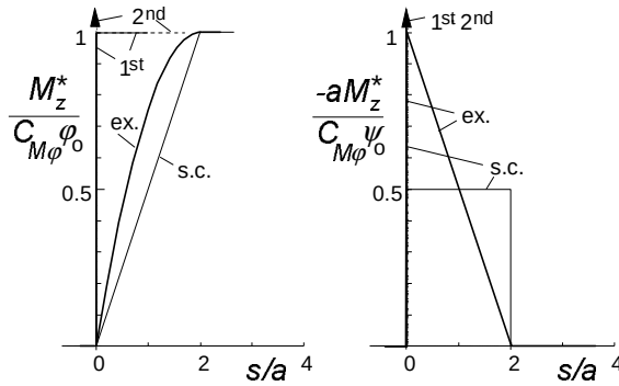
Fig. 5.22. Step response of the moment due to tread width to turn slip (path curvature) and yaw angle for exact and approximations: ex.: exact (brush model); s.c.: straight connection (linear interpolation); 2nd : second-order approximation; 1st : first-order approximation.
