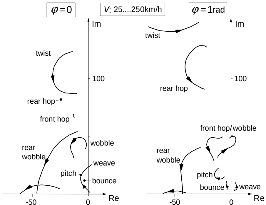
Fig. 10.29. Eigenvalues of Koenen's motorcycle model at straight ahead running ( \varphi = 0 ) and at a roll angle of one radian. The speed varies from 25 to 250 km/h.
