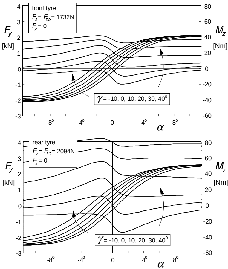
Fig. 10.5. Side force and aligning torque characteristics for the freely rolling front and rear motorcycle tyre model at a series of camber angles.
