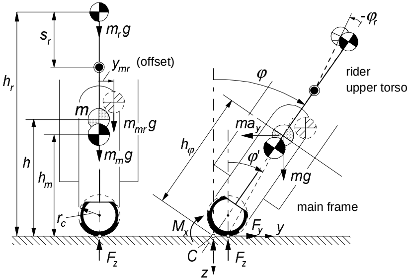
Fig 10.2. Rear view of motorcycle with tyre cross section and possible c.g. offset indicated.
