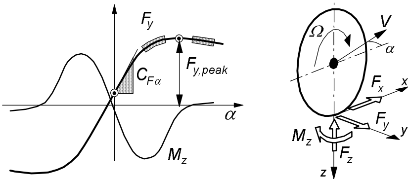
Fig. 1.1 Characteristic shape factors (indicated by points and shaded areas) of tyre or axle characteristics that may influence vehicle handling and stability properties. Slip angle and force and moment positive directions, cf. App.1.
