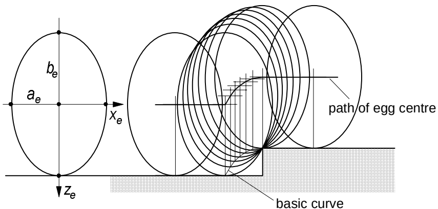
Fig. 9.55. 'Egg' moving over step road profile, producing basic curve.
