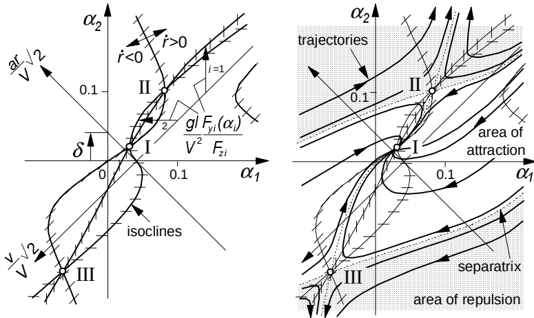
Fig. 1.22. Isoclines for the construction of trajectories in the phase-plane. Also shown: the three singular points I, II and III (cf. Fig. 1.17) and the separatrices constituting the boundary of the domain of attraction. Point I represents the stable cornering motion at steer angle \delta .
