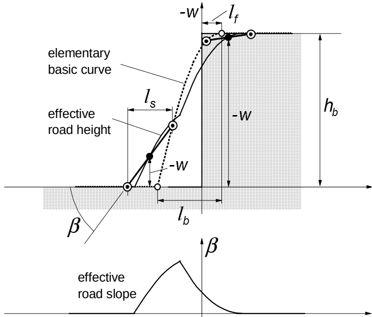
Fig. 9.52. The effective road response curves resulting from the (elementary) basic curve associated with the step change in road level by using the two-point follower concept.
