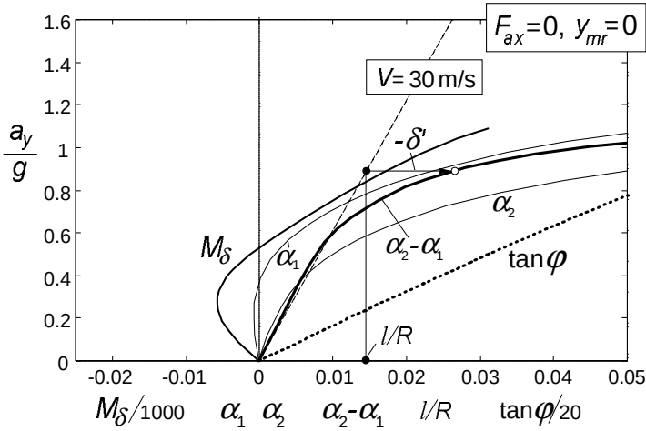
Fig. 10.25. The handling diagram with air drag considered and zero forward acceleration, ( V = 108 \text{ km/h} ).
