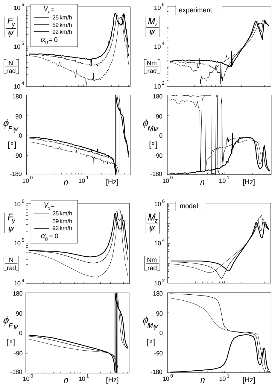
Fig. 9.42. Measured and calculated out-of-plane frequency response functions of the side force and aligning torque to steer angle variations at zero average slip angle for three values of forward speed and normal load F_N = 4000\text{N} .
