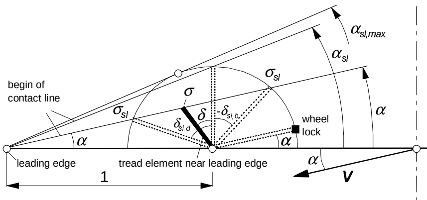
Fig.3.14. The situation near the leading edge. Various deflections of an element at a distance equal to 1 from the leading edge are shown corresponding with points in the upper diagram of Fig 3.13.
