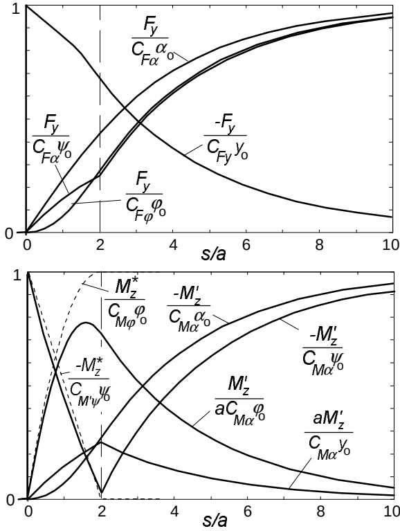
Fig. 5.10. Step response of side force F_y , aligning torque M'_z and tread width moment M_z^* to side slip \alpha , lateral displacement \dot{y} , turn slip \phi and yaw angle \psi . Computed for string model with deflection relaxation length \sigma = 3a .
