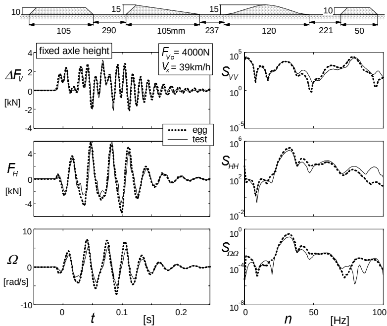
Fig. 9.69. Running over a series of cleats mounted on the drum surface, at constant axle height.
