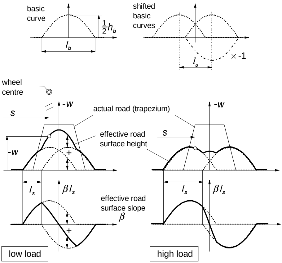
Fig. 9.49. The construction of the curves representing the effective height end effective slope of the local road plane from the basic function associated with the trapezium cleat.
