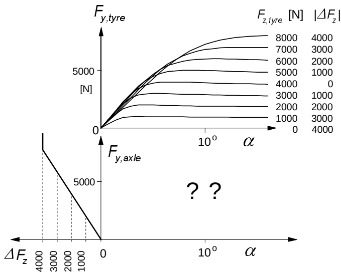
Fig. 1.8. The construction of the resulting axle cornering characteristics at load transfer (Exercise 1.1).
