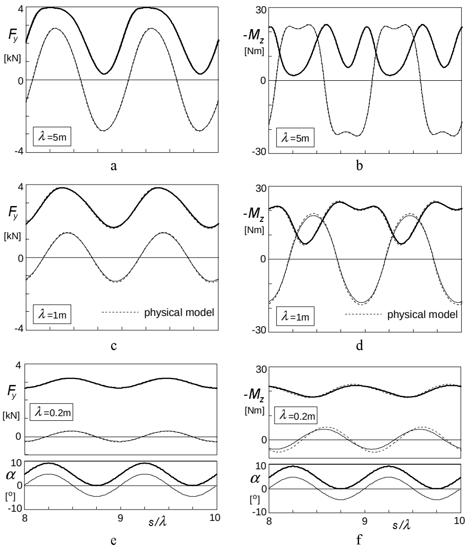
Fig.9.10. Side force and aligning torque responses of the non-linear brush simulation model with flexible carcass to sinusoidal slip angle input of the wheel plane with a slip angle amplitude of 0.08rad and average levels of 0 (thin curves) and 0.08rad (fat curves), compared with results of the physical model (broken curves).
