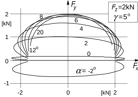
Fig. 4.7a. Cornering force versus longitudinal force at a new load and camber angle as computed with the similarity method.
