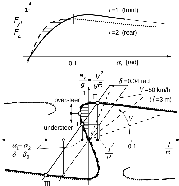
Fig. 1.17. Handling diagram resulting from normalized tyre characteristics. Equilibrium points I, II and III (steady turns) of which only I is stable, arise for speed V=50 \text{ km/h} and steer angle \delta = 0.04 \text{ rad} . From the different line types the manner in which the curves are obtained from the upper diagram may be retrieved.
