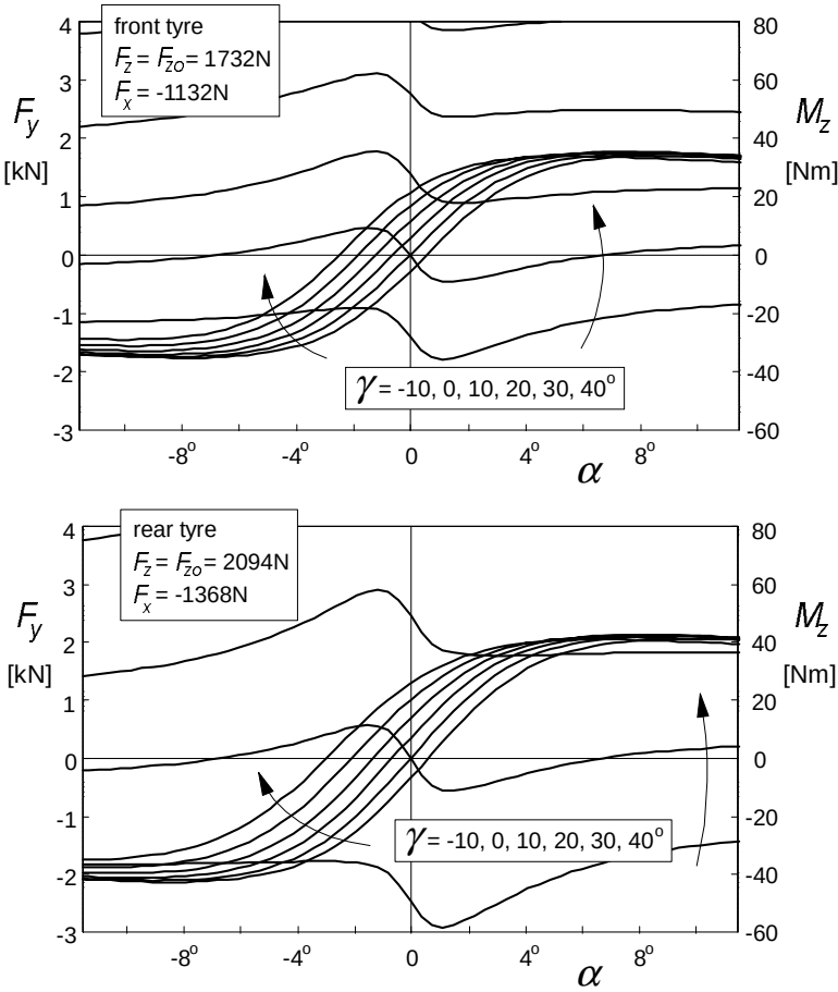
Fig. 10.6. Side force and aligning torque characteristics for the braked front and rear motorcycle tyre at a series of camber angles.
