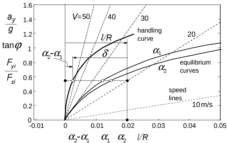
Fig. 10.23. The handling diagram for the simplified case where tyre moments and gyroscopic couples are deleted and air drag is disregarded. The normalised side force versus slip angle curves (in this simplified case equal to the equilibrium curves) have been depicted as well.
