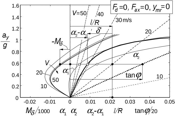
Fig. 10.24. Handling diagram for complex model with all tyre moments and gyroscopic couples included. Air drag = 0 which makes the diagram valid for all speeds V . Curves for roll angle, front and rear slip angles and steer torque (different for each speed).
