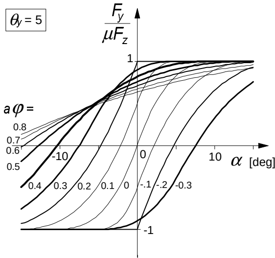
Fig. 3.31. Side force characteristics of the single row brush model up to large levels of spin. (Compare with Fig.3.28 where spin is small and a\phi = 0.33 \sin\gamma ).
