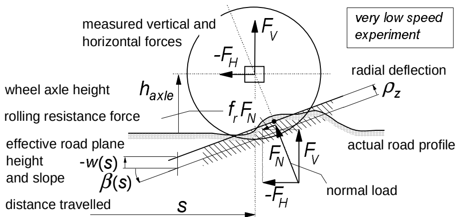
Fig. 9.48. The wheel rolled over a road irregularity at constant axle height to establish the effective road plane variation.
