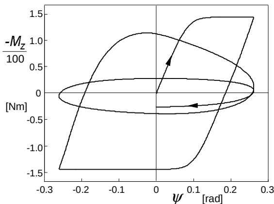
Fig. 9.24. The steer torque plotted versus steer angle during the manoeuvre of Fig 9.23.
