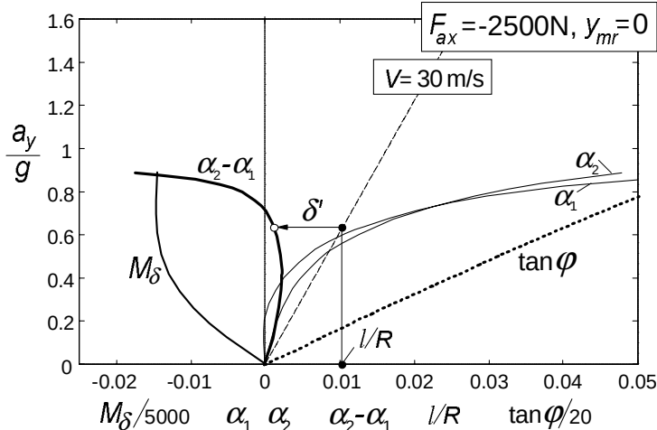
Fig. 10.27. The handling diagram at hard braking ( V = 108\text{ km/h} ).
