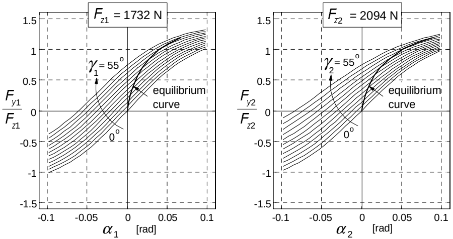
Fig. 10.22. Tyre side force diagrams at a series of camber angles \gamma . Simplified situation where wheel loads remain unchanged (no air drag) and tyre moments and gyroscopic couples are left out of consideration. Equilibrium curves have been shown where the tyre side force agrees with the roll angle ( \approx \gamma_{1,2} ).
