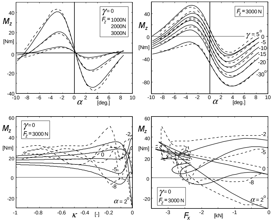
Fig. 10.32. Aligning torque characteristics of a 160/70 ZR17 motorcycle tyre. Modified Magic Formula computed results compared with data from measurements conducted with the Delft Tyre Test Trailer.
