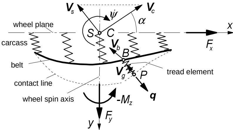
Fig. 3.33. Enhanced model with deflected carcass and tread element that is followed from front to rear.
