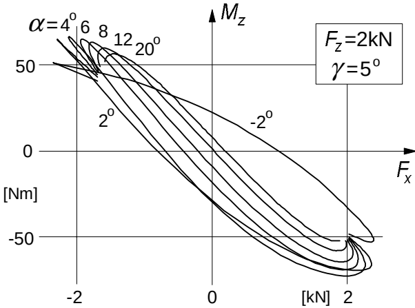
Fig. 4.7b. Aligning torque versus longitudinal force at a new load and camber angle as computed with the similarity method.
