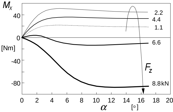
Fig. 4.26. Overturning couple calculated with formulae (4.122-124), cf. Fig.4.30 for similar measured characteristics.
