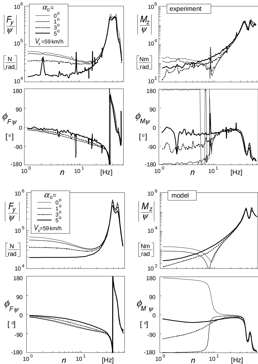
Fig. 9.43. Measured and calculated out-of-plane frequency response functions of the side force and aligning torque to steer angle variations at one value of speed and at four levels of average side slip and wheel load F_N = 4000 N.
