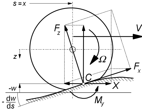
Fig. 8.15. In-plane excitation by road unevenness and by vertical and fore and aft axle motions.
