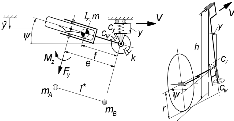
Fig. 6.5. Lateral compliance introduced in the system.
