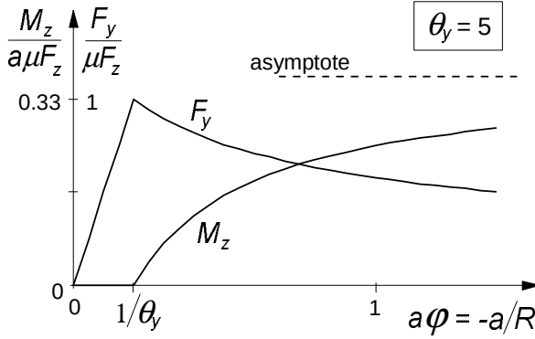
Fig. 3.25. Force and moment versus non-dimensional spin for single row brush model.
