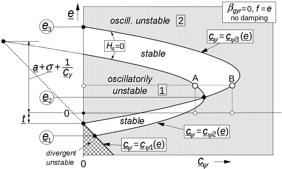
Fig. 6.17. Basic stability diagram for the case f=e (c.g. distance e behind steer axis). Steer and tread damping are equal to zero. Gyroscopic coupling is disregarded. The functions c_{\psi i}(e) are defined by Eqs. (6.55, 58, 59). Eigenvalues and eigenvectors of points A and B are analysed in Fig. 6.18, 19. (From: Besselink 2000).
