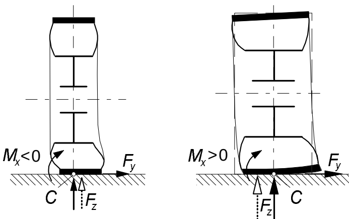
Fig. 4.25. Narrow and wide tyre subjected to side slip giving rise to an overturning couple that may be of a different sign.
