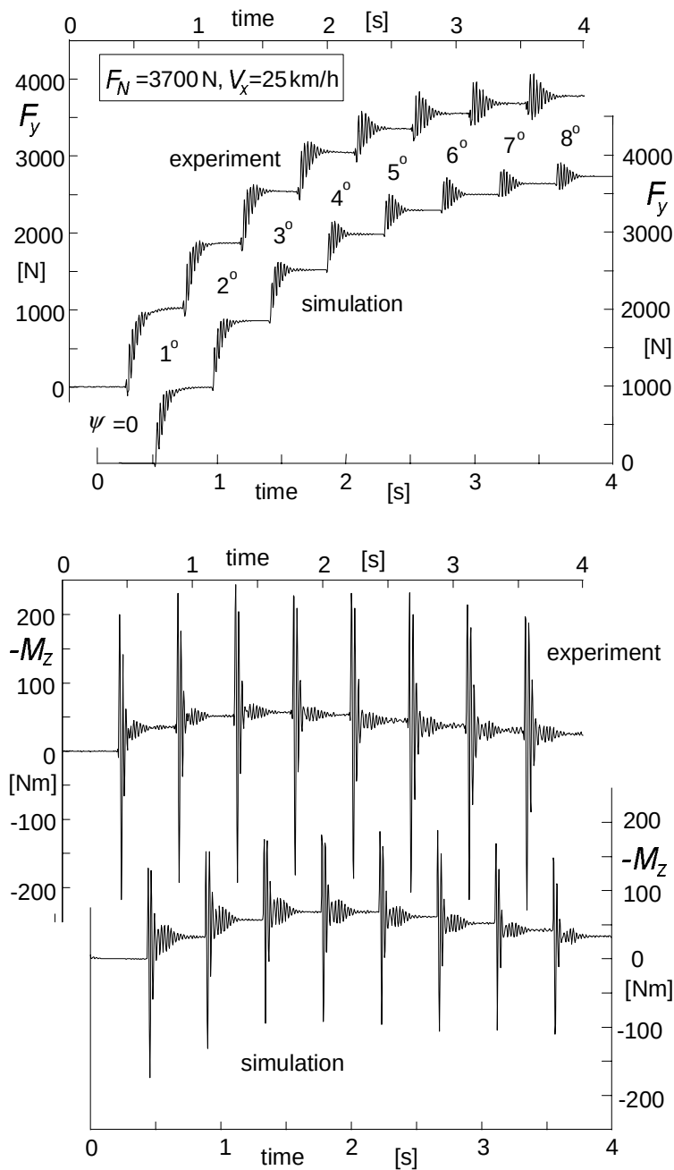
Fig. 9.45. Side force and aligning torque response to successive step changes in steer angle. (Maurice, 2000)
