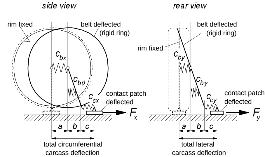
Fig. A3.2. Longitudinal and lateral deflections of the rigid ring and contact patch.
