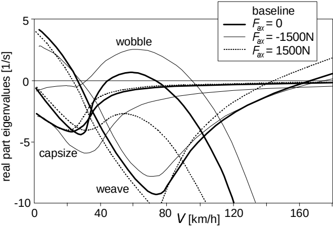
Fig. 10.10. Effect of the application of braking ( F_{ax}, F_{x1,2} < 0 ) and driving forces ( F_{ax}, F_{x2} > 0 ) on the stability diagram (baseline configuration).
