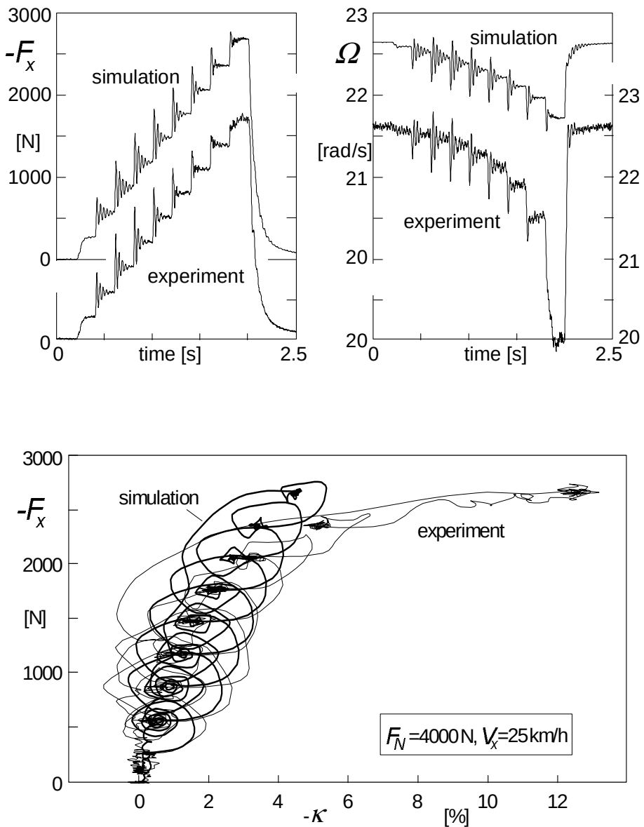
Fig. 9.44. Brake force response to successive step increments of brake pressure. The upper diagrams depict the variation of force and wheel speed of revolution with time. The lower figure shows the loops in the force versus wheel slip diagram. Apparently, the actual friction coefficient is lower than assumed in the model. (Zegelaar, 1998).
