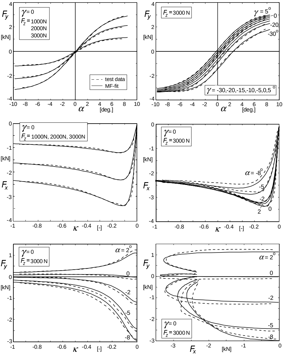
Fig. 10.31. Force characteristics of a 160/70 ZR17 motorcycle tyre. Modified Magic Formula computed results compared with data from measurements conducted with the Delft Tyre Test Trailer.
