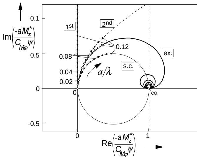
Fig. 5.26. Nyquist plot of the frequency response function of the torque due to tread width -M_z^* with respect to the wheel yaw angle \psi . ex.: exact (brush); s.c.: straight connection (linear interpolation); 2nd: second-order app.; 1st: first-order approx.
