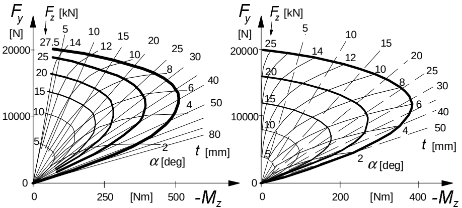
Fig. 3.6. Left: Gough plot of truck tyre 9.00-20, measured on a dry road surface (Freudenstein, 1961). Right: brush model with tread element stiffness c_p decaying linearly with F_z .
