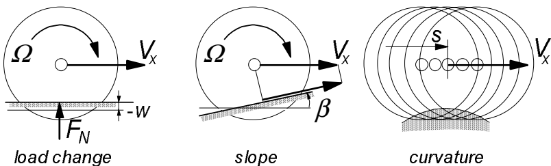
Fig. 9.58. Three contributions to the change in effective rolling radius.
