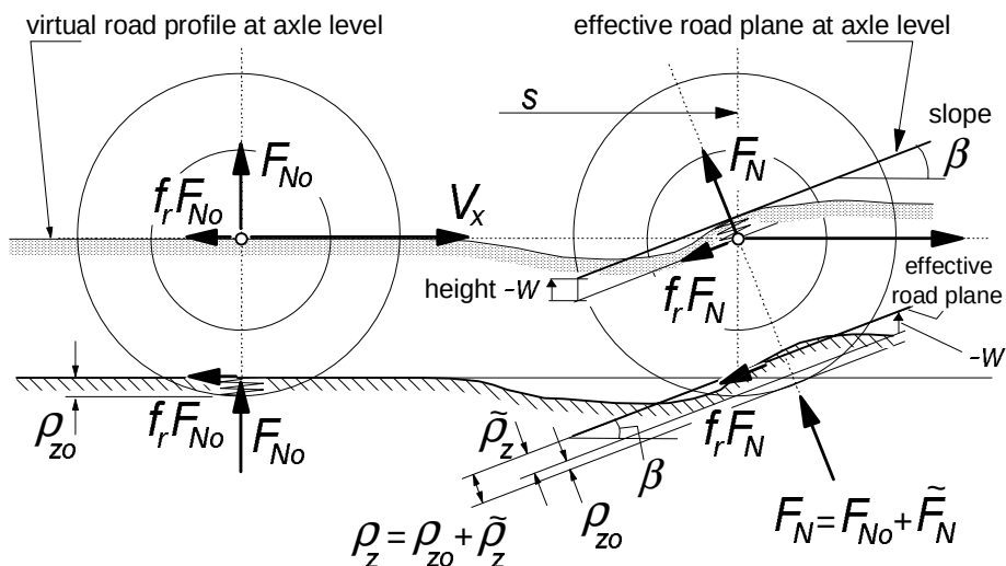
Fig. 9.50. The virtual road profile and effective road plane as sensed at wheel axle level.
