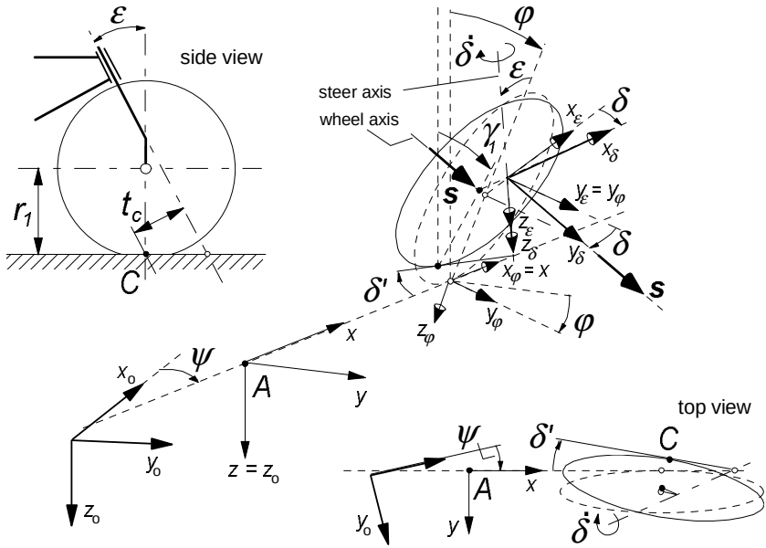
Fig. 10.3. View of front wheel assembly with various coordinate system triads to assess the ground steer angle \delta' and camber angle \gamma_1 of the front wheel using the unit vector s along the wheel spin axis ( \beta = 0 ).
