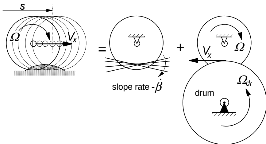
Fig. 9.60. Unravelling the process of rolling over a curved obstacle.
