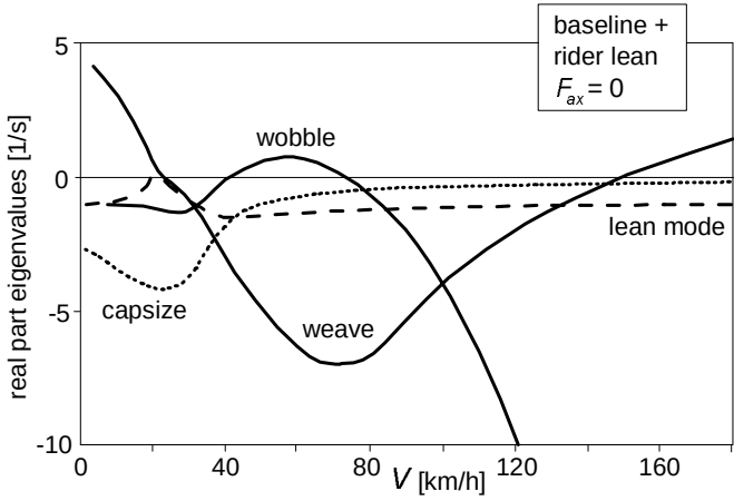
Fig. 10.11. The stability diagram with the rider lean degree of freedom introduced.
