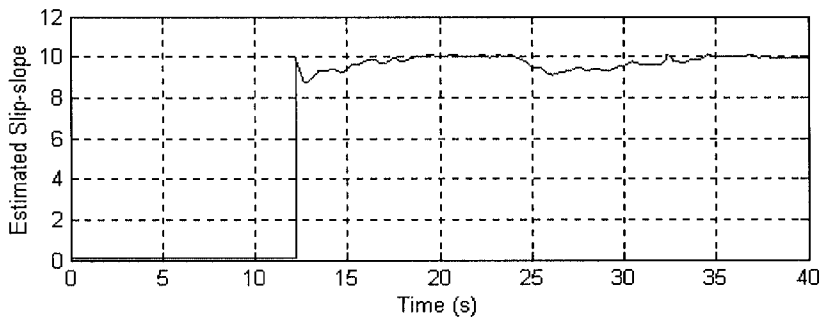
Figure 14-8. Slip-slope estimation during acceleration and braking
