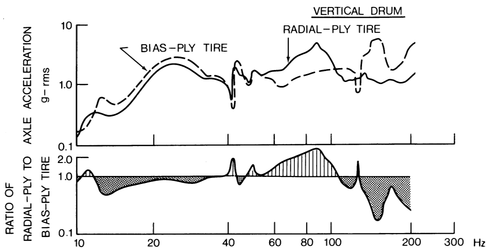
Fig. 1.66 Vibration characteristics of a bias-ply and a radial-ply car tire subject to sinusoidal excitation. (Reproduced with permission of the Council of the Institution of Mechanical Engineers from reference 1.38.)
