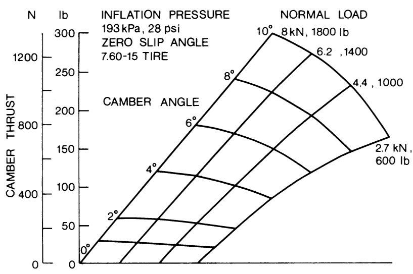
Fig. 1.34 Variation of camber thrust with camber angle and normal load for a car tire. (Reproduced with permission of the Society of Automotive Engineers from reference 1.21.)
