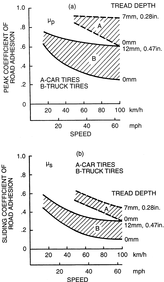
Fig. 1.52 Comparison of (a) the peak value of road adhesion coefficient \mu_p and (b) the sliding value of road adhesion coefficient \mu_s of car and truck tires on wet surfaces. (Reproduced with permission from reference 1.8.)
