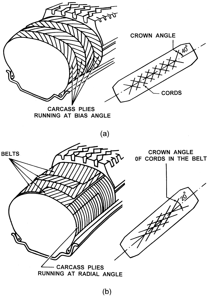
Fig. 1.1 Tire construction. (a) Bias-ply tire. (b) Radial-ply tire.
