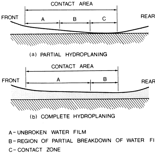
Fig. 1.49 Hydroplaning of a tire on flooded surfaces. (Reproduced with permission from Mechanics of Pneumatic Tires , edited by S.K. Clark, Monograph 122, National Bureau of Standards, 1971.)
