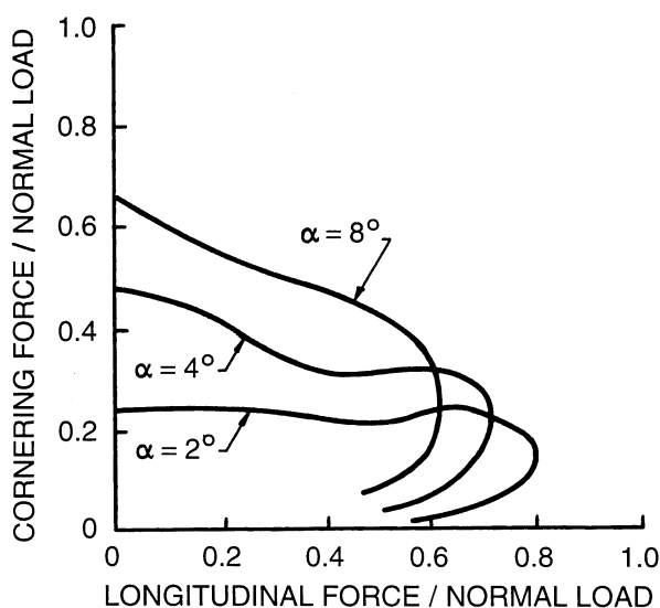
Fig. 1.40 Effect of longitudinal force on the cornering characteristics of truck tires. (Reproduced with permission of the Society of Automotive Engineers from reference 1.23.)
