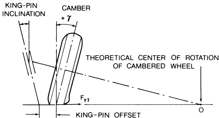
Fig. 1.33 Behavior of a cambered tire.
