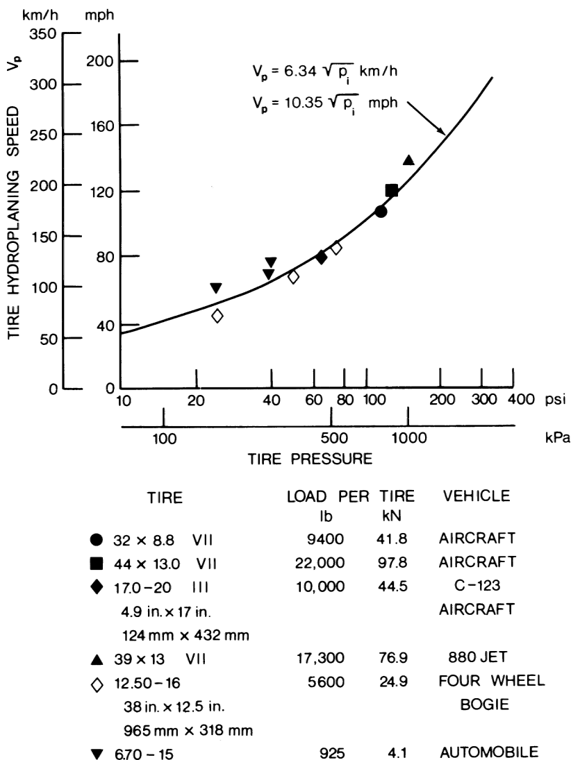
Fig. 1.50 Variation of hydroplaning speed with inflation pressure of tires. (Reproduced with permission of the Society of Automotive Engineers from reference 1.34.)
