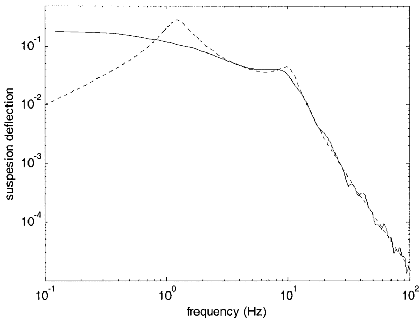
Figure 12-17. Suspension deflection transfer functions for semi-active control with sky hook damping
