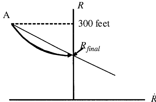
Figure 6-15. Trajectory during coasting
