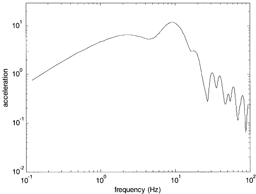
Figure 12-12. FFT of the initial condition response of the semi-active system
