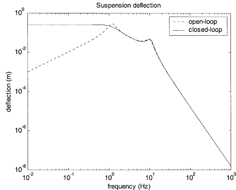
Figure 11-12. Suspension deflection with sky-hook damping
