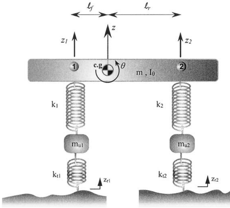
Figure 10-2. Half car automotive suspension model
