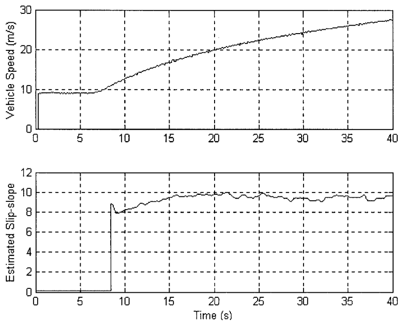
Figure 14-7. Acceleration starting at 20mph on dry concrete surface
