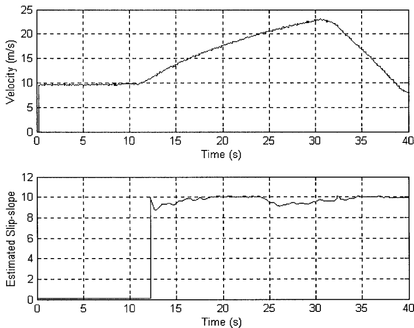
Figure 14-8. Slip-slope estimation during acceleration and braking
