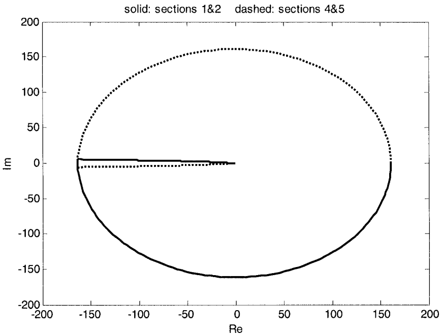
Figure 3-15. Nyquist plot obtained using sections 1, 2, 4 and 5 of the \Gamma_s contour
