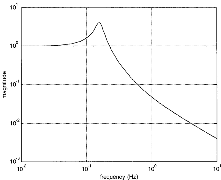
Figure 7-4. Magnitude of G(s) from Eqn. (5)
