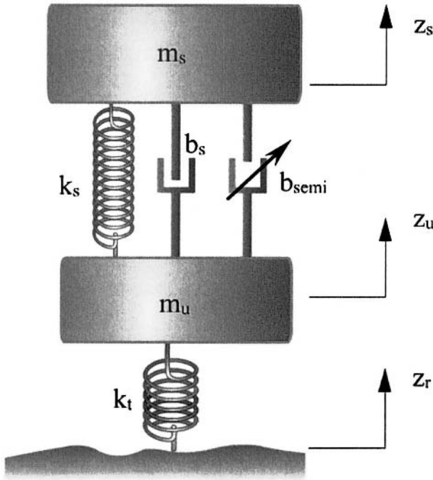
Figure 12-4. Quarter-car active automotive suspension
