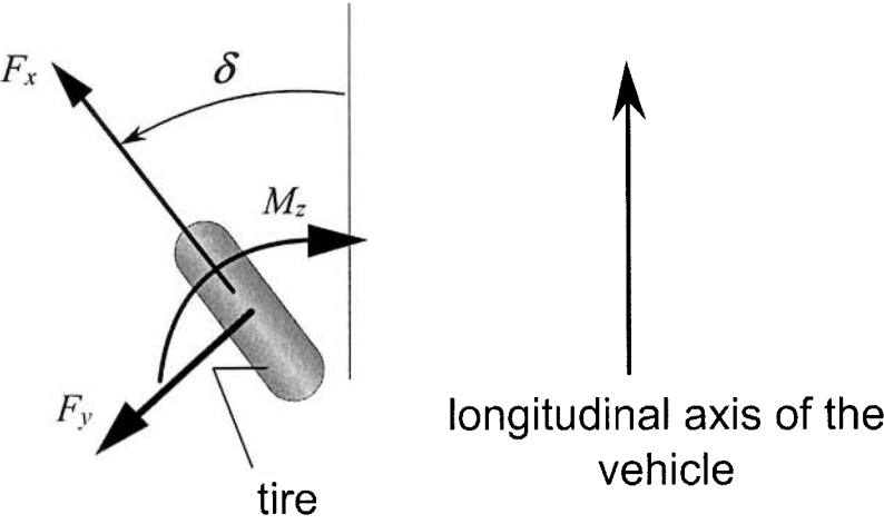
Figure 13-3. Lateral and longitudinal forces and restoring moment
