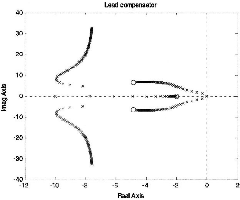
Figure 3-25. Root locus with lead compensator
