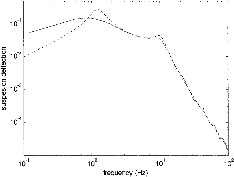
Figure 12-14. Suspension deflection transfer function for a performance index with moderate weights
