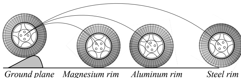
FIGURE 1.20. The difference between aluminum, magnesium, and steel rims in regaining road contact after a jump.
