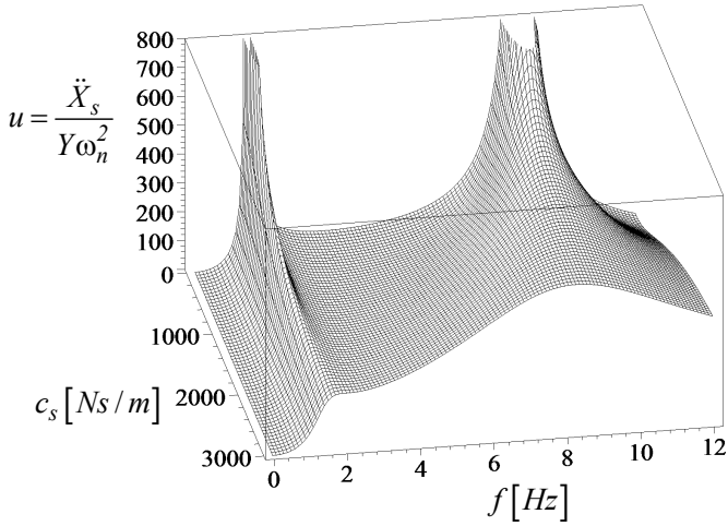
FIGURE 15.8. Three-dimensional view of the frequency response u = \left| \frac{\ddot{X}_s}{Y\omega_u^2} \right| .
