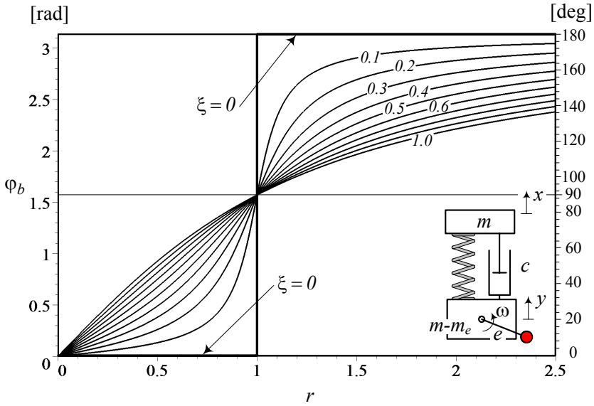
FIGURE 12.37. The frequency response for \varphi_b .
