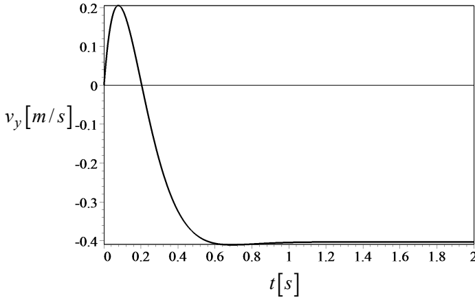
FIGURE 10.30. Lateral velocity response in example 406.
