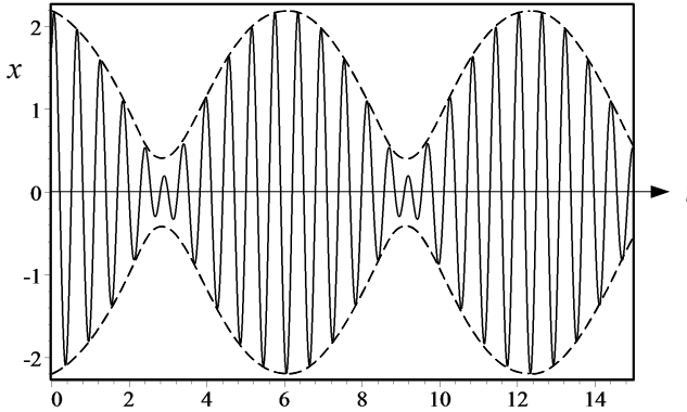
FIGURE 12.22. Beating phenomena.
