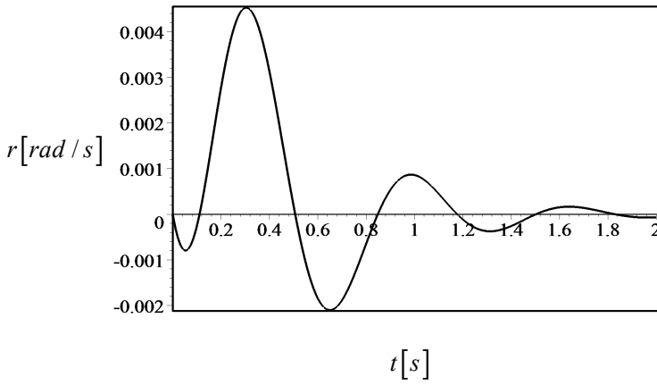
FIGURE 11.10. Yaw rate response over time.
