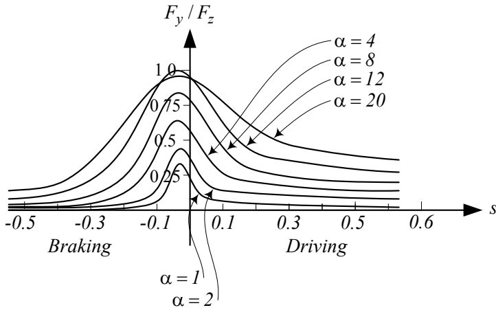
FIGURE 3.54. Lateral force ratio F_y/F_z as a function of slip ratio s for different sideslip \alpha .
