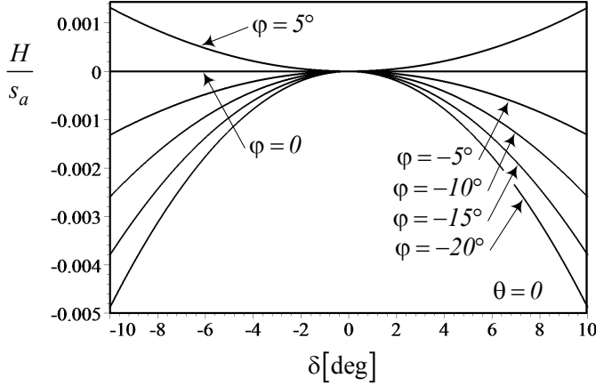
FIGURE 8.54. H/s_a for the caster angle \varphi = 5^\circ , 0^\circ , -5^\circ , -10^\circ , -15^\circ , -20^\circ and the steer angle in the range -10^\circ < \delta < 10^\circ .
