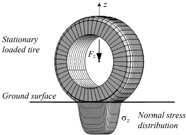
FIGURE 3.11. Normal stress \sigma_z applied on the road because of a stationary tire under a normal load F_z .
