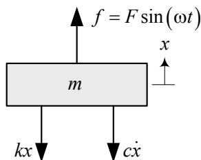
FIGURE 12.18. Free body diagram of the harmonically forced excited, single-DOF system shown in Figure 12.15.
