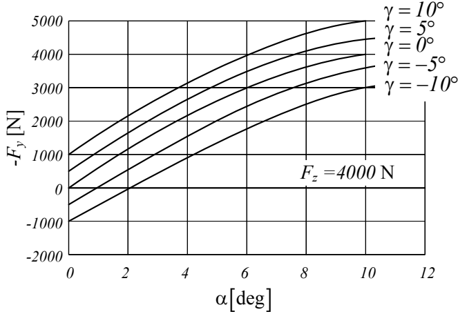
FIGURE 3.52. An example for lateral force as a function of \gamma and \alpha at a constant load F_z = 4000 N.
