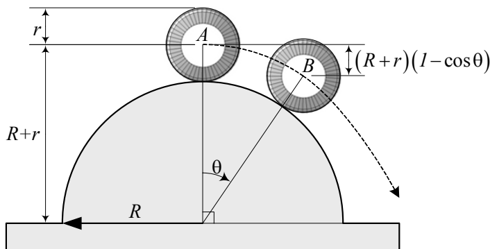
FIGURE 9.16. A wheel turning, without slip, over a cylindrical hill.
