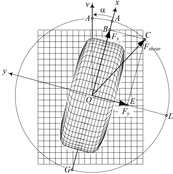
FIGURE 3.58. Friction ellipse.
