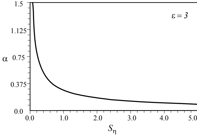
FIGURE 15.35. The optimal value of \alpha as a function of relative displacement RMS S_\eta .
