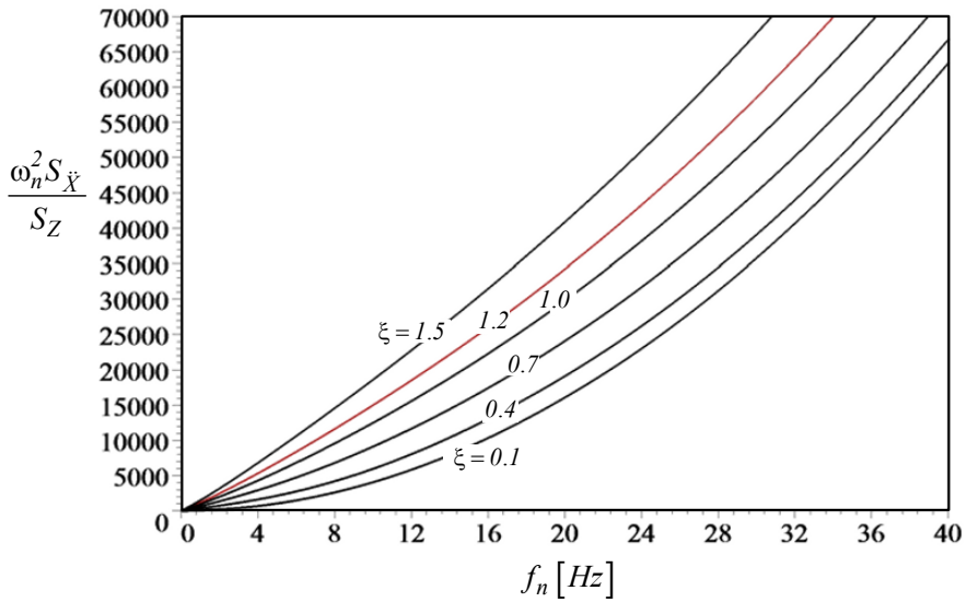
FIGURE 14.12. A plot of ratio \omega_n^2 S_{\ddot{X}} / S_Z versus f_n for different values of \xi .
