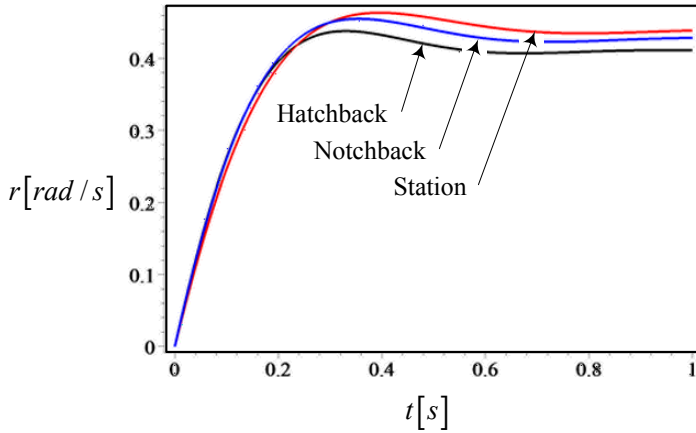
FIGURE 11.28. Yaw rate response for hatchback, notchback, and station models of a car to a step steer angle.
