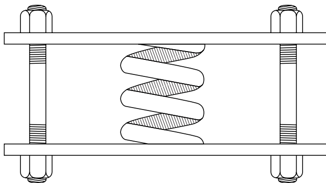
FIGURE 6.21 A simulated model of a bolted joint, in which the joint members are represented by a large spring, here “loaded” by the first two bolts to be tightened.
