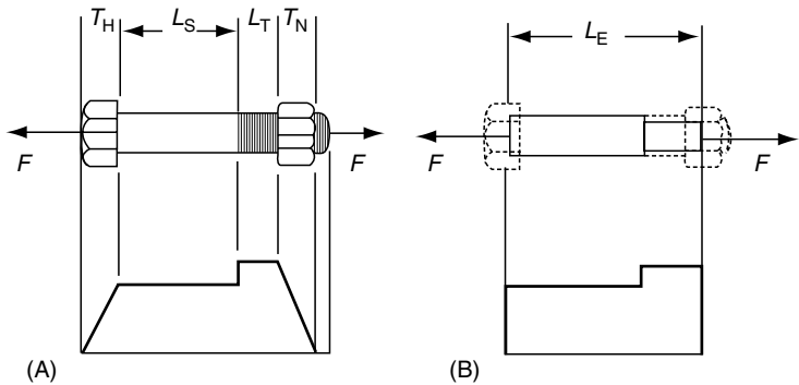
FIGURE 5.3 Illustration of actual bolt configuration and average tensile stress levels (A), and the equivalent configuration and stress distribution assumed for calculation purposes (B).
