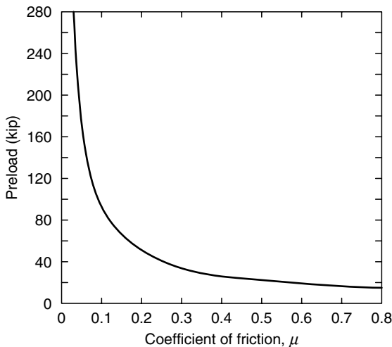
FIGURE 7.7 Theoretical preload achieved for a given input torque as a function of the coefficient of friction.
