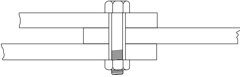
FIGURE 12.3 Any contact between bolts and joint members in a friction-type joint is accidental, so there is no shear stress on the bolts. The space between bolt and joint members is free.
