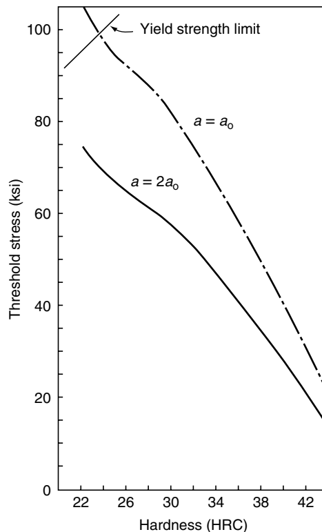
FIGURE 16.9 Plot of threshold stress limits versus hardness for 1½ in. diameter bolts of LAQT steel, used in humid air or chloride-containing aqueous environments. The K_{ISCC} values used to compute threshold stresses were taken from the solid line of Figure 16.7. Crack depths equal to the thread depth (dashed line above) and twice that (solid line) were assumed.
