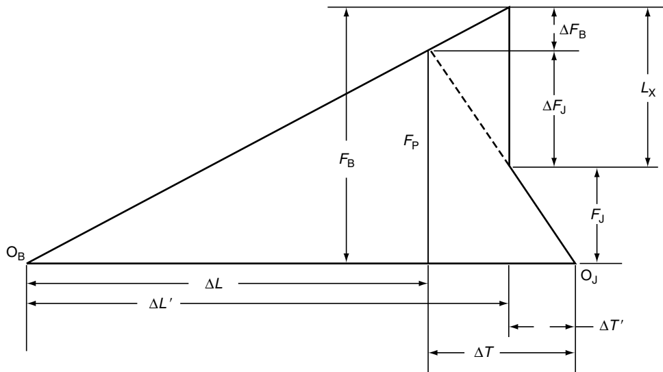
FIGURE 10.12 Summary of the discussion of the joint diagram. F_P is the initial preload; F_B is the present bolt load; F_J is the present joint load; L_X is the external tension load applied to bolt.
