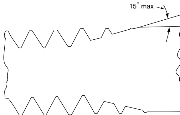
FIGURE 15.23 Thread run-out should be gradual—some people suggest a maximum of 15°—to maximize stress concentrations at this critical point in the fastener.
