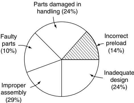
FIGURE 7.9 A summary of the causes of bolted joint failure on the Skylab program. All fasteners have been torqued. (Modified from Investigation of threaded fastener structural integrity, Final report, Contract no. NAS9-15140, DRL-T-1190, CLIN 3, DRD MA 129 TA, Southwest Research Institute, Project no. 15-4665, October 1977.)
