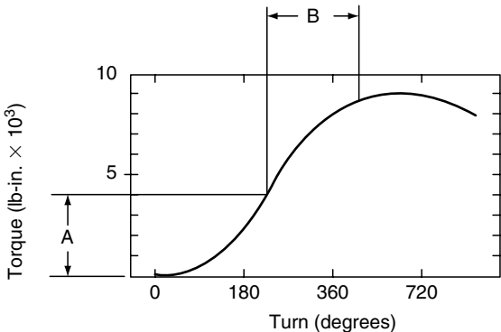
FIGURE 8.11 In turn-of-nut techniques the nut is first tightened with an approximate torque (A) and then further tightened with a measured turn (B). \frac{7}{8} \times 5\frac{1}{2} ASTM A325 bolt.
