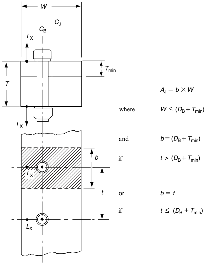
FIGURE 5.11 Sketch of an eccentric joint. The shaded area, b \times W , can be considered that portion of the joint interface which is loaded by a single bolt. See text for the equations used to estimate this area, A_J .
