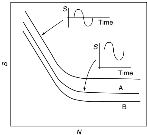
FIGURE 15.5 Increasing the mean stress will reduce the number of cycles to failure produced by a given magnitude of alternating stress. The uppermost curve here is repeated from Figure 15.3 for comparison. The mean stress associated with curve B is higher than that associated with curve A. (Modified from Wayne, D.M., Fatigue design considerations in bolted joints, presented at Using Threaded Fasteners Seminar, University of Wisconsin-Extension, Madison, WI, April 1979.)
