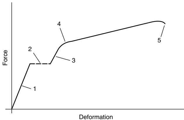
FIGURE 12.9 This chart illustrates the sequence by which a shear joint fails. See text for a discussion.
