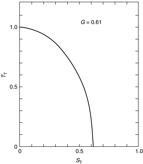
FIGURE 12.10 Elliptic curve used to relate the tensile capacity of a bolt to the shear stress imposed on a bolt, and vice versa. See Equation 12.1 for definition of the terms T_T , S_T , and G . This curve is for static loads on the thread stress area of ASTM A325 or A354 BD bolts. (Modified from Fisher, J.W. and Struik, J.H.A., Guide to Design Criteria for Bolted and Riveted Joints , Wiley, New York, 1974.)
