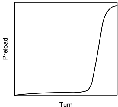
FIGURE 8.5 Turn–preload curve for a sheet metal screw. (Modified from Ehrhart, K.F., Assembly and Fastener , June 1971.)
