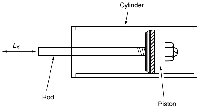
FIGURE 10.34 Joint diagram for a joint loaded in axial compression. The compressive load is L_X ; the resulting bolt tension and joint load are F_B and F_J , respectively. Bolt and joint deflections are \Delta L and \Delta T .
