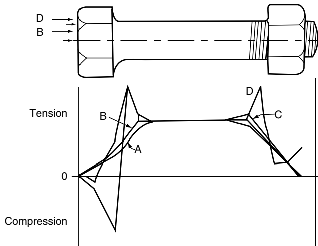
FIGURE 3.5 More accurate view of the tensile stress along four lines parallel to the axis of the bolt (see also Figure 3.6).
