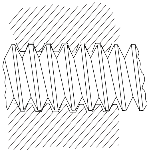
FIGURE 4.7 If the pitch of the male threads differs significantly from that of the female threads, they may be in contact for only part of the length of engagement.
