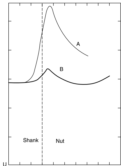
FIGURE 3.9 Relative stress level in nut and bolt threads for a tension nut (curve B) and for a conventional nut (curve A).
