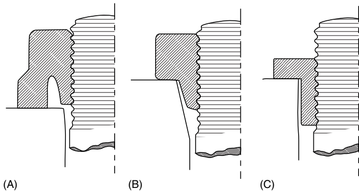
FIGURE 3.8 Nuts which are partially loaded in tension, such as those shown here, see a more uniform tooth stress distribution than do conventional nuts.
