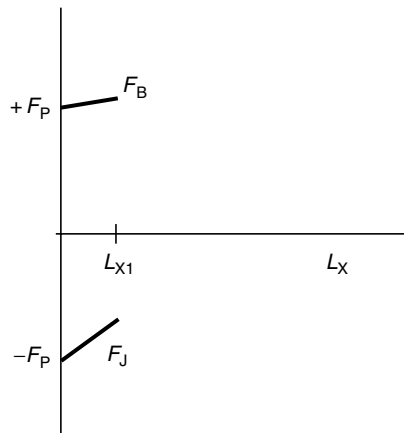
FIGURE 10.18 The initial preloads in bolt and joint are \pm F_P . The bolt load ( F_B ) increases and the joint load ( F_J ) decreases when we apply an external load L_{X1} .
