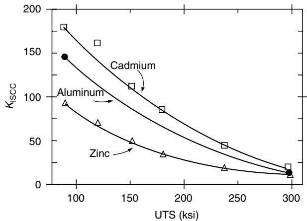
FIGURE 16.15 K_{ISCC} versus tensile strength for low-alloy steel fasteners electroplated with cadmium, aluminum, or zinc. As the chart shows, some platings are more beneficial than others in fighting SCC, but none help very much if the bolts are too hard. (From Raymond, L., Am. Fast. J. , 12ff, March/April, 1993.)
