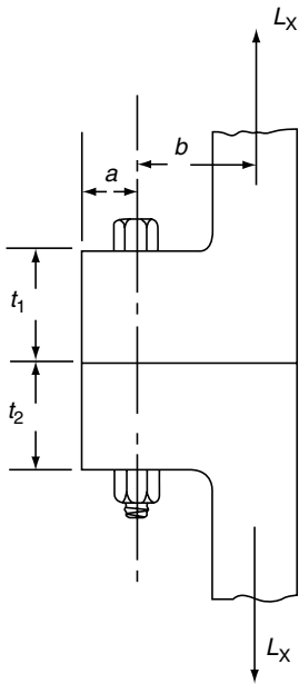
FIGURE 11.7 Prying forces can be reduced by increasing a , t_1 , or t_2 and by decreasing b .
