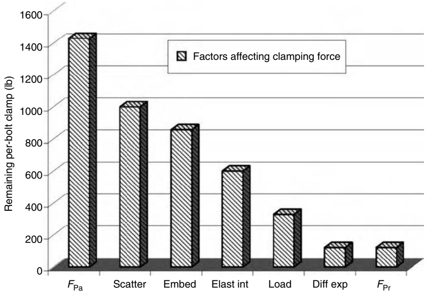
FIGURE 17.9 Chart showing the large difference expected between the average, initial, per-bolt clamping force applied to a joint during assembly ( F_{Pa} ) and the residual, in-service clamping force ( F_{Pr} ) when we assume worst-case tool scatter and embedment losses in bolt tension, plus an average elastic interaction loss, plus the unavoidable losses in clamping force caused by the external tensile load and differential expansion between bolts and joints. This is a plot of the calculations made in Chapter 11.
