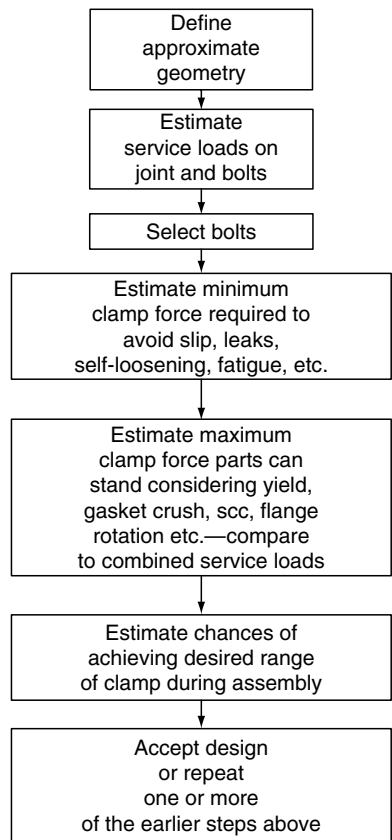
FIGURE 18.1 Block diagram that summarizes the activities involved in the design of bolted joints.
