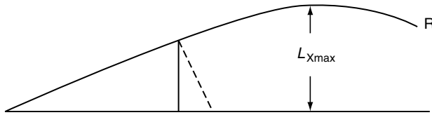
FIGURE 10.16 L_{x\max} is the maximum external load the bolt can support before it ruptures (at R).
