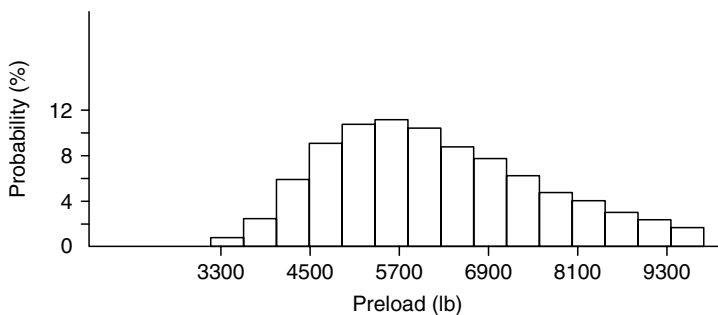
FIGURE 7.5 Histogram of the initial preload achieved in a large number of \frac{5}{16} –24, SAE Grade 8 fasteners with a 2.3 in. grip length tightened to a uniform torque level. (Modified from Eshghy, S., Fastener Technology , July 8, 1978.)
