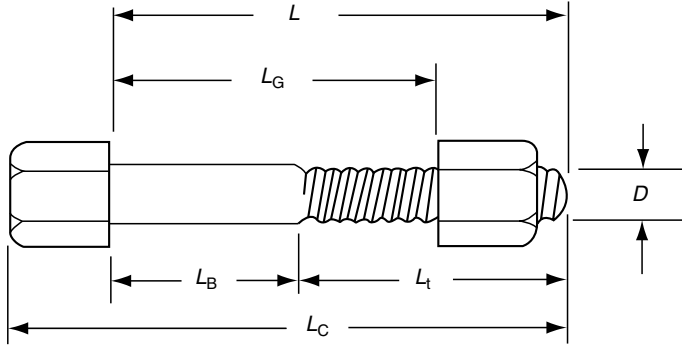
FIGURE 5.5 The bolt whose stiffness and elongation are computed in the text.
