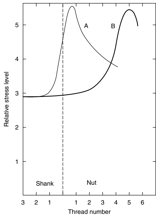
FIGURE 3.10 Stress distribution in threads with nominal pitch (A) and when there is a +0.13% error in the pitch of the bolt threads (B).
