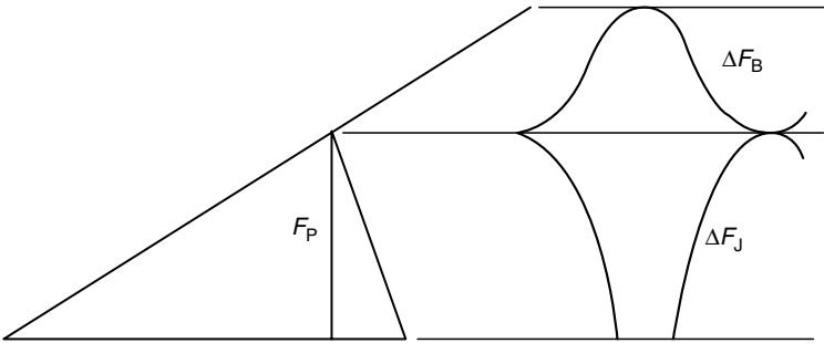
FIGURE 10.32 Joint diagram when the fluctuating external load exceeds the critical load.
