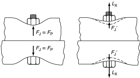
FIGURE 10.6 Forces on the tightened bolt and joint deflection before and after application of external tension load L_X .
