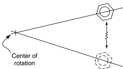
FIGURE 14.4 Vibration along the circular path will sometimes tighten, sometimes loosen, and sometimes do “neither” to a fastener.
