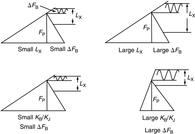
FIGURE 15.13 The load excursions ( \Delta F_B ) in the bolt are increased with an increase in external load ( L_X ) or an increase in the bolt-to-joint stiffness ratio ( K_B/K_J ). Note that the initial preload is the same in each case.
