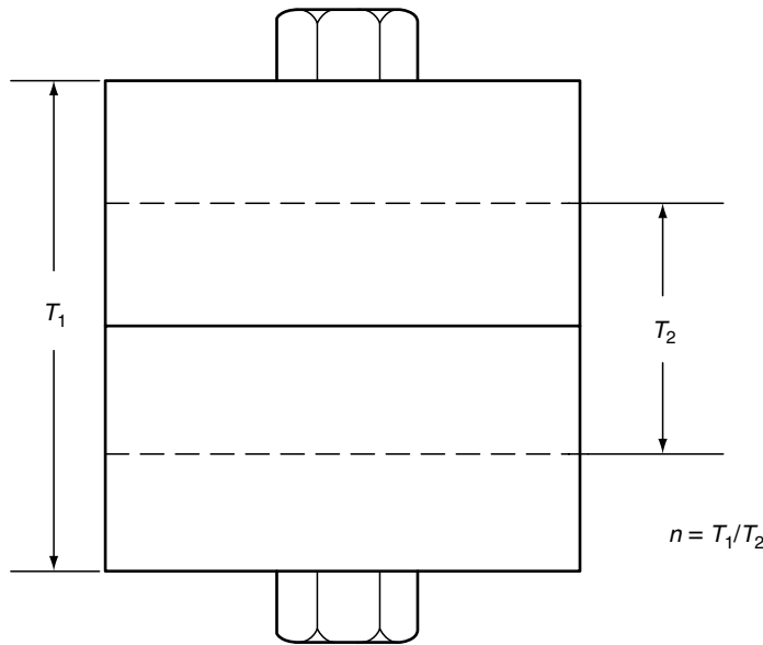
FIGURE 10.27 The “loading plane factor” discussed in the text is defined as the ratio between that portion of the joint which is unloaded by an external tensile load, 7%, and the total thickness of the joint, T_1 .
