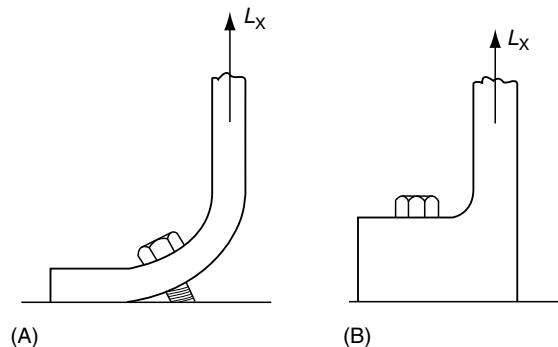
FIGURE 11.2 Joint members can act as levers to pry the bolt. The action is far more severe if the joint members are (A) flexible than if (B) they are not.
