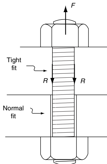
FIGURE 6.6 If there is interference between the bolt and the hole, the clamping force between joint members may be less than the tension in the bolt, changing the torque–clamping force relationship.
