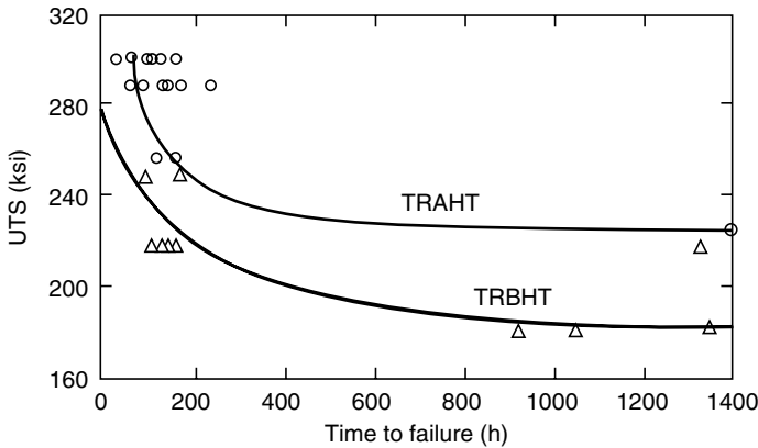
FIGURE 16.6 Rolling fastener threads after heat treatment (TRAHT) gives the fastener greater resistance to SCC than rolling them before heat treatment (TRBHT). The data shown here are based on tests of 1/4–28 × 2 AISI H-11 bolts heat treated to a strength of 260 ksi UTS. (From Hood, A.C., Met. Prog. , September, 1967.)
