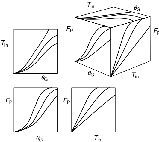
FIGURE 8.10 Anything—such as a change in friction—which affects one view of the torque–turn–preload process must affect the other views as well.
