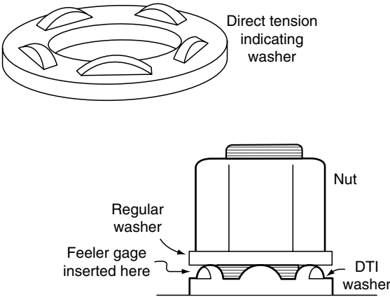
FIGURE 9.5 Direct tension indicator (DTI). This tension-indicating washer can be used under the head of a bolt or, as shown here, under the nut. If it is used under the nut, it is best to interpose a conventional washer between the DTI and nut. (J. & M. Turner, Inc.)
