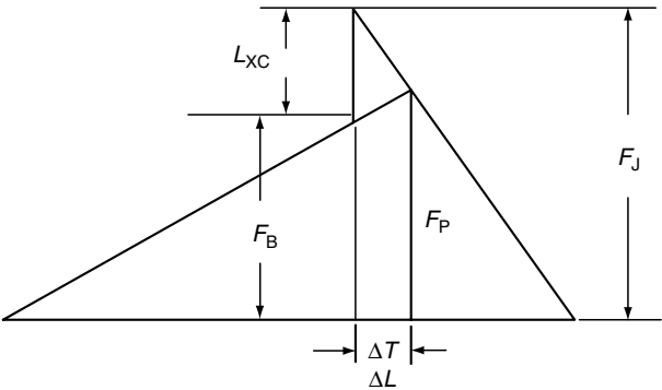
FIGURE 10.33 If a hydraulic cylinder is used in a push-pull mode, the joint between piston and rod will be subjected to alternating tensile and compressive loads. The tensile loads can be analyzed with the joint diagram of Figures 10.12, 10.21, or 10.30. The diagram of Figure 10.34 can be used for the compressive loads.
