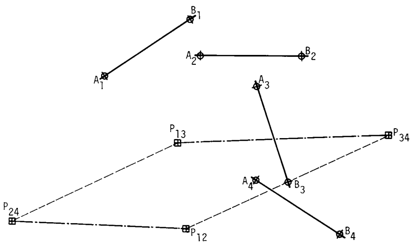
FIGURE 3.13 Four positions of a plane: definition of the opposite-pole quadrilateral formed by lines P_{13}P_{24} and P_{12}P_{34} .
