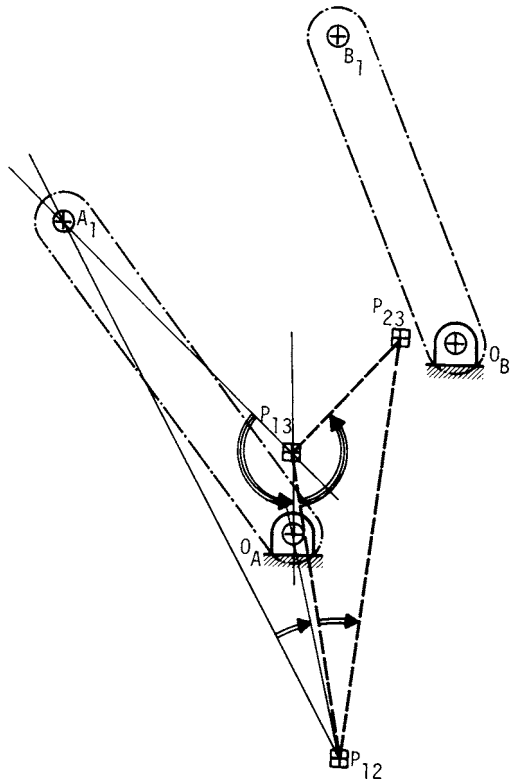
FIGURE 3.12 Determining the moving or fixed pivot by using the pole triangle.
