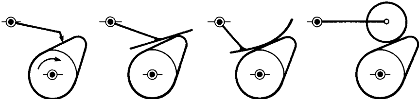
FIGURE 4.3 Plate cams with oscillating followers.
