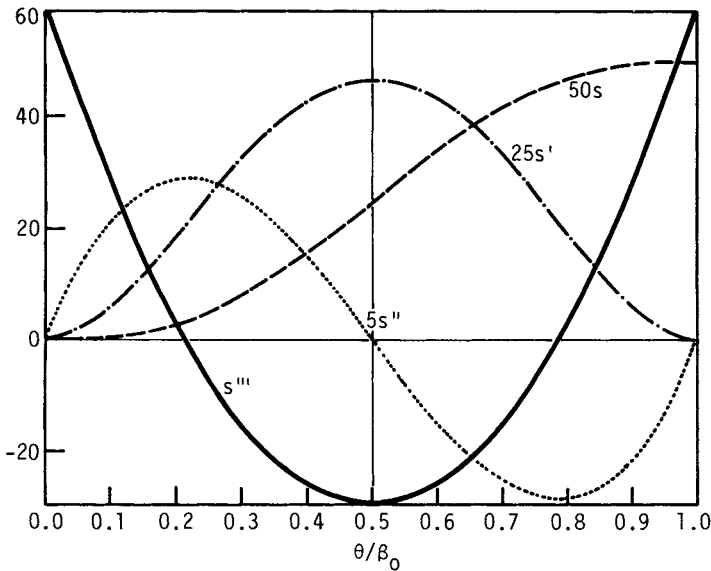
FIGURE 4.11 Full-rise 3-4-5 polynomial motion.
