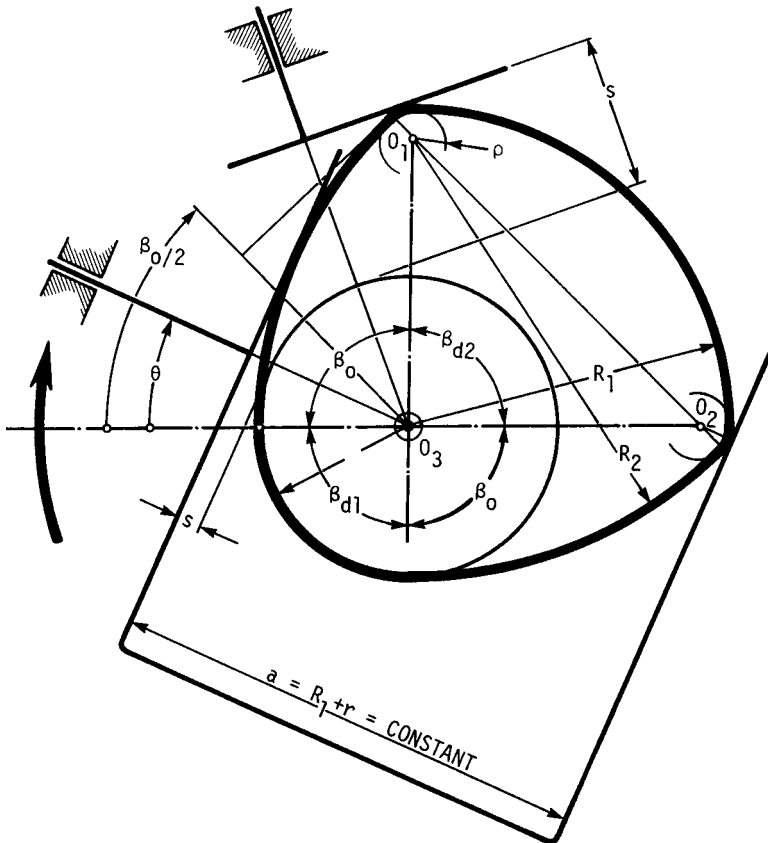
FIGURE 4.12 Constant-breadth circular-arc cam.
