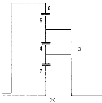
FIGURE 5.9 (a) Planetary train; (b) symbolic notation.
