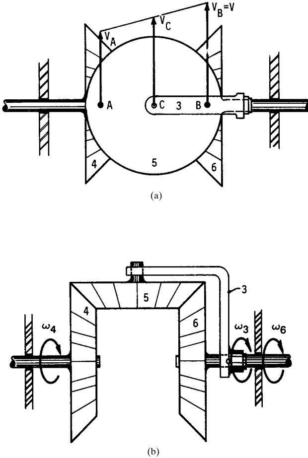
FIGURE 5.10 (a) Top and (b) front views of a bevel-gear differential used as a mechanical averaging linkage. Point A is the pitch point of gears 4 and 5. Point B is the pitch point of gears 5 and 6.
