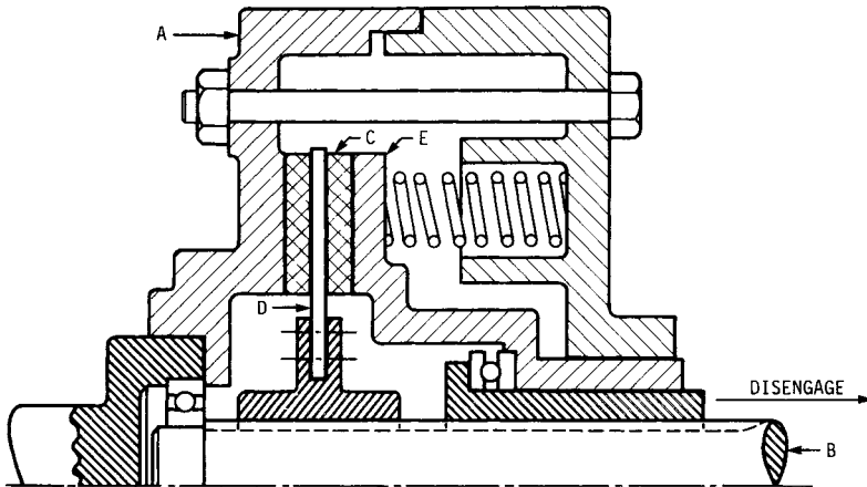
FIGURE 8.2 Schematic drawing of an axial clutch; A, driving member; B, driven shaft; C, friction plates; D, driven plate; E, pressure plate.
