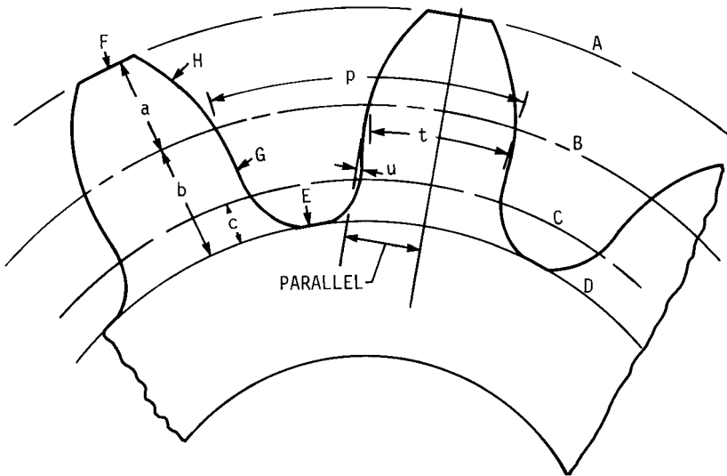
FIGURE 9.1 Terminology of gear teeth. A, addendum circle; B, pitch circle; C, clearance circle; D, dedendum circle; E, bottom land; F, top land; G, flank; H, face; a = addendum distance; b = dedendum distance; c = clearance distance; p = circular pitch; t = tooth thickness; u = undercut distance.
