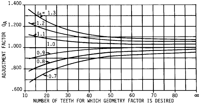
FIGURE 10.22 Addendum adjustment factor Q_A for 25^\circ spur teeth. Addendum factor modification = \delta_a for 1-diametral-pitch gears.
