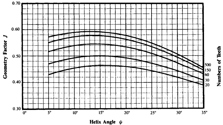
FIGURE 10.30 Geometry factor J for a 20^\circ normal-pressure-angle helical gear. These factors are for standard addendum teeth cut with a finishing hob as the final machining operation. See Fig. 10.31a. (From AGMA 908-B89.)
