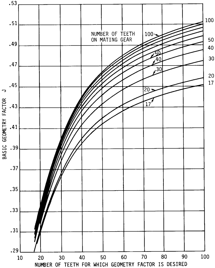
FIGURE 10.11 Basic geometry factors for 20^\circ spur teeth; \phi_N = 20^\circ , a = 1.00 , b = 1.35 , r_T = 0.42 , \Delta t = 0 .
