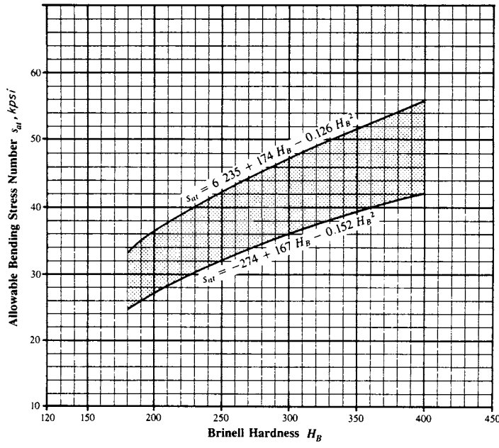
FIGURE 10.41 Allowable bending stress number s_{at} for steel gears. Lower curve is maximum for grade 1 and upper curve is maximum for grade 2. (From Ref. [10.1].)
