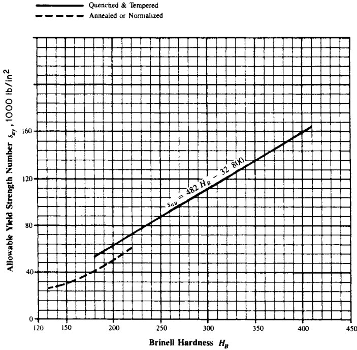
FIGURE 10.46 Allowable yield strength number s_{ay} for steel gears. (From Ref. [10.1].)
