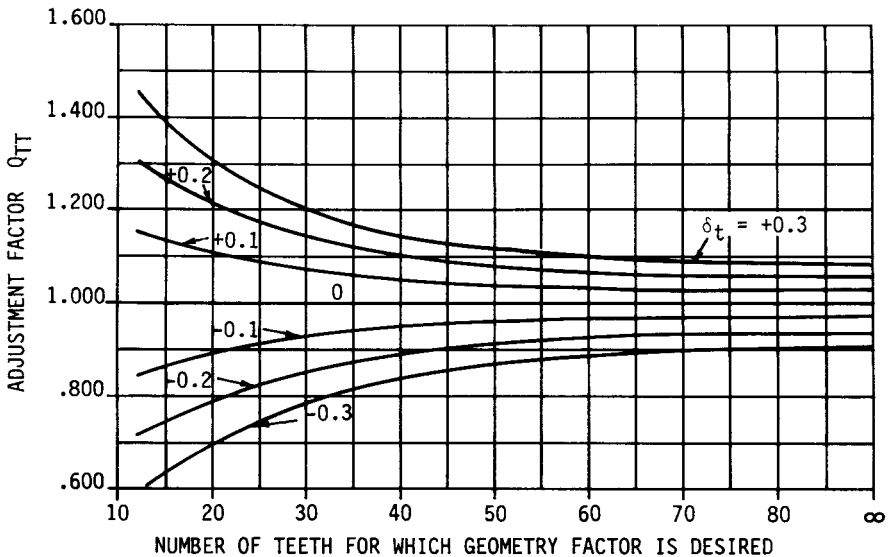
FIGURE 10.19 Tooth thickness adjustment factor Q_{TT} for 25° spur teeth. Tooth thickness modification = \delta_t for 1-diametral-pitch gears.
