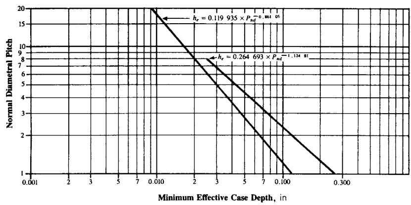
FIGURE 10.42 Effective case depth h_e for carburized gears based on normal diametral pitch. The effective case depth is defined as the depth of case which has a minimum hardness of 50 R_C . The total case depth to core carbon is about 1.5h_e . The values and ranges shown on the case depth curves are to be used as guides. For gearing in which maximum performance is required, detailed studies must be made of the application, loading, and manufacturing procedures to obtain desirable gradients of both hardness and internal stress. Furthermore, the method of measuring the case as well as the allowable tolerance in case depth should be a matter of agreement between the customer and the manufacturer. (From Ref. [10.1].)
