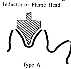
FIGURE 10.45 Variations in hardening patterns obtainable with flame or induction hardening. (From Ref. [10.1].)
