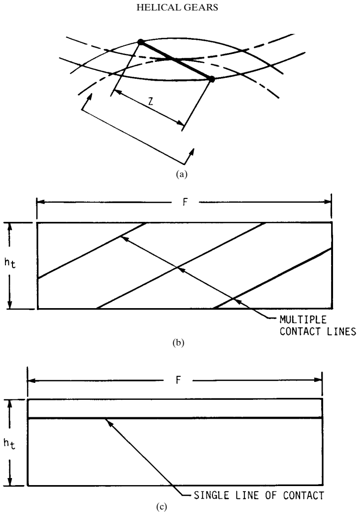
FIGURE 10.3 Comparison of spur and helical contact lines. (a) Transverse section; (b) helical contact lines; (c) spur contact line.
