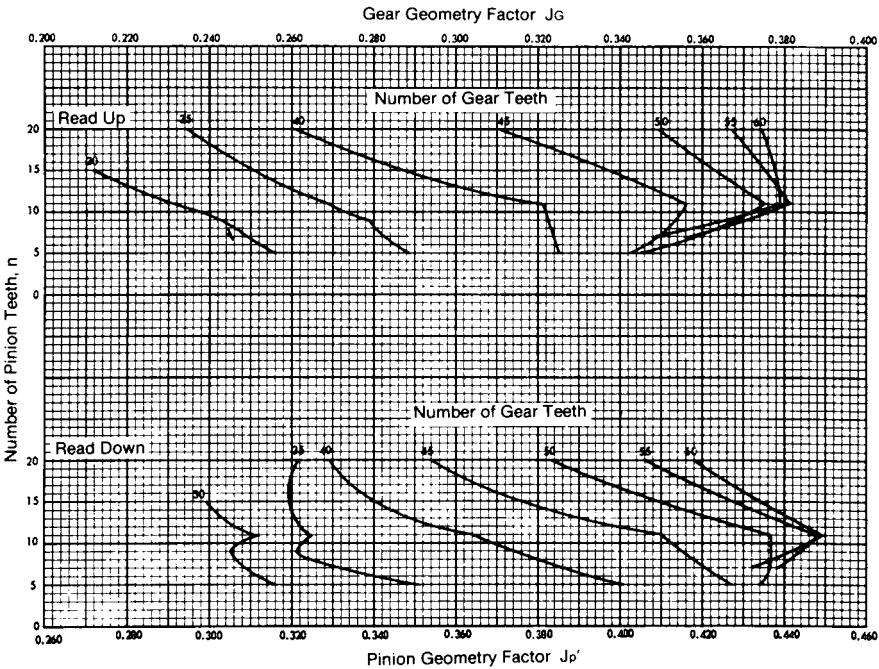
FIGURE 11.48 Geometry factor J for strength of hypoid gears with 22\frac{1}{2}^\circ average pressure angle and E/D ratio of 0.20.
