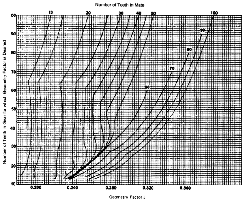
FIGURE 11.22 Geometry factor J for strength of straight-bevel gears with 25° pressure angle and 90° shaft angle.
