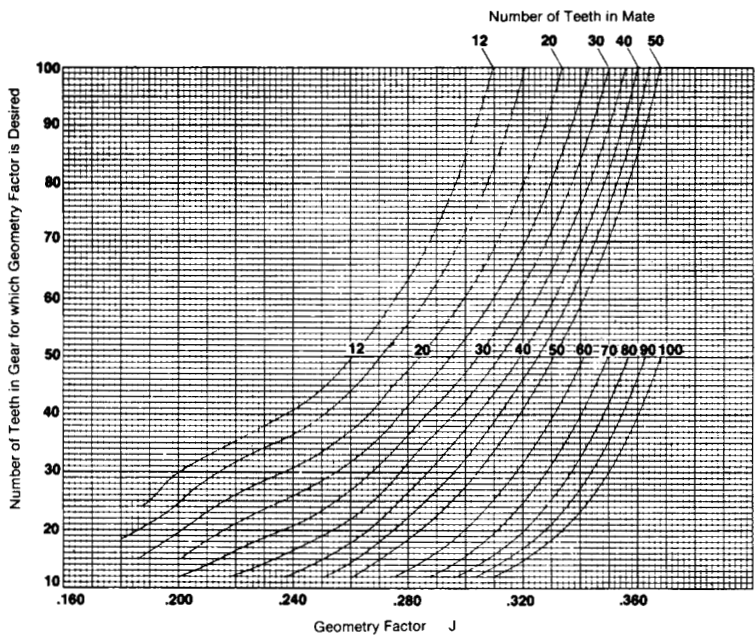
FIGURE 11.32 Geometry factor J for strength of spiral-bevel gears with 20° pressure angle, 35° spiral angle, and 60° shaft angle.
