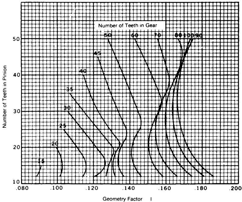
FIGURE 11.33 Geometry factor I for durability of spiral-bevel gears with 20° pressure angle, 35° spiral angle, and 120° shaft angle.
