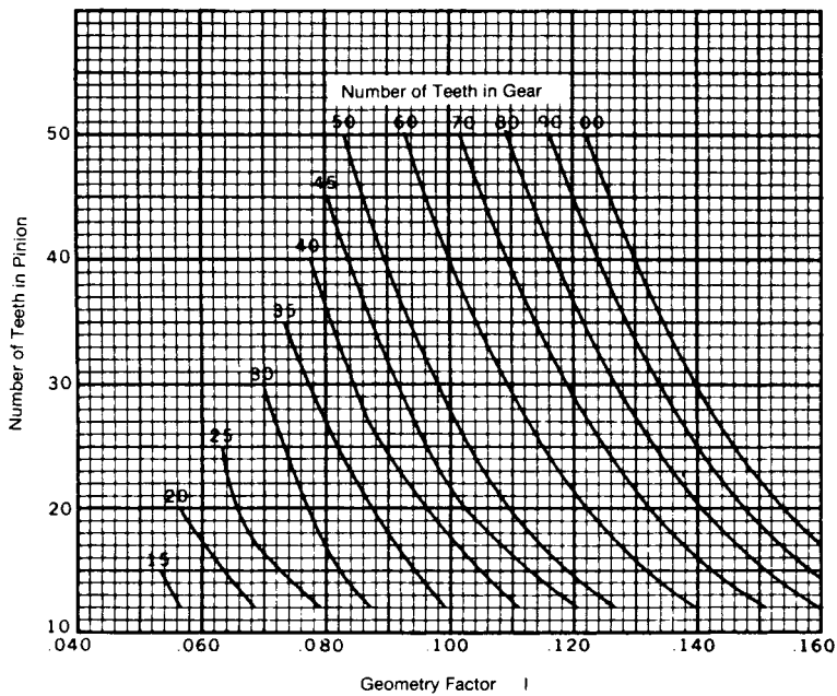
FIGURE 11.31 Geometry factor I for durability of spiral-bevel gears with 20° pressure angle, 35° spiral angle, and 60° shaft angle.
