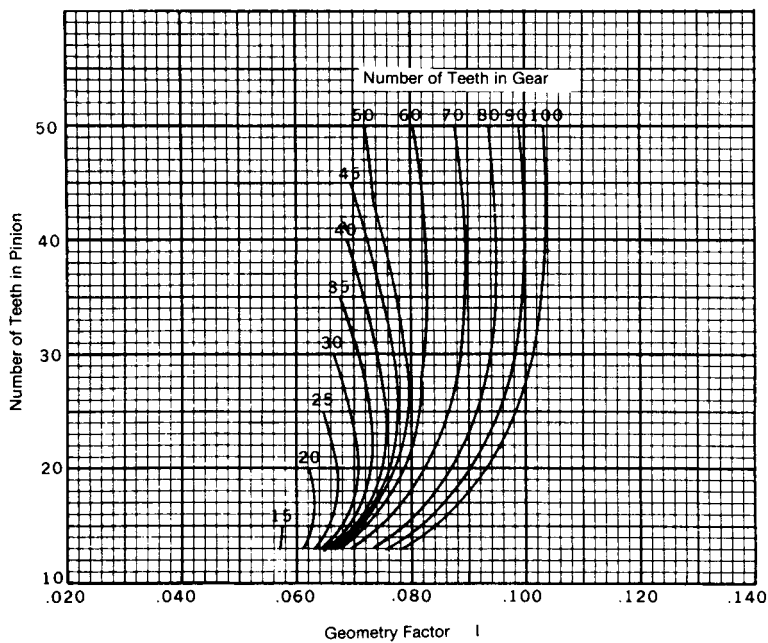
FIGURE 11.21 Geometry factor I for durability of straight-bevel gears with 25° pressure angle and 90° shaft angle.
