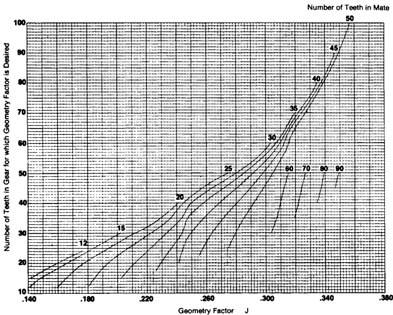
FIGURE 11.34 Geometry factor J for strength of spiral-bevel gears with 20° pressure angle, 35° spiral angle, and 120° shaft angle.
