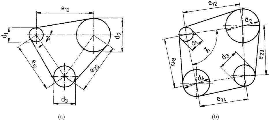
FIGURE 14.2 Multiple-pulley drives.
