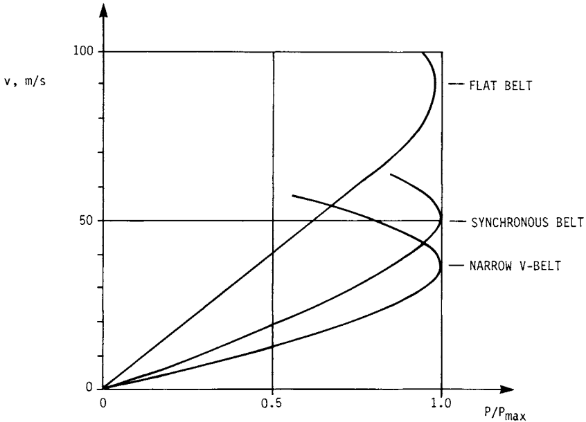
FIGURE 14.35 Optimum velocities.
