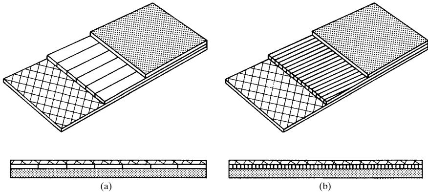
FIGURE 14.15 Multiple-ply belt.
