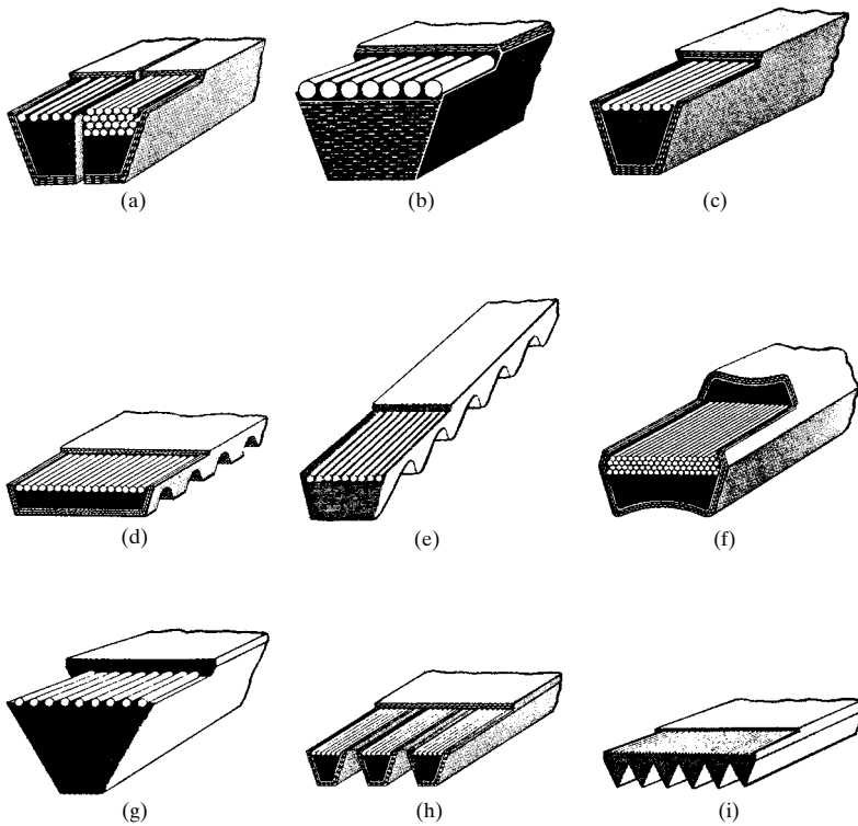
FIGURE 14.20 V-belt configurations.
