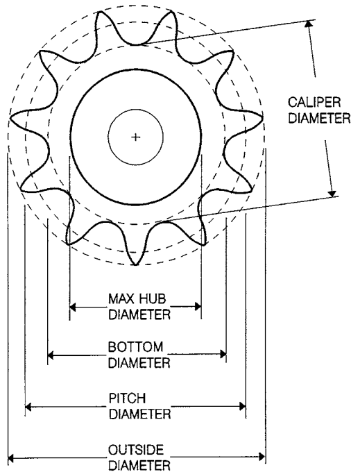
FIGURE 15.2 Roller-chain sprocket diameters. ( Diamond Chain Company. )
