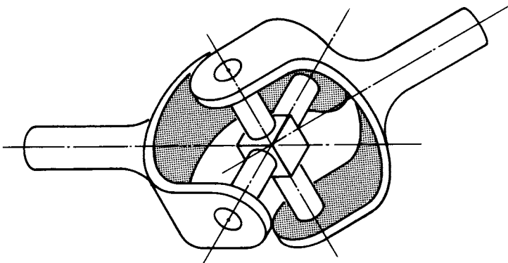
FIGURE 16.36 Basic Hooke's or Cardan universal joint.
