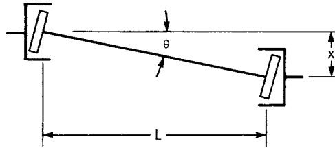
FIGURE 16.20 Diagram shows how parallel misalignment is converted to angular gear coupling mesh. For example, for an extended floating shaft with L = 12 in and \theta = 1^\circ , the misalignment is x = L \tan \theta = 0.20 in. For a standard double-engagement coupling with L = 2 in and \theta = 1^\circ , x = 0.03 , which is significantly less.
