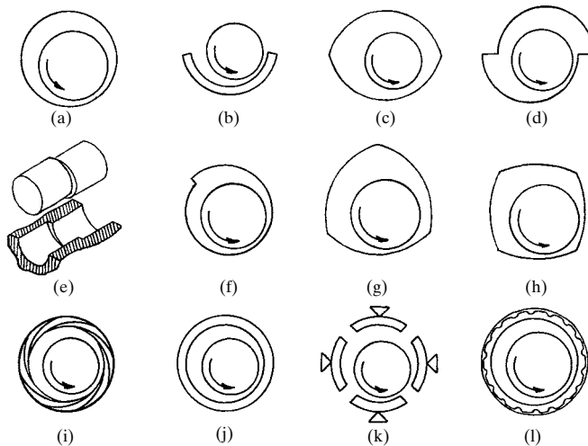
FIGURE 19.3 Journal bearing geometries. (a) Full bearing; (b) partial bearing; (c) elliptical, or lemon, bearing; (d) offset bearing; (e) rocking journal bearing; (f) pressure dam bearing; (g) three-lobe bearing; (h) four-lobe bearing; (i) multileaf bearing; (j) floating-ring bearing; (k) tilting- or pivoted-pad bearing; (l) foil bearing.
