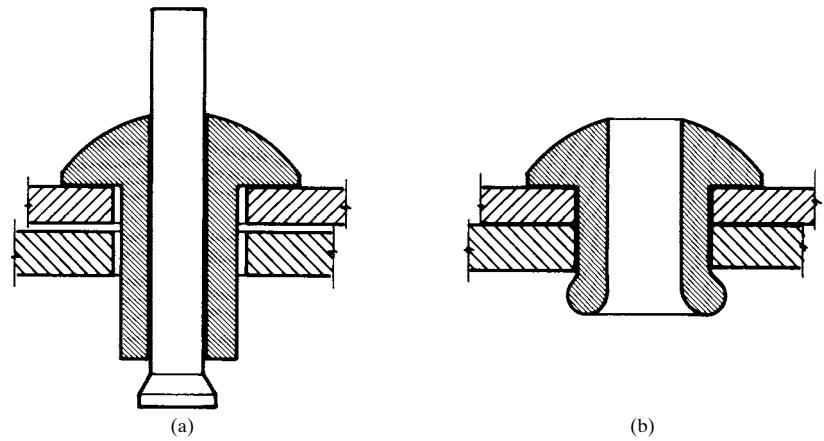
FIGURE 24.5 Pull-through-type blind riveting. (a) Before riveting; (b) after riveting.
