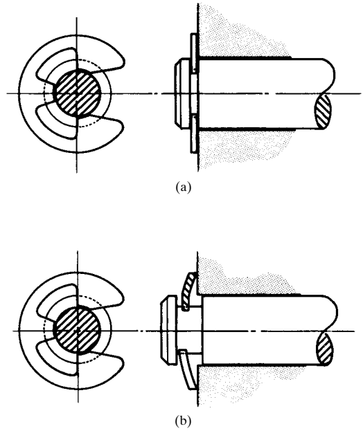
FIGURE 24.14 Open-type E rings. (a) Flat; (b) bowed. (Industrial Retaining Ring Company.)
