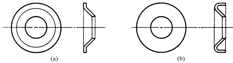
FIGURE 24.22 Finish washers. (a) Flush; (b) raised.
