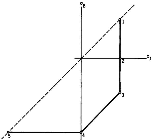
FIGURE 28.1 \sigma_A\sigma_B plane with straight-line Coulomb-Mohr strength locus.
