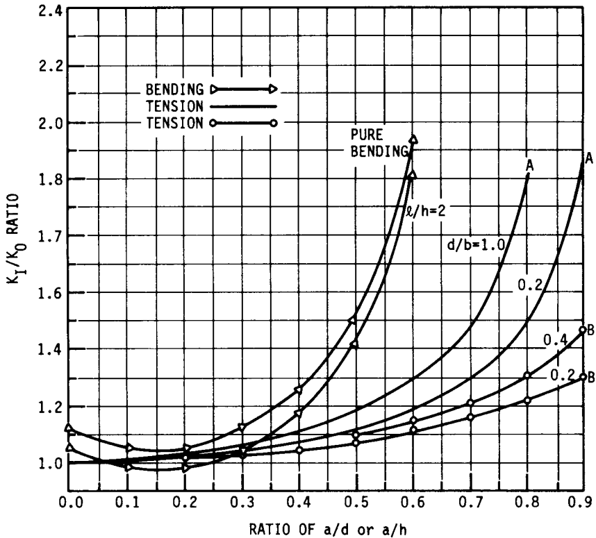
FIGURE 28.19 Stress-intensity charts for cracks shown in Fig. 28.18a and c. Letters A and B identify the ends of the crack shown in Fig. 28.18a. Values of \ell/h > 2 will produce curves closer to the curve for pure bending.
