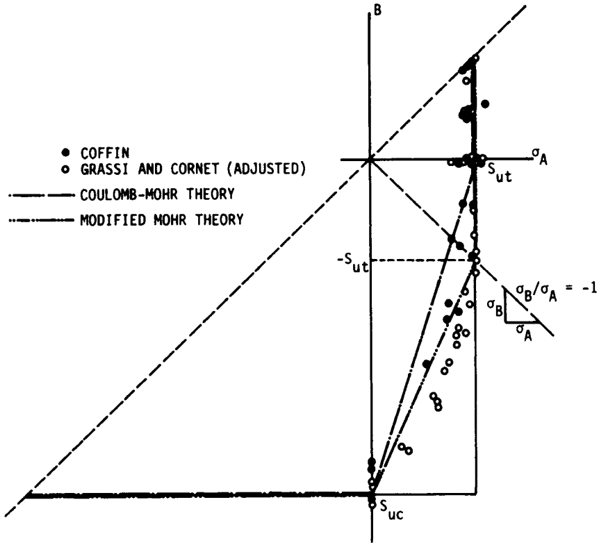
FIGURE 28.2 Experimental data from tests of gray cast iron subjected to biaxial stresses. The data were adjusted to correspond to S_{ut} = 32 ksi and S_{uc} = 105 ksi. Superposed on the plot are graphs of the maximum-normal-stress theory, the Coulomb-Mohr theory, and the modified Mohr theory. (Adapted from J. E. Shigley and L. D. Mitchell, Mechanical Engineering Design , 4th ed., McGraw-Hill, 1983, with permission.)
