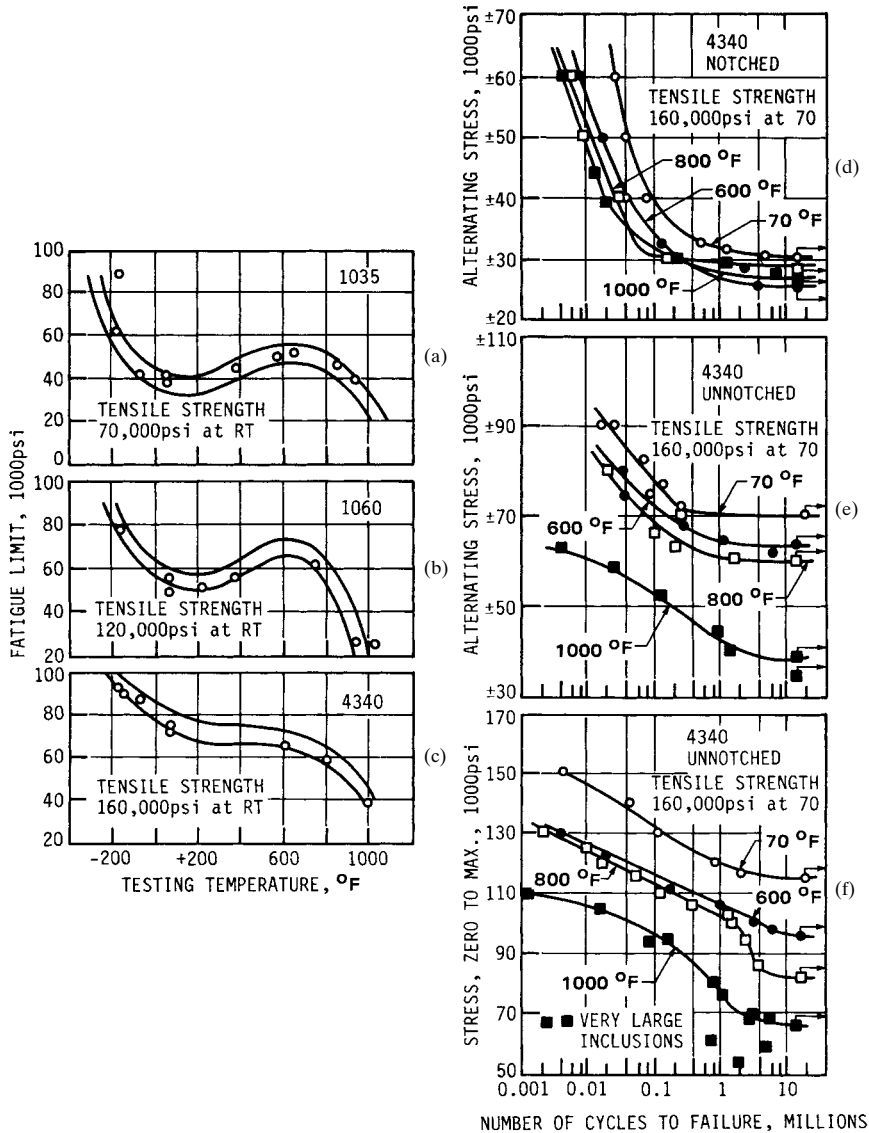
FIGURE 29.9 Effect of temperature on the fatigue limits of three steels: (a) 1035; (b) 1060; (c) 4340; (d) 4340, completely reversed loading K = 3 to 3.5 ; (e) 4340, completely reversed loading, unnotched; (f) 4340, repeatedly applied tension. ( American Society for Metals. )
