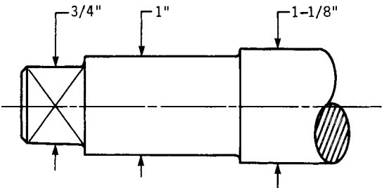
FIGURE 29.17 A portion of a 4140 steel shaft quenched in still oil ( H = 0.35 ) and tempered for 2 hours at 1000°F, grain size 7.5.
