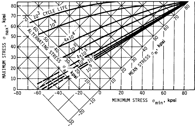
FIGURE 29.6 Fatigue-strength diagram for 7075-T6 aluminum alloy, axial loading. Average of test data for polished specimens (unclad) from rolled and drawn sheet and bar. Static properties: S_u = 82 kpsi, S_y = 75 kpsi. (Grumman Aerospace Corp.)
