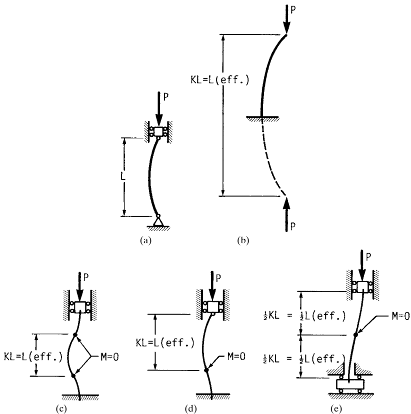
FIGURE 30.2 Effective column lengths for different types of support. (a) Simply supported, K = 1 ; (b) fixed-free, K = 2 ; (c) fixed-fixed, K = 1/2 ; (d) fixed-pinned, K = 0.707 ; (e) ends nonrotating, but have transverse translation.
