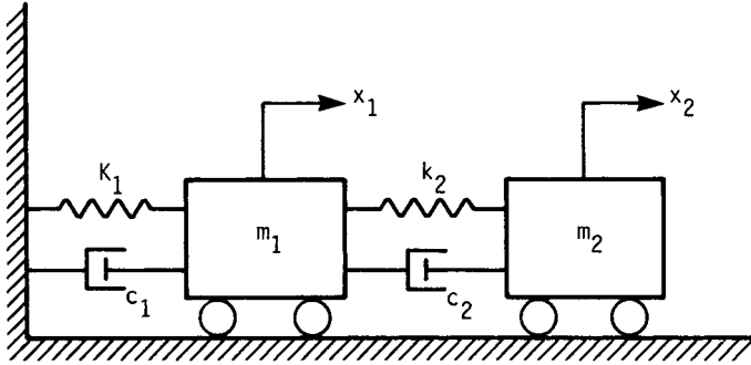
FIGURE 31.18 Two-degree-of-freedom system.
