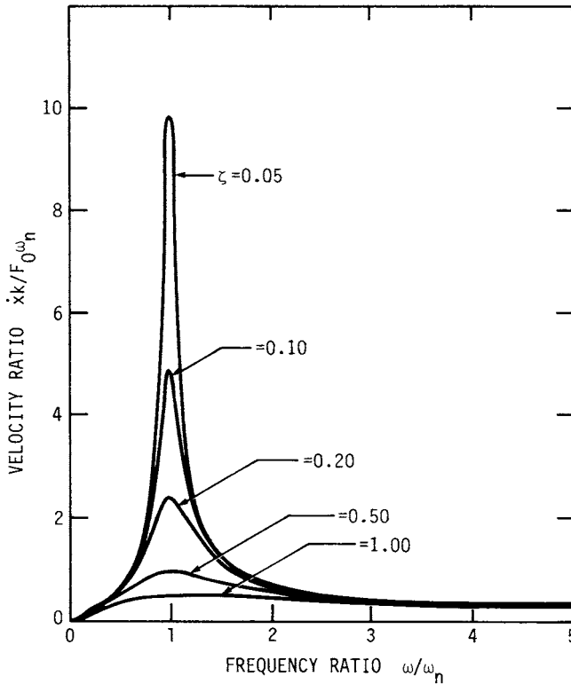
FIGURE 31.10 Velocity frequency response.
