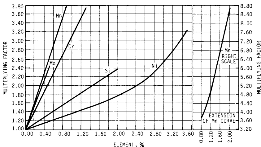
FIGURE 33.13 Multiplying factors for five common alloying elements (for trace copper, use nickel curve). (From [33.4] with permission of Pitman Publishing Ltd., London).
