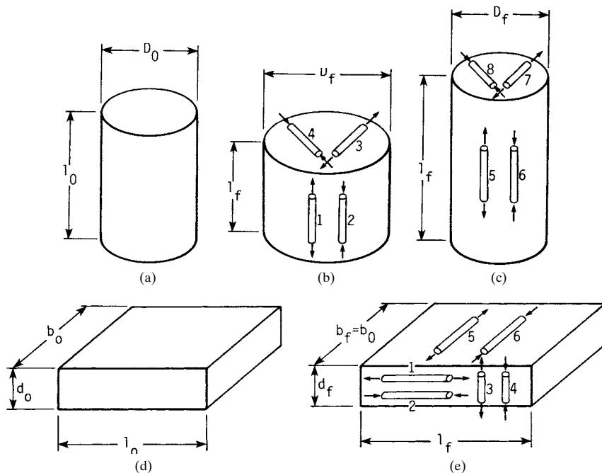
FIGURE 33.1 Sense of strengths in bar and plate. (Adapted from [33.1], p. 7-7 with permission.)
