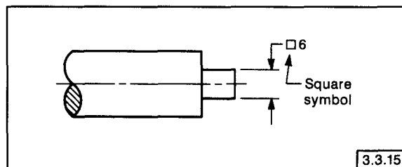
FIG. 3-15 SQUARE SYMBOL
