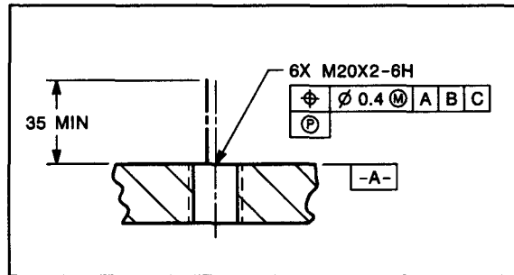
FIG. D-5 FORMER METHOD OF INDICATING A PROJECTED TOLERANCE ZONE
