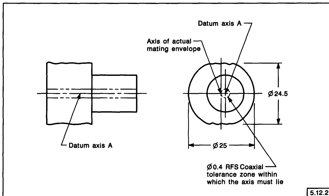
FIG. 5-57 ONE POSSIBLE ACCEPTABLE CONFIGURATION OF PART DEPICTED IN FIG. 5-55
