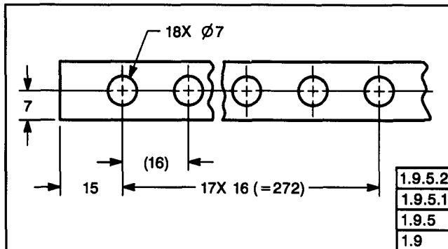
FIG. 1-54 ' REPETITIVE FEATURES AND DIMENSIONS
