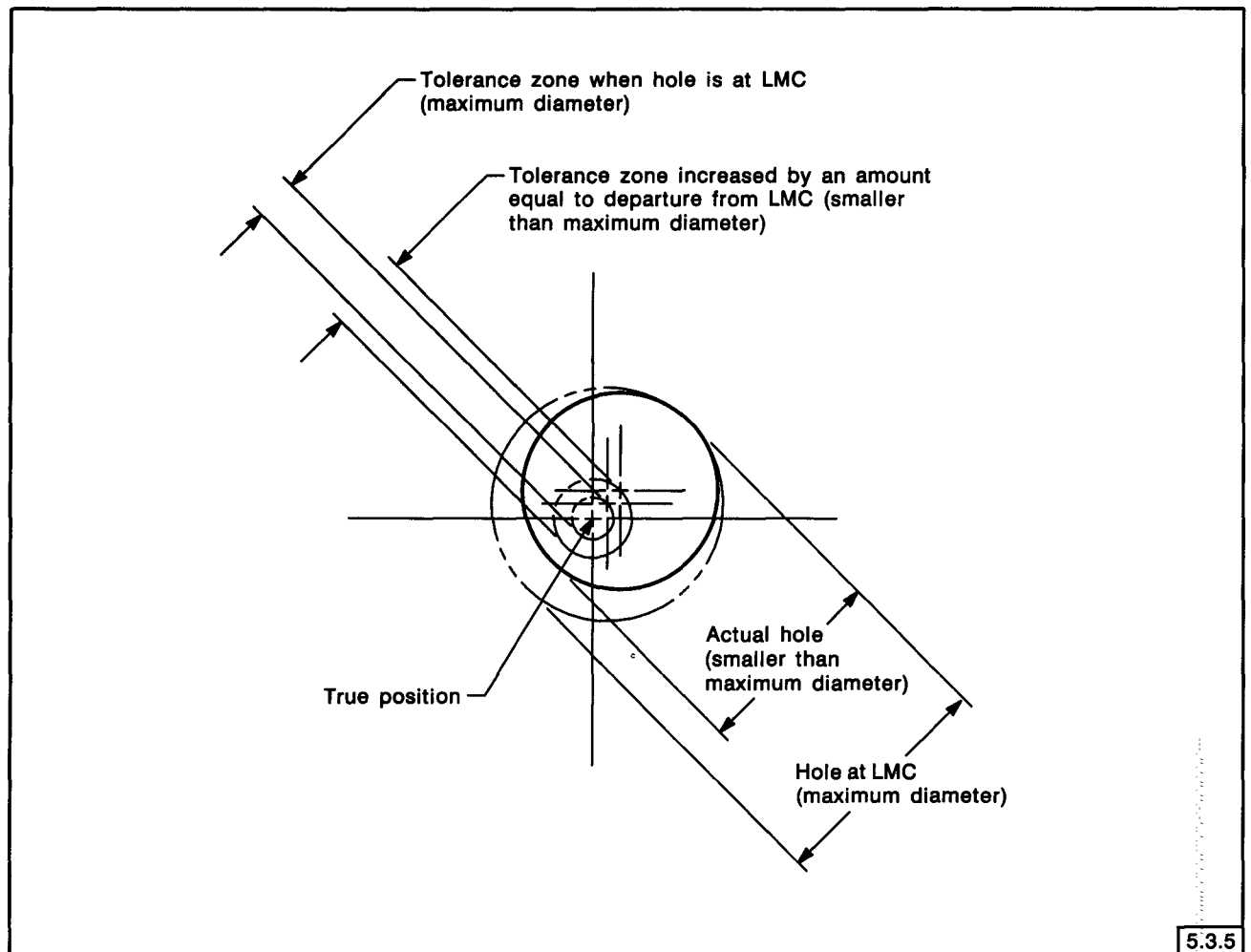
FIG. 5-12 INCREASE IN POSITIONAL TOLERANCE WHERE HOLE IS NOT AT LMC
