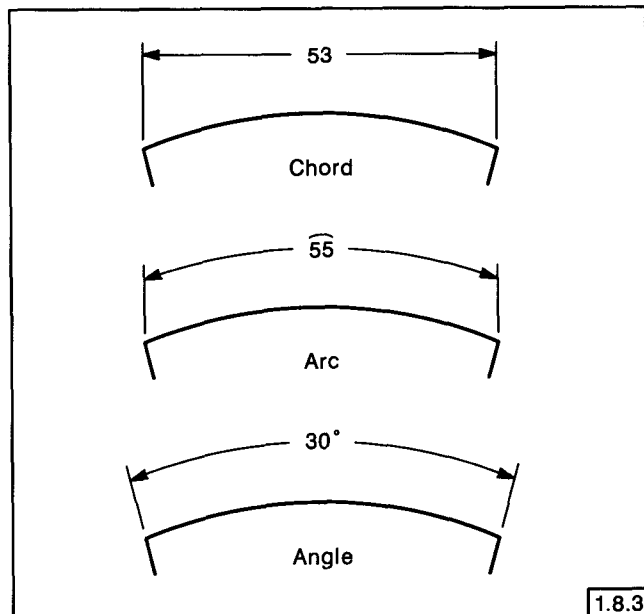
FIG. 1-26 DIMENSIONING CHORDS, ARCS, AND ANGLES
