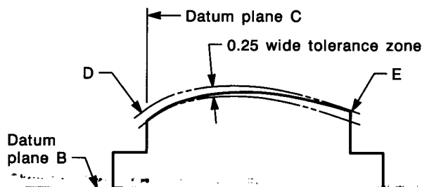
FIG. 6-14 SPECIFYING PROFILE OF A SURFACE BETWEEN POINTS
