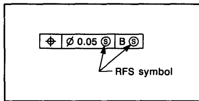
FIG. D-1 FORMER RFS SYMBOL APPLIED TO A FEATURE AND DATUM
