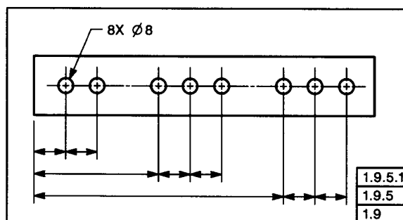
FIG. 1-52 REPETITIVE FEATURES
