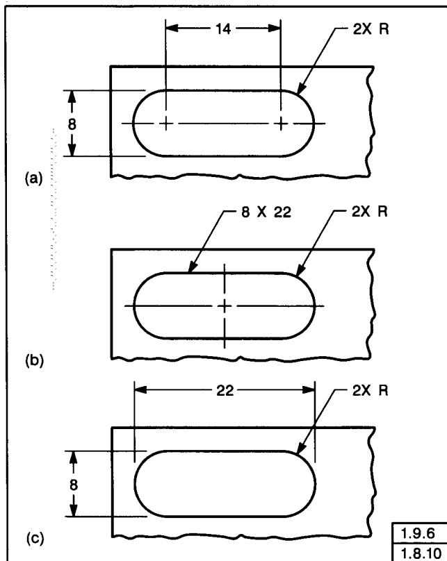
FIG. 1-35 SLOTTED HOLES
