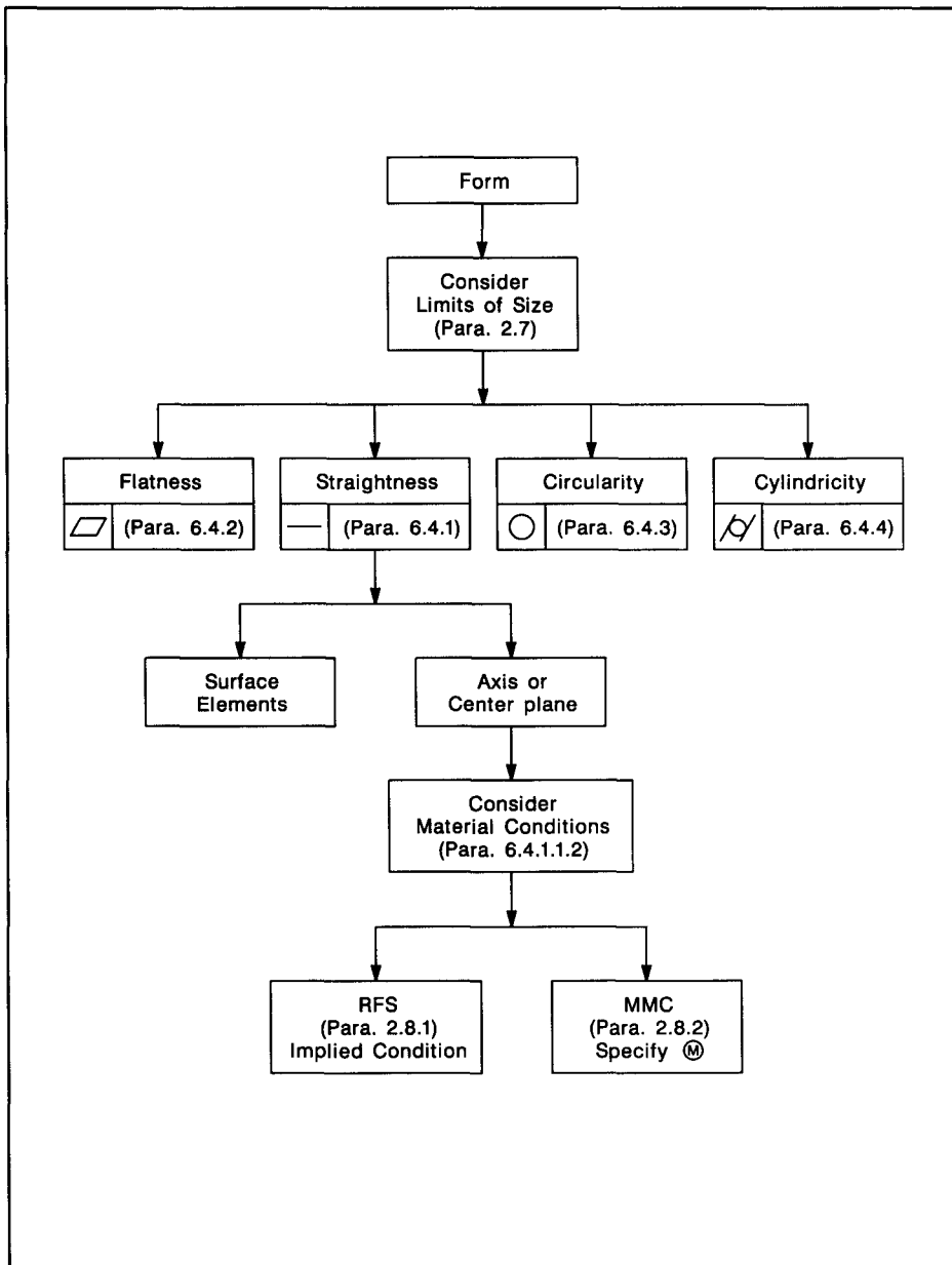
FIG. E-2 FORM
