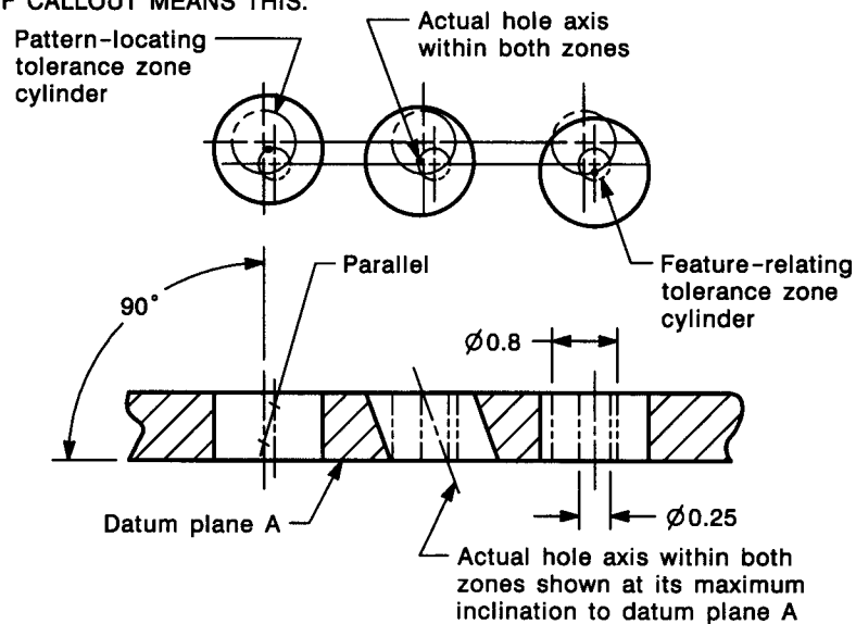
FIG. 5-20 HOLE PATTERNS OF FIG. 5-19 WITH SECONDARY DATUMS IN FEATURE-RELATING SEGMENTS OF COMPOSITE FEATURE CONTROL FRAMES (CONT'D) Tolerance Zones for Three-Hole Pattern (Cont'd)
