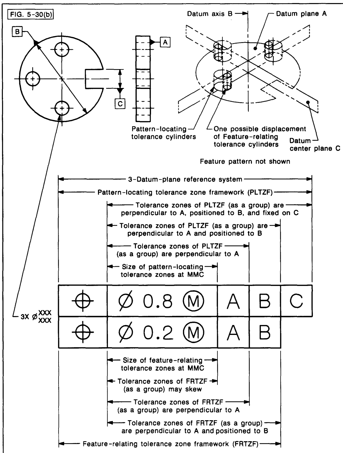
FIG. 5-30 RELATIONSHIPS OF FEATURE-RELATING TOLERANCE ZONE FRAMEWORK (FRTZF) TO PATTERN-LOCATING TOLERANCE ZONE FRAMEWORK (PLTZF) (CONT'D)
