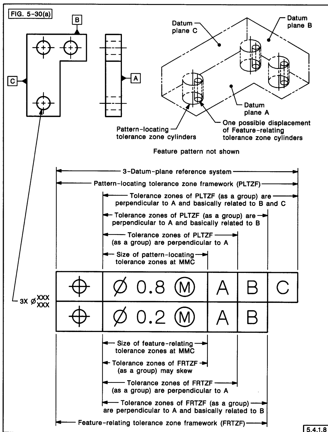
FIG. 5-30 RELATIONSHIPS OF FEATURE-RELATING TOLERANCE ZONE FRAMEWORK (FRTZF) TO PATTERN-LOCATING TOLERANCE ZONE FRAMEWORK (PLTZF)
