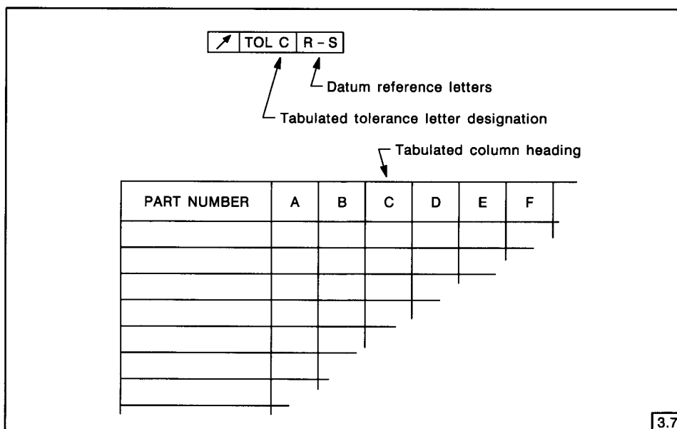
FIG. 3-26 TABULATED TOLERANCES
