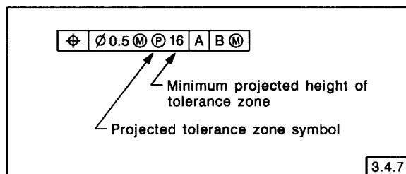
FIG. 3-24 FEATURE CONTROL FRAME WITH A PROJECTED TOLERANCE ZONE SYMBOL
