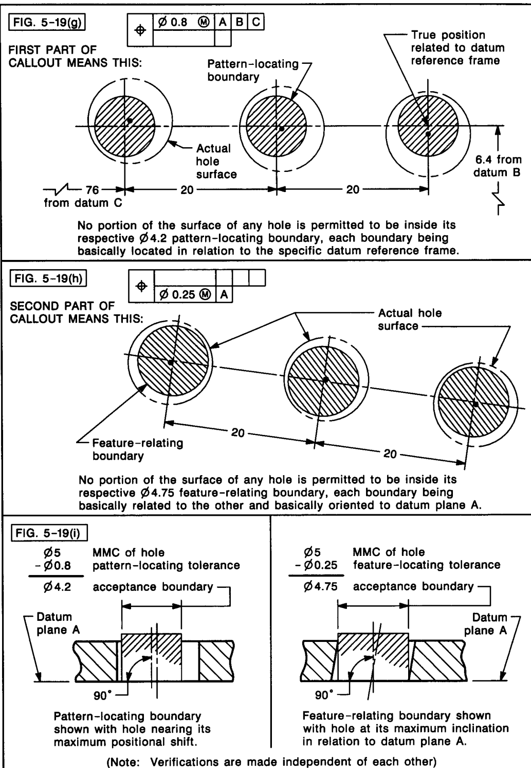
FIG. 5-19 HOLE PATTERNS LOCATED BY COMPOSITE POSITIONAL TOLERANCING (CONT'D) Acceptance Boundaries for Three-Hole Pattern
