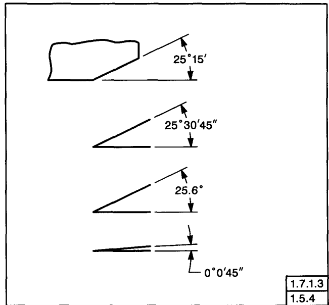
FIG. 1-1 ANGULAR UNITS
