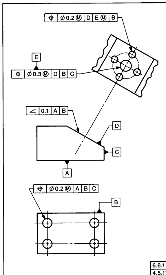
FIG. 4-24 INTERRELATED DATUM REFERENCE FRAMES
