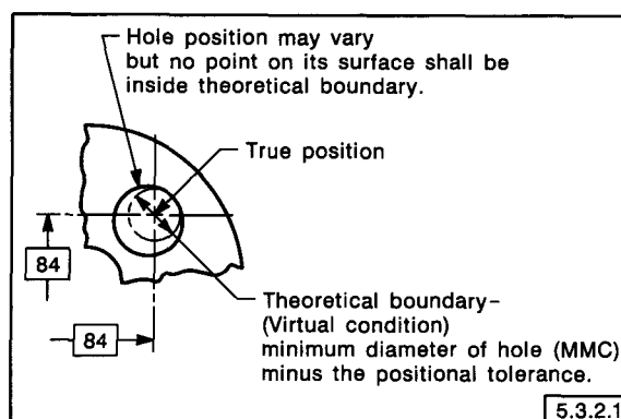
FIG. 5-5 BOUNDARY FOR SURFACE OF HOLE AT MMC
