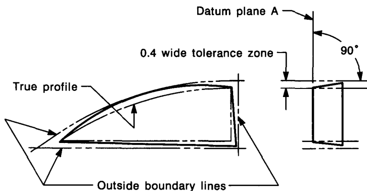
FIG. 6-15 SPECIFYING PROFILE OF A SURFACE FOR SHARP CORNERS
