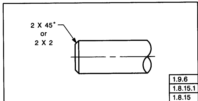
FIG. 1-42 45 DEGREE CHAMFER
