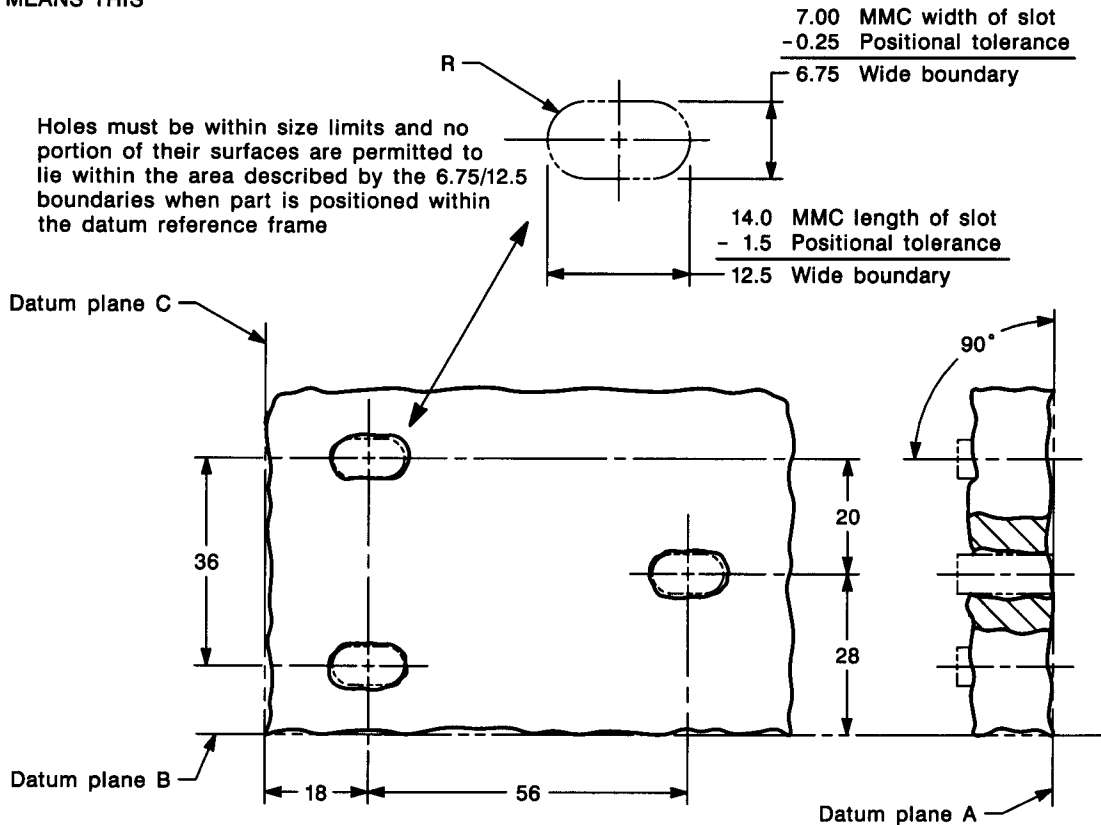
FIG. 5-47 POSITIONAL TOLERANCING OF ENLONGATED HOLES, BOUNDARY CONCEPT
