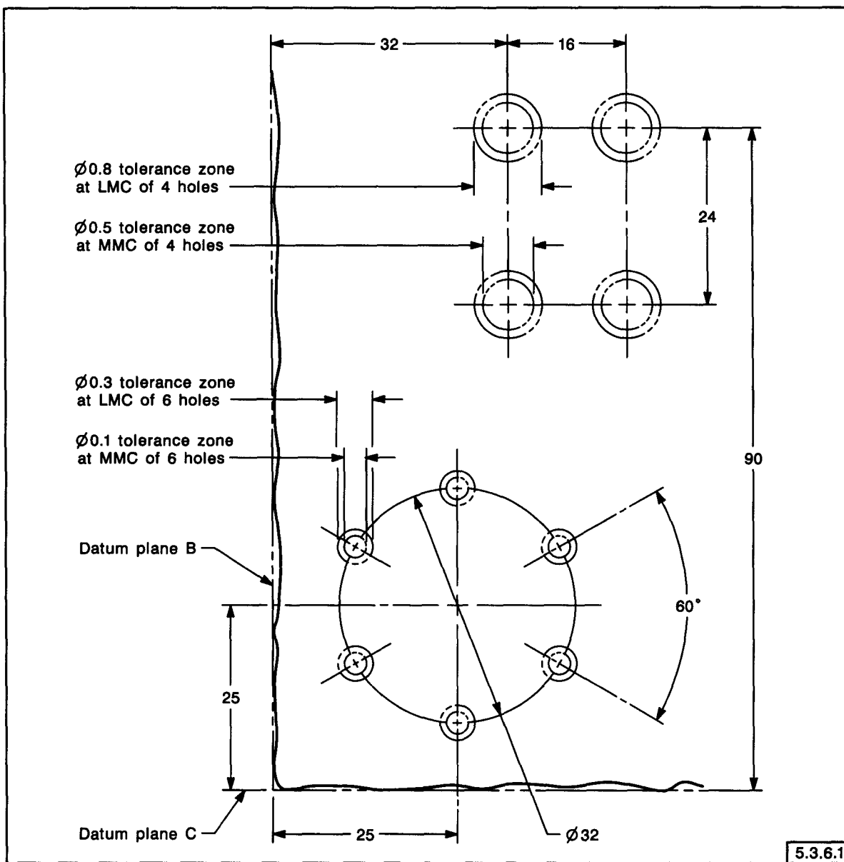
FIG. 5-17 TOLERANCE ZONES FOR PATTERNS SHOWN IN FIG. 5-16
