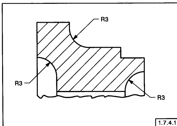
FIG. 1-13 LEADER-DIRECTED DIMENSIONS
