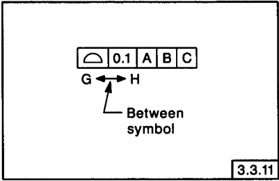
FIG. 3-11 BETWEEN SYMBOL
