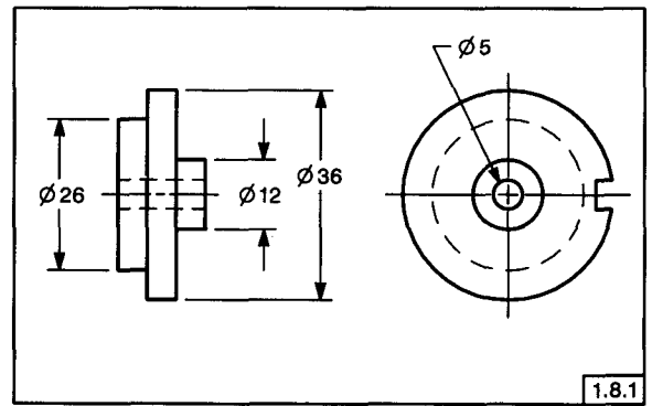
FIG. 1-19 DIAMETERS
