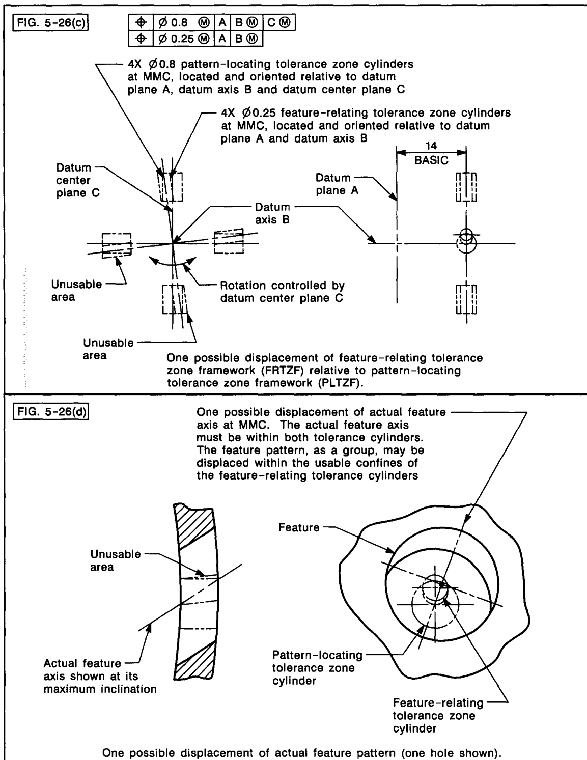
FIG. 5-26 RADIAL HOLE PATTERN LOCATED BY TWO SINGLE-SEGMENT FEATURE CONTROL FRAMES (CONT'D) Tolerance Zones for Radial Hole Pattern (Cont'd)
