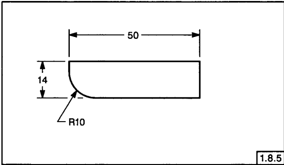
FIG. 1-29 ROUNDED CORNERS
