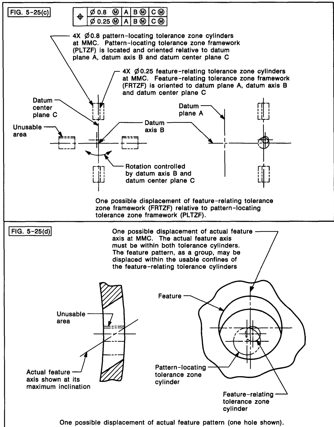
FIG. 5-25 RADIAL HOLE PATTERN LOCATED BY COMPOSITE POSITIONAL TOLERANCING (CONT'D) Tolerance Zones for Radial Hole Pattern (Cont'd)
