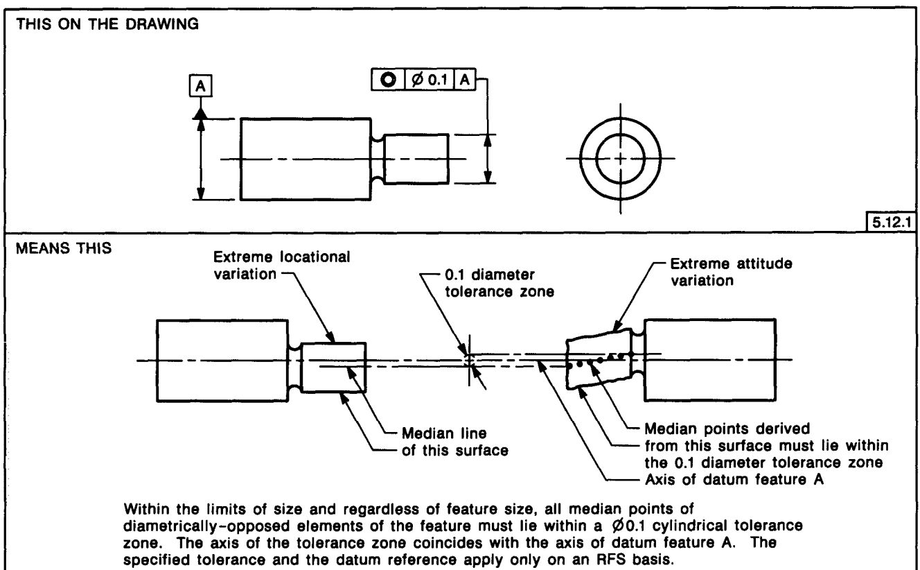
FIG. 5-54 CONCENTRICITY TOLERANCING
