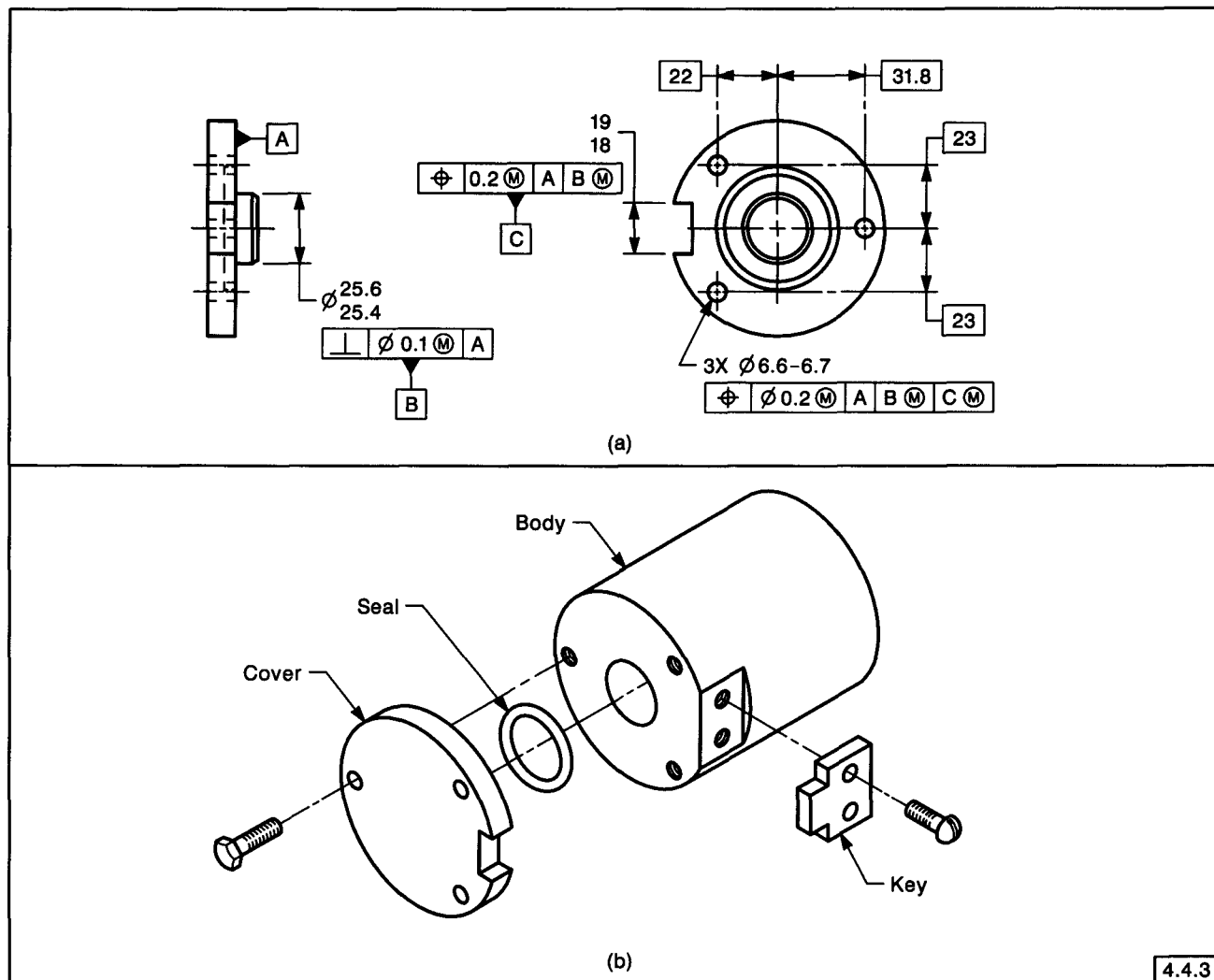
FIG. 4-6 PART WHERE ANGULAR ORIENTATION IS IMPORTANT
