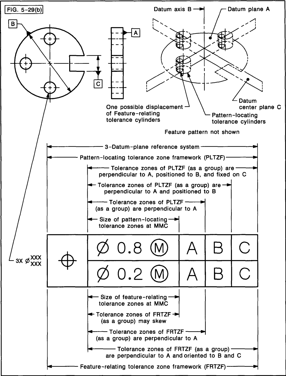
FIG. 5-29 RELATIONSHIPS OF FEATURE-RELATING TOLERANCE ZONE FRAMEWORK (FRTZF) TO PATTERN-LOCATING TOLERANCE ZONE FRAMEWORK (PLTZF) (CONT'D)
