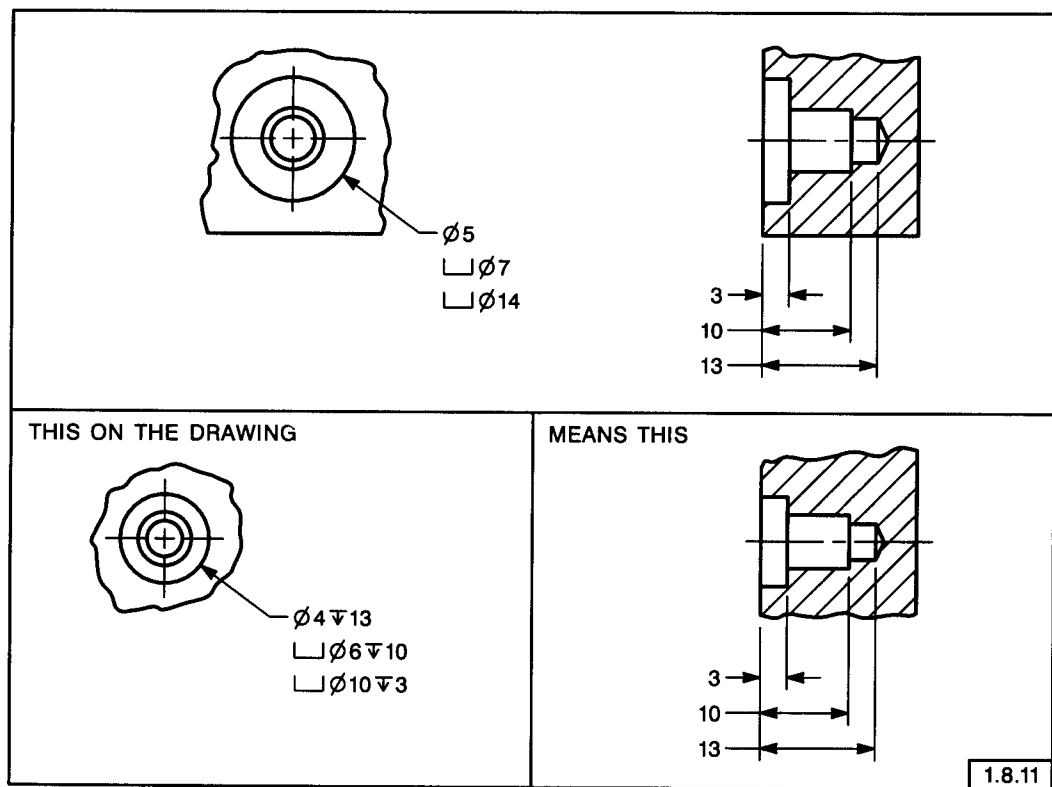
FIG. 1-37 COUNTERBORED HOLES
