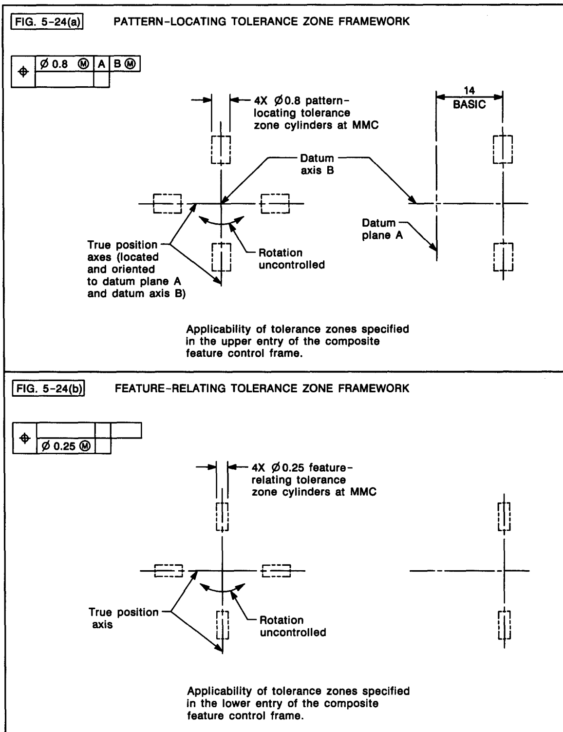
FIG. 5-24 RADIAL HOLE PATTERN LOCATED BY COMPOSITE POSITIONAL TOLERANCING (CONT'D) Tolerance Zones for Radial Hole Pattern
