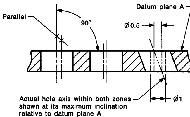
FIG. 5-22 COMPOSITE POSITIONAL TOLERANCING OF A CIRCULAR PATTERN OF FEATURES (CONT'D)
