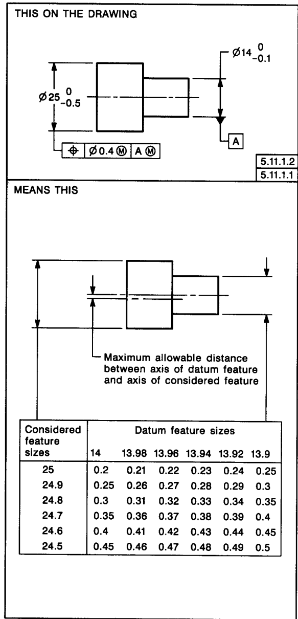
FIG. 5-48 POSITIONAL TOLERANCING FOR COAXIALITY
