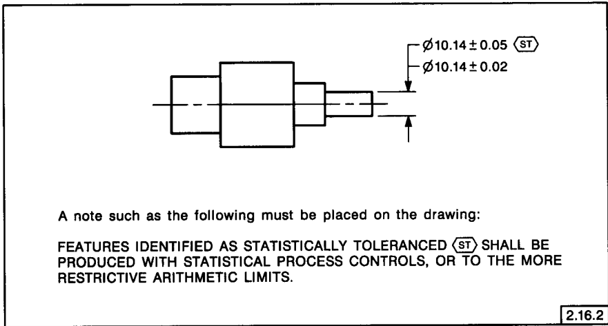
FIG. 2-21 STATISTICAL TOLERANCING WITH ARITHMETIC LIMITS
