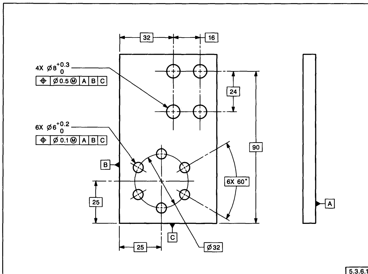
FIG. 5-16 MULTIPLE PATTERNS OF FEATURES
