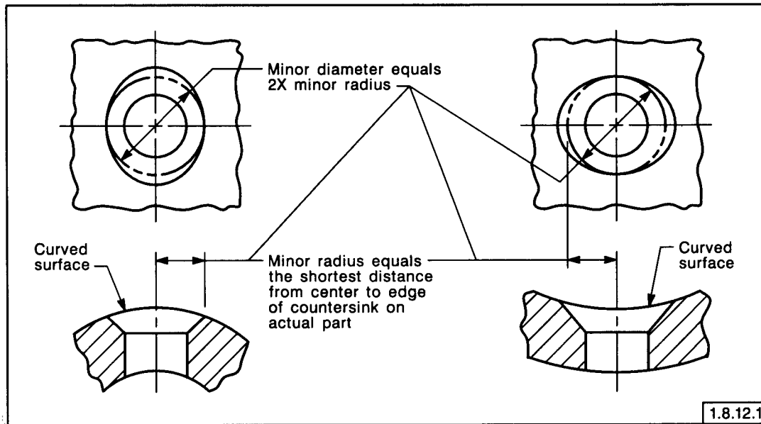
FIG. 1-39 COUNTERSINK ON A CURVED SURFACE
