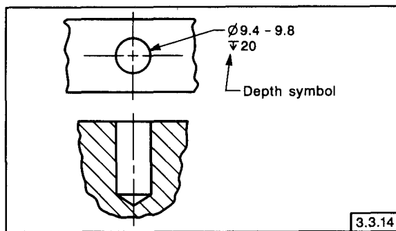
FIG. 3-14 DEPTH SYMBOL
