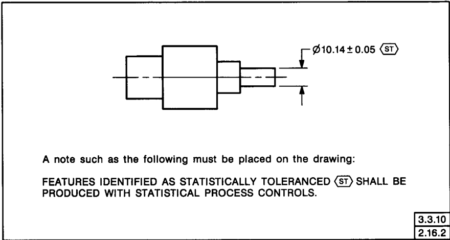
FIG. 2-20 STATISTICAL TOLERANCING
