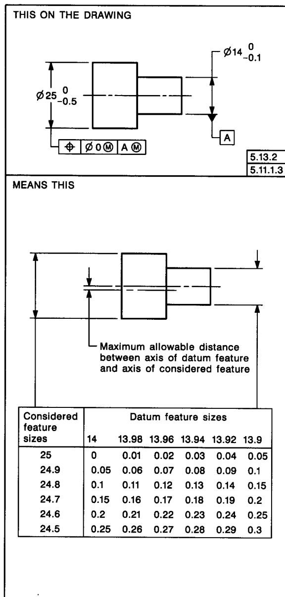
FIG. 5-50 ZERO POSITIONAL TOLERANCING AT MMC FOR COAXIALITY
