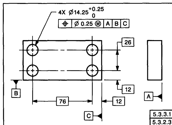
FIG. 5-9 CONVENTIONAL POSITIONAL TOLERANCING AT MMC
