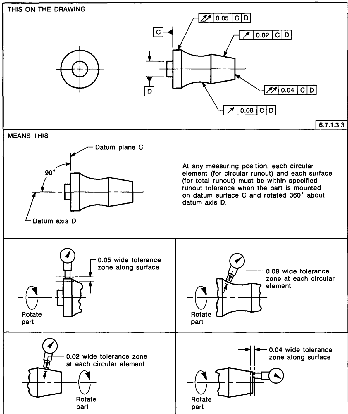
FIG. 6-50 SPECIFYING RUNOUT RELATIVE TO A DATUM SURFACE AND A DIAMETER
