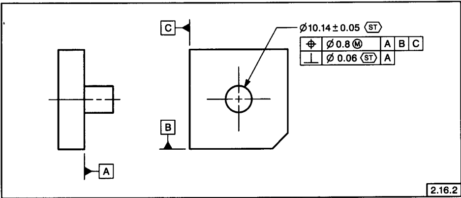
FIG. 2-22 STATISTICAL TOLERANCING WITH GEOMETRIC CONTROLS
