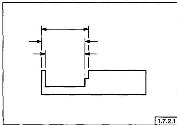
FIG. 1-9 BREAKS IN EXTENSION LINES
