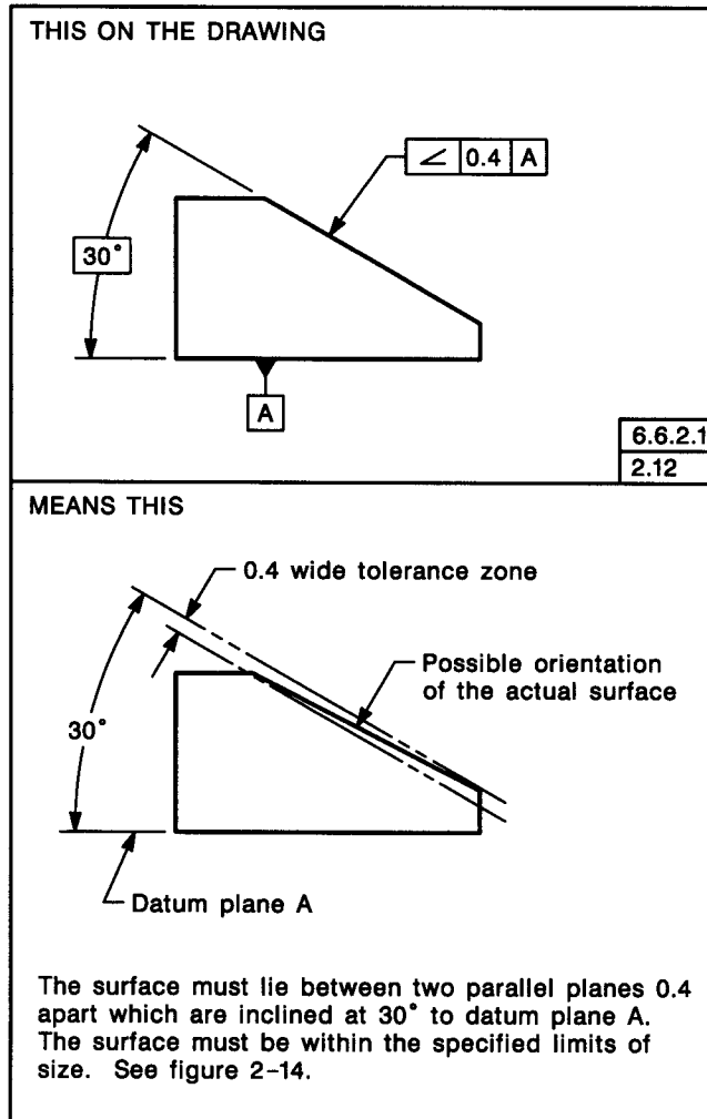
FIG. 6-27 SPECIFYING ANGULARITY FOR A PLANE SURFACE
