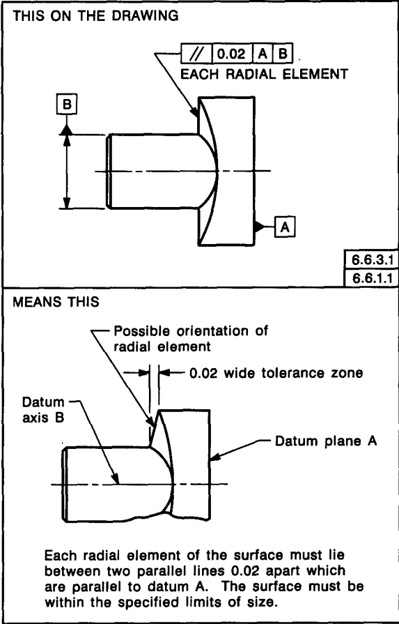
FIG. 6-45 SPECIFYING PARALLELISM FOR A RADIAL ELEMENT OF A SURFACE
