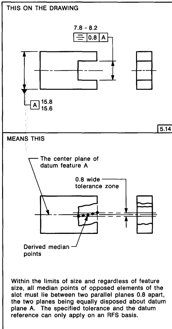
FIG. 5-61 SYMMETRY TOLERANCING
