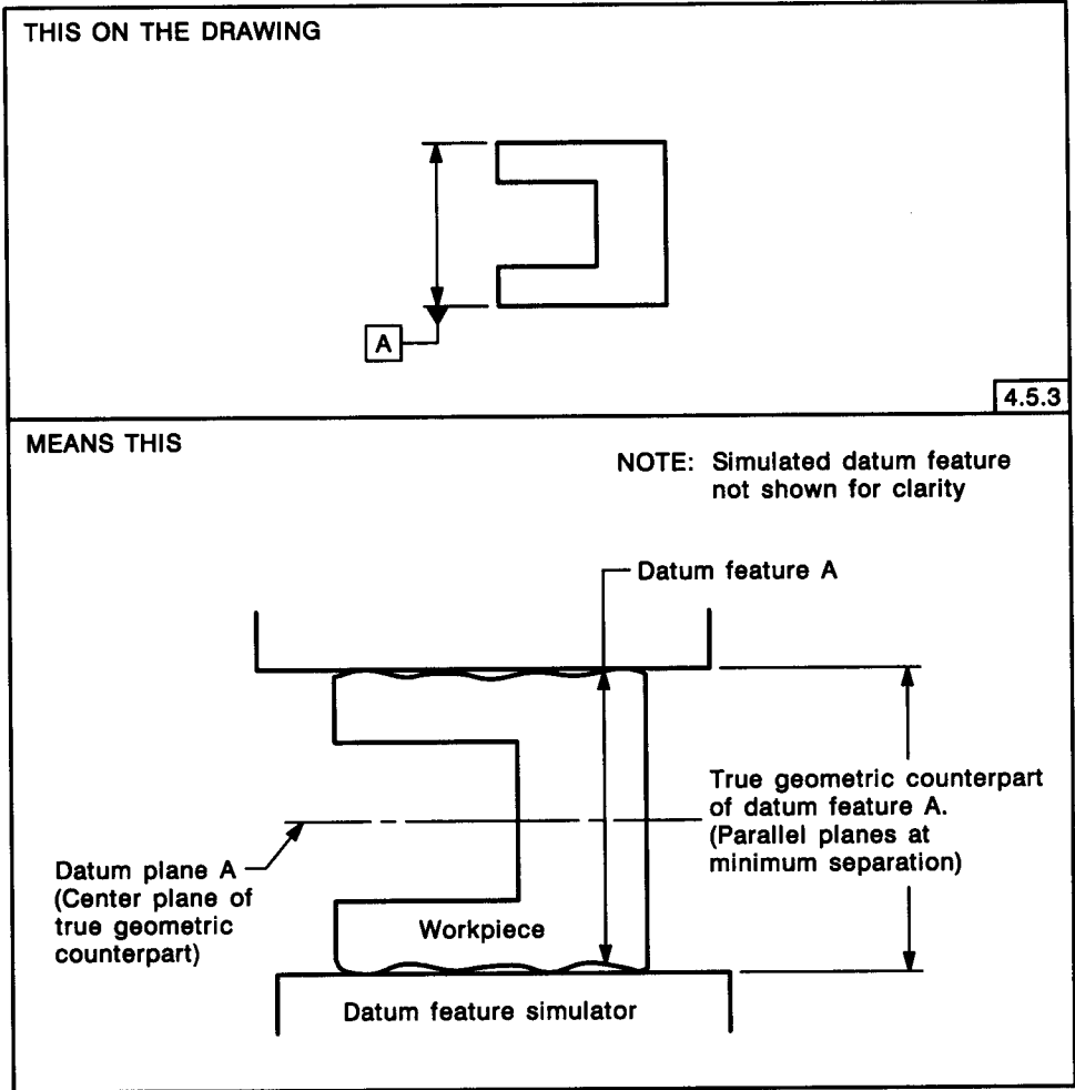
FIG. 4-13 PRIMARY EXTERNAL DATUM WIDTH — RFS
