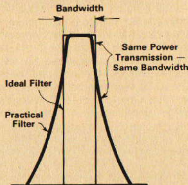
Effective Noise Bandwidth
