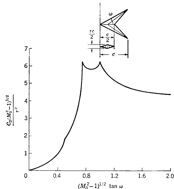
FIG. 9-14. Pressure drag at zero angle of attack for arrow wing on basis of supersonic wing theory.
