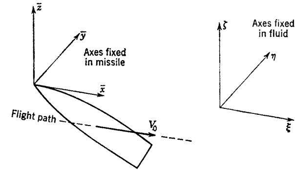
FIG. 2-1. Axes fixed in fluid and axes fixed in missile for uniform translation.
