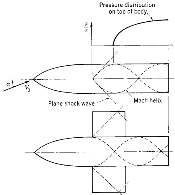
FIG. 9-37. Mach waves and helices due to rectangular wing panels of wing-body combination.
