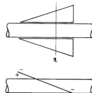
FIG. 8-24. Gaps associated with large deflections of all-movable controls.
