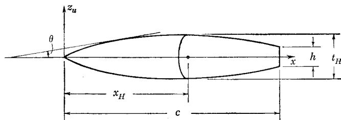
FIG. 8-25. Blunt trailing-edge control with symmetrical section.
