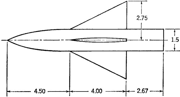
FIG. 5-16. Dimensions of model used in calculative example.
