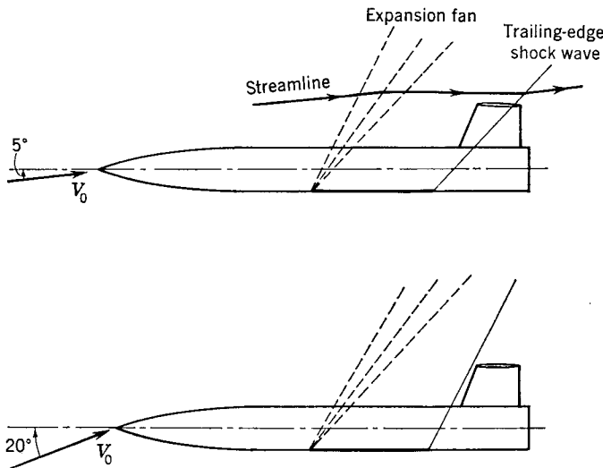
FIG. 7-15. Interference of wing shock-expansion field on tail.
