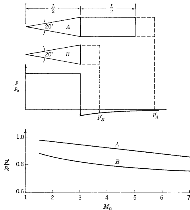
Fig. 9-27. Method of evaluating p' together with some specific values.
