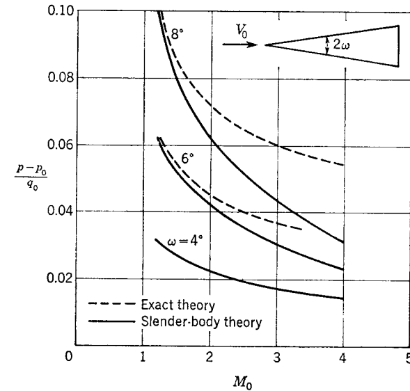
FIG. 4-4. Thickness pressure coefficients for circular cones.
