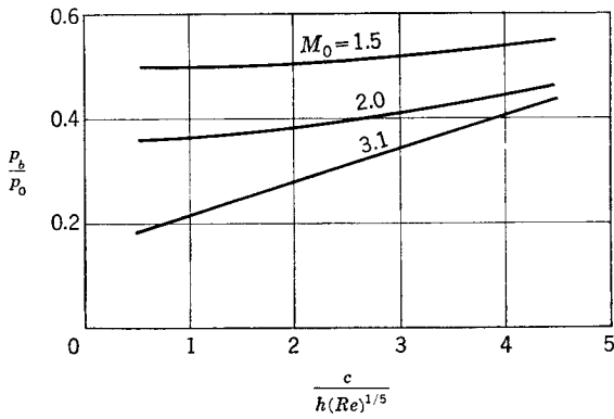
FIG. 9-29. Effect of Reynolds number on base pressure of airfoils with turbulent boundary layers.
