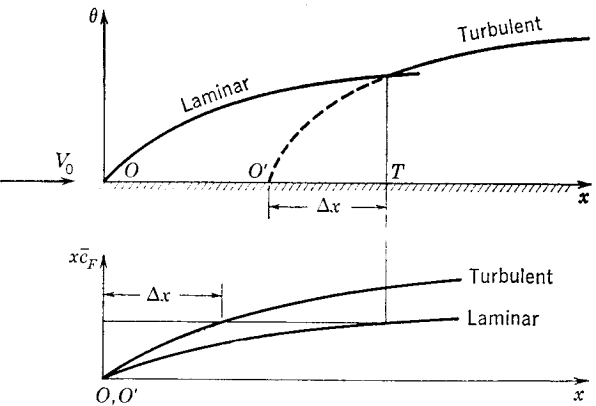
FIG. 9-38. Example illustrating method of locating virtual origin of turbulent boundary layer for transition on flat plate; narrow transition zone.
