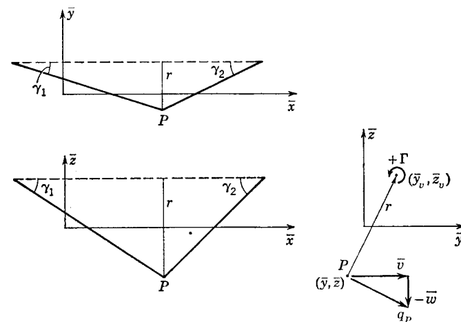
FIG. 6-8. Vortex line segment of Biot-Savart law.
