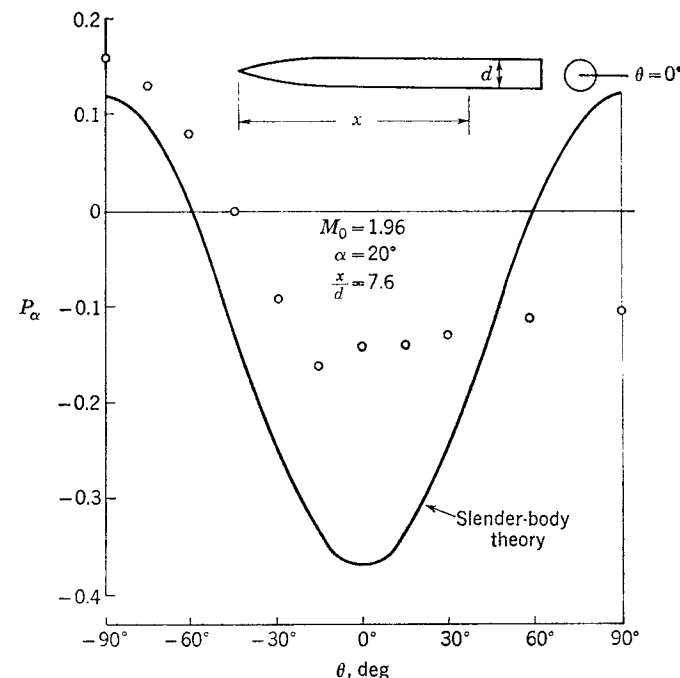
FIG. 4-13. Pressure distributions around body of revolution; comparison of theory and experiment.
