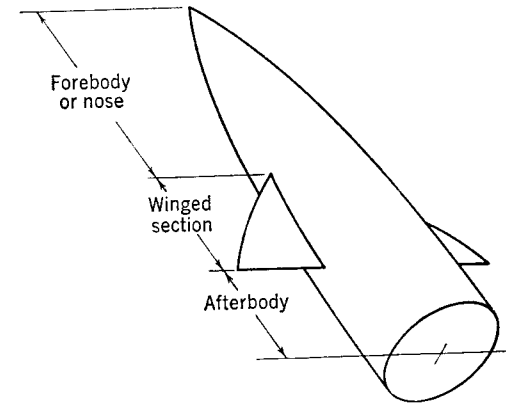
FIG. 5-1. Sections of wing-body combination.
