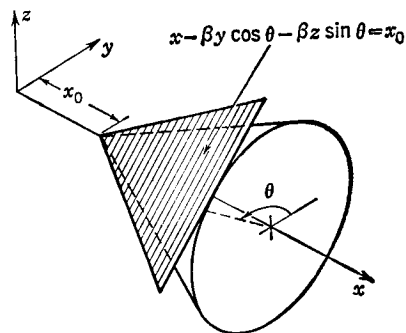
FIG. 9-19. Oblique tangent plane characterized by the parameters x_0 and \theta .
