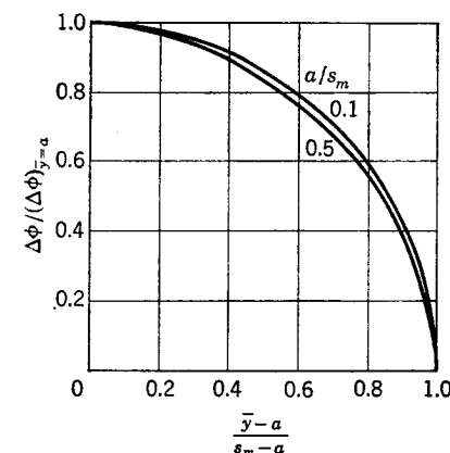
FIG. 6-12. Potential-difference distribution at trailing edge of wing in combination with body according to slender-body theory.
