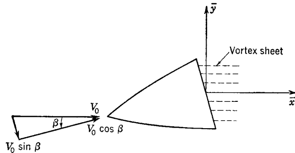
FIG. 6-4. Vortex system representing slender wing with sideslip.
