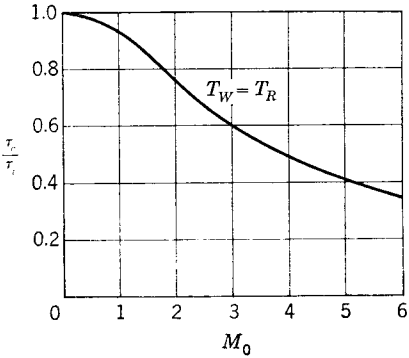
FIG. 9-35. Effect of Mach number on the local skin-friction coefficient of an insulated flat plate in air at room stagnation temperatures.
