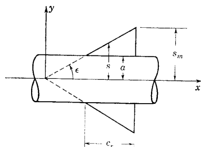
FIG. 5-5. Triangular wing and body combination.
