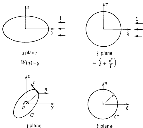
FIG. 10-11. Further notation for use in determination of apparent-mass coefficients.
