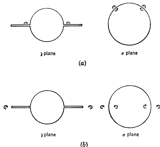
FIG. 7-17. Vortices in plane of tail panels. (a) Case 1, s_v < s ; (b) case 2, s_v > s .
