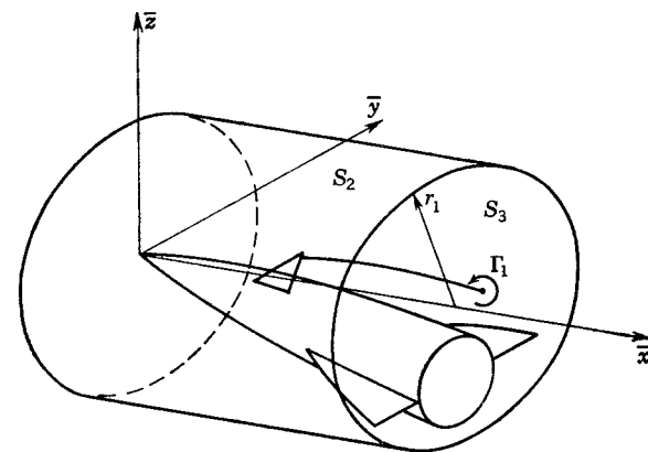
FIG. 4-22. Control areas for calculating forces and moments due to free vortices.
