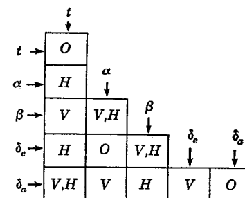
FIG. 8-14. Types of coupling between horizontal and vertical control panels.
