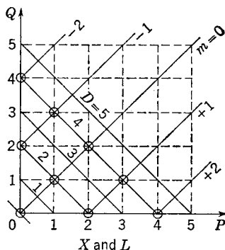
FIG. 10-31. PQ diagram for missile with 2-gonal and mirror symmetries.
