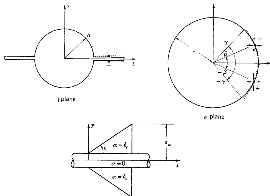
FIG. 8-5. Crossflow plane and transformed plane for pitch control of planar configuration.
