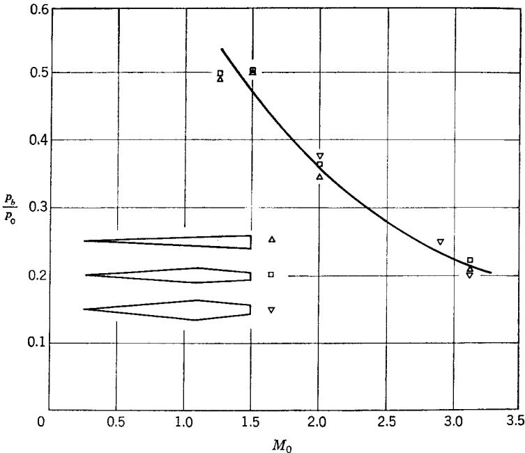
FIG. 9-28. Base-pressure correlation for airfoils with relatively thin turbulent boundary layers.
