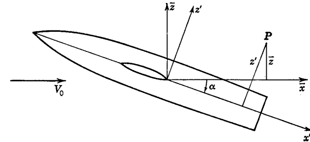
FIG. 6-15. Wind and body axes.
