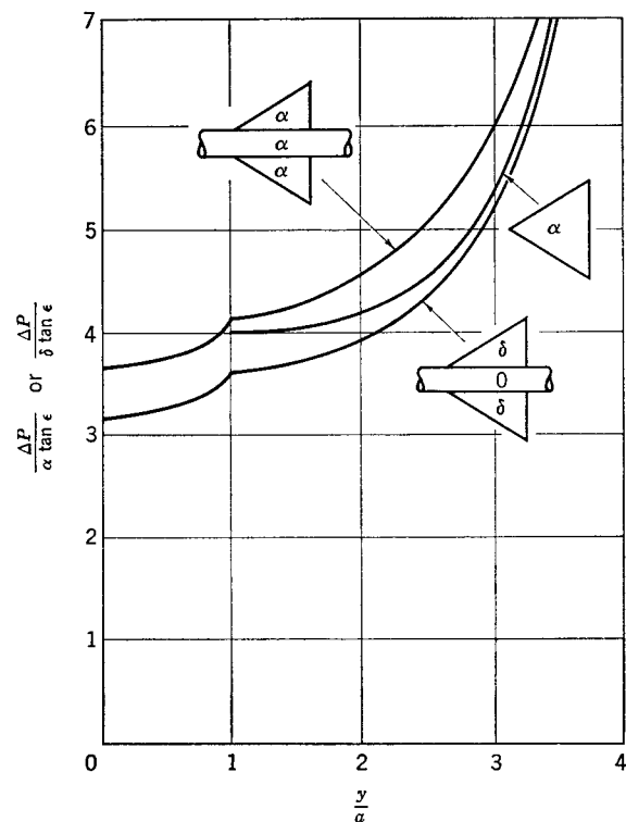
FIG. 8-7. Loading coefficient at trailing edge of various configurations employing triangular panels.
