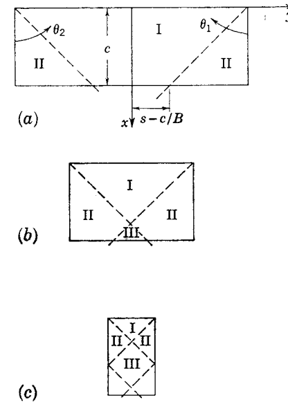
FIG. 2-8. Cases for rectangular wings. (a) Case 1, BA \geq 2 ; (b) case 2, 1 \leq BA \leq 2 ; (c) case 3, \frac{1}{2} \leq BA \leq 1 .
