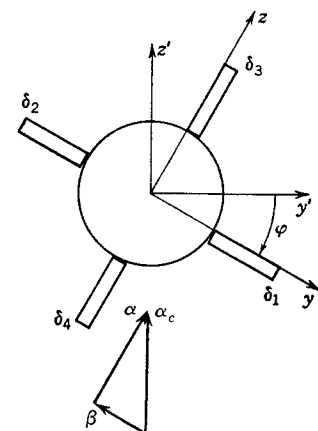
FIG. 8-10. Combined pitch and yaw control of cruciform configuration.
