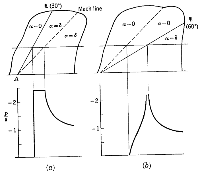
FIG. 8-18. Typical pressure distributions associated with flap-type controls utilizing (a) supersonic and (b) subsonic hinge lines for M_0^2 = 2 .
