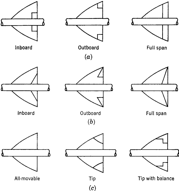
FIG. 8-17. Types of trailing-edge controls. (a) Constant chord; (b) constant taper; (c) others.
