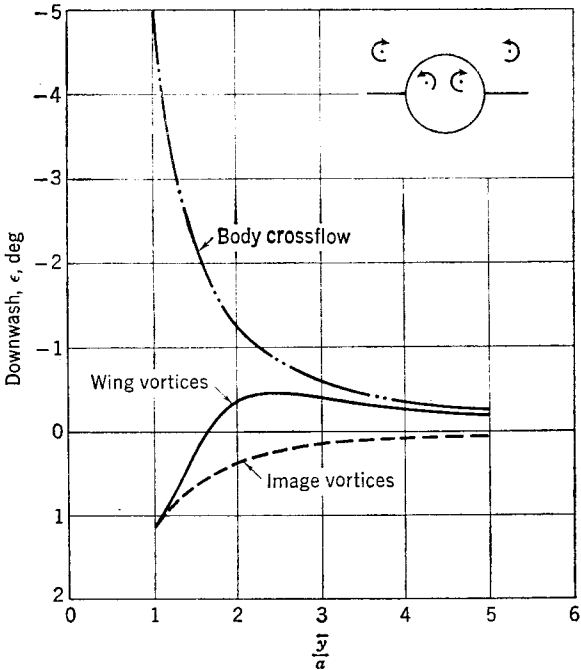
FIG. 6-22. Components of downwash on horizontal plane of symmetry 10 radii behind wing panel; A = \frac{2}{3} , M_0 = 2 , a/s_m = 0.6 .
