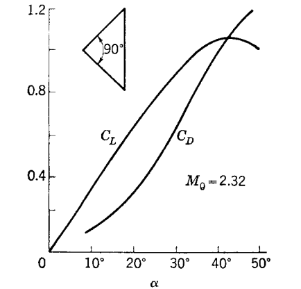
FIG. 8-28. Maximum lift characteristics of triangular wing at supersonic speed.
