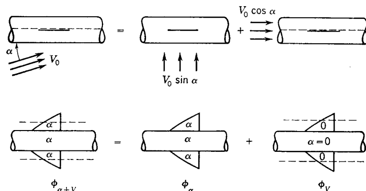
FIG. 7-3. Discrete line vortices intersecting tailplane.
