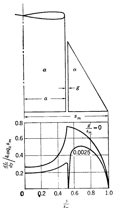
FIG. 8-23. Effect of gaps on span loading of wing-body combination; no viscosity.
