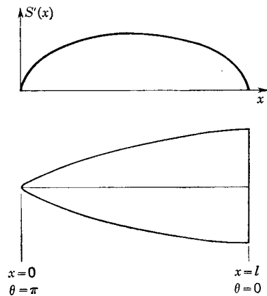
FIG. 9-10. Notation for use in minimizing pressure foredrag of slender bodies at zero angle of attack.
