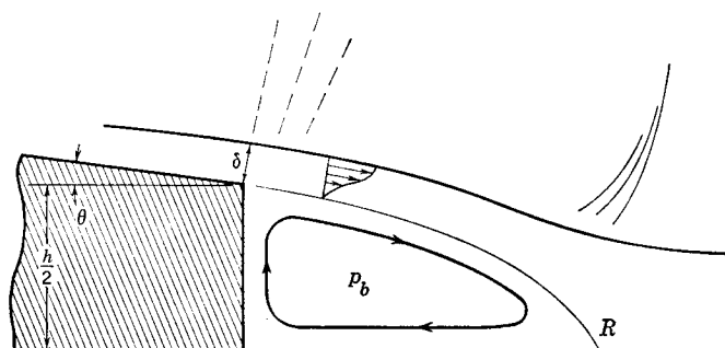
FIG. 9-26. Theoretical model of flow behind a blunt base.
