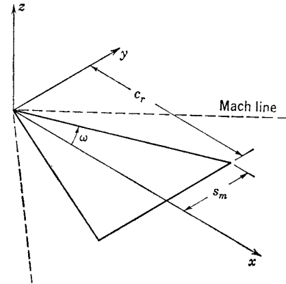
FIG. 2-6. Notation for triangular wings.
