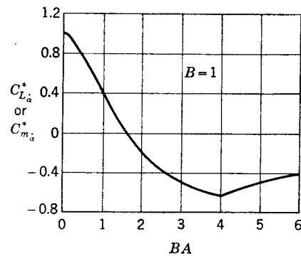
FIG. 10-21. Variation with aspect ratio of certain pitch damping derivatives of triangular wings.
