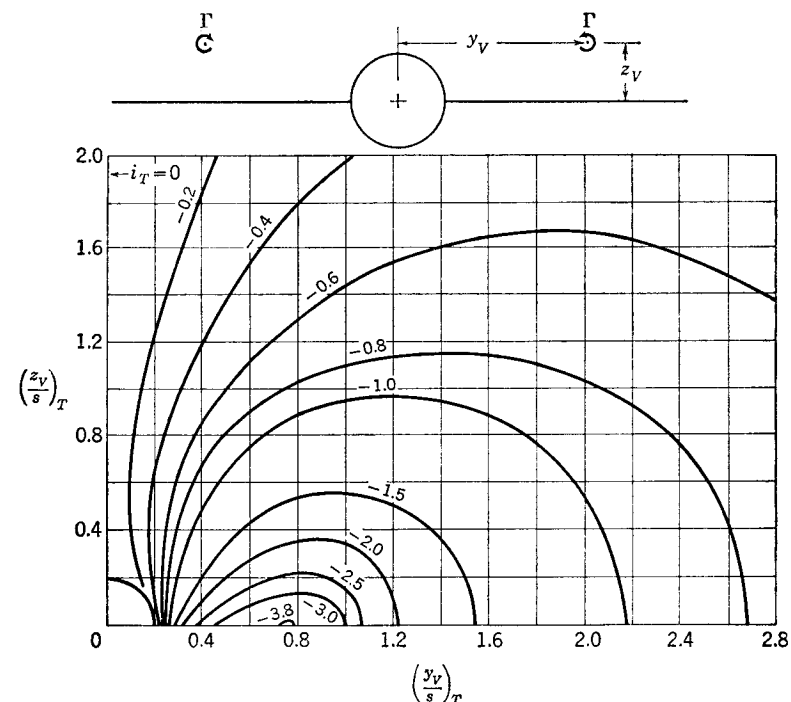
FIG. 7-8. Chart of tail interference factor based on strip theory; \lambda_T = 0 , (a/s)_T = 0.2 .
