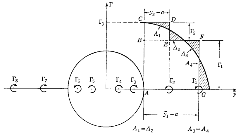
FIG. 6-14 Vortex model utilizing two external vortices per panel.
