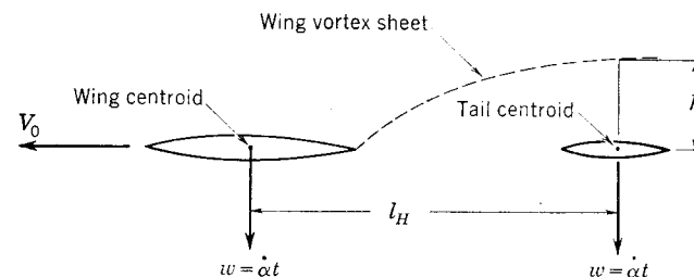
FIG. 10-26. Wing-tail combination in uniform \dot{\alpha} motion.
