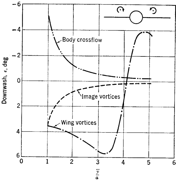
FIG. 6-23. Components of downwash on horizontal plane of symmetry 10 radii behind wing panel; A = \frac{2}{3} , M_0 = 2 , a/s_m = 0.2 .
