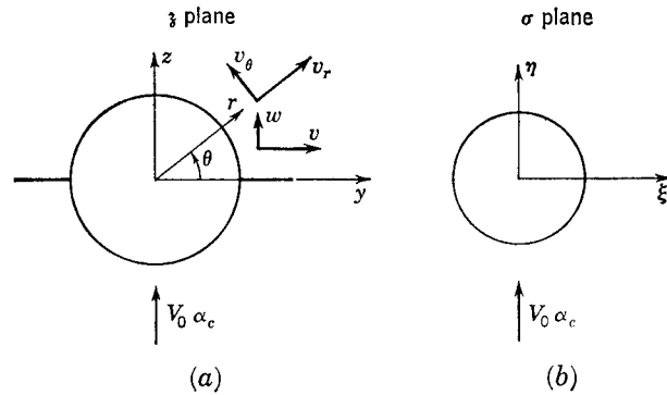
FIG. 2-11. Notation for (a) physical and (b) transformed planes.
