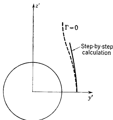
FIG. 6-19. Streamline and vortex path for crossflow past a circular cylinder.
