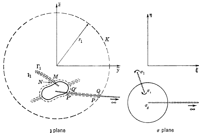
FIG. 4-23. Cuts and contours of integration.
