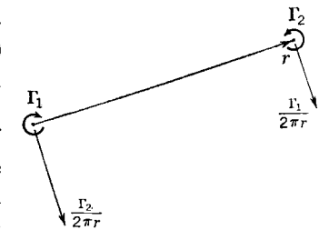
FIG. 6-5. Mutual induction between pair of two-dimensional vortices.
