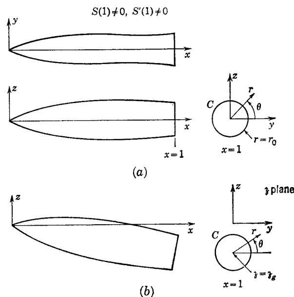
FIG. 9-5. Nonaxisymmetric slender body at zero angle of attack and at angle of attack; circular base. (a) \alpha = 0 ; (b) \alpha > 0 .
