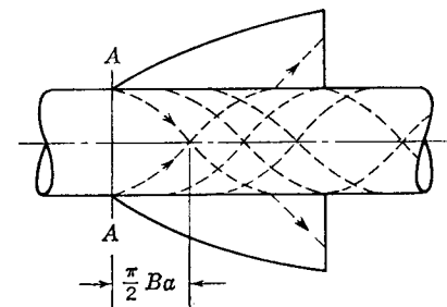
FIG. 5-11. Transference of lift from wing to body.
