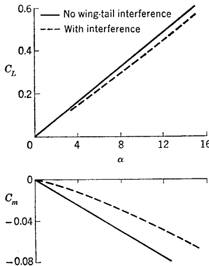
FIG. 7-10. Calculated lift and moment curves of example configuration.
