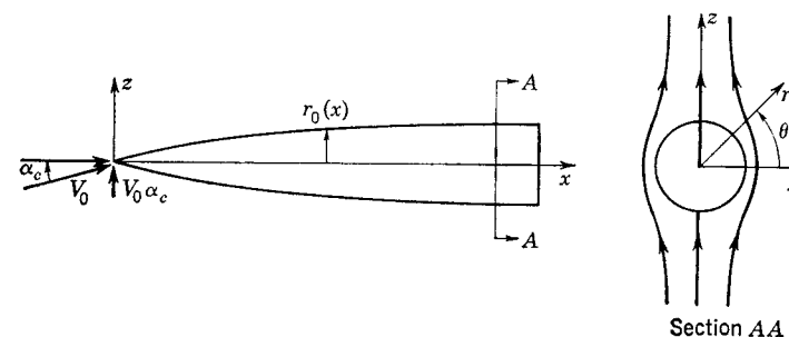
FIG. 3-3. Incompressible crossflow around body of revolution at angle of attack.
