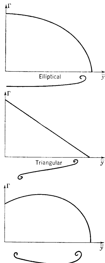
FIG. 6-21. Effect of circulation distribution on wake shape.
