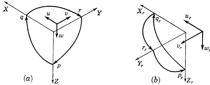
FIG. 10-29. Positive conventions involved in mirror symmetry (a) before and (b) after reflection.
