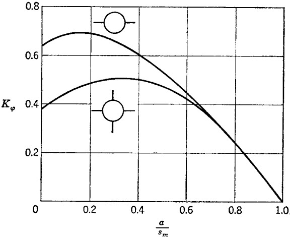
FIG. 5-8. Interference lift ratios for loading associated with bank angle.
