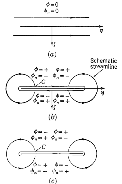
FIG. 10-9. Signs of potentials and their normal derivatives for various unit velocities. (a) Unit velocity along \eta , \phi_1 ; (b) unit velocity along \zeta , \phi_2 ; (c) unit rolling velocity, \phi_3 .
