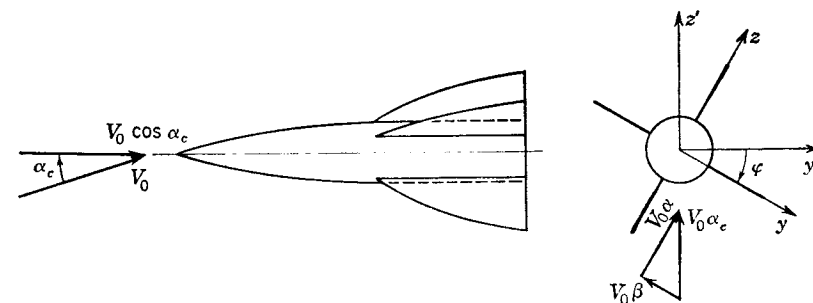
FIG. 8-13. Cruciform missile under combined pitch and bank.
