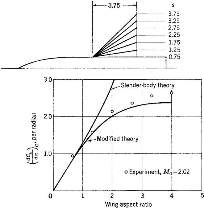
FIG. 5-15. Comparison of theory and experiment for triangular wing and body combinations.
