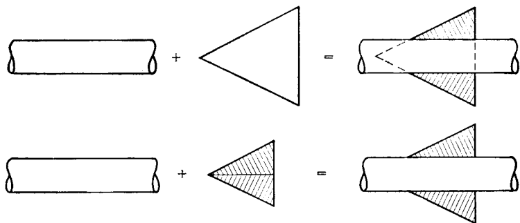
FIG. 9-15. Methods of superposing wing and body to form a wing-body combination.
