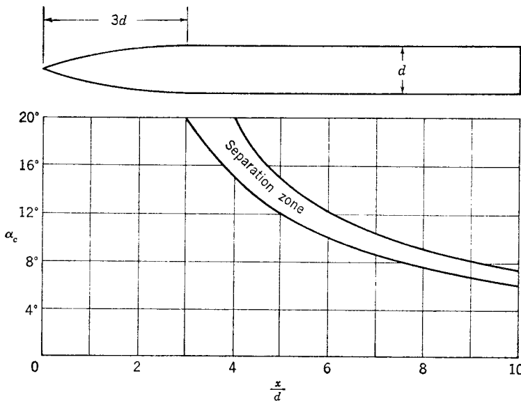
FIG. 4-15. Location of vortex separation for body of revolution.
