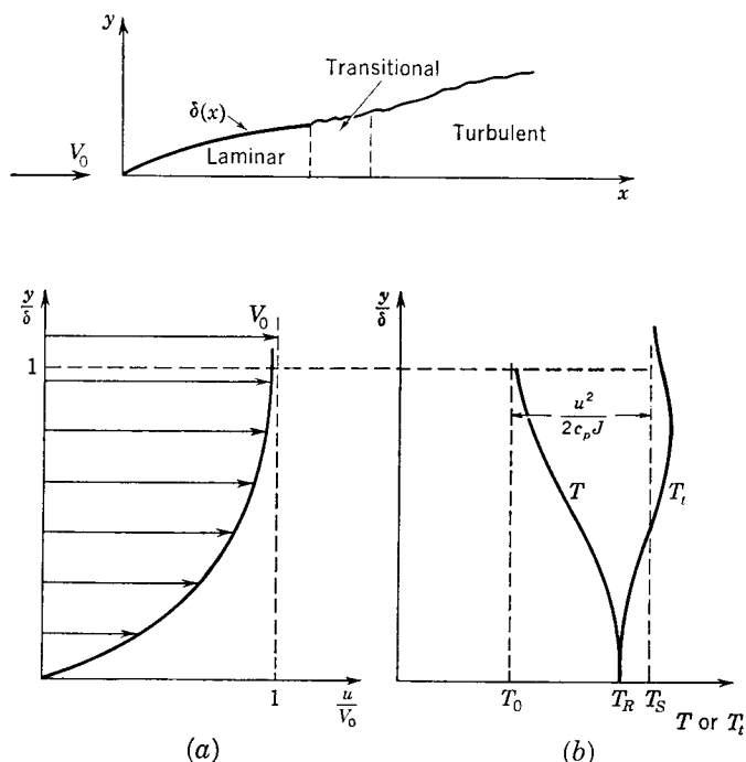
FIG. 9-33. (a) Velocity and (b) temperature profiles in high-speed boundary layer of insulated plate.
