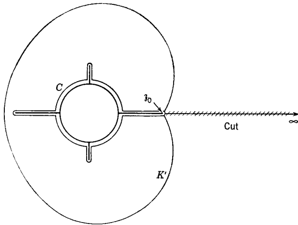
FIG. 3-9. Distortion of contour in cut z plane.
