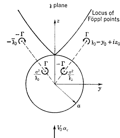
FIG. 4-19. Symmetrical vortex pair in presence of circular cylinder.
