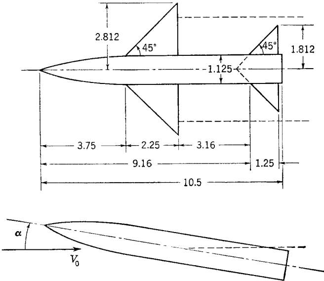
FIG. 7-9. Wing-body-tail combination of illustrative example.
