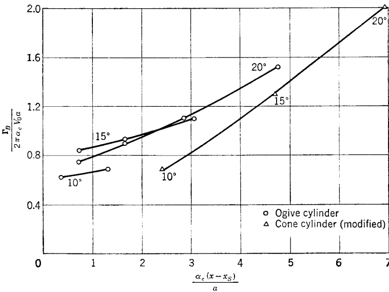
FIG. 4-16. Nondimensional vortex strengths for bodies of revolution.
