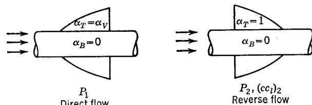
FIG. 7-14. Special configuration in direct and reverse flow.
