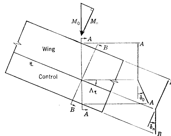
FIG. 8-22. Simple sweep theory for trailing-edge controls.
