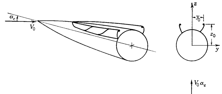
FIG. 4-14. Crossflow vortices of body of revolution.
