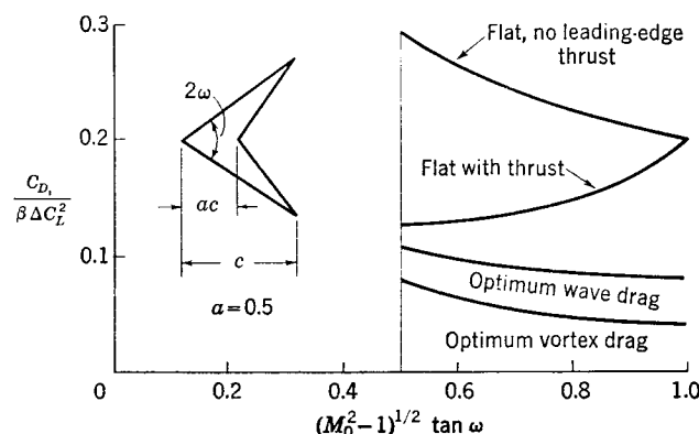
FIG. 9-25. Drag due to lift of arrow-shaped lifting surfaces.
