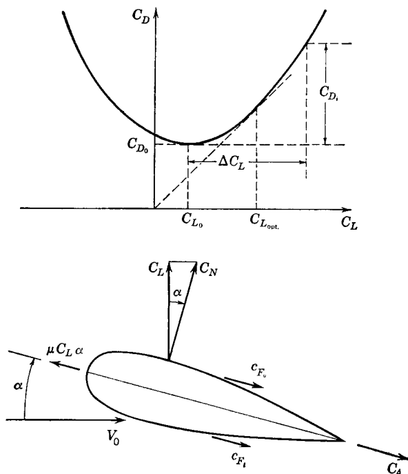
FIG. 9-3. Drag polar and forces acting on aerodynamic body.
