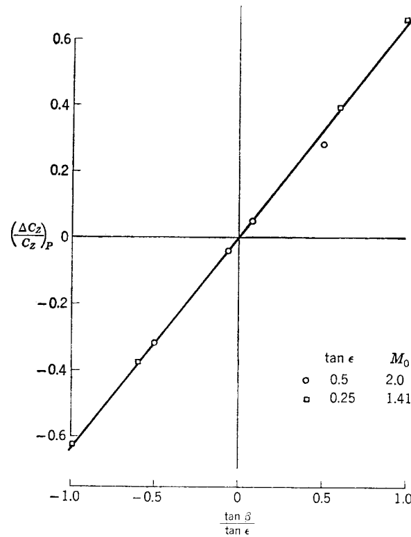
FIG. 5-10. Change in loading of panel of triangular wing due to sideslip.
