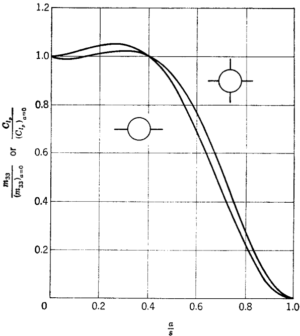
FIG. 10-16. Effect of body radius on damping in roll for fixed span.
