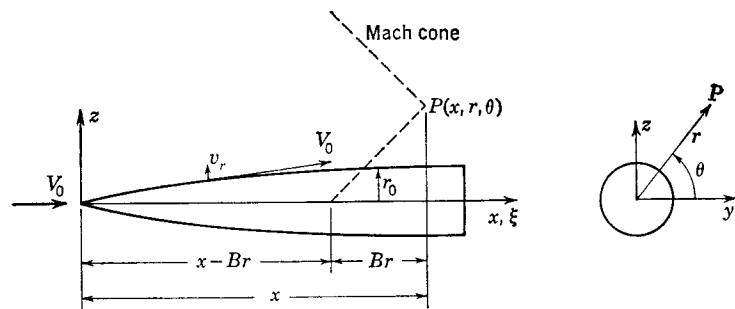
FIG. 3-1. Axes and notation for body of revolution at zero incidence.
