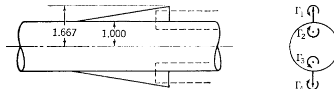
FIG. 6-16. Configuration of example calculation.
