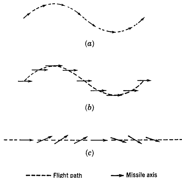
FIG. 10-20. Types of sinusoidal pitching motions. (a) \dot{\alpha} = 0 , q = \theta = \sin \omega t ; (b) \dot{\alpha} = \sin \omega t , q = \theta = 0 ; (c) q = \dot{\alpha} = \sin \omega t .
