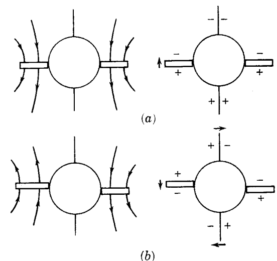
FIG. 8-11. Induced flow and direction of panel forces due to (a) pitch control and (b) roll control of horizontal control panels.
