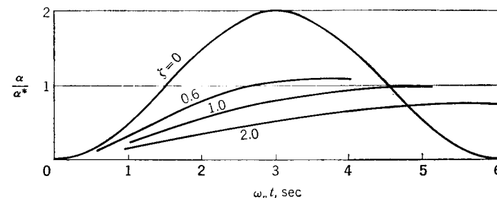
FIG. 8-30. Change in attitude of missile due to sudden application of pitch control.
