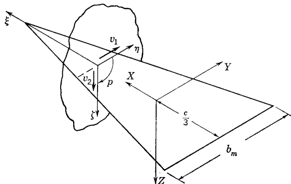
FIG. 10-8. Axes and notation for slender triangular wing.
