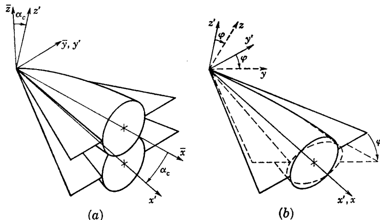
FIG. 1-2. Axis conventions for pitch and bank. (a) Pitch about \bar{y} ; (b) bank about \bar{x} .
