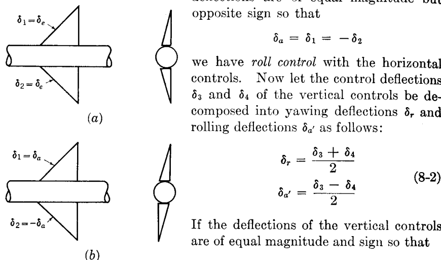
FIG. 8-3. (a) Pitch control and (b) roll control with horizontal controls.
