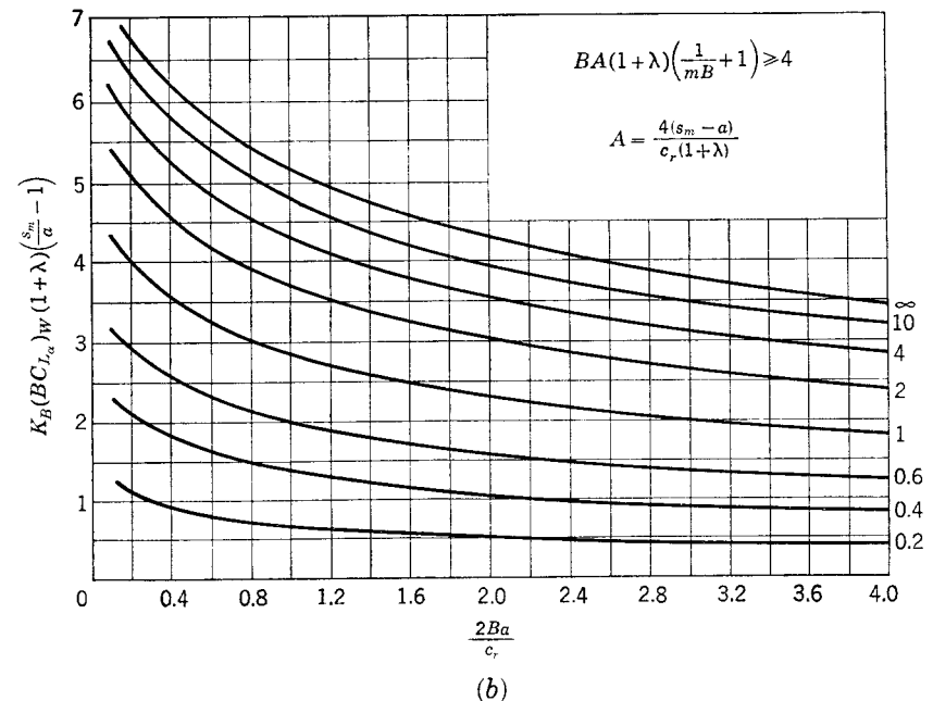
FIG. 5-13. Values of K_B based on planar model. (a) No afterbody; (b) afterbody
