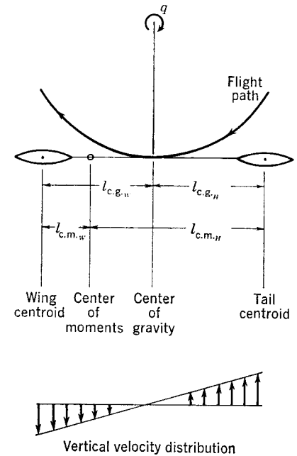
FIG. 10-25. Wing-tail combination in uniform q motion.
