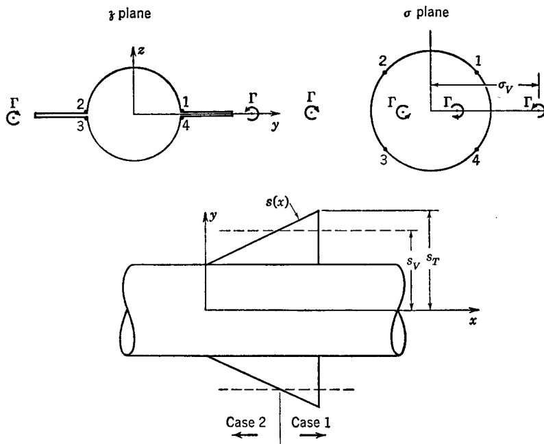
FIG. 7-4. Transformation of tail cross section into unit circle.
