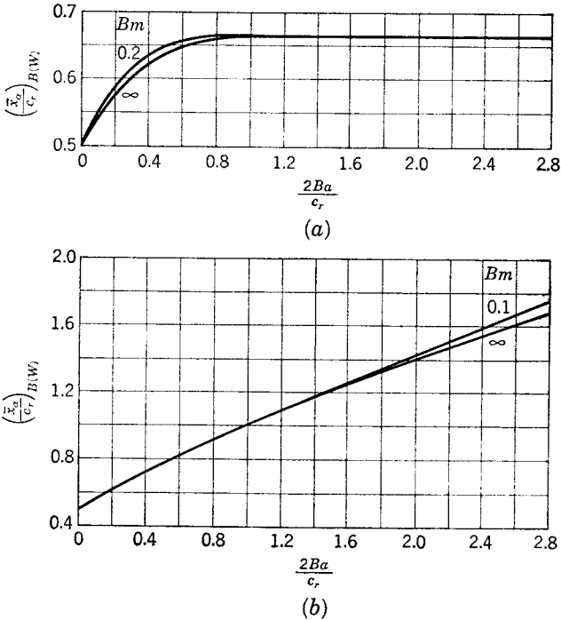
FIG. 5-14. Values of (\bar{x}_c/c_r)_{B(W)} based on planar model. (a) No afterbody; (b) afterbody.
