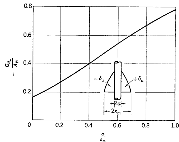
Fig. 8-9. Rolling effectiveness of planar all-movable controls.
