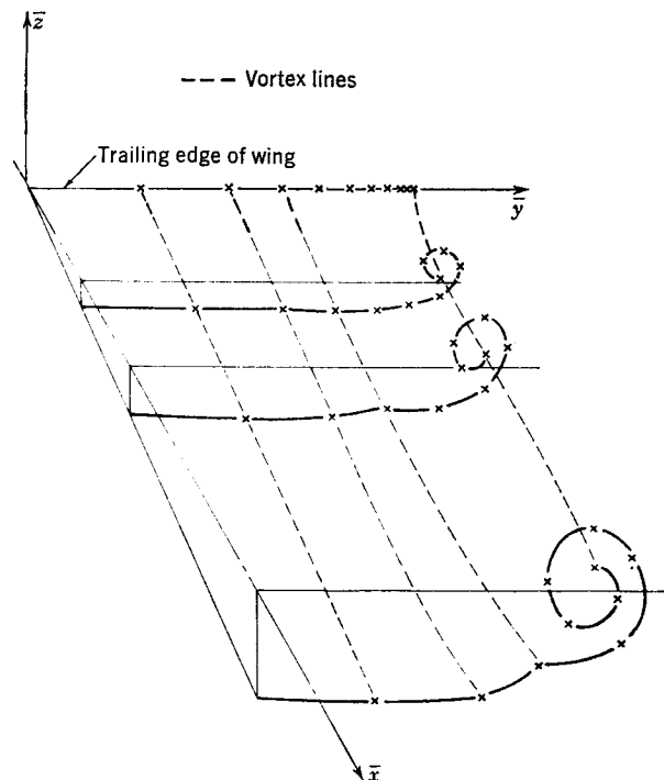
FIG. 6-6. Shape of vortex sheet associated with elliptical potential distribution according to Westwater.
