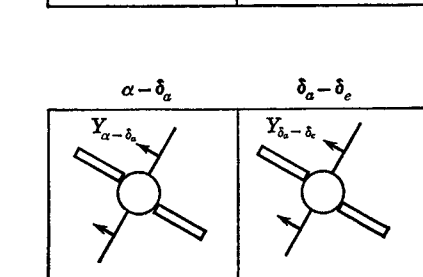
FIG. 8-16. Qualitative effects of coupling on panel forces for roll control.
