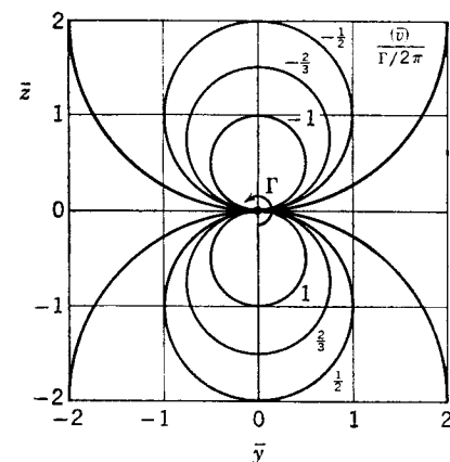
FIG. 6-9. Contours of constant downwash and sidewash associated with infinite line vortex in streamwise direction.
