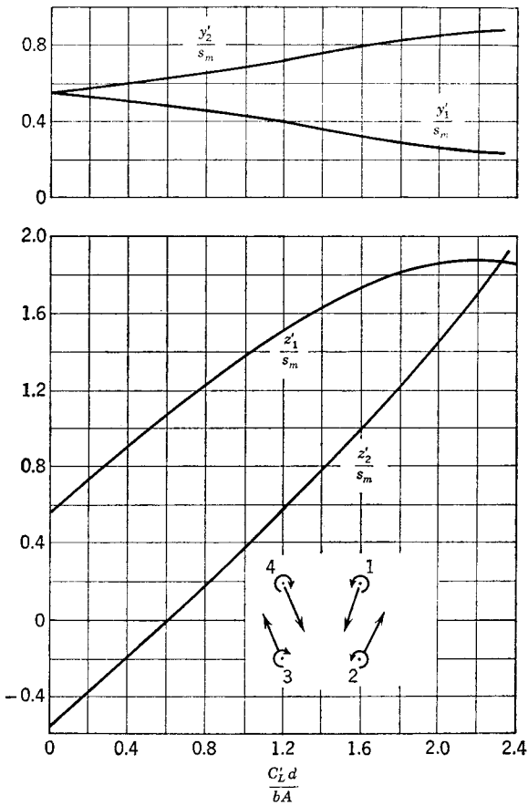
FIG. 6-26. Vortex positions behind panels of cruciform wing; \varphi = 45^\circ .
