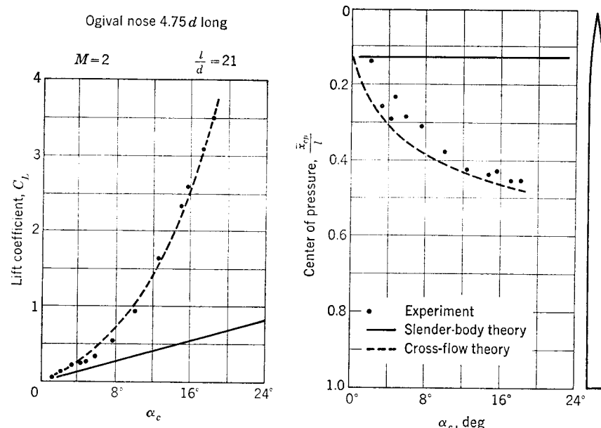
Fig. 4-18. Comparison of measured and predicted body aerodynamic characteristics.
