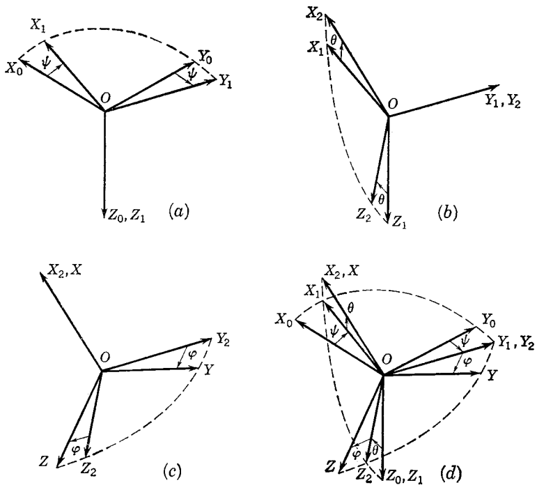
FIG. 10-2. System of angular displacements. (a) Yaw about OZ_0 by \psi ; (b) pitch about OY_1 by \theta ; (c) roll about OX_2 by \phi ; (d) composite diagram.
