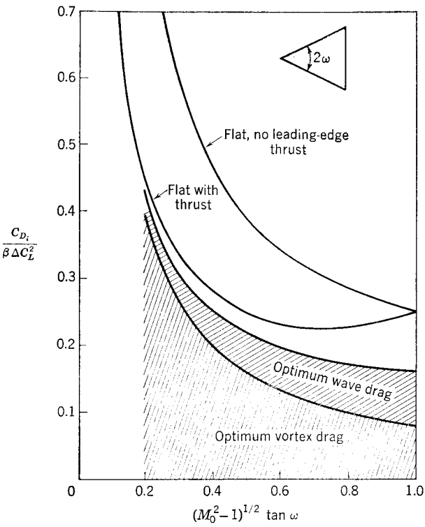
FIG. 9-23. Drag due to lift for triangular lifting surfaces.
