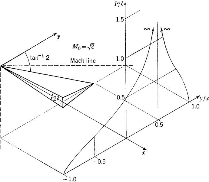
FIG. 2-4. Thickness pressure distribution on infinite wedge with subsonic leading edge.
