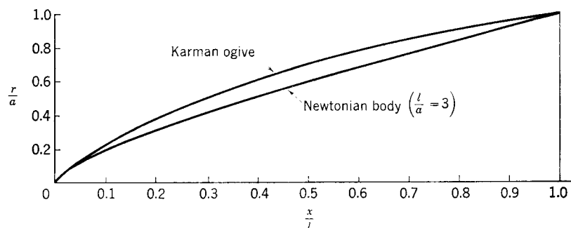
FIG. 9-11. Comparison of shape of Kármán ogive with that of Newtonian body of least pressure foredrag.
