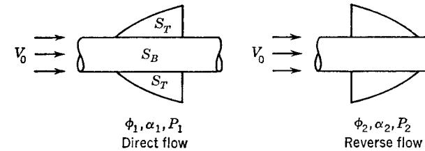
FIG. 7-12. Configuration in direct and reverse flow.
