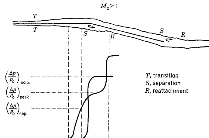
FIG. 8-26. Separation of supersonic turbulent boundary layer on trailing-edge control
