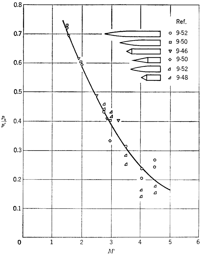
FIG. 9-30. Base-pressure correlation for bodies of revolution with relatively thin turbulent boundary layers.
