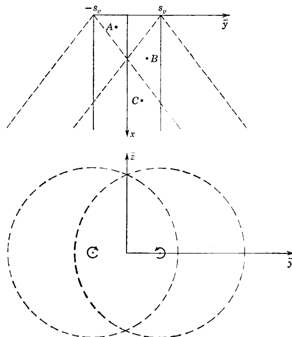
FIG. 6-10. Regions of influence of supersonic horseshoe vortex.
