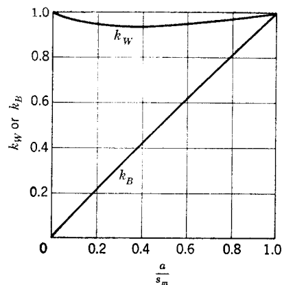
Fig. 8-6. Lift ratios for symmetrical deflection of all-movable panels on circular cylindrical body.
