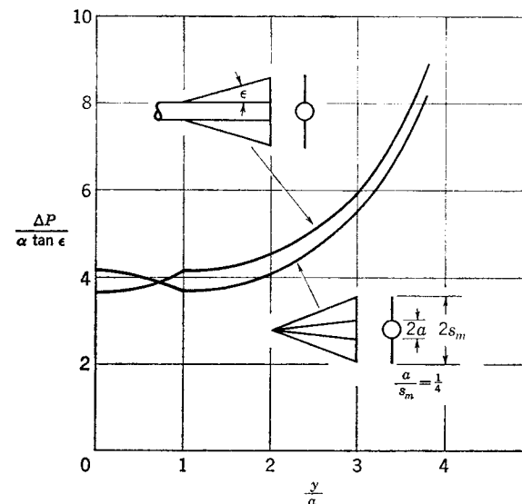
FIG. 5-4. Pressure differences at trailing edges of slender wing-body combinations.
