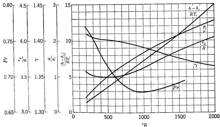
FIG. 9-34. Variation with temperature of certain physical constants for air.
