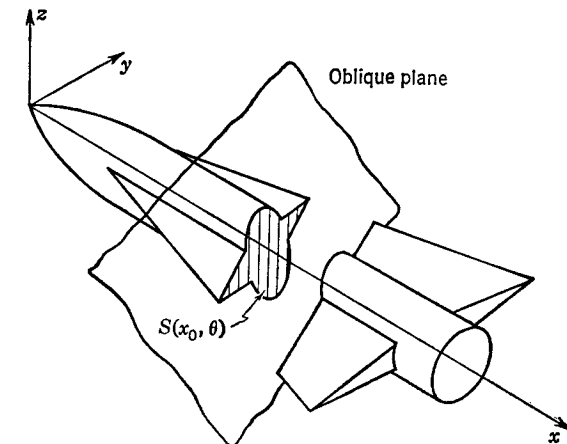
FIG. 9-20. Oblique cutting planes as used in the supersonic area rule.
