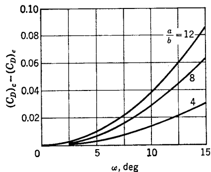
FIG. 4-9. Wave drag of circular cones versus elliptical cones.
