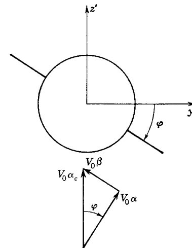
FIG. 6-17. Angle of attack and angle of sideslip components of crossflow velocity.
