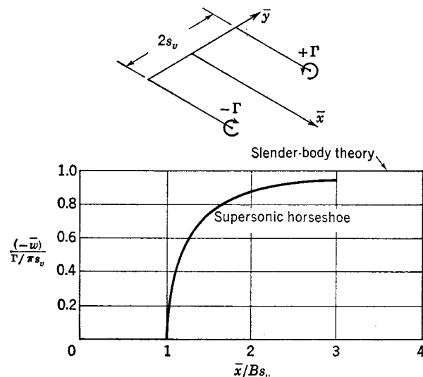
FIG. 6-11. Comparison of downwash calculated by supersonic horseshoe-vortex theory and slender-body theory.
