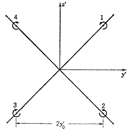
FIG. 6-25. Initial vortex positions for cruciform wing; \varphi = 45^\circ .
