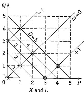
FIG. 10-30. PQ diagram for triform missile.
