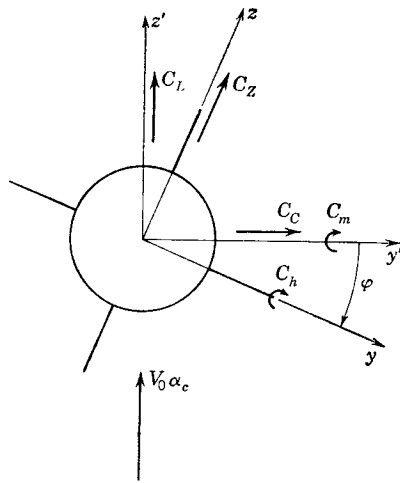
FIG. 5-2. Force and moment coefficients for panels and complete configuration.
