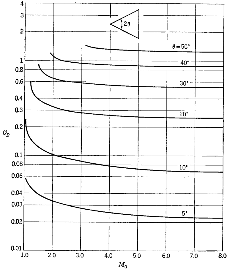
FIG. 9-6. Drag coefficients of cones at supersonic speeds.
