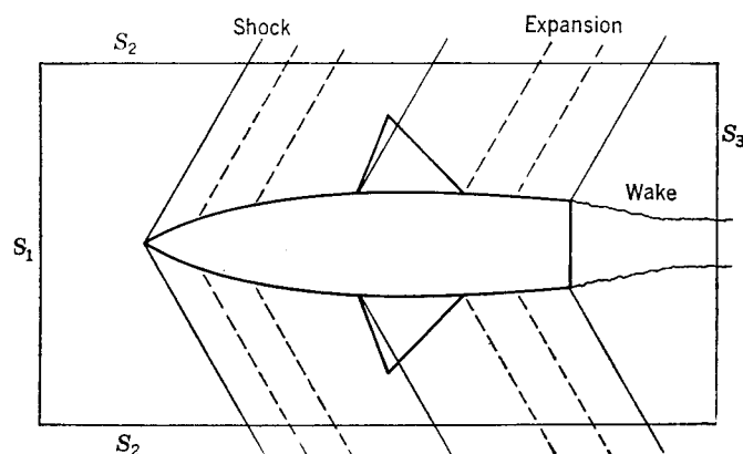
FIG. 9-2. Missile at supersonic speeds enclosed by cylindrical control surface.
