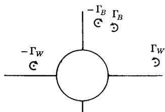
FIG. 10-24. Body and wing vortices in vicinity of empennage for combined pitch and sideslip.
