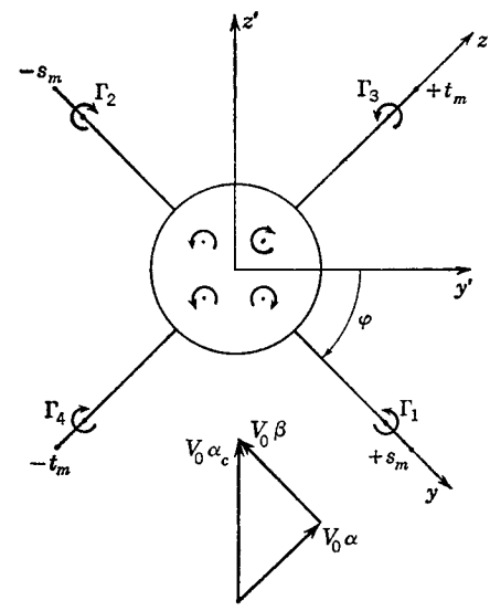
FIG. 6-24. Vortex model of cruciform wing-body arrangement.
