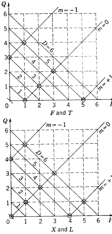
FIG. 10-28. PQ diagrams for cruciform missile.
