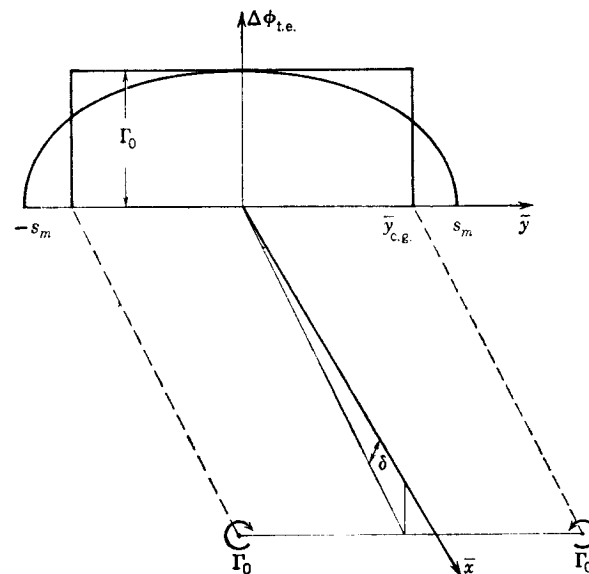
FIG. 6-7. Horseshoe vortex representing elliptical potential distribution.
