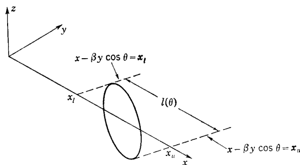
FIG. 9-22. Method of determining l(\theta) .
