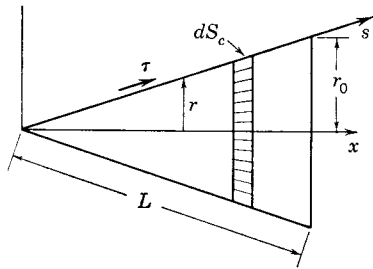
FIG. 9-39. Notation for evaluating laminar skin friction on cone.
