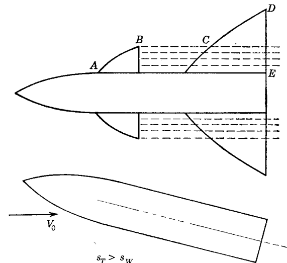
FIG. 7-1. Flat vortex sheet intersecting tailplane.
