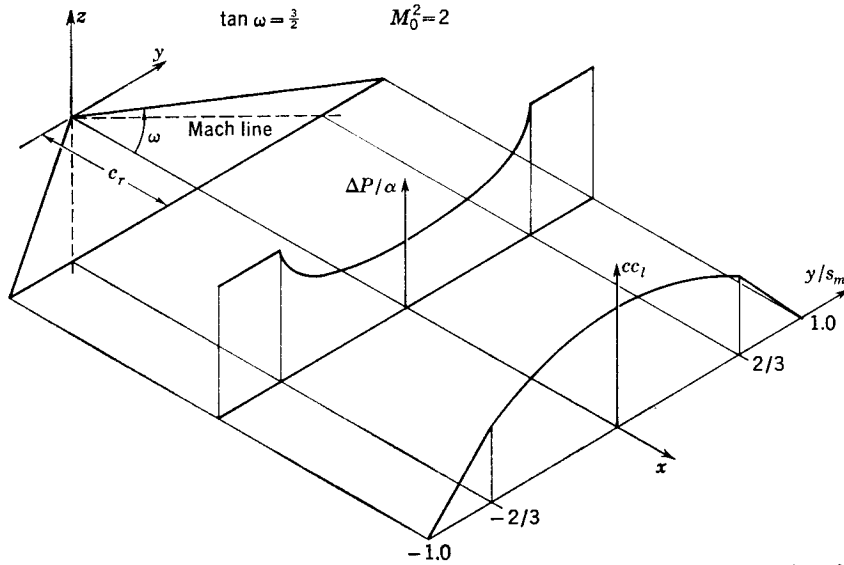
FIG. 2-7. Loading distribution along trailing edge, and span-load distribution for triangular wing with supersonic leading edges.
