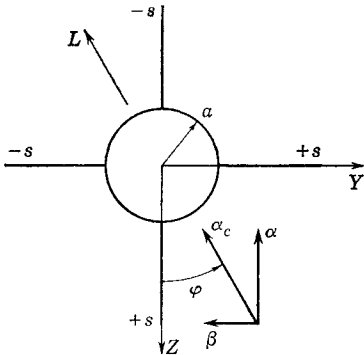
FIG. 10-15. Crossflow plane at wing trailing edges of slender cruciform missile.
