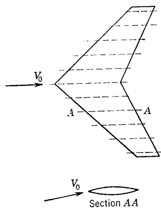
Fig. 2-2. Strip theory.
