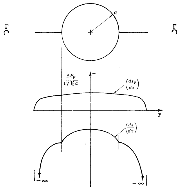
FIG. 7-5. Types of loadings associated with discrete vortices in plane of tail.
