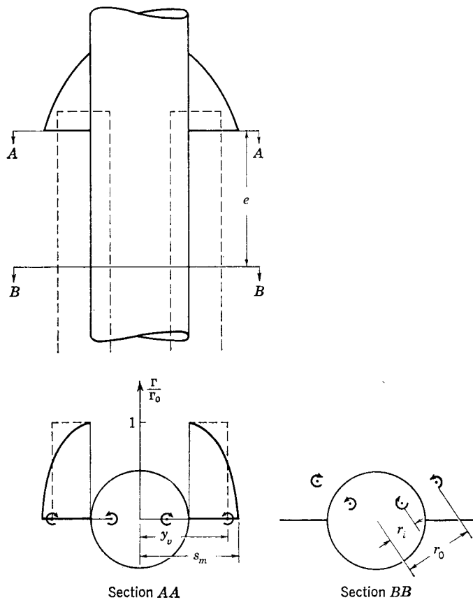
FIG. 5-17. Simplified vortex model of slender wing-body combination.
