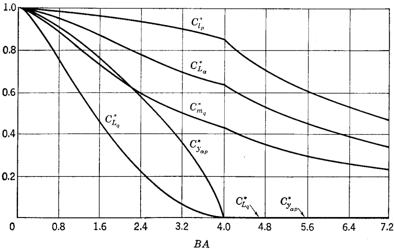
FIG. 10-17. Effect of aspect ratio on stability derivatives of triangular wing.
