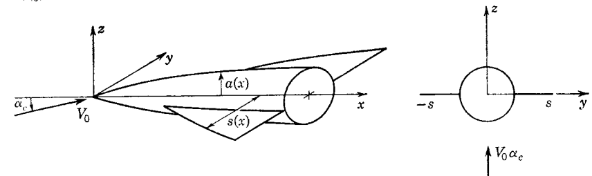
FIG. 5-3. Planar wing and body combination at zero angle of bank.
