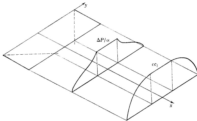
FIG. 2-9. Loading distribution at trailing edge, and span-load distribution for rectangular wing.
