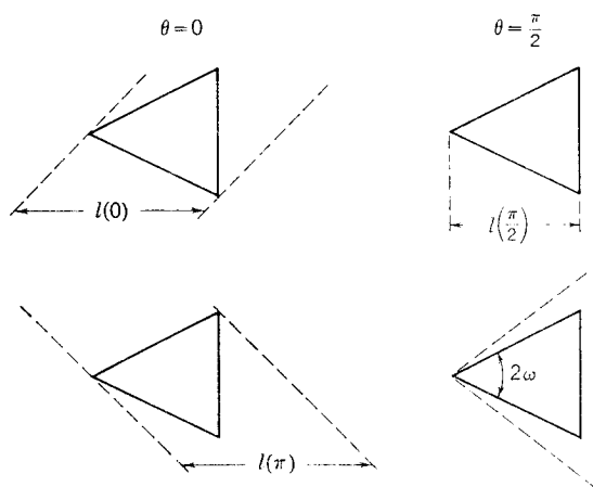
FIG. 9-24. Values of l(\theta) for triangular wings.
