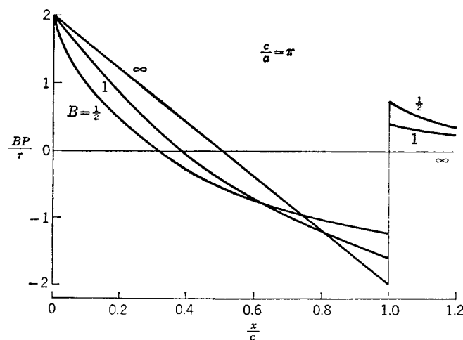
FIG. 4-12. Pressure distribution on circular cylinder with axially symmetric bump.
