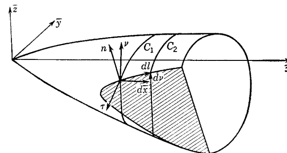
FIG. 3-6. Boundary conditions in streamwise plane through slender body.
