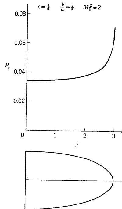
FIG. 4-7. Thickness pressure distribution for elliptical cone.
