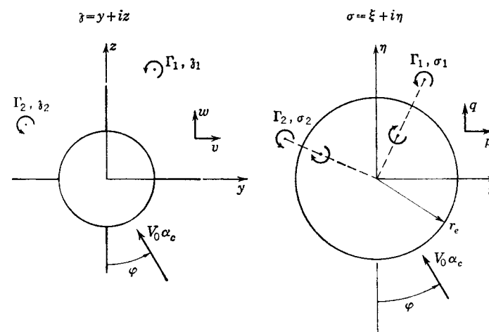
FIG. 4-21. Transformation of missile cross section into circle.
