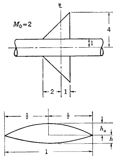
FIG. 8-29. Calculative example for hinge-moment coefficient.
