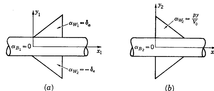
FIG. 8-8. Direct and reverse flows for calculating rolling effectiveness of planar configurations. (a) Case 1; (b) case 2.
