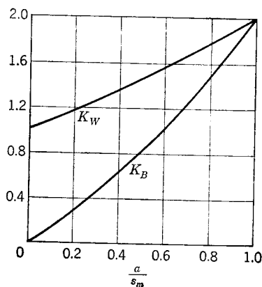
FIG. 5-6. Interference lift ratios for lift associated with pitch.
