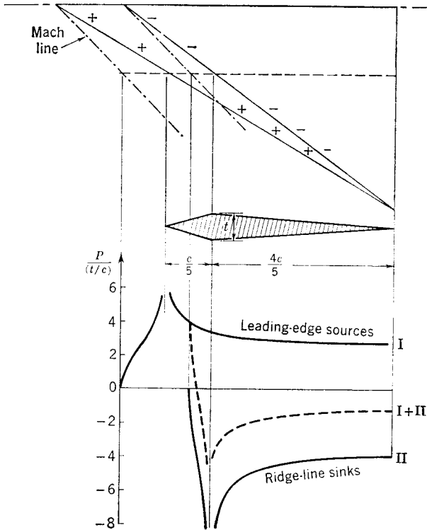
FIG. 9-36. Pressure distribution due to thickness on double-wedge triangular wing with subsonic ridge line.
