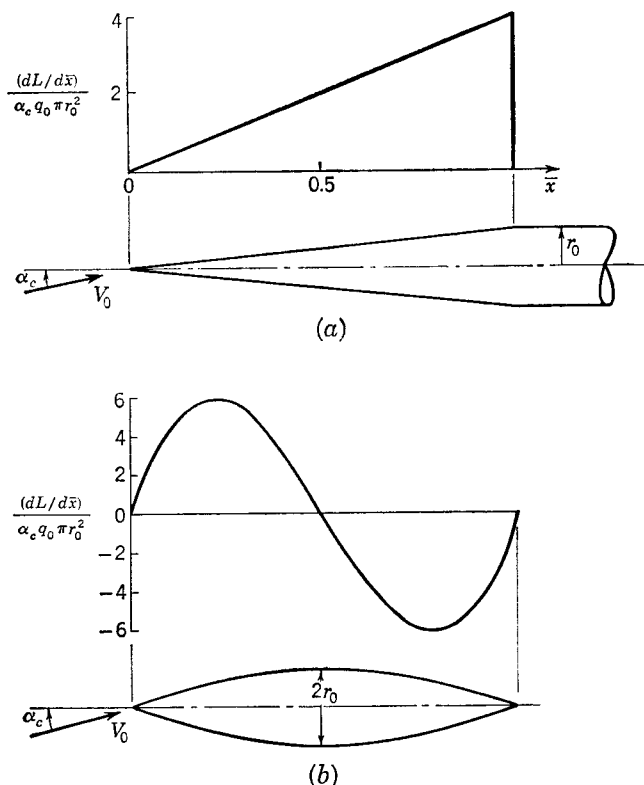
FIG. 4-1. Lift distributions for slender bodies of revolution. (a) Cone-cylinder; (b) parabolic body.
