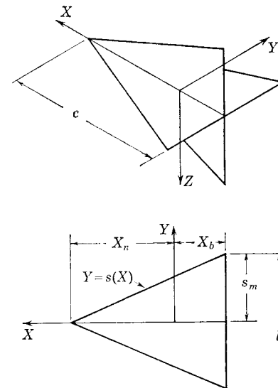
FIG. 10-12. Slender cruciform wing.
