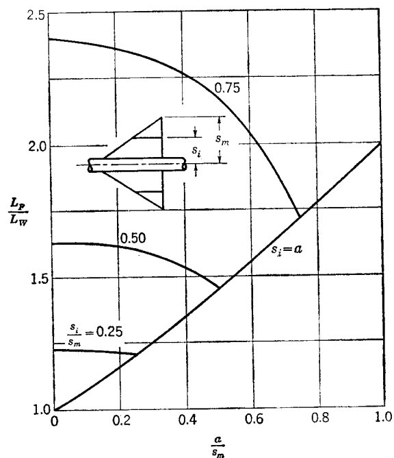
FIG. 8-21. Lift effectiveness of all-movable tip controls with unswept trailing edges.
