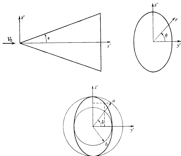
FIG. 4-6. Elliptical cone at zero angle of attack.
