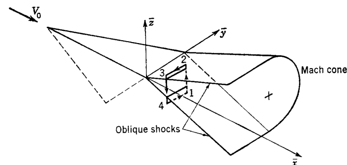
FIG. 6-3. Circulation contour with trailing shock waves.
