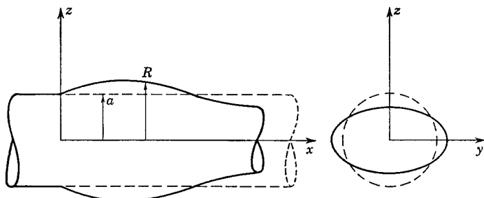
FIG. 4-10. Axes and notation for quasi-cylindrical bodies.
