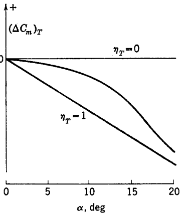
FIG. 7-16. Tail pitching-moment contribution with shock-expansion interference.
