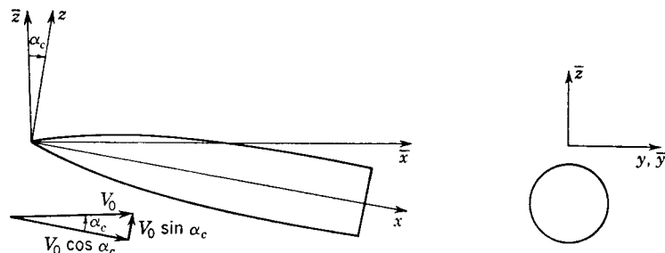
FIG. 4-3. Axis conventions.
