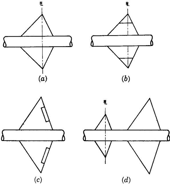
FIG. 8-1. Common types of missile controls. (a) All-movable; (b) all-movable tip; (c) trailing edge; (d) canard.
