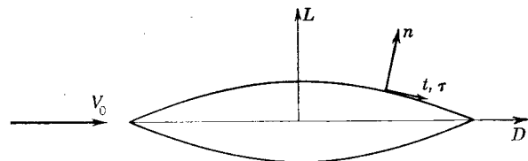
FIG. 9-1. Aerodynamic body subject to normal and tangential stresses.
