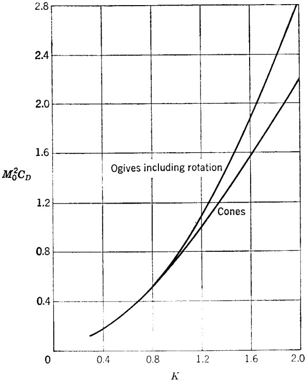
FIG. 9-8. Correlation curves for drag of cones and tangent ogives on basis of hypersonic similarity parameter.
