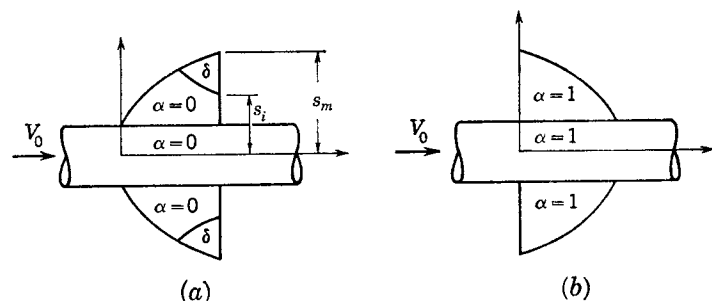
FIG. 8-20. Direct and reverse flows for calculating lift effectiveness of all-movable tip controls. (a) Case 1; (b) case 2.
