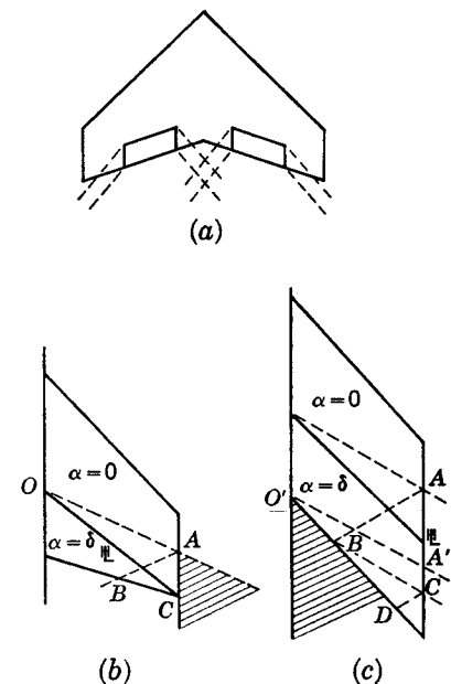
FIG. 8-19. Some cases encountered in using the lift-cancellation technique. (a) No lift cancellation; (b) tip sector; (c) trailing-edge sector.
