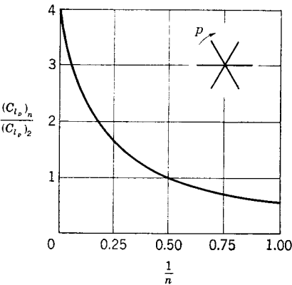
FIG. 10-14. Effect of number of fins on damping in roll.
