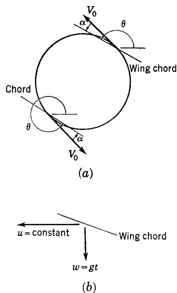
FIG. 10-19. Types of uniform motion involved in damping in pitch. (a) \dot{\alpha} = 0 , q = \text{constant} ; (b) q = 0 , \dot{\alpha} = \text{constant} .
