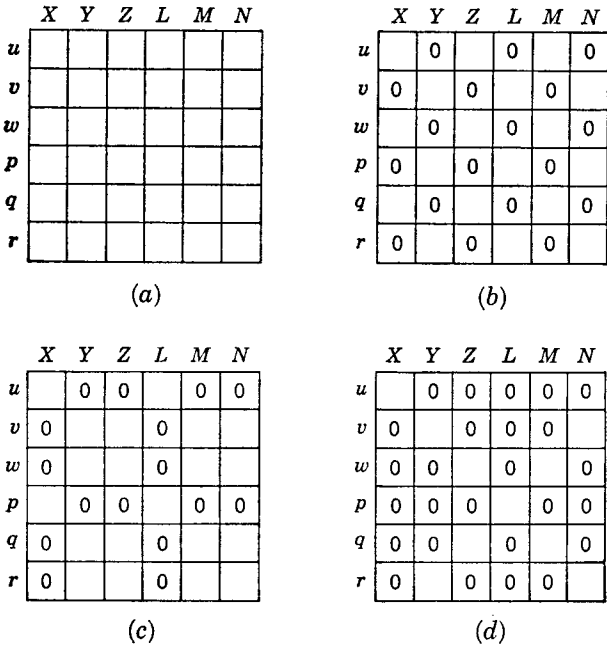
FIG. 10-5. Zero stability derivatives for missile with 2-gonal and mirror symmetries. (a) Case 1: u \neq 0, w \neq 0, p \neq 0, v = q = r = 0 ; (b) case 2: u \neq 0, w \neq 0, p = 0, v = q = r = 0 ; (c) case 3: u \neq 0, w = 0, p \neq 0, v = q = r = 0 ; (d) case 4: u \neq 0, w = 0, p = 0, v = q = r = 0 .
