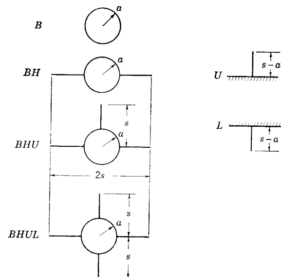
FIG. 10-27. Components in build-up of cruciform empennage.
