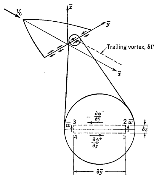
FIG. 6-1. Wind axes and sidewash at the trailing edge of the wing.
