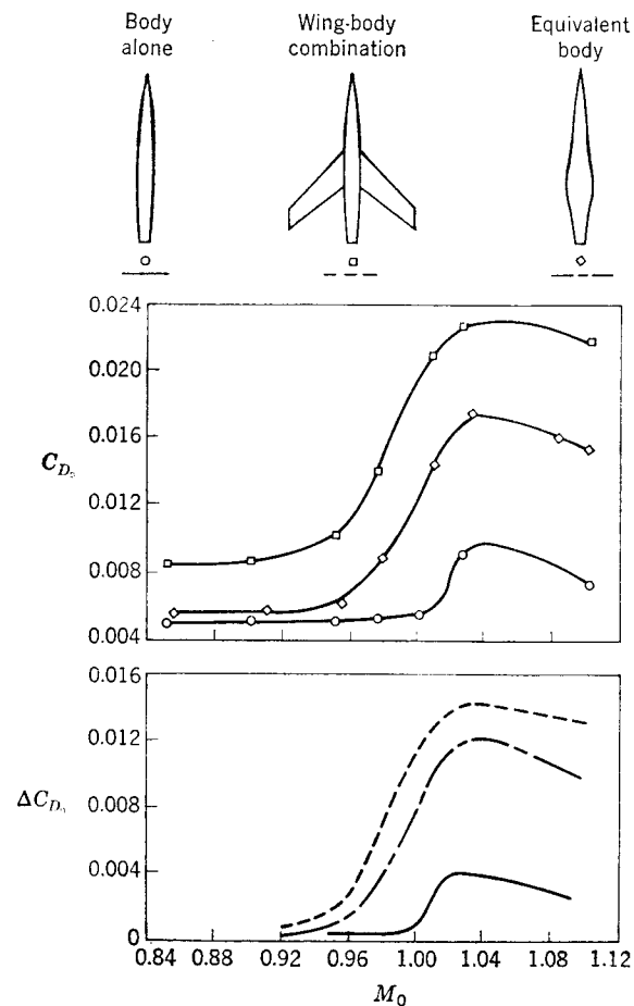
FIG. 9-17. Experimental results illustrating equivalent-body concept of Whitcomb.
