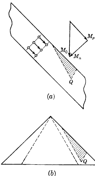
FIG. 2-10. Simple sweep theory with application to triangular wing with supersonic leading edges. (a) Infinite swept wing; (b) triangular wing.
