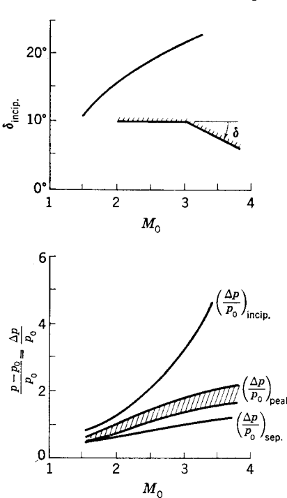
FIG. 8-27. Control deflection and pressure ratio for incipient separation of supersonic turbulent boundary layer.
