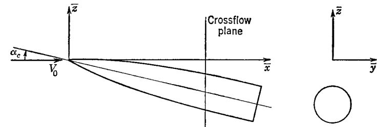
FIG. 3-4. Axes used in slender-body theory.
