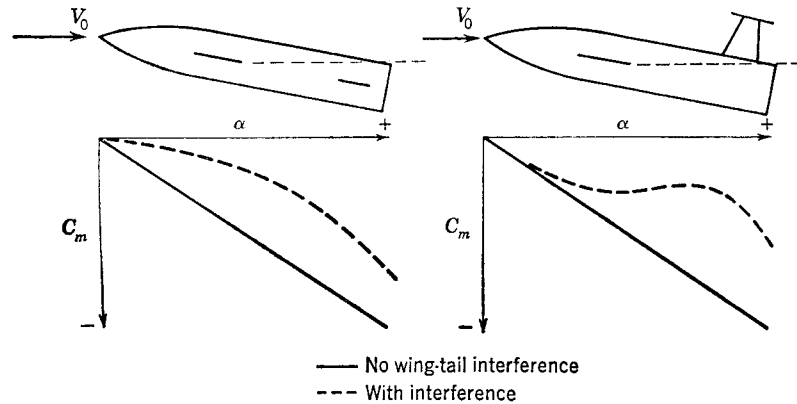
FIG. 7-11. Effect of tail height on moment curve of complete configuration.
