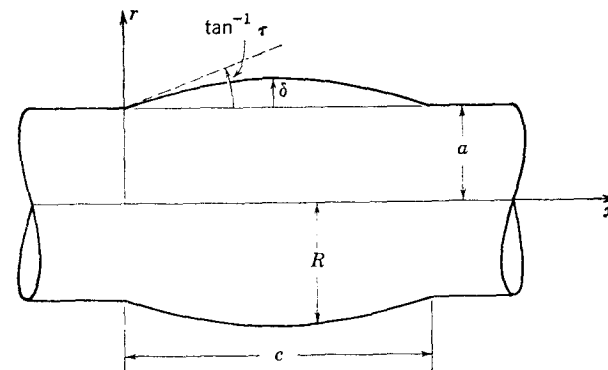
FIG. 4-11. Circular cylinder with axially symmetric bump.
