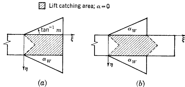
FIG. 5-12. Planar models for calculating afterbody effects. (a) No afterbody; (b) afterbody.
