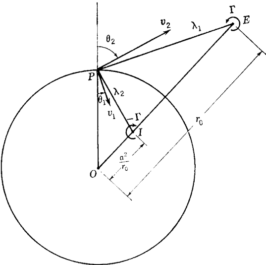
FIG. 6-13. External vortex with internal image vortex.
