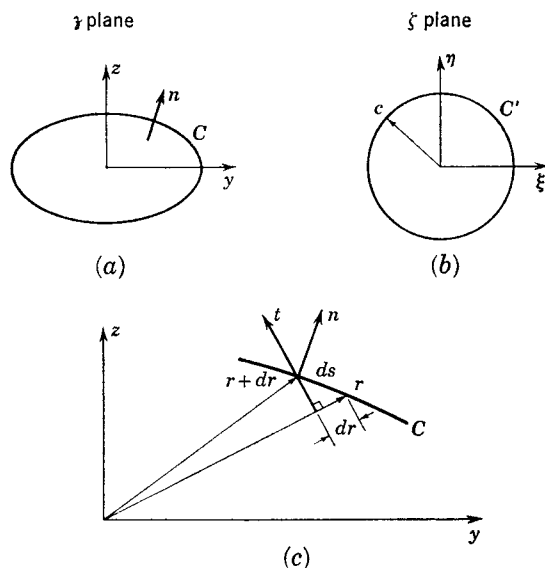
FIG. 10-10. Notation in determination of apparent-mass coefficients. (a) Physical plane; (b) transformed plane; (c) boundary conditions for \phi_3 .
