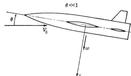
FIG. 8-31. Missile undergoing impulsive pitch control.
