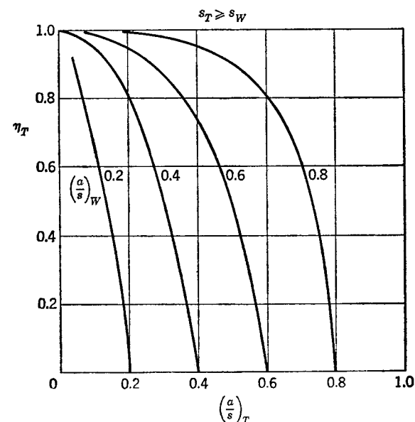
FIG. 7-2. Tail effectiveness for flat vortex sheet.
