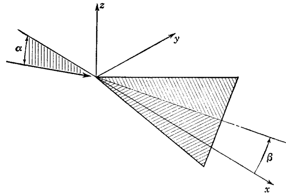
FIG. 5-9. Triangular lifting surface at combined pitch and sideslip.
