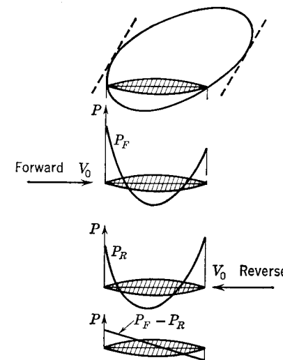
Fig. 9-16. Example illustrating Jones's criterion for minimum thickness drag for a given wing planform and wing volume.
