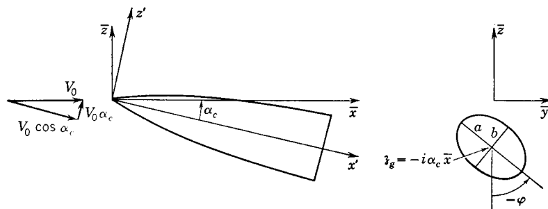
Fig. 4-5. Axis conventions and notation for elliptical bodies.
