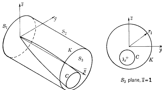
FIG. 3-5. Cylindrical control surface enclosing slender body.
