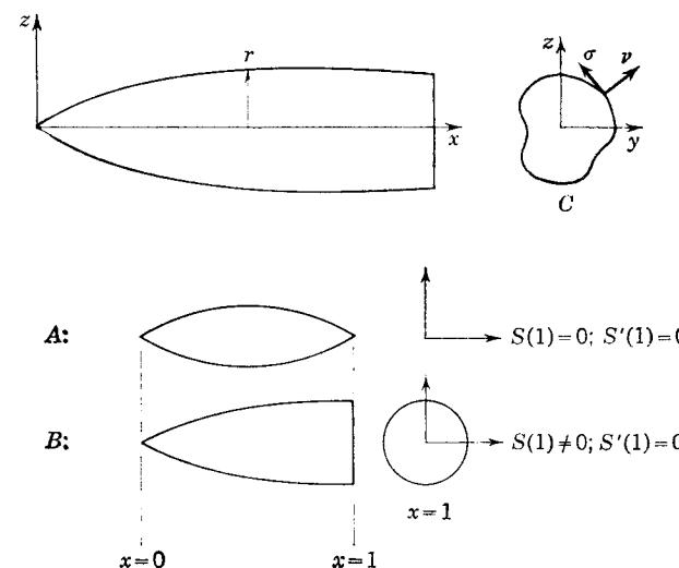
FIG. 9-4. Notation for use in drag formula of Ward.
