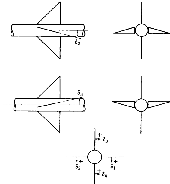
FIG. 8-2. Positive deflection angles. Top left, side view; center left, top view; bottom, end view.
