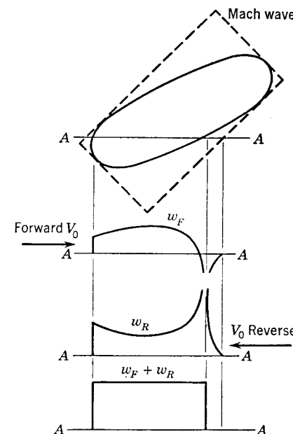
FIG. 9-21. Example illustrating Jones's criterion for minimum drag due to lift for lifting surface of given planform and total lift.
