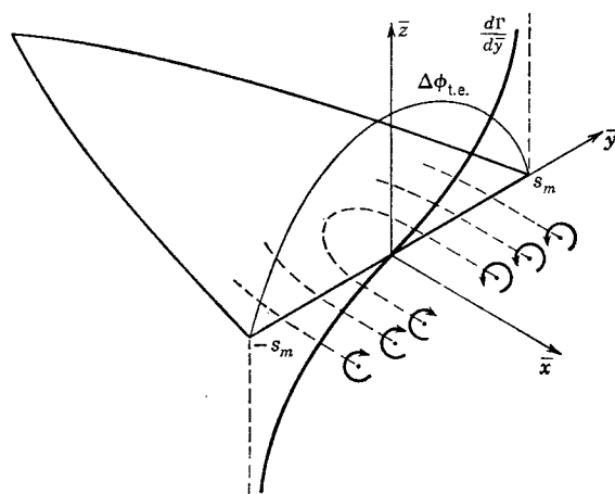
FIG. 6-2. Vortex system representing wing.
