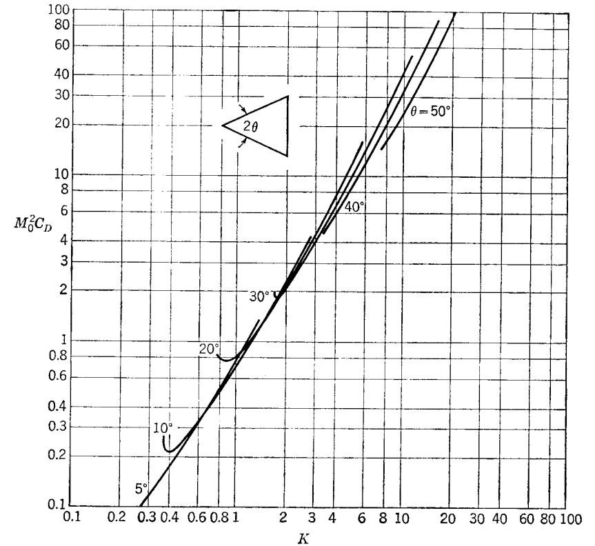
FIG. 9-7. Correlation of drag coefficients of cones at supersonic speeds by hypersonic similarity parameter.
