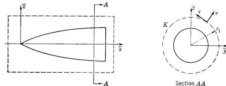
FIG. 3-7. Contour for evaluation of a_0(\bar{x}) .
