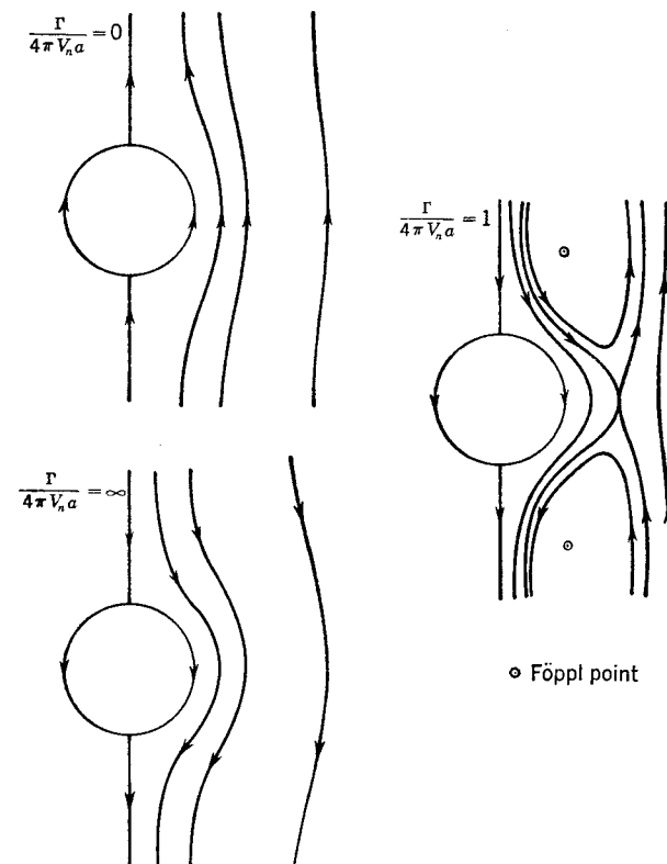
FIG. 6-20. Vortex paths in crossflow past a circular cylinder.
