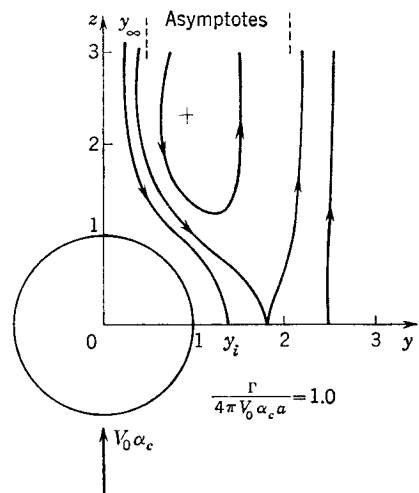
FIG. 4-20. Paths of symmetrical vortex pair in presence of circular cylinder.
