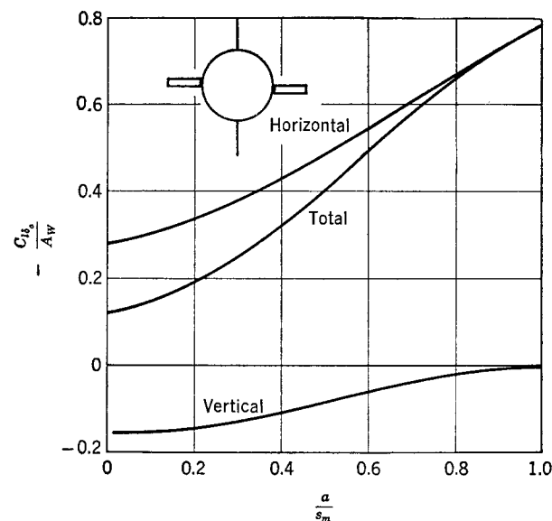
FIG. 8-12. Rolling effectiveness of cruciform all-movable controls.
