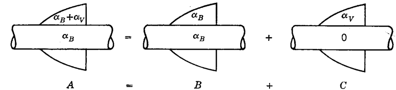
FIG. 7-13. Decomposition of twisted tail configuration into components.
