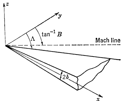
FIG. 2-3. Infinite wedge or infinite triangular cone.
