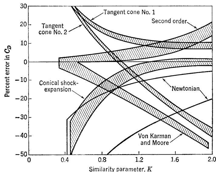
FIG. 9-9. Accuracy of various methods for estimating pressure drag of nonslender missile noses at zero angle of attack.
