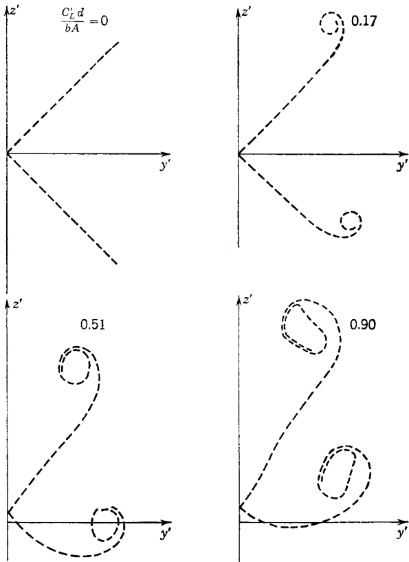
FIG. 6-27. Wake shapes behind a cruciform wing; \varphi = 45^\circ .
