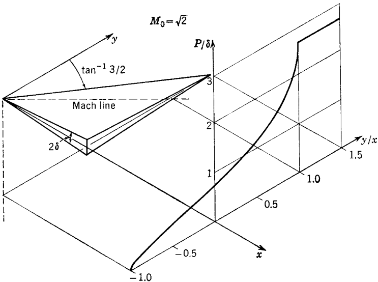
FIG. 2-5. Thickness pressure distribution on infinite wedge with supersonic leading edge.
