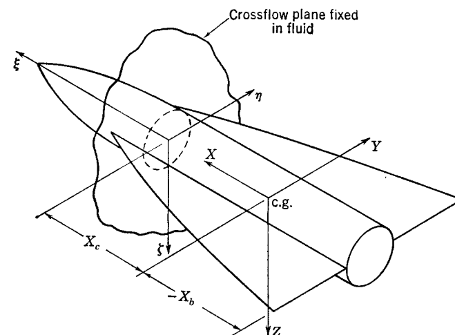
FIG. 10-7. Coordinate systems for apparent-mass analysis.
