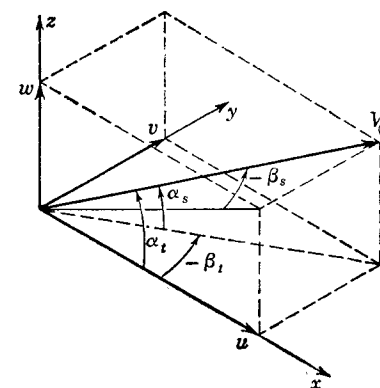
FIG. 1-3. Angles of attack and sideslip.
