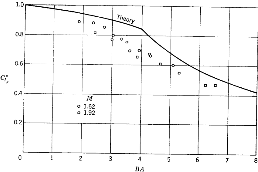
FIG. 10-18. Comparison between experiment and theory for damping in roll of triangular wings.
