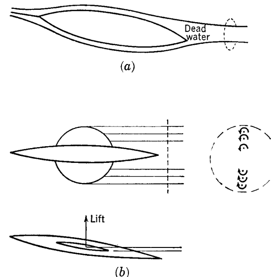
FIG. 3-8. Separated or vortex flows requiring distortion of contour of integration. (a) Body; (b) Wing-body combination.
