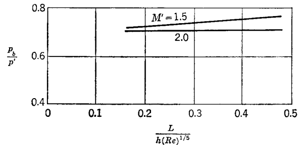
FIG. 9-31. Effect of Reynolds number on base pressure of bodies of revolution with turbulent boundary layers.
