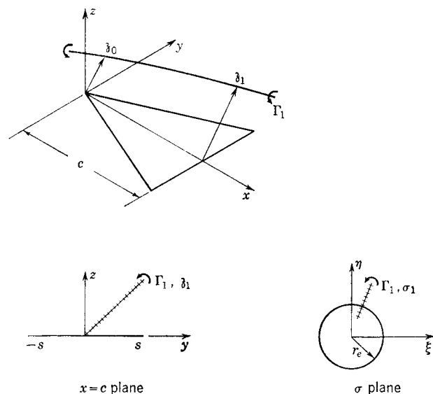
FIG. 4-24. Free vortex passing triangular wing.
