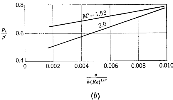
FIG. 9-32. Base-pressure correlations for (a) airfoils and (b) bodies of revolution with boundary layers turning turbulent behind the base.
