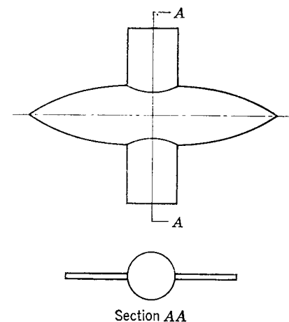
FIG. 9-18. Indentation of body to minimize pressure drag at zero angle of attack according to NACA area rule.
