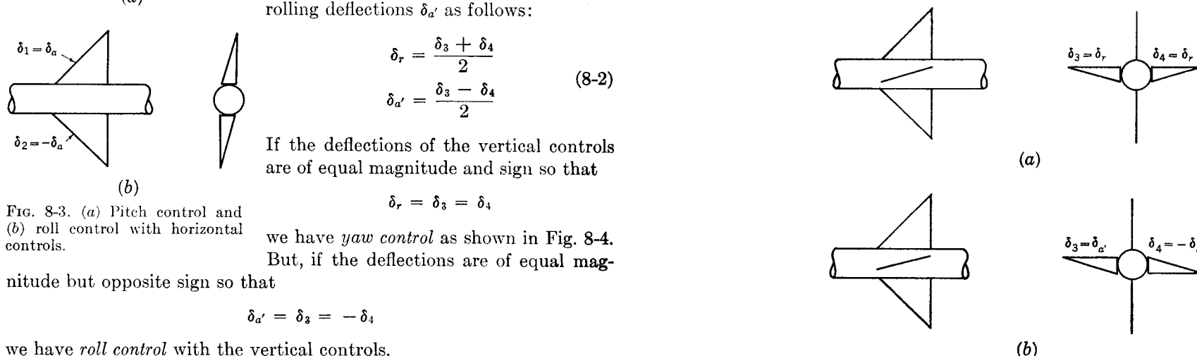
FIG. 8-4. (a) Yaw control and (b) roll control with vertical controls.
