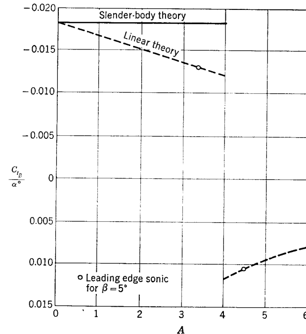
FIG. 10-22. Rolling moment due to sideslip of triangular wings; M_0^2 = 2 .
