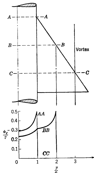
FIG. 7-6. Span loadings associated with straight-line vortices in plane of tail.
