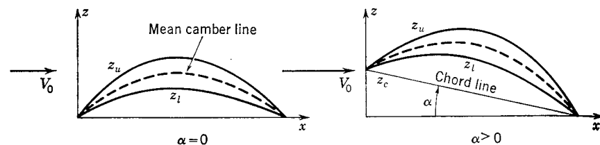
FIG. 9-12. Notation used in specifying thickness and camber distributions.
