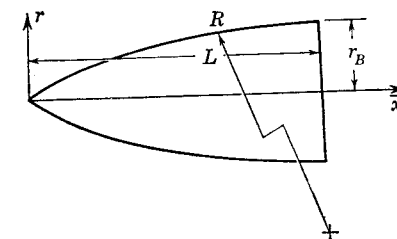
FIG. 4-2. Coordinates of tangent ogive.
