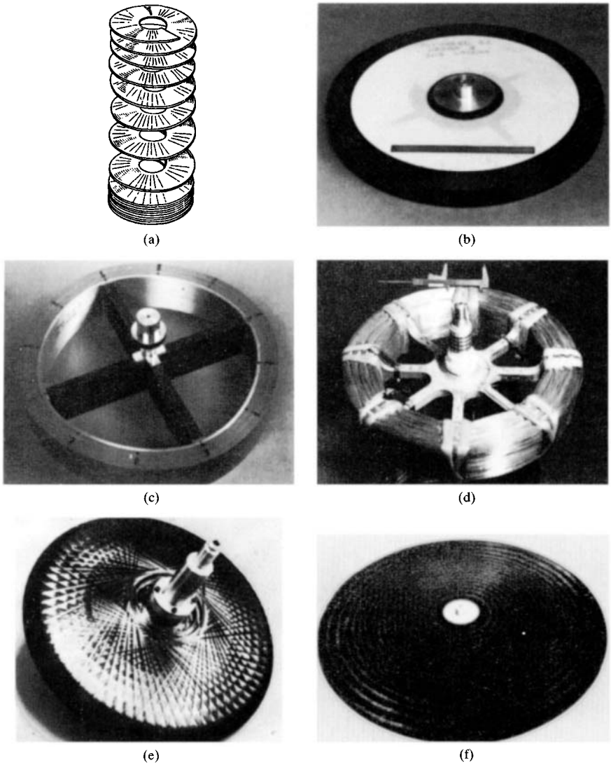
FIGURE 7.7 Energy-storage flywheel designs. (a) Flywheel of helically woven fabric with variable properties in the radial and circumferential directions ( exploded view ) (Avco Systems Division); (b) filament-wound graphite/epoxy rim with laminated S2-glass/epoxy disk (General Electric Company); (c) subcircular multilayer rim of S-glass and Kevlar, with graphite/epoxy spokes (Garrett AiResearch Corporation); (d) bare-filament Kevlar rim with aluminum hub (Istituto della Motorizzazione, Torino, Italy, built by Industrie Pirelli S.p.A. and sponsored by the Italian National Research Council); (e) graphite/epoxy and steel-filament/epoxy rim with a woven graphite/epoxy overwrap (MAN Advanced Technology, Munich, Germany); (f) variable-thickness graphite/epoxy laminated disk (Lawrence Livermore National Laboratory).
