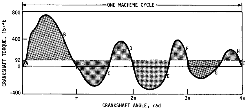
FIGURE 7.2 Torque-angle curve for the engine in Example 2. The dashed line indicates the average torque of 92.0 \text{ lb} \cdot \text{ft} , and the shaded areas are the energy variations from the average speed. Sections A and I correspond to the values given in Table 7.2.
