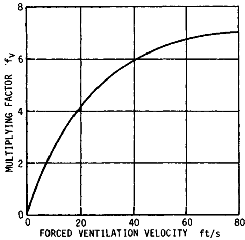
FIGURE 8.14 Ventilation factors. ( Tol-o-matic .)
