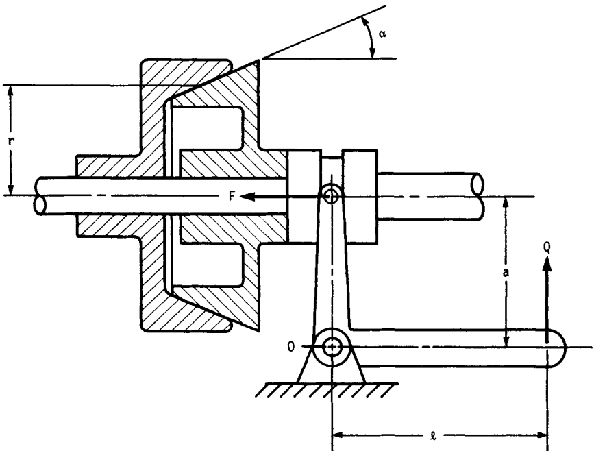
FIGURE 8.21 Cone brake; \alpha = cone angle.
