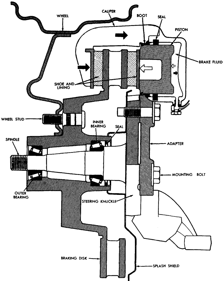
FIGURE 8.9 Automotive disk brake. (Chrysler Corporation.)
