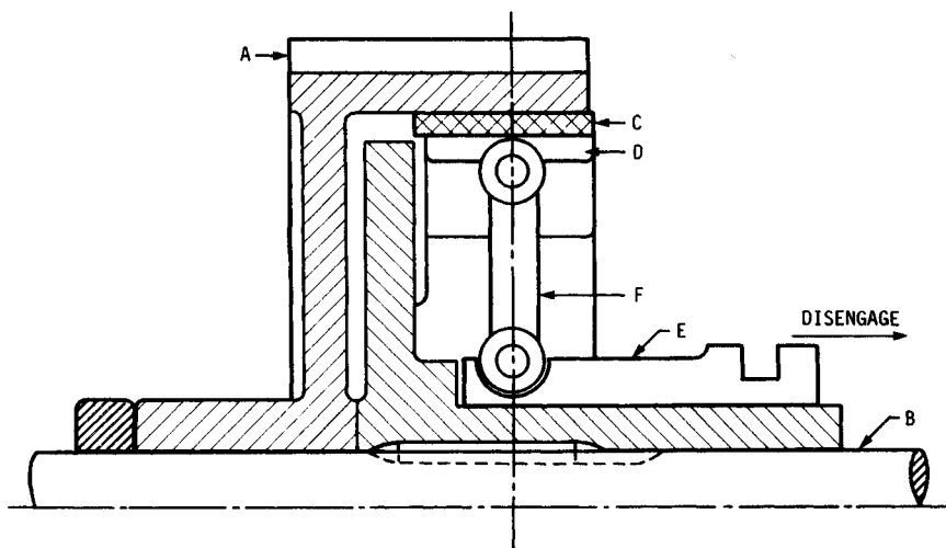
FIGURE 8.3 Schematic drawing of a radial clutch built within a gear; A, gear, the driving member; B, driven shaft; C, friction plate; D, pressure plate; E, movable sleeve; F, toggle link. This type of clutch can also be made within a V-belt sheave.
