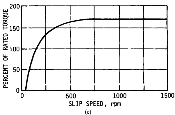
FIGURE 8.29 Torque characteristics of magnetic clutches. (a) Magnetic-particle clutch has a characteristic that is independent of slip and increases almost linearly with coil current. (b) Hysteresis clutch exhibits almost a constant torque out to the thermal, which begins at B; temperature then limits the torque capacity from B to C. (c) Eddy-current clutch exhibits a constant-torque characteristic at rated slip speed. (From Ref. [8.5].)
