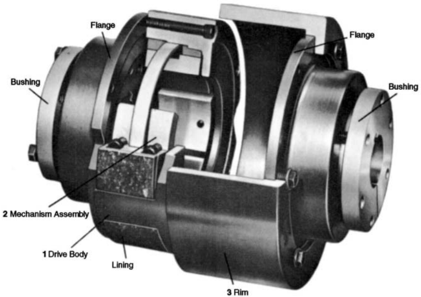
FIGURE 8.6 Centrifugal clutch. ( BLM Automatic Clutch Limited. )
