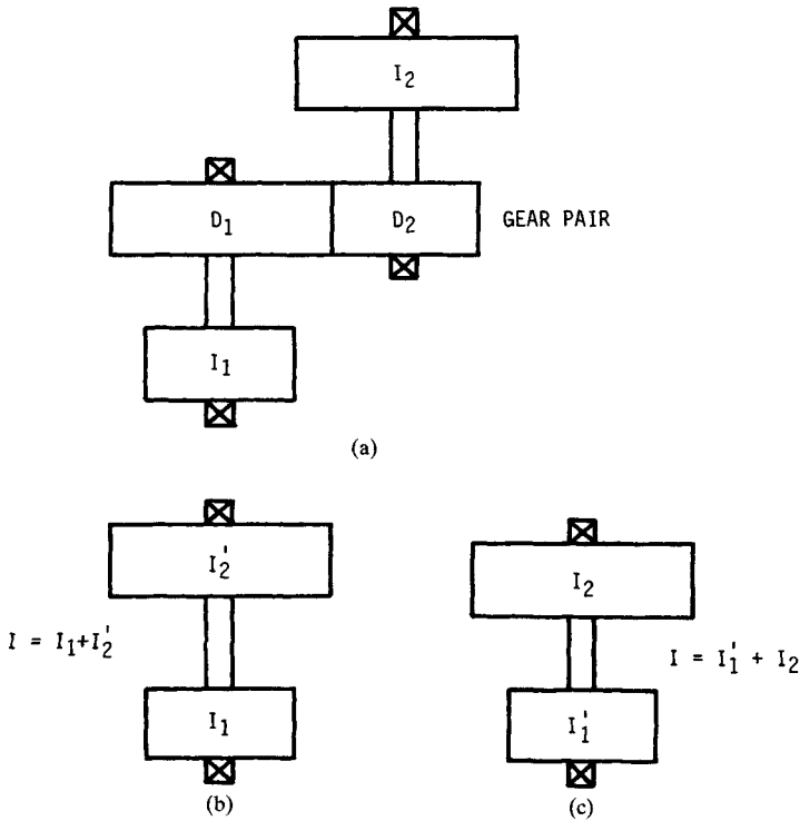
FIGURE 8.11 Equivalent inertia. I_1, I_2 = inertia of input and output shafts, respectively; I' = equivalent inertia. (a) Original configuration; (b) equivalent system referred to input shaft; (c) equivalent system referred to output shaft. For a more extensive treatment of equivalent inertias, see “Suggested Reading” list, Mischke.
