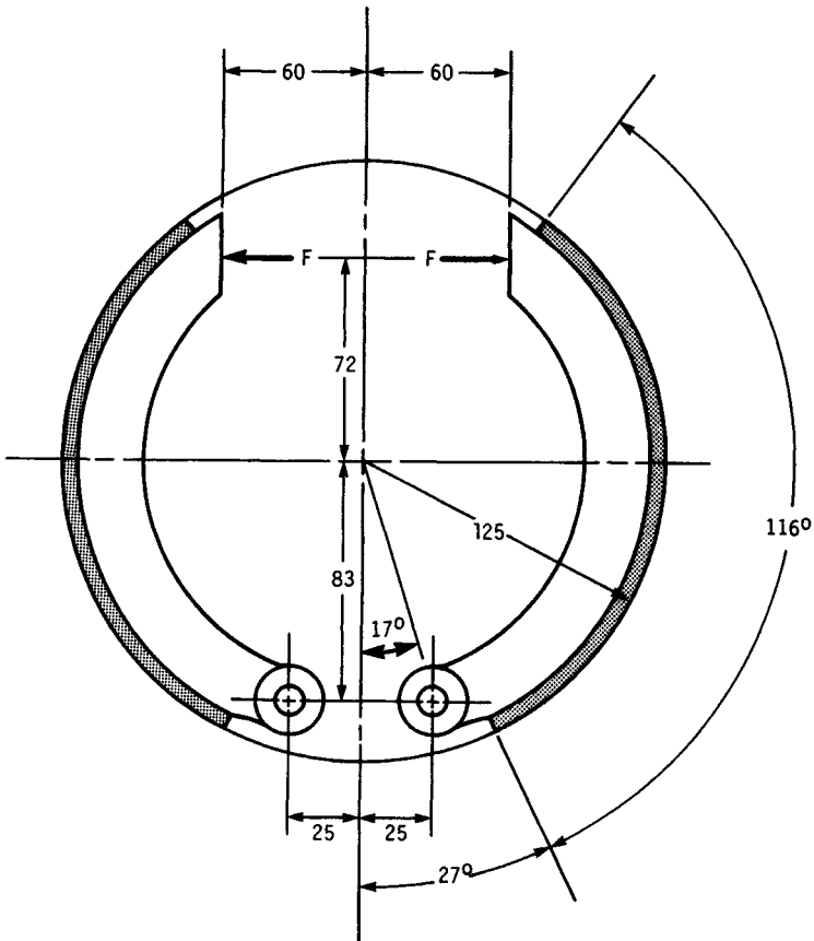
FIGURE 8.17 A leading-shoe trailing-shoe automotive brake.
