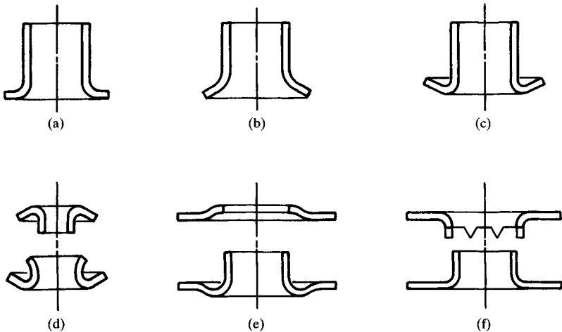
FIGURE 24.12 (a) Flat-flange eyelet; (b) funnel-flange eyelet; (c) rolled-flange eyelet; (d) telescoping eyelet with neck washer; (e) plain grommet; (f) toothed grommet.
