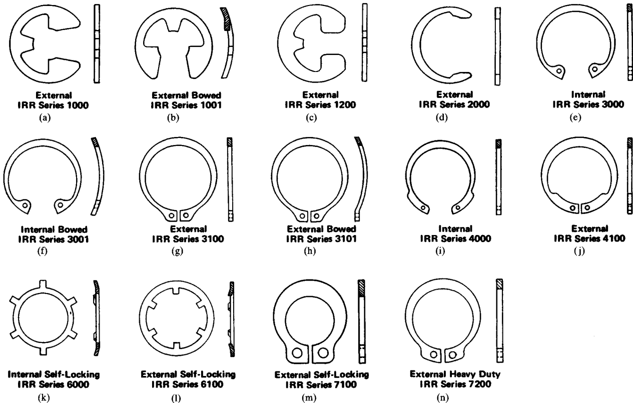
FIGURE 24.13 Retaining rings. The IRR numbers are catalog numbers. See Table 24.17 for conversion to military standard numbers. ( Industrial Retaining Ring Company. )
