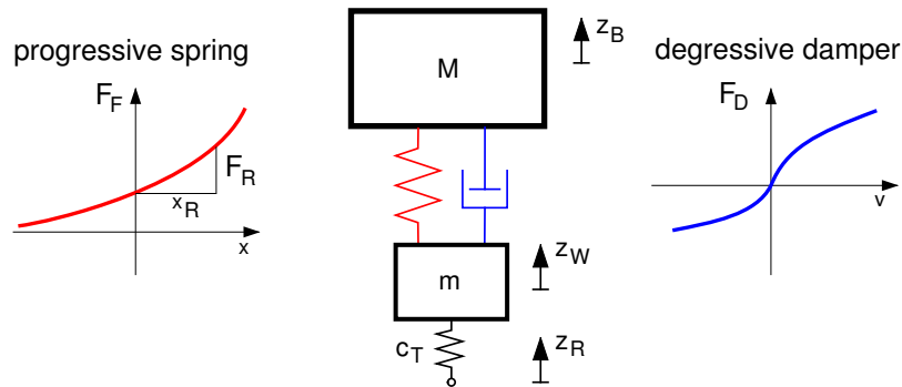
Figure 3.5: Quarter Car Model with nonlinear Characteristics
