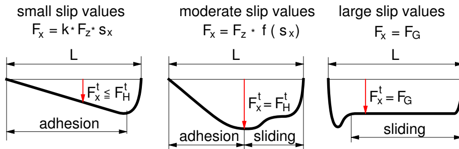
Figure 2.7: Longitudinal Force Distribution for different Slip Values
