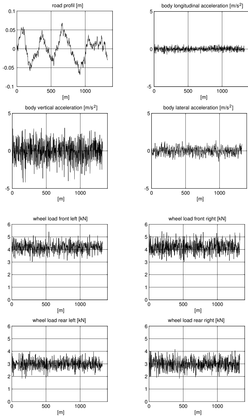
Figure 6.12: Road Profile, Accelerations and Wheel Loads
