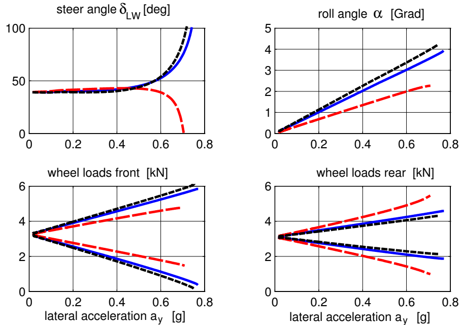
Figure 6.10: Steady State Cornering, — Semi-Trailing Arm, - - Single Wishbone, \cdots Trailing Arm
