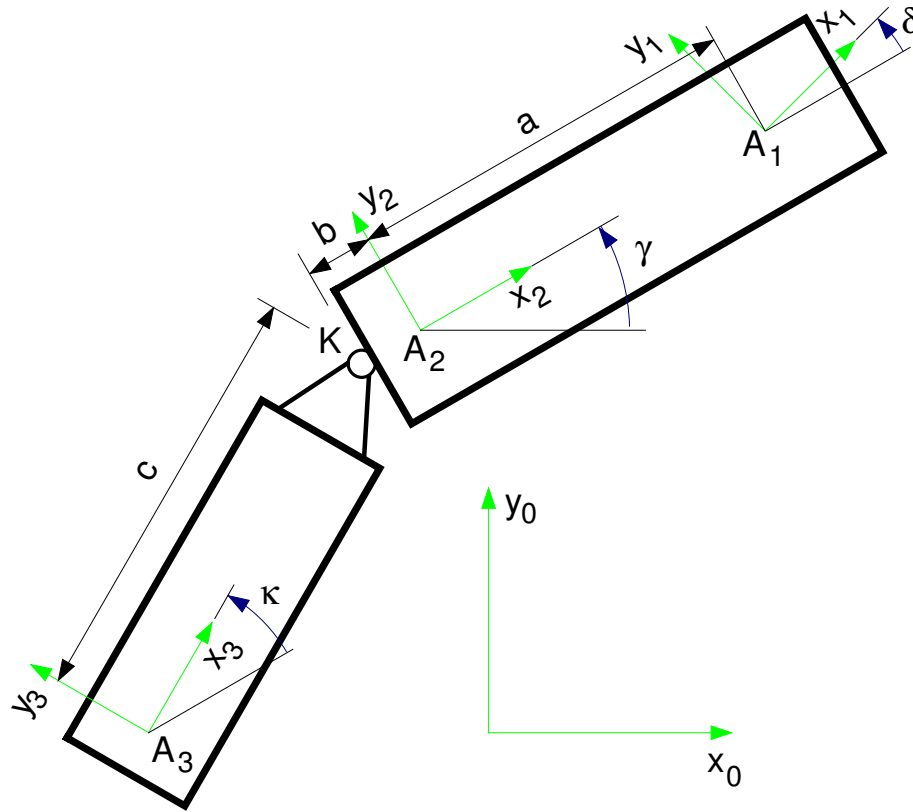
Figure 5.4: Kinematic Model with Trailer
