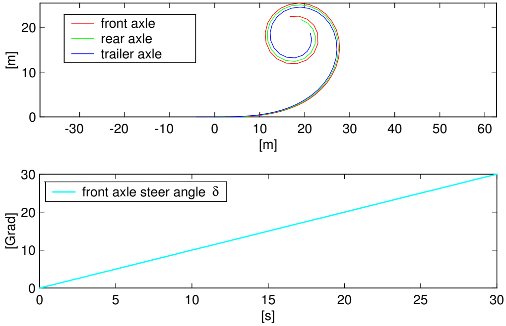
Figure 5.5: Entering a Curve
