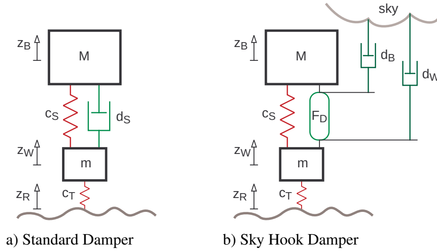
Figure 3.3: Quarter Car Model with Standard and Sky Hook Damper
