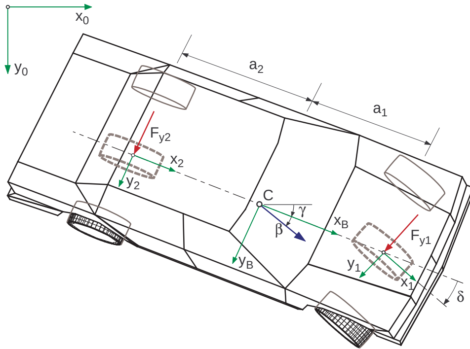
Figure 5.13: Simple Handling Model
