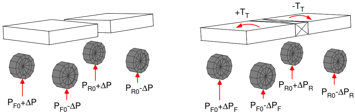
Figure 5.12: Wheel Loads for a flexible and a rigid Chassis
