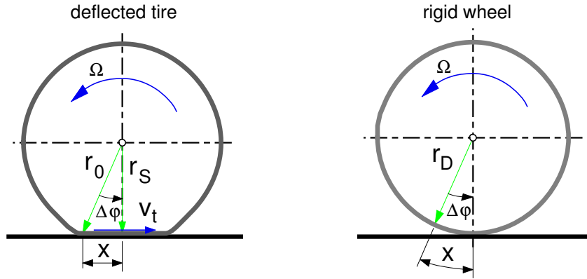
Figure 2.4: Dynamic Rolling Radius
