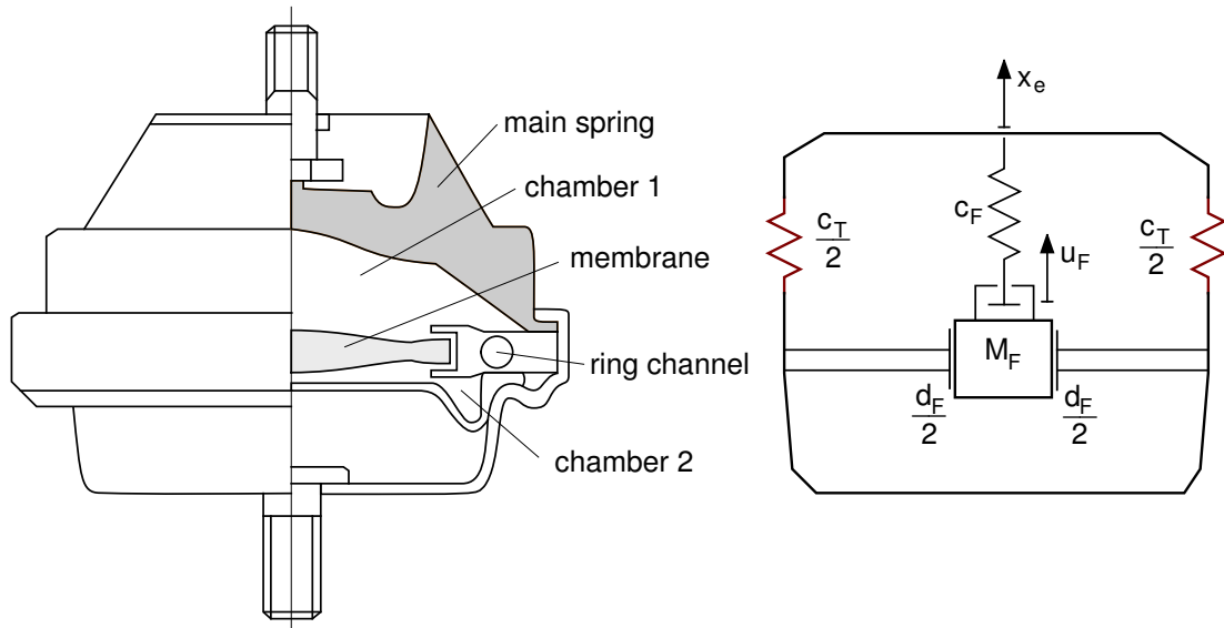
Figure 3.11: Hydro-Mount
