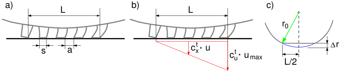
Figure 2.6: a) Particles, b) Force Distribution, c) Tire Deformation
