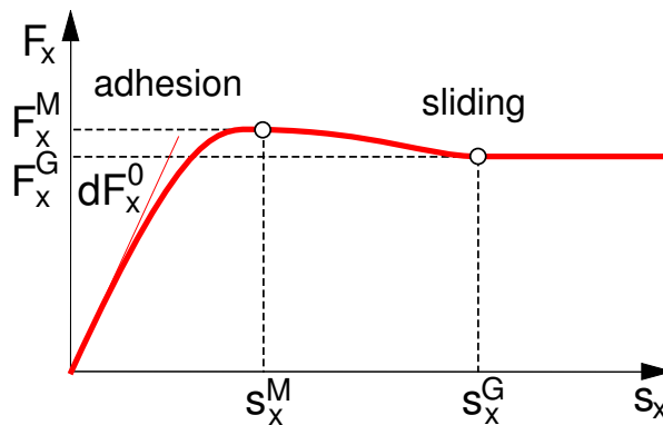
Figure 2.8: Typical Longitudinal Force Characteristics
