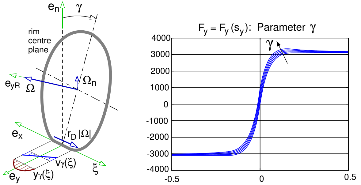
Figure 2.11: Cambered Tire F_y(\gamma) at F_z = 3.2 \text{ kN} and \gamma = 0^\circ, 2^\circ, 4^\circ, 6^\circ, 8^\circ
