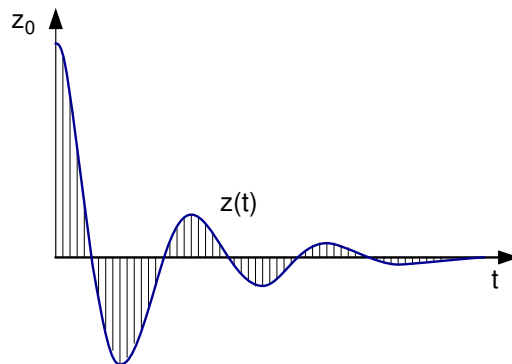
Figure 3.2: Damped Vibration
