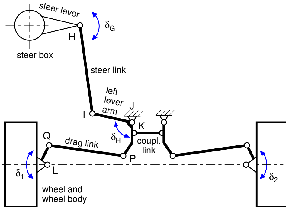
Figure 1.7: Bus Steer System
