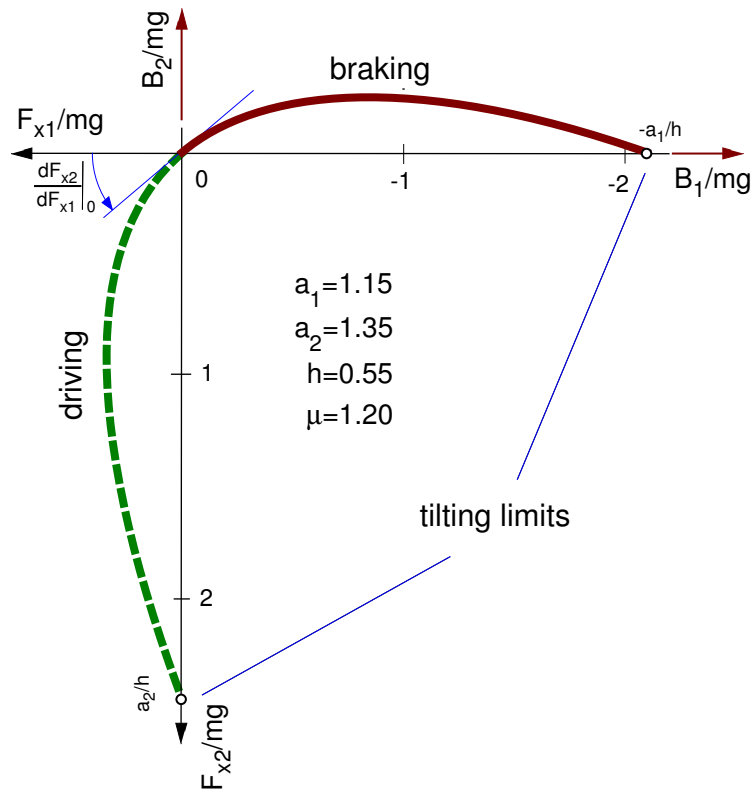
Figure 4.6: Optimal Distribution of Drive and Brake Forces
