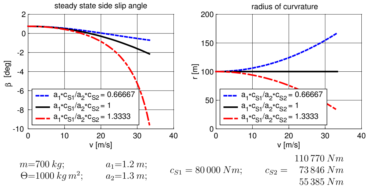
Figure 5.14: Steady State Cornering
