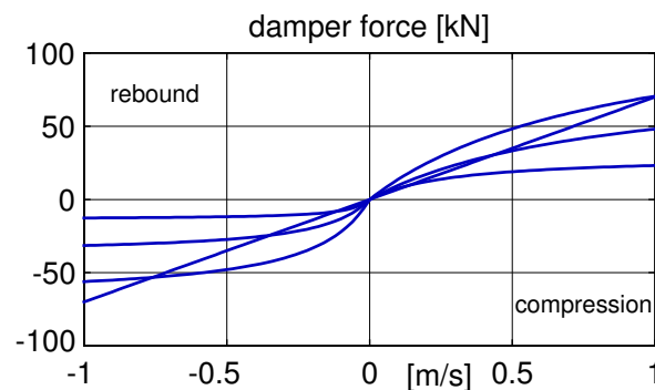
Figure 3.10: Optimal Damper Characteristics according to Table 3.6
