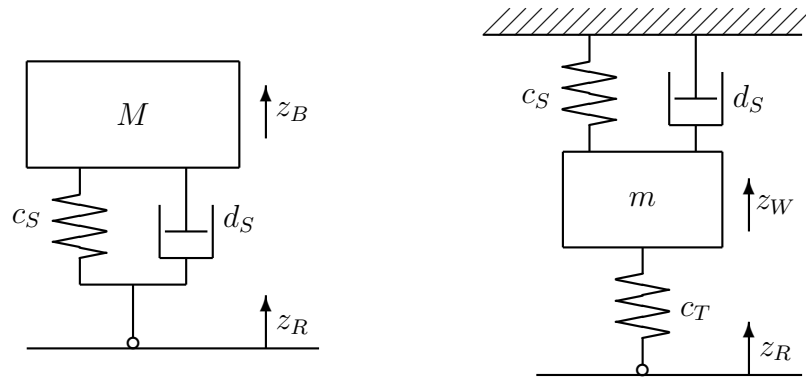
Figure 3.1: Simple Vehicle and Suspension Model
