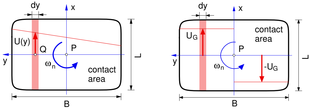
Figure 2.12: Bore Torque generated by Longitudinal Forces
