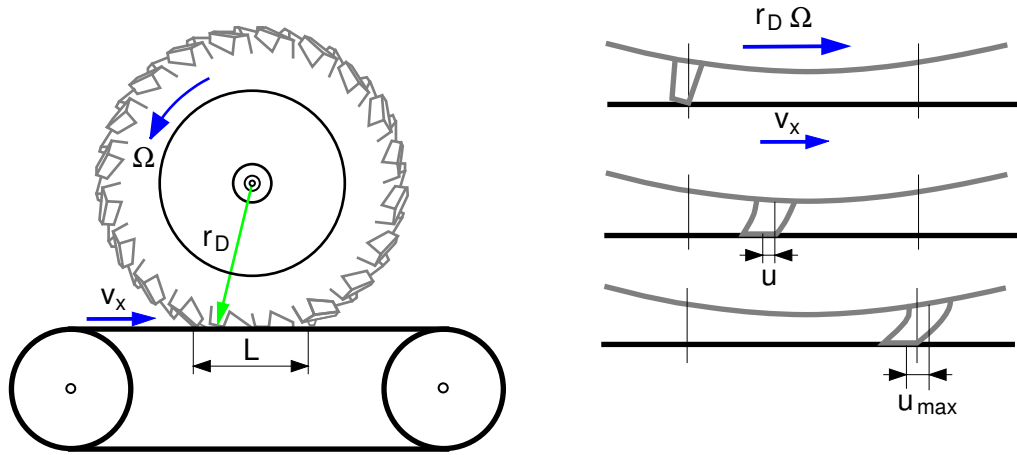
Figure 2.5: Tire on Flat Track Test Rig
