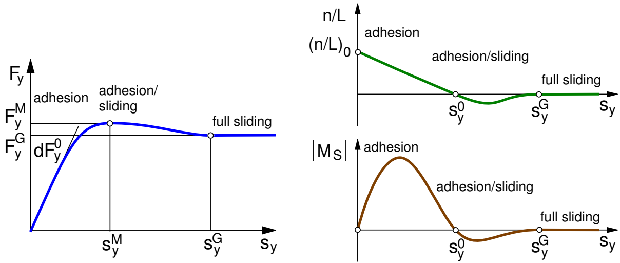
Figure 2.10: Typical Plot of Lateral Force, Tire Offset and Self Aligning Torque
