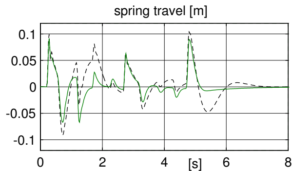
Figure 3.9: Spring Travels on Profile 2 (--- G_{K1} , — G_{K2} )
