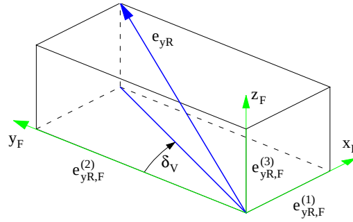
Figure 1.11: Toe Angle
