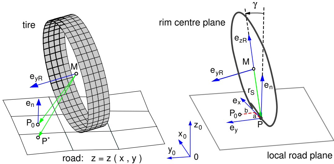
Figure 2.2: Contact Geometry
