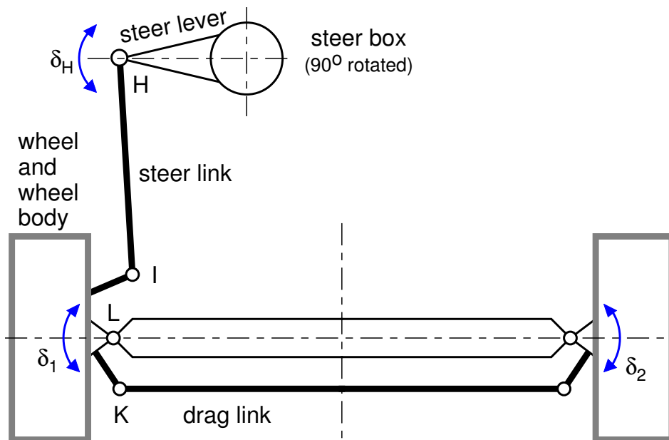
Figure 1.6: Drag Link Steering System
