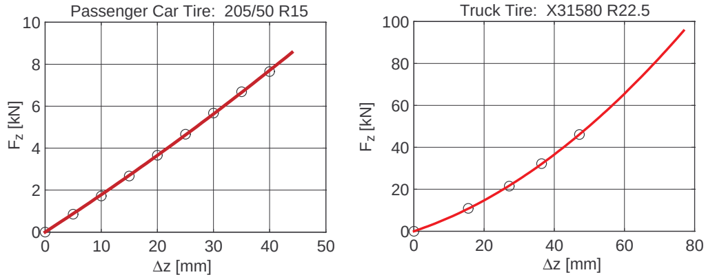
Figure 2.3: Tire Radial Stiffness: \circ Measurements, — Approximation
