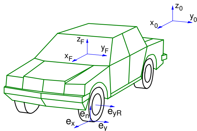
Figure 1.8: Coordinate Systems
