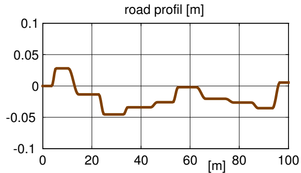
Figure 3.6: Track profile 1
