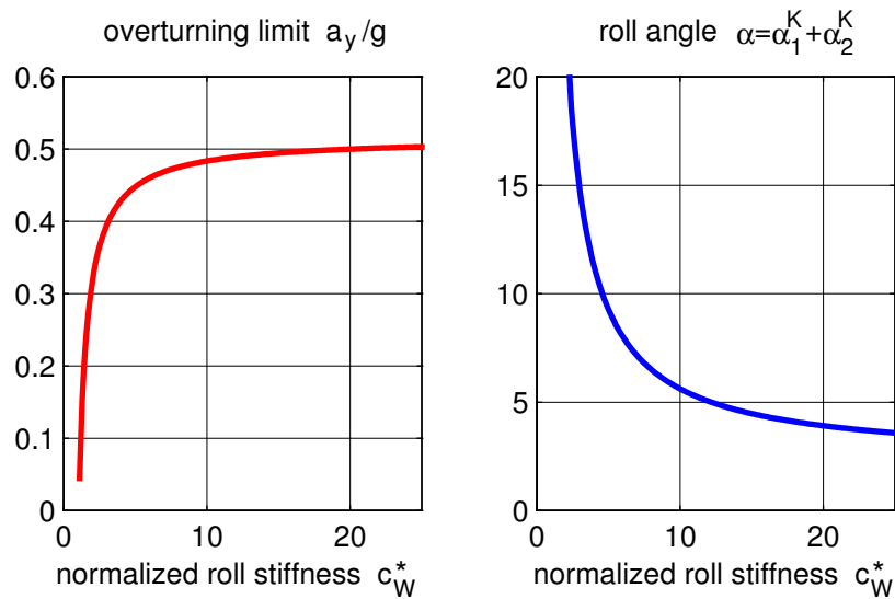
Figure 5.8: Tilting Limit for a Truck at Steady State Cornering
