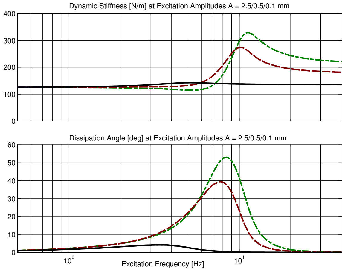
Figure 3.12: Dynamic Stiffness [N/mm] and Dissipation Angle [deg] for a Hydro-Mount
