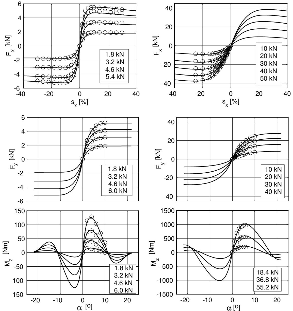
Figure 2.13: Longitudinal Force, Lateral Force and Self Aligning Torque: \circ Meas., — TMeasy
