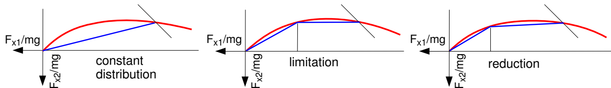
Figure 4.7: Different Distributions of Brake Forces
