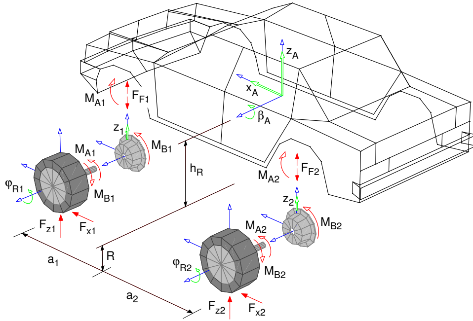
Figure 4.8: Plane Vehicle Model
