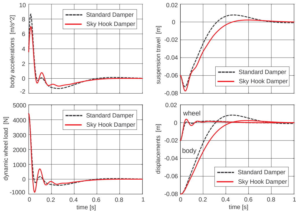
Figure 3.4: Standard and Sky Hook Damper Performance
