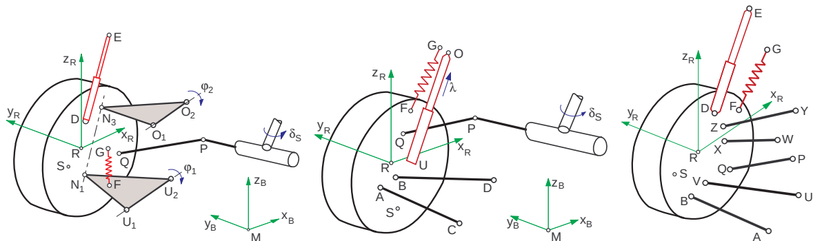
Figure 1.1: Double Wishbone, McPherson and Multi-Link Suspension
