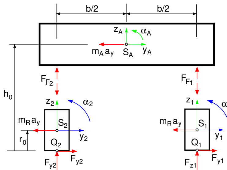
Figure 5.9: Plane Roll Model
