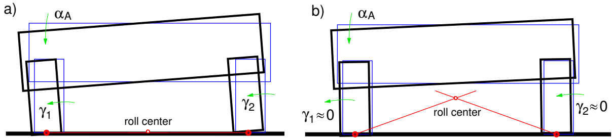
Figure 5.10: Roll Behavior at Cornering: a) without and b) with Camber Compensation
