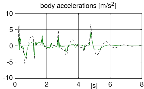
Figure 3.7: Body Accelerations optimized via G_{K1} (··· linear, — nonlinear)
