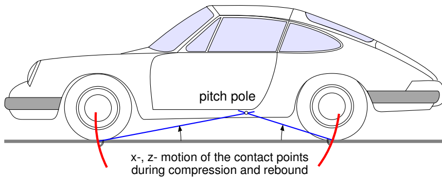
Figure 4.9: Brake Pitch Pole
