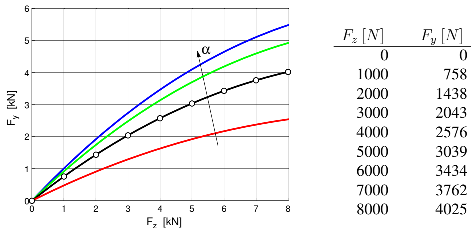
Figure 5.15: Lateral Force F_y over Wheel Load F_z at different Slip Angles
