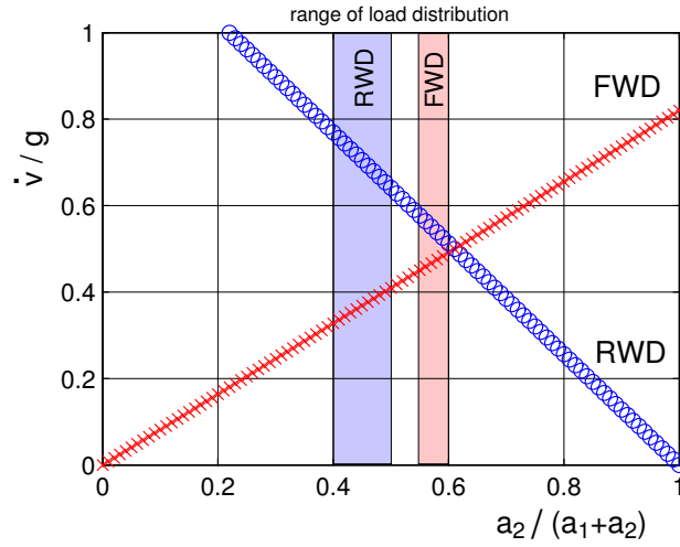
Figure 4.4: Single Axle Driven Passenger Car: \mu = 1 , h = 0.55 \text{ m} , a_1 + a_2 = 2.5 \text{ m}
