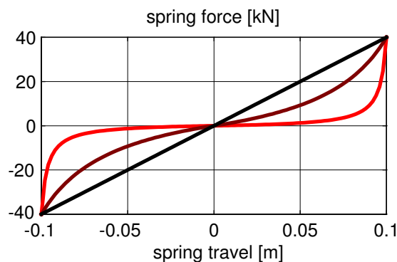
Figure 3.8: Optimal Spring Characteristics for fully loaded Vehicle; Criteria: G_{K1}
