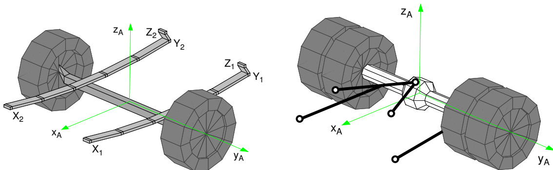
Figure 1.2: Solid Axles
