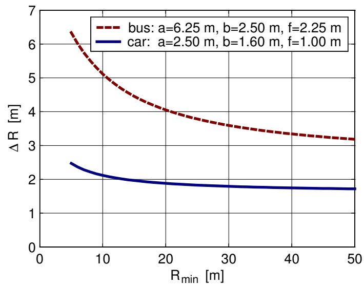
Figure 5.3: Space Requirement of typical Passenger Car and Bus
