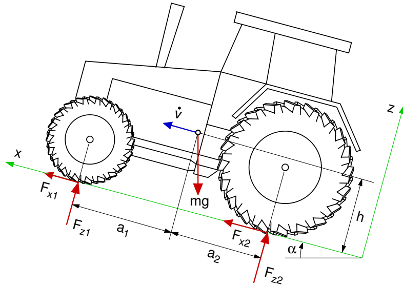
Figure 4.2: Vehicle on Grade
