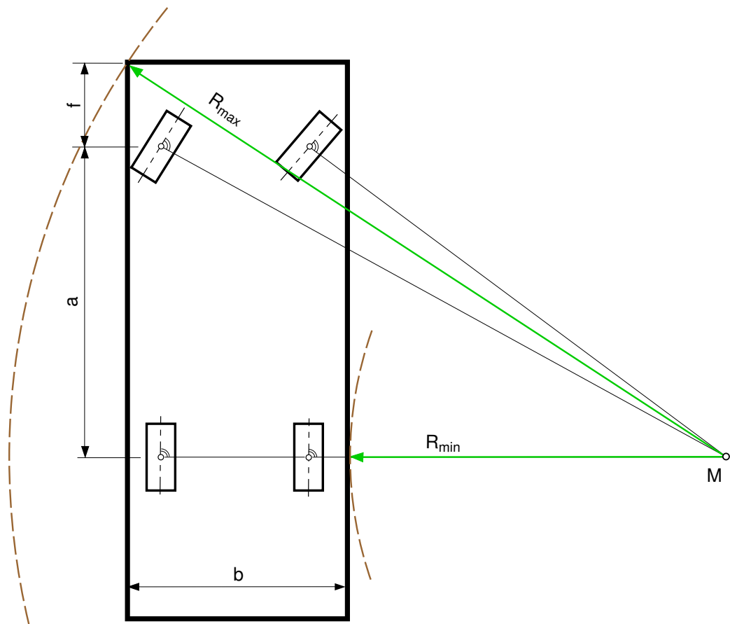
Figure 5.2: Space Requirement
