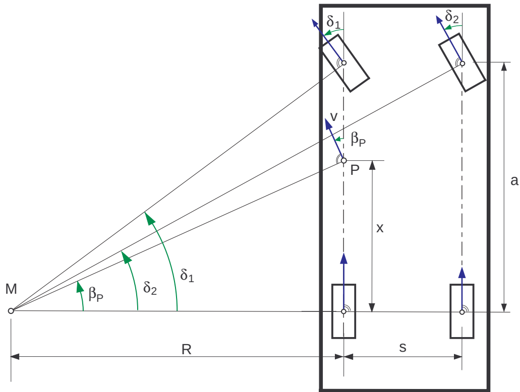
Figure 5.1: Ackermann Steering Geometry at a two-axled Vehicle
