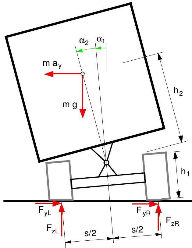
Figure 5.7: Overturning Hazard on Trucks
