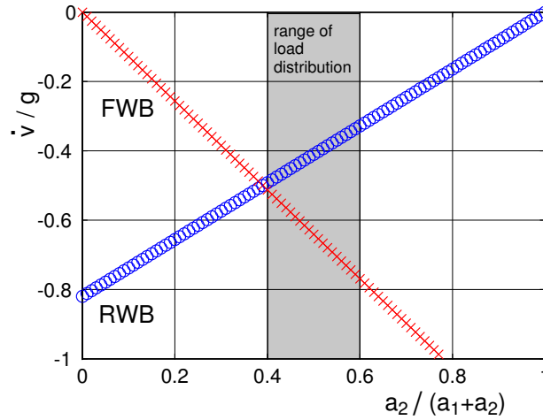
Figure 4.5: Single Axle Braked Passenger Car: \mu = 1 , h = 0.55 \text{ m} , a_1 + a_2 = 2.5 \text{ m}
