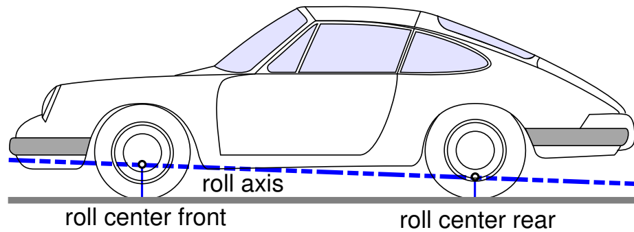
Figure 5.11: Roll Axis
