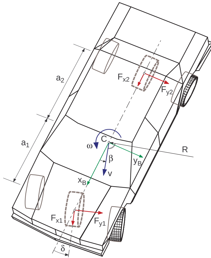
Figure 5.6: Cornering Resistance
