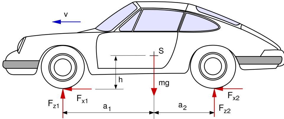
Figure 4.1: Simple Vehicle Model
