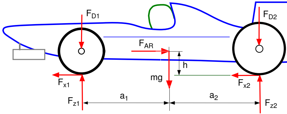
Figure 4.3: Vehicle with Aerodynamic Forces
