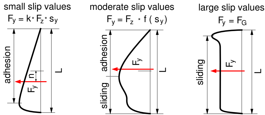
Figure 2.9: Lateral Force Distribution over Contact Area
