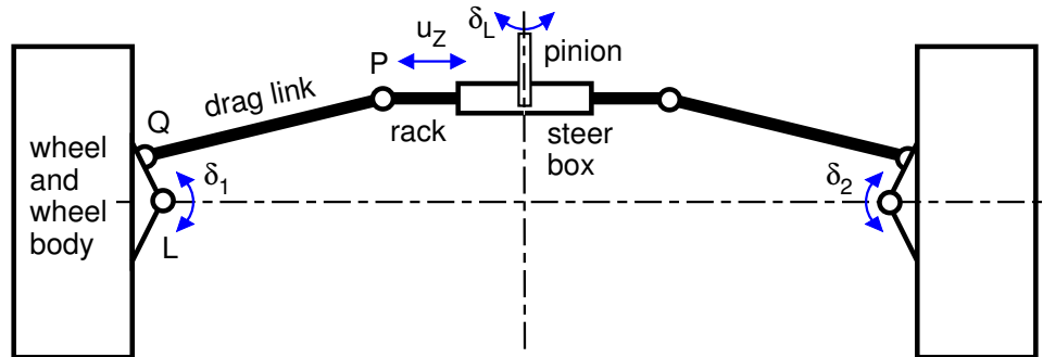
Figure 1.4: Rack and Pinion Steering
