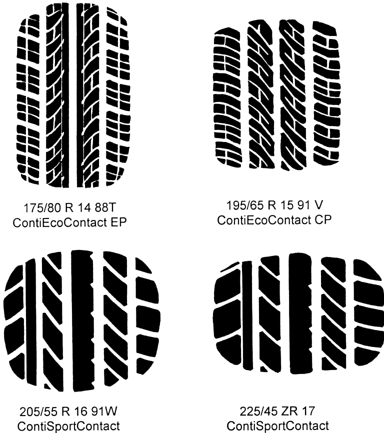
Fig. 2.9 If they have the same outside diameter and load capacity the four tyre sizes used on medium-sized passenger cars are interchangeable. The series 65, 55 and 45 wide tyres each allow a 1" larger rim (and therefore larger brake discs). The different widths and lengths of the tyre contact patch, known as 'tyre print', are clearly shown (Fig. 3.119), as are the different designs of the standard road profile and the asymmetric design of the sports profile (see also Section 2.2.10). The 65 series is intended for commercial vehicles, and the 60, 55 and 45 series for sports cars. (Illustration: Continental; see also Fig. 2.19.)
