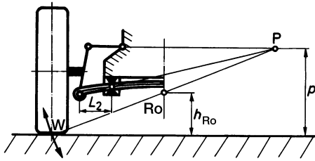
Fig. 3.28 Determination of Ro and P on a low transverse leaf spring supported in two places.
