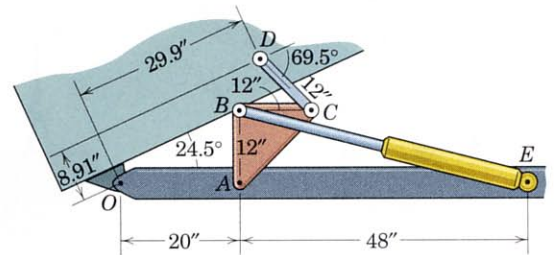
Detail of hoisting mechanism
