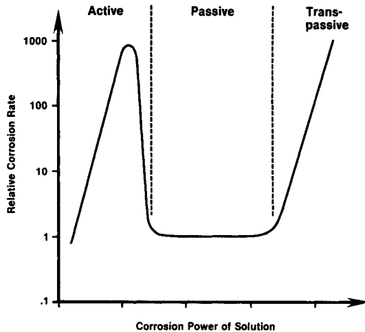
FIGURE 35.1 Corrosion characteristics of an active-passive metal.
