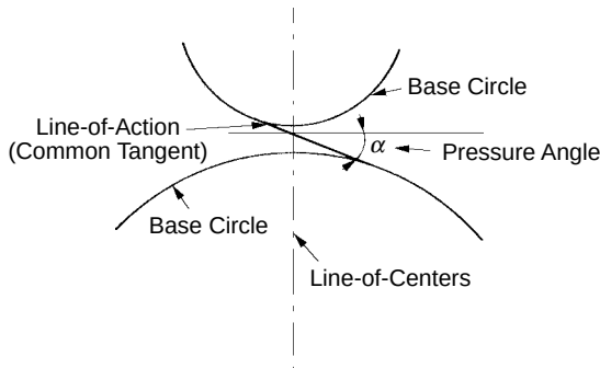
Fig. 3-1 Definition of Pressure Angle
