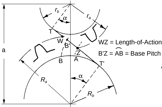
Fig. 4-3 Geometry of Contact Ratio
