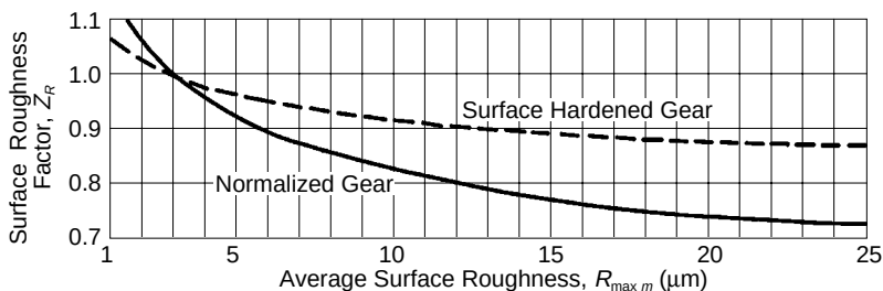
Fig. 17-11 Surface Roughness Factor, Z_R
