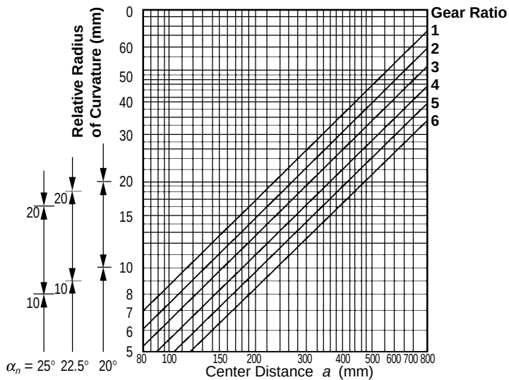
Fig. 17-6 Relative Radius of Curvature
