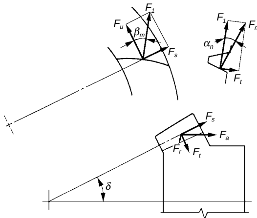
Fig. 16-9 When Meshing on the Concave Side of Tooth Face
