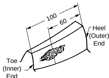
Fig. 19-1 The Contact Trace on Central Front End
