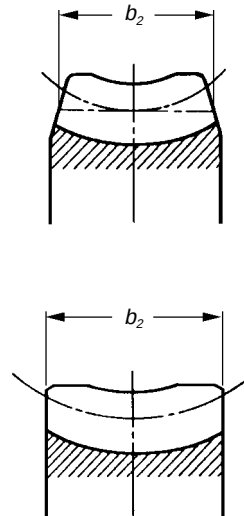
Fig. 17-13 Tooth Width of Worm Gear
