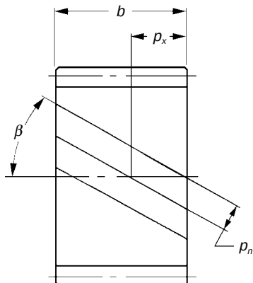
Fig. 11-3 Axial (Overlap) Contact Ratio
