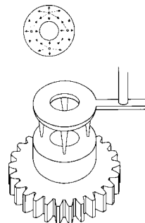
Fig. 18-13 Multiple Pin Gating
