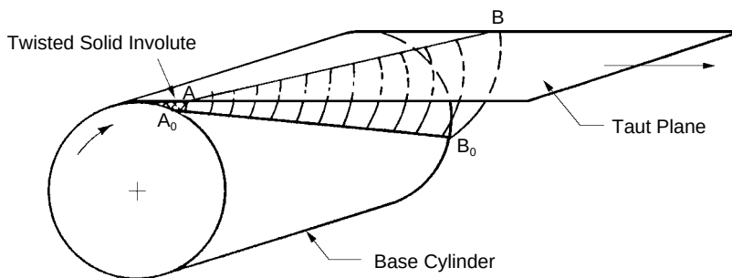
Fig. 6-2 Generation of the Helical Tooth Profile
