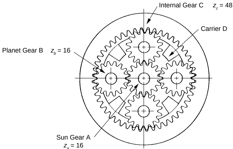
Fig. 13-4 An Example of a Planetary Gear System
