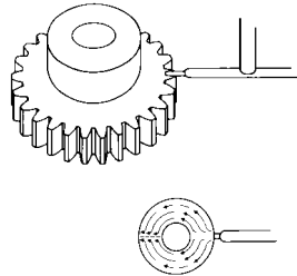
Fig. 18-11 Side Gating
