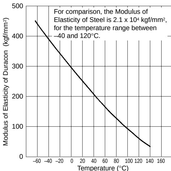
Fig. 18-5 Modulus of Elasticity in Bending of Duracon
