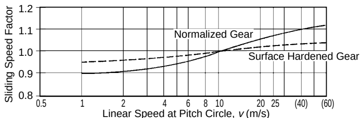
Fig. 17-5 Sliding Speed Factor, Z_v
