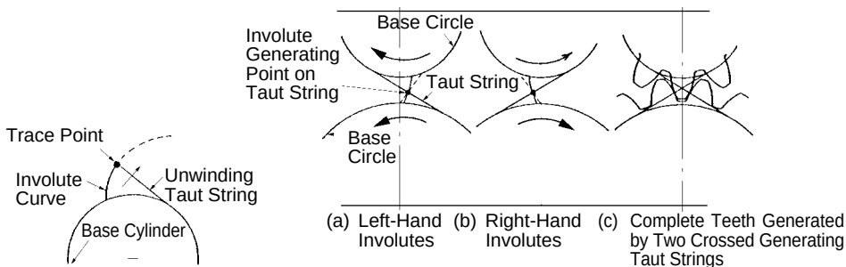
Fig. 2-2 Generation of an Involute by a Taut String
