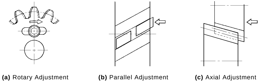
Fig. 14-10 Ways of Decreasing Backlash in Case II
