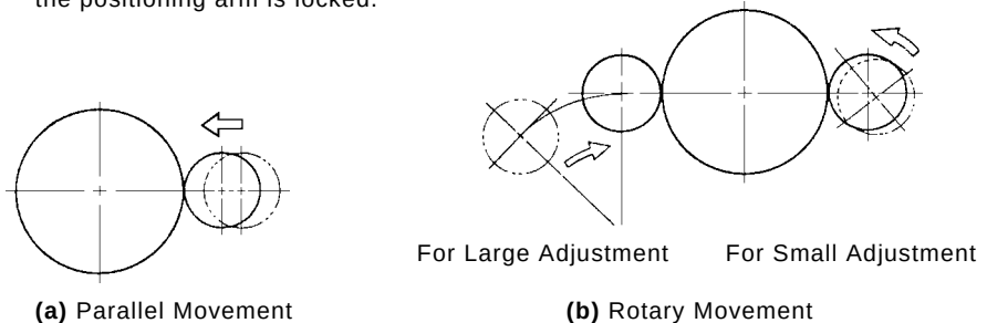
Fig. 14-11 Ways of Decreasing Backlash in Case III
