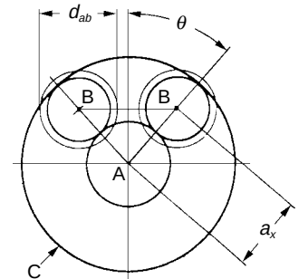
Fig. 13-5(c) Condition No. 3 of Planetary Gear System
