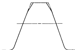
(a) Addendum Tip Relief
