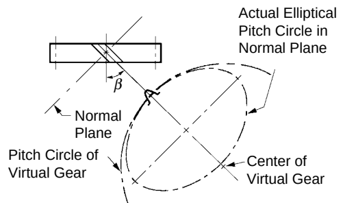
Fig. 6-7 Geometry of Helical Gear's Virtual Number of Teeth
