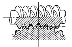
Fig. 2-17 Worm Gear
