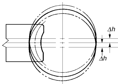
Fig. 9-7 Offsetting Up or Down
