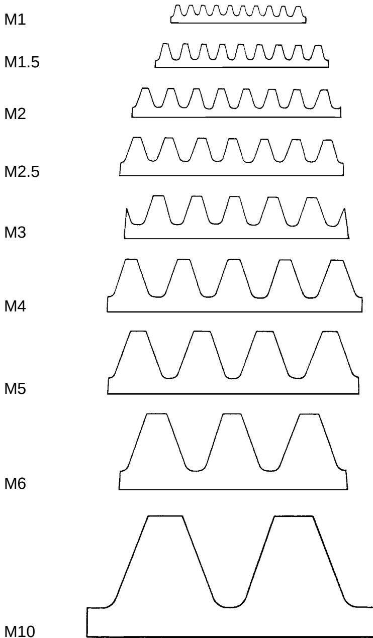
Fig. 2-6 Comparative Size of Various Rack Teeth
