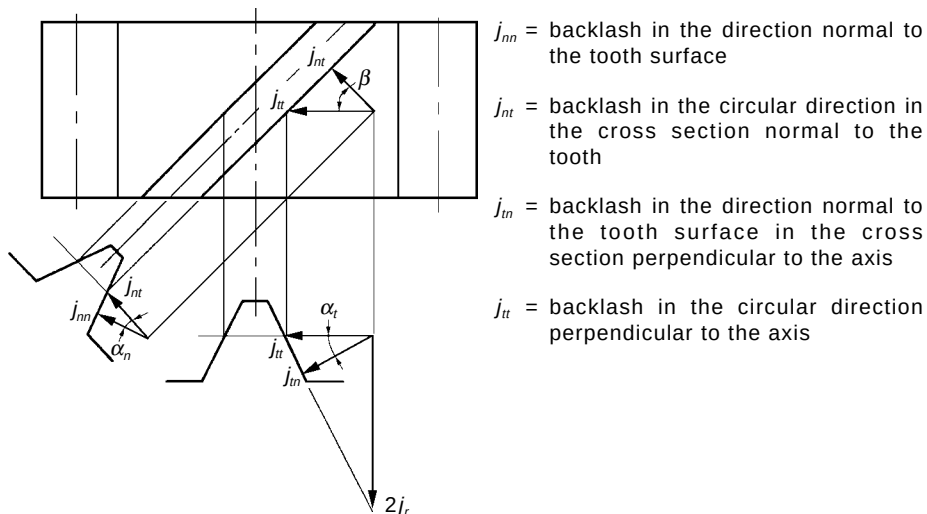
Fig. 14-5 Backlash of Helical Gear Mesh
