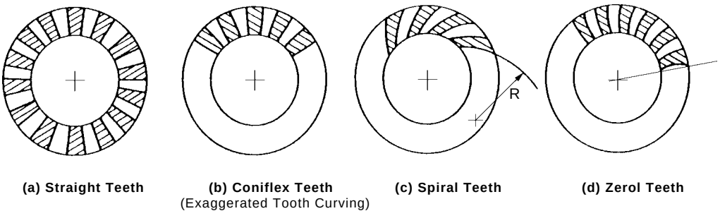
Fig. 8-6 Forms of Bevel Gear Teeth
