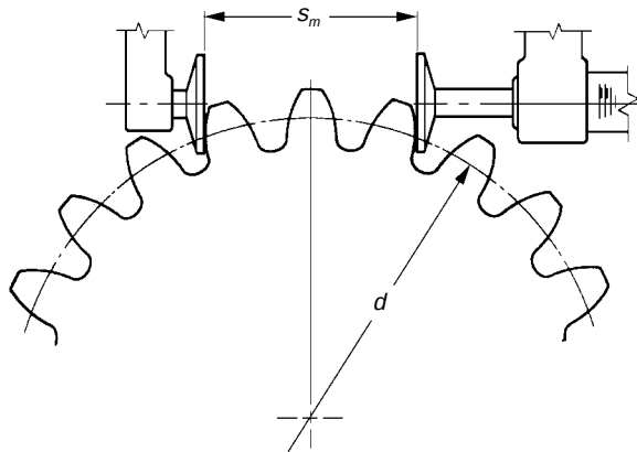
Fig. 10-4 Span Measurement of Teeth (Spur Gear)
