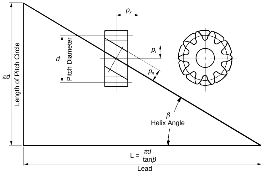
Fig. 6-6 Fundamental Relationships of a Helical Gear (Right-Handed)
