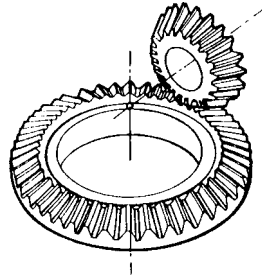
Fig. 2-16 Zerol Gear
