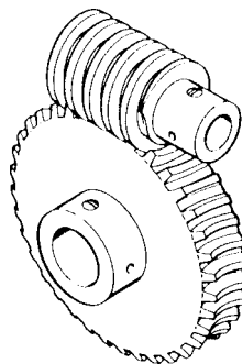
Fig. 9-1 Typical Worm Mesh
