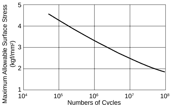
Fig. 18-6 Maximum Allowable Surface Stress (Spur Gears)
