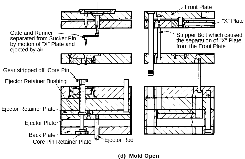
Fig. 18-14 (Cont.) Three-Plate Mold
