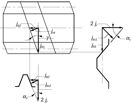
Fig. 14-8 Backlash of Worm Gear Mesh
