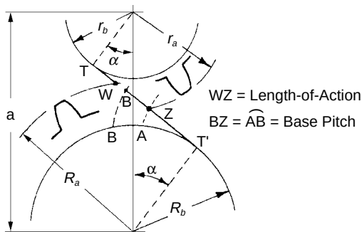
Fig. 11-1 Geometry of Contact Ratio
