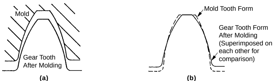
Fig. 18-8 Change of Tooth Profile
