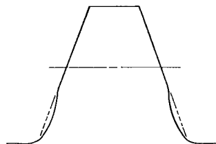
(b) Dedendum Modification
