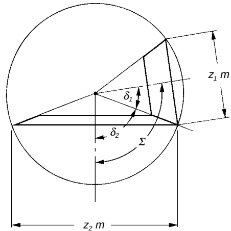
Fig. 8-7 The Pitch Cone Angle of Bevel Gear
