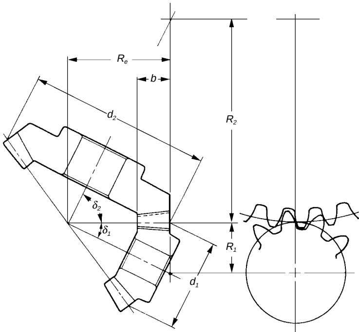
Fig. 8-8 The Meshing of Bevel Gears
