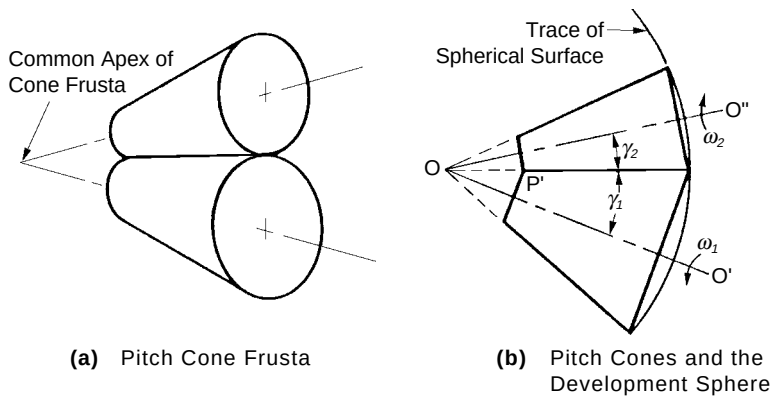
Fig. 8-2 Pitch Cones of Bevel Gears
