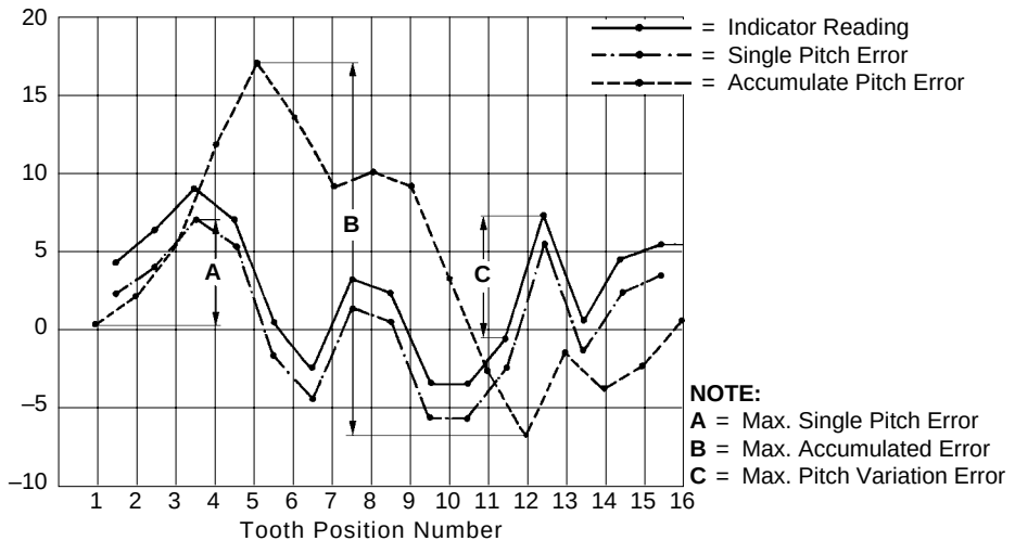
Fig. 15-1 Examples of Pitch Errors for a 15 Tooth Gear
