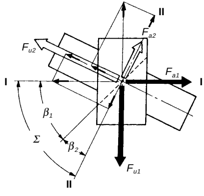
Fig. 16-15 The Forces in a Screw Gear Mesh
