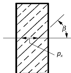
Fig. 6-5 Axial Pitch of a Helical Gear
