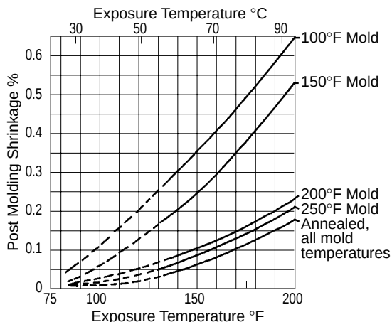
Fig. 18-7 Shrinkage for Delrin in Air
