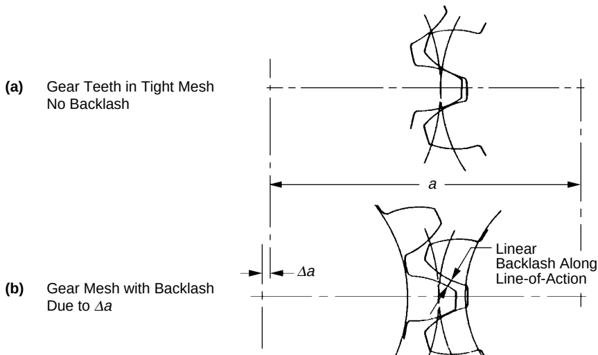
Figure 14-3 Backlash Caused by Opening of Center Distance
