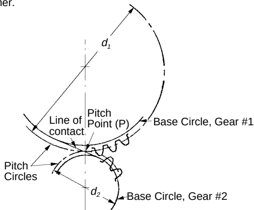
Fig. 2-4 Definition of Pitch Circle and Pitch Point
