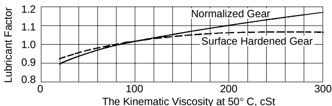
Fig. 17-3 Lubricant Factor, Z_L
