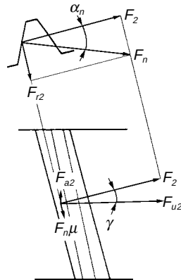
Fig. 16-14 Forces in a Worm Gear Mesh
