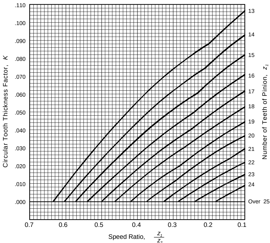
Fig. 10-2 Chart to Determine the Circular Tooth Thickness Factor K for Gleason Straight Bevel Gear
