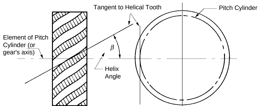
Fig. 6-3 Definition of Helix Angle
