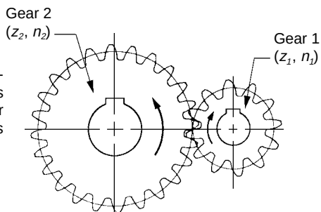
(a) A Pair of Spur Gears
