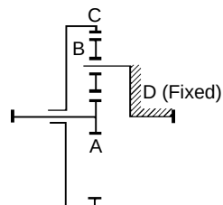
Fig. 13-6(c) Star Type Planetary Gear Mechanism
