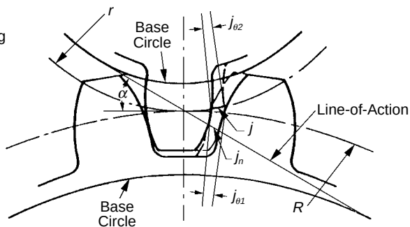
Fig. 14-2(b) Geometrical Definition of Linear Backlash
