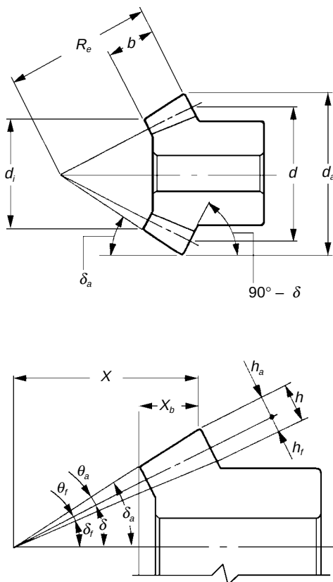
Fig. 8-9 Dimensions and Angles of Bevel Gear
