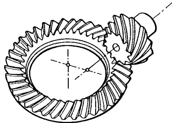
Fig. 2-21 Hypoid Gear
