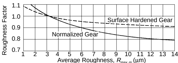
Fig. 17-4 Surface Roughness Factor, Z_R
