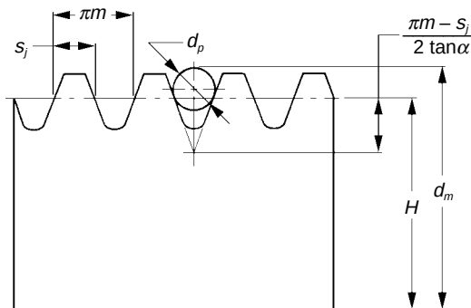
Fig. 10-9 Over Pins Measurement for a Rack Using a Pin or a Ball
