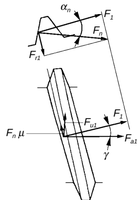
Fig. 16-12 Forces Acting on the Tooth Surface of a Worm
