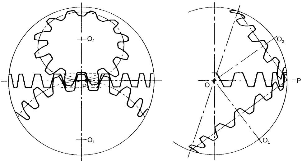
Fig. 8-3 Meshing Bevel Gear Pair with Conjugate Crown Gear
