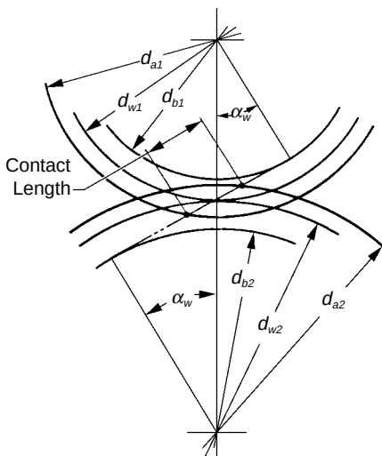
Fig. 11-2 Radial Contact Ratio of Parallel Axes Gear \epsilon_\alpha
