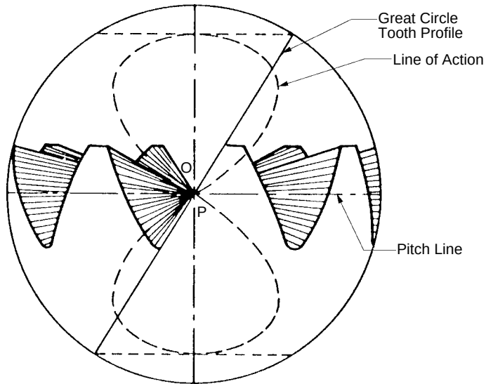
Fig. 8-4 Spherical Basis of Octoid Bevel Crown Gear
