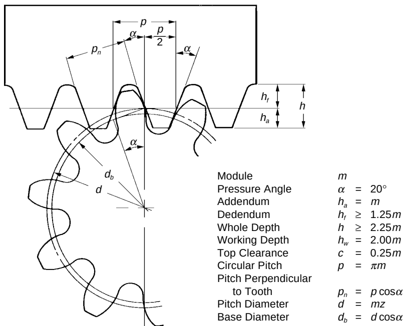
Fig. 2-7 The Tooth Profile and Dimension of Standard Rack
