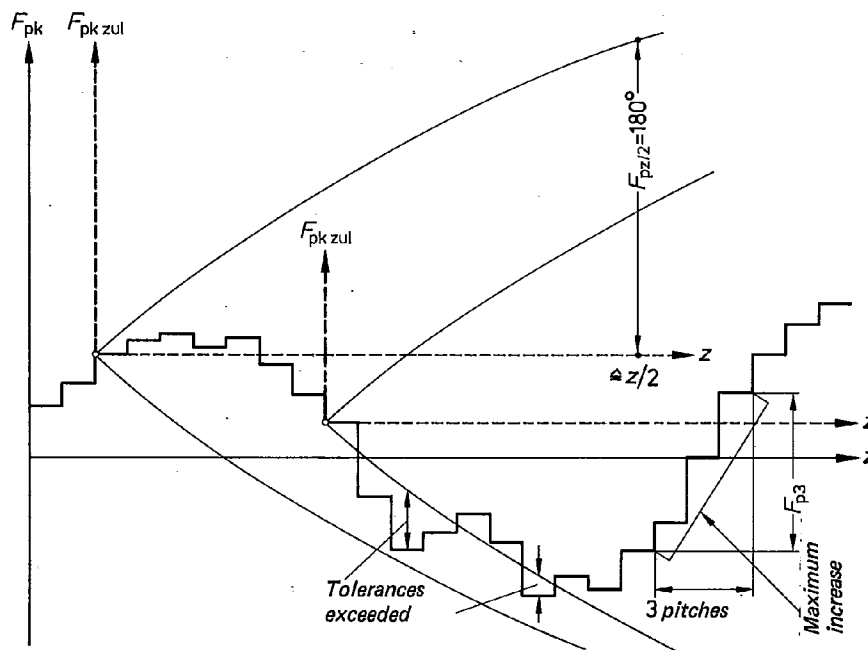
Figure 3. Evaluation of pitch-span measurement
