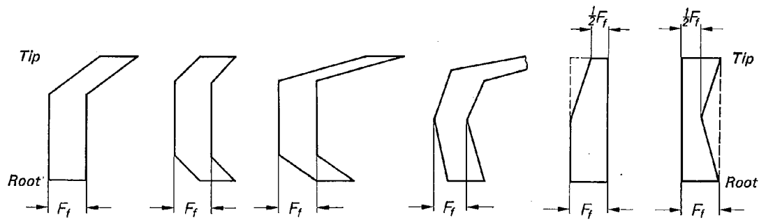
Figure 1. Altered pattern of permissible range of profile deviations (examples)
