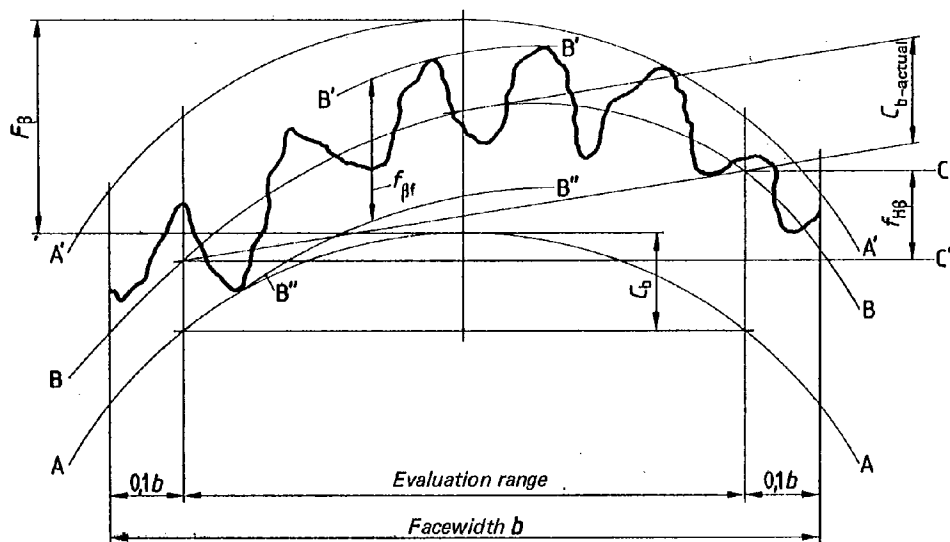
Figure 2. Tooth trace test pattern for narrowed tooth trace test range
