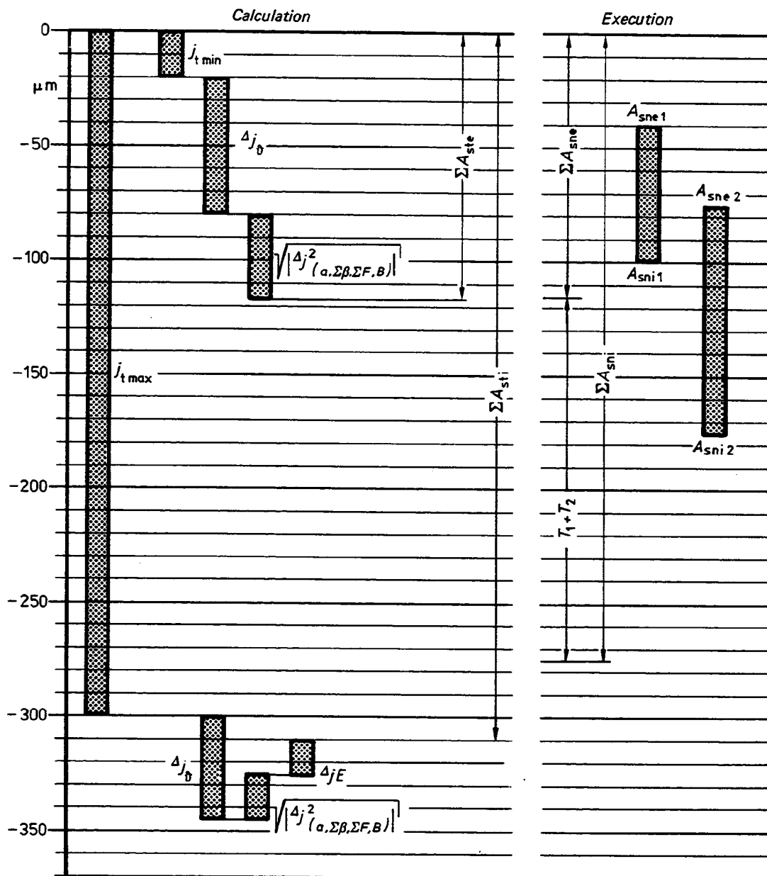
Figure A.3. Backlash, backlash modifications
