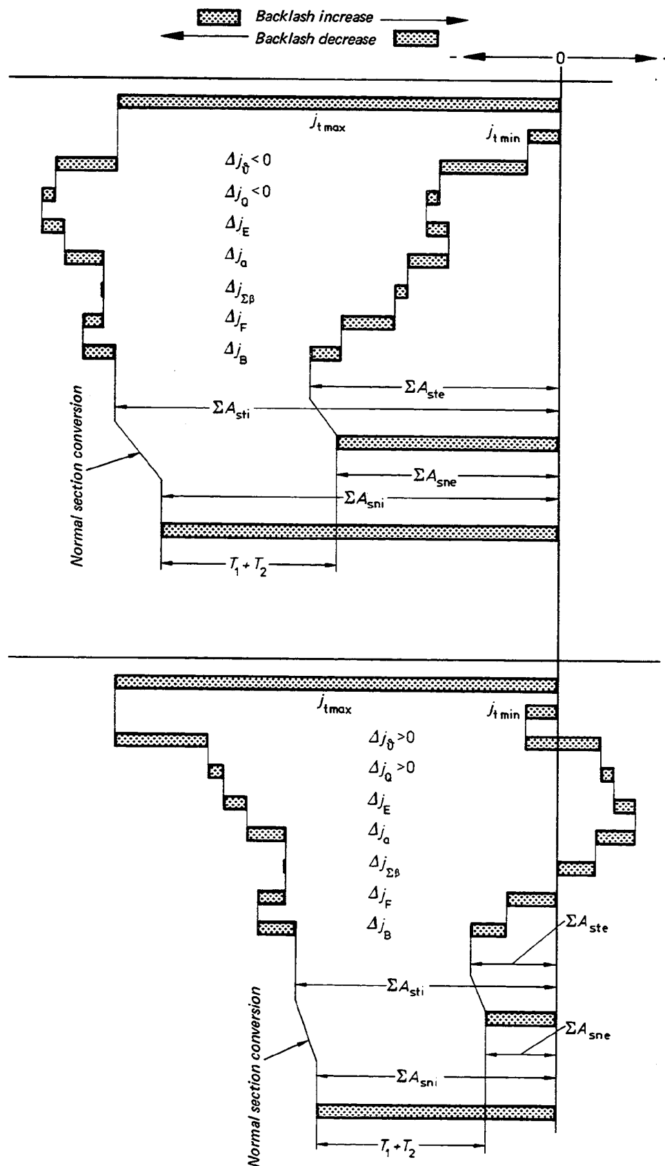
Figure A.2. Backlash-modifying effects and tooth thickness allowances under different conditions
