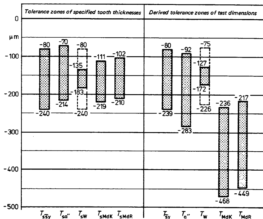
Figure B.3. Altered tolerance zones of tooth thickness and resulting tolerance zones of the test dimensions
