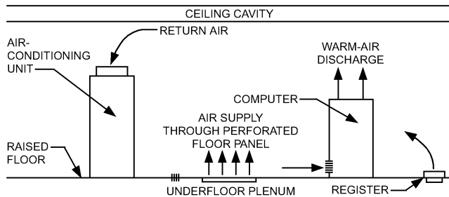
Fig. 4 Typical Underfloor Distribution
