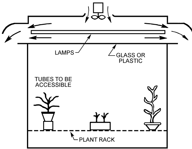
GROWTH CABINET – LIGHTS AIR-COOLED
