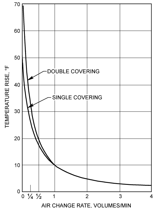
Fig. 10 Influence of Air Exchange Rate on Temperature Rise in Single- and Double-Covered Greenhouses
