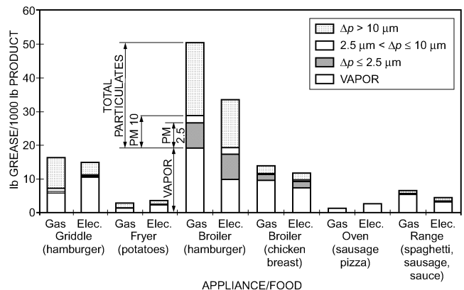
Fig. 1 Grease in Particle and Vapor Phases Emitted by Selected Commercial Cooking Appliances and Food Products Source: Kuehn et al. (1999)
