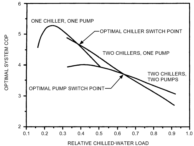
Fig. 7 Effect of Chiller and Pump Sequencing on Optimal Performance
