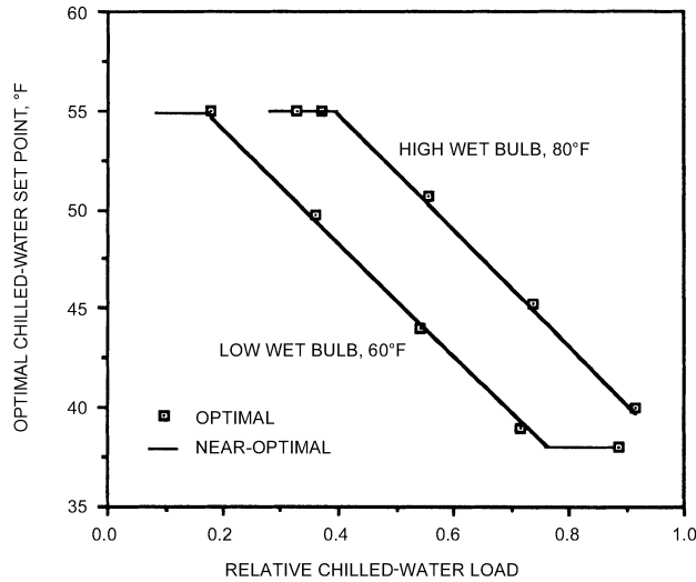
Fig. 25 Comparisons of Optimal Chilled-Water Temperature
