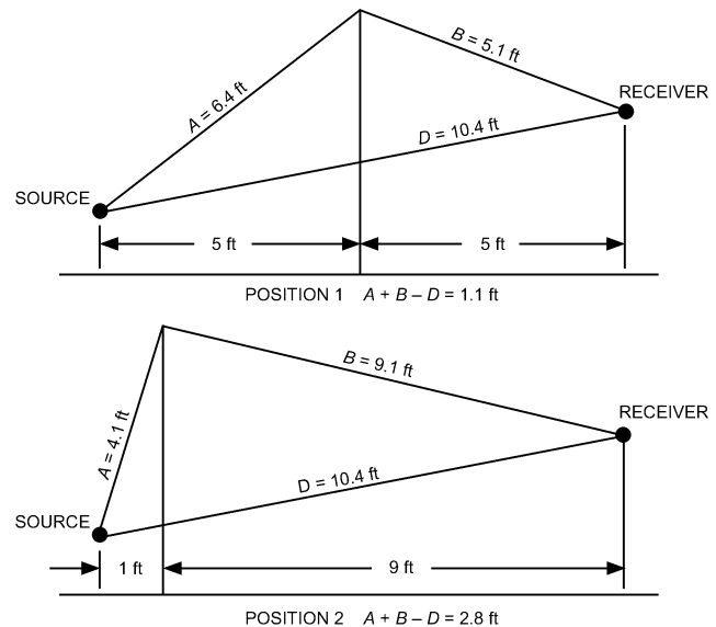
Fig. 32 Noise Barrier
