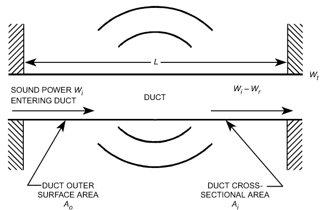
Fig. 24 Breakout Noise
