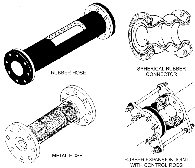
Fig. 43 Flexible Pipe Connectors
