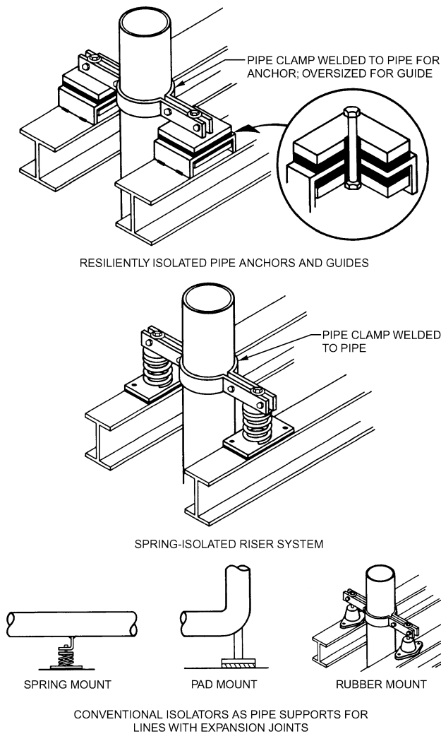
Fig. 41 Resilient Anchors and Guides for Pipes
