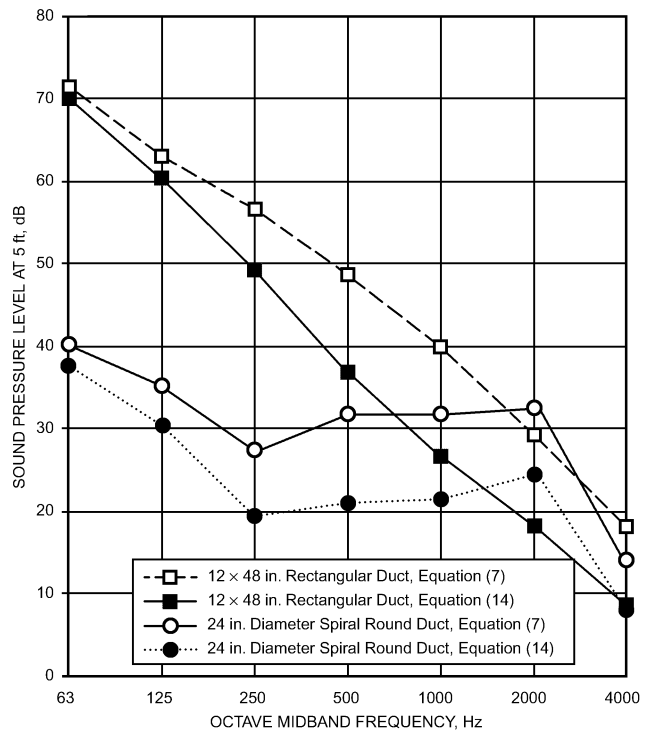
Fig. 27 Plotted Examples of Breakout Noise from Lined Duct
