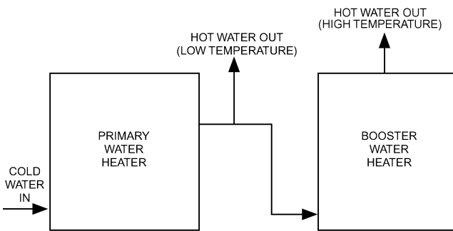
Fig. 5 Two-Temperature Service with Primary Heater and Booster Heater in Series
