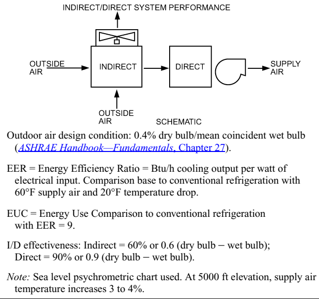
Fig. 3 Indirect/Direct Two-Stage System Performance
